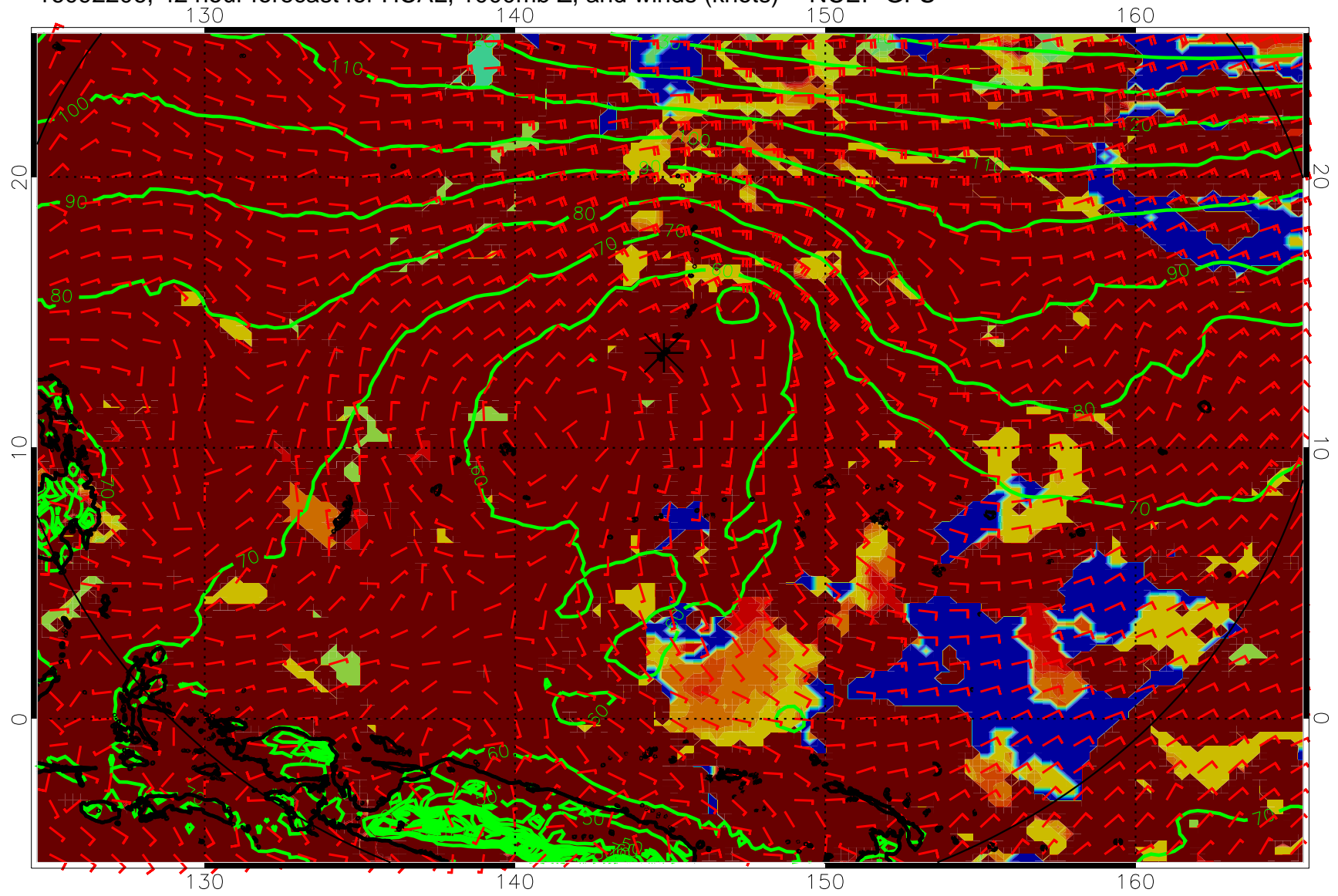
16092206, 42 hour forecast for HCAL, 1000mb Z, and winds (knots) -- NCEP GFS
