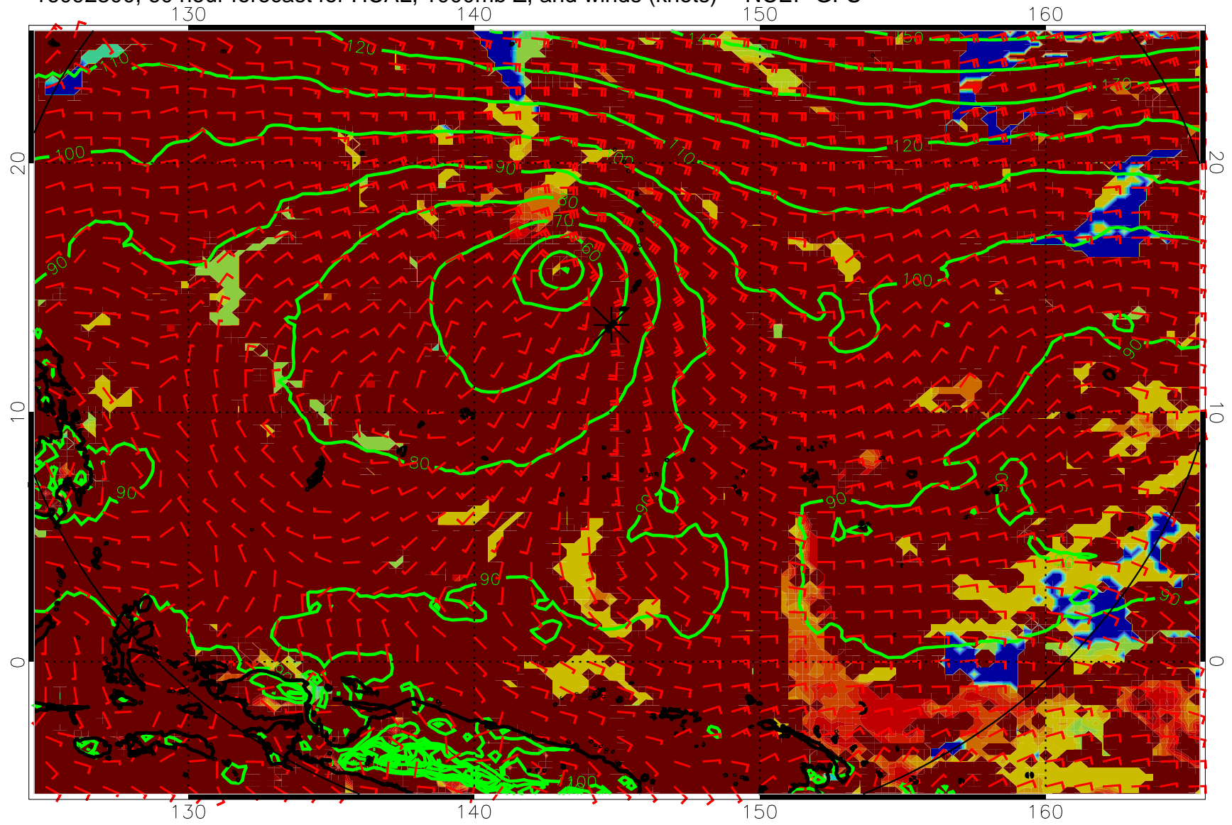
16092300, 60 hour forecast for HCAL, 1000mb Z, and winds (knots) -- NCEP GFS
