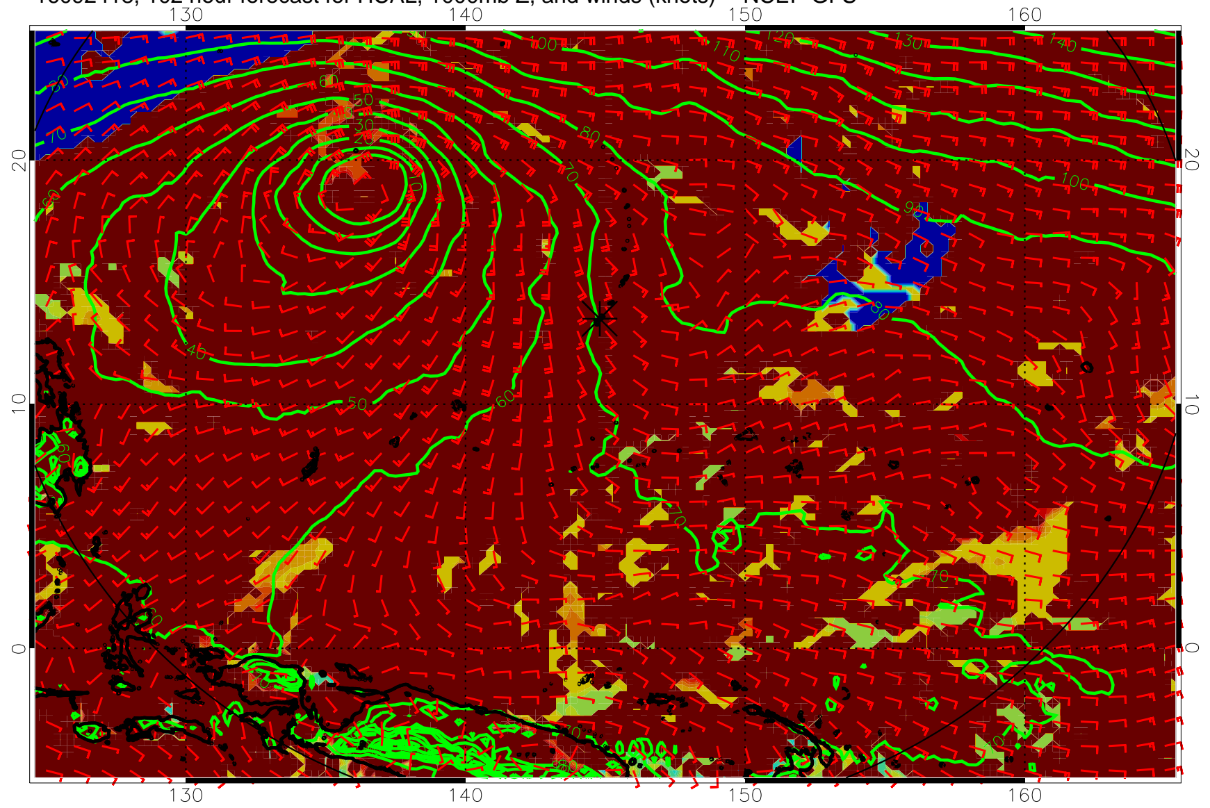
16092418, 102 hour forecast for HCAL, 1000mb Z, and winds (knots) -- NCEP GFS
