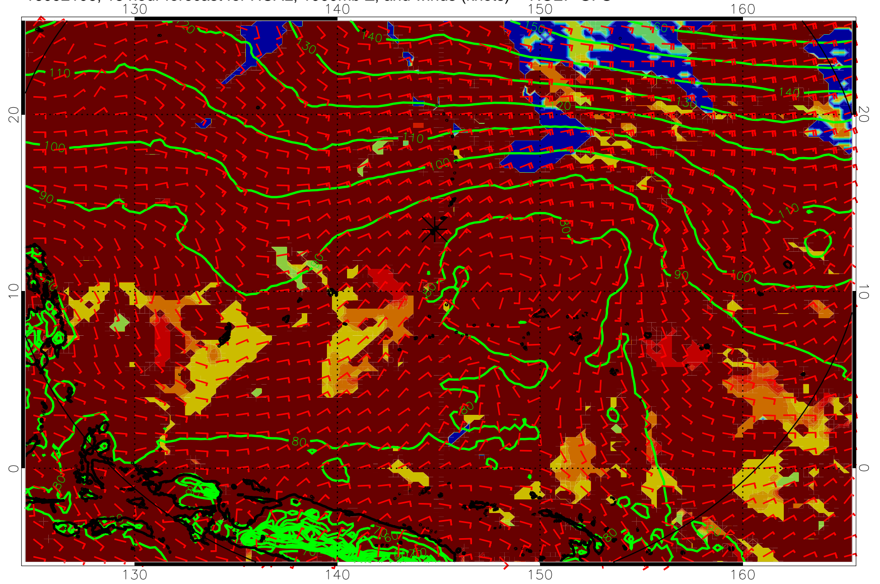
16092106, 18 hour forecast for HCAL, 1000mb Z, and winds (knots) -- NCEP GFS
