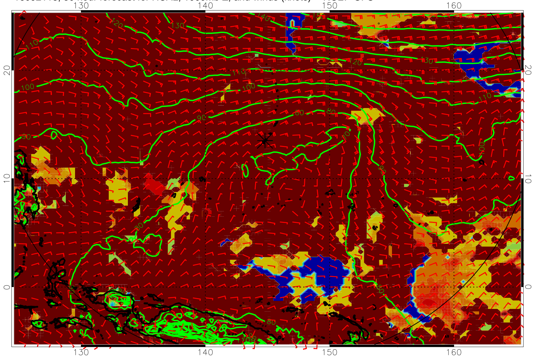
16092118, 30 hour forecast for HCAL, 1000mb Z, and winds (knots) -- NCEP GFS
