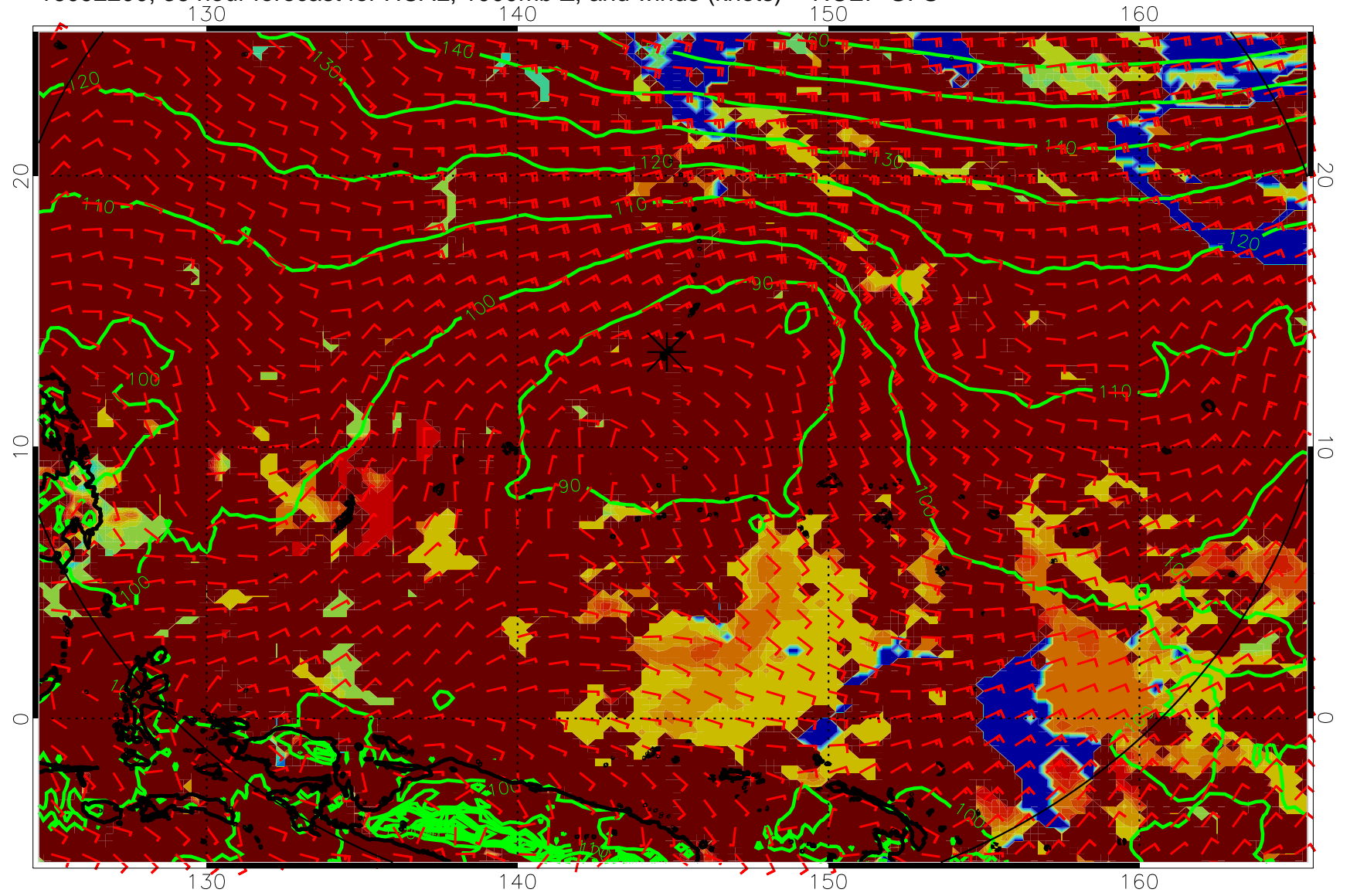
16092200, 36 hour forecast for HCAL, 1000mb Z, and winds (knots) -- NCEP GFS
