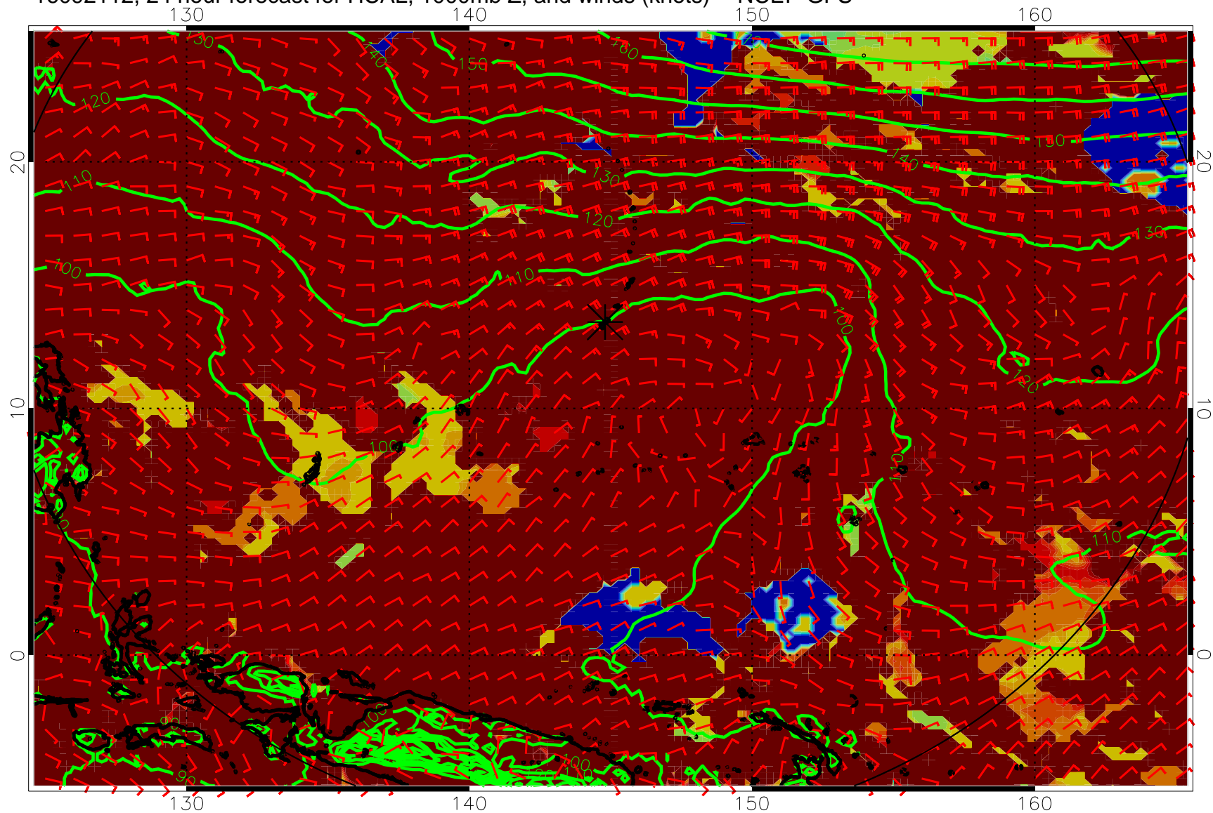
16092112, 24 hour forecast for HCAL, 1000mb Z, and winds (knots) -- NCEP GFS
