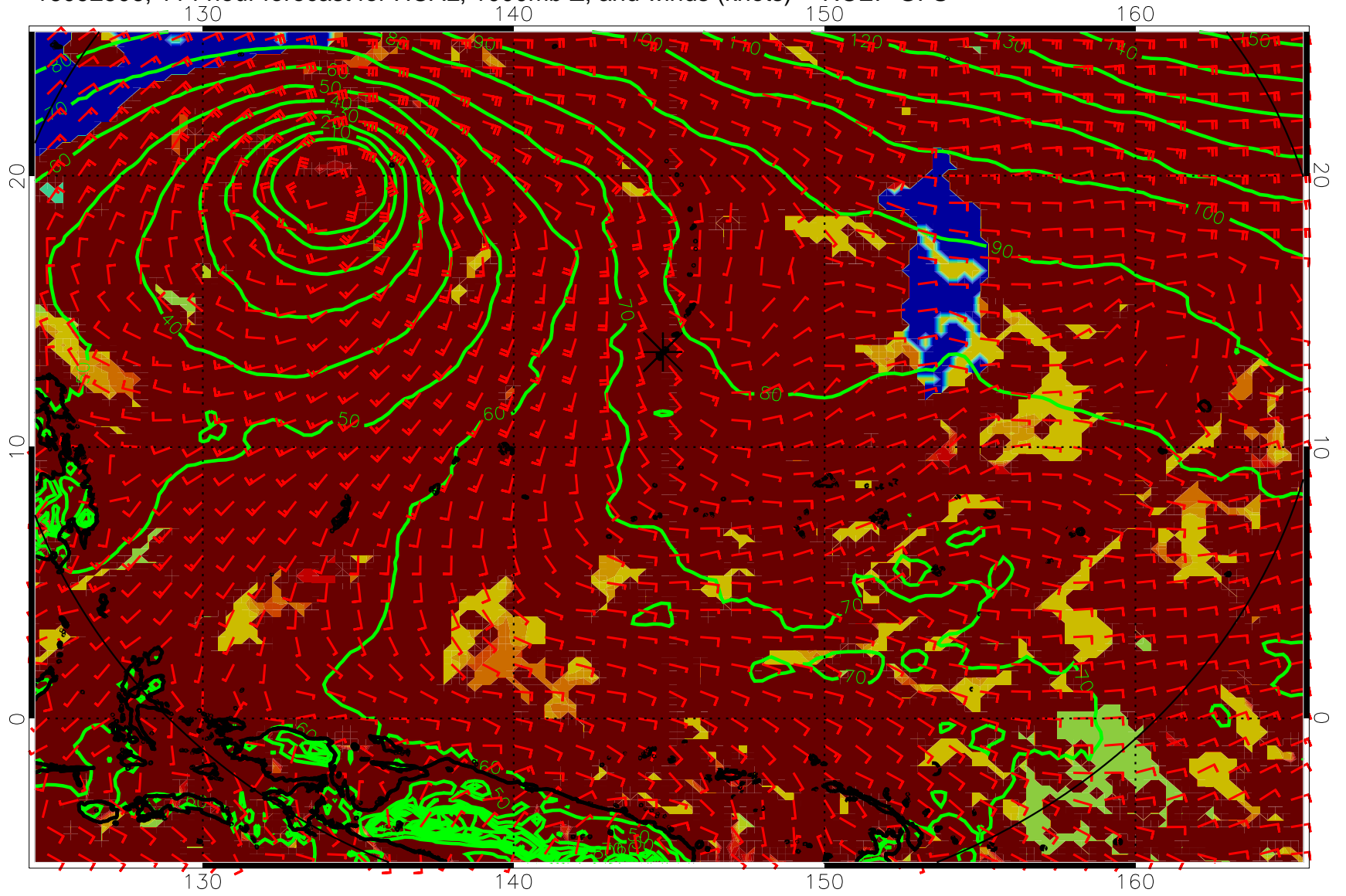
16092506, 114 hour forecast for HCAL, 1000mb Z, and winds (knots) -- NCEP GFS
