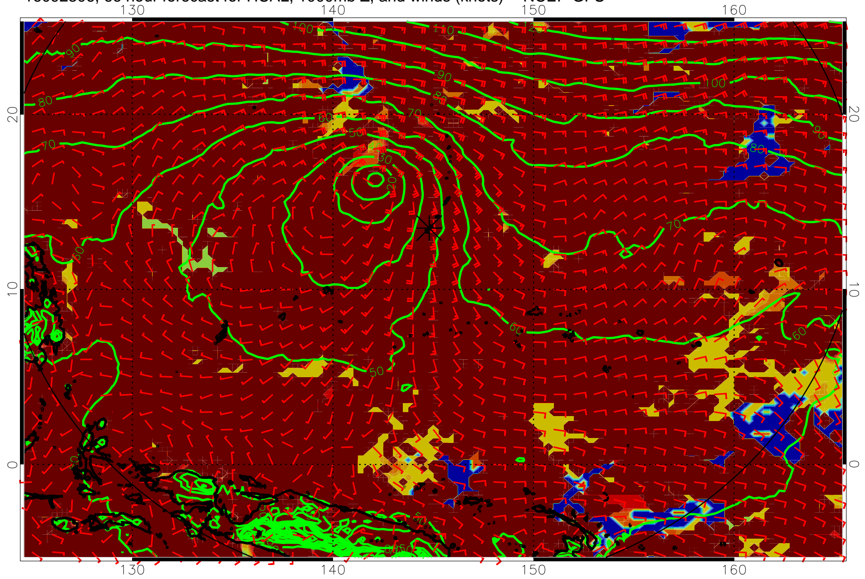
16092306, 66 hour forecast for HCAL, 1000mb Z, and winds (knots) -- NCEP GFS
