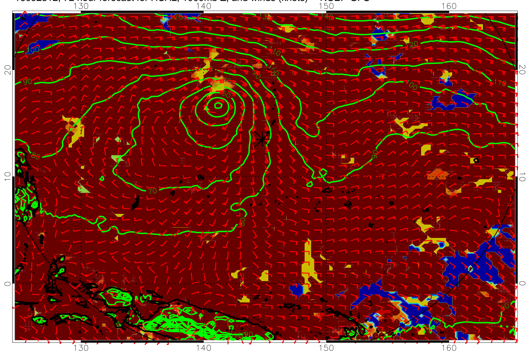
16092312, 72 hour forecast for HCAL, 1000mb Z, and winds (knots) -- NCEP GFS
