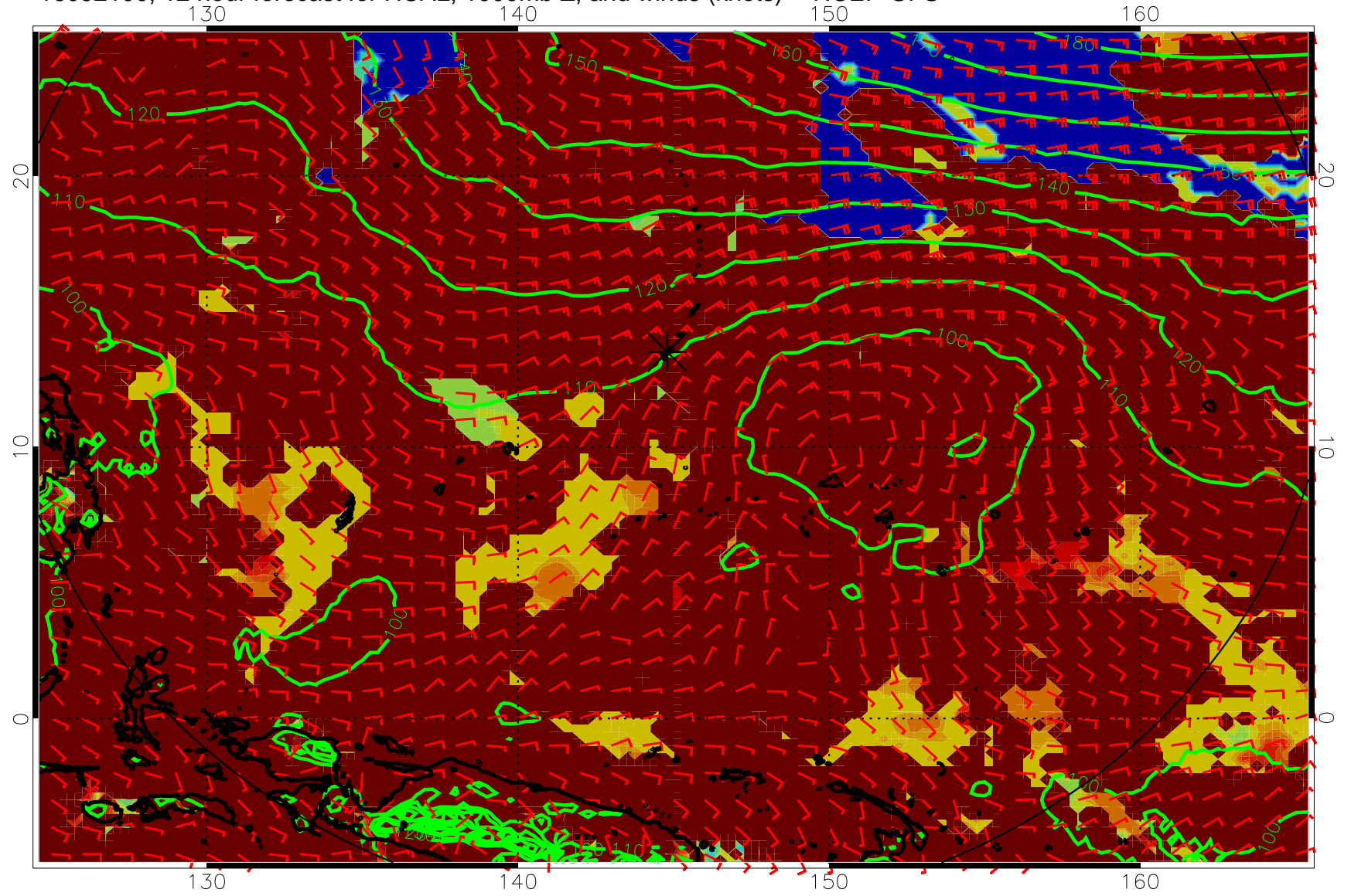
16092100, 12 hour forecast for HCAL, 1000mb Z, and winds (knots) -- NCEP GFS
