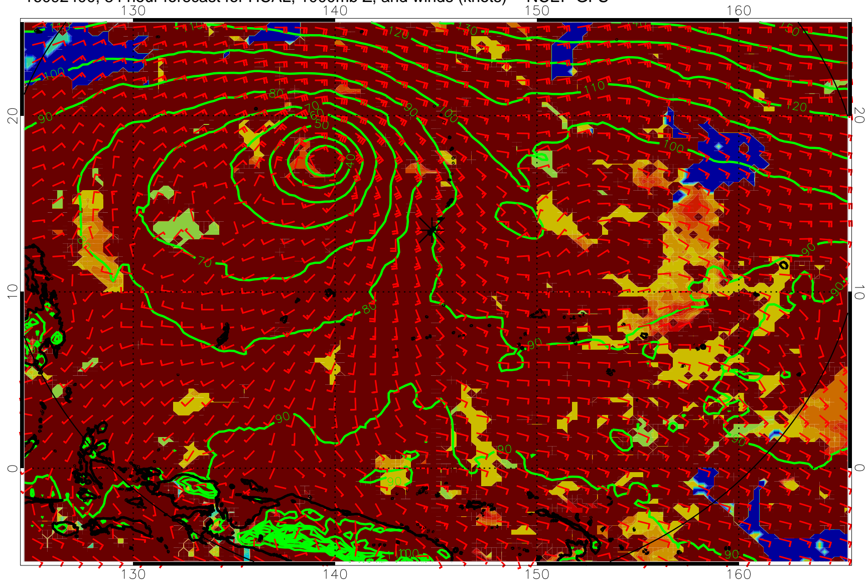
16092400, 84 hour forecast for HCAL, 1000mb Z, and winds (knots) -- NCEP GFS
