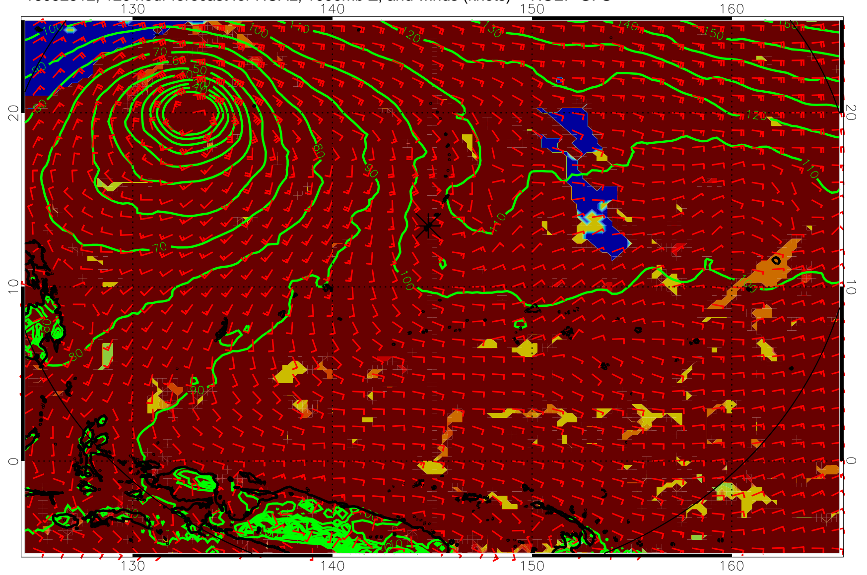
16092512, 120 hour forecast for HCAL, 1000mb Z, and winds (knots) -- NCEP GFS
