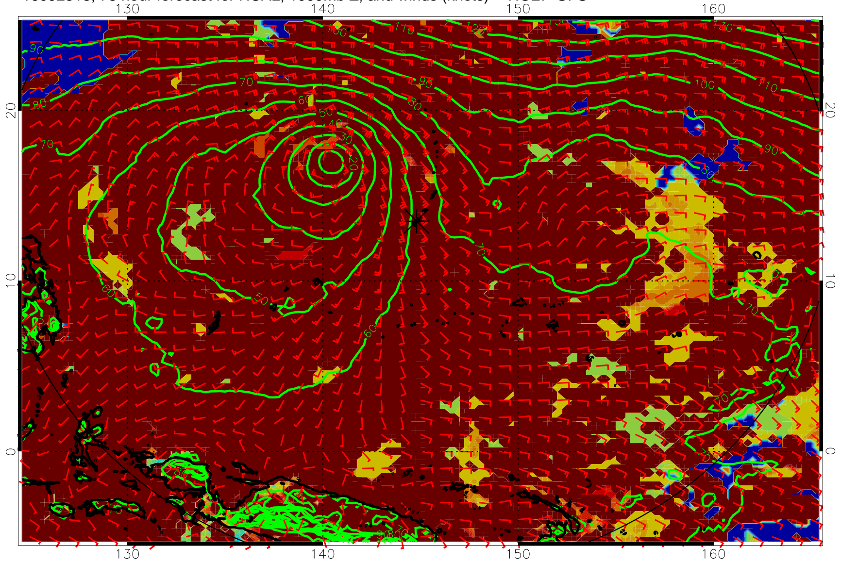
16092318, 78 hour forecast for HCAL, 1000mb Z, and winds (knots) -- NCEP GFS
