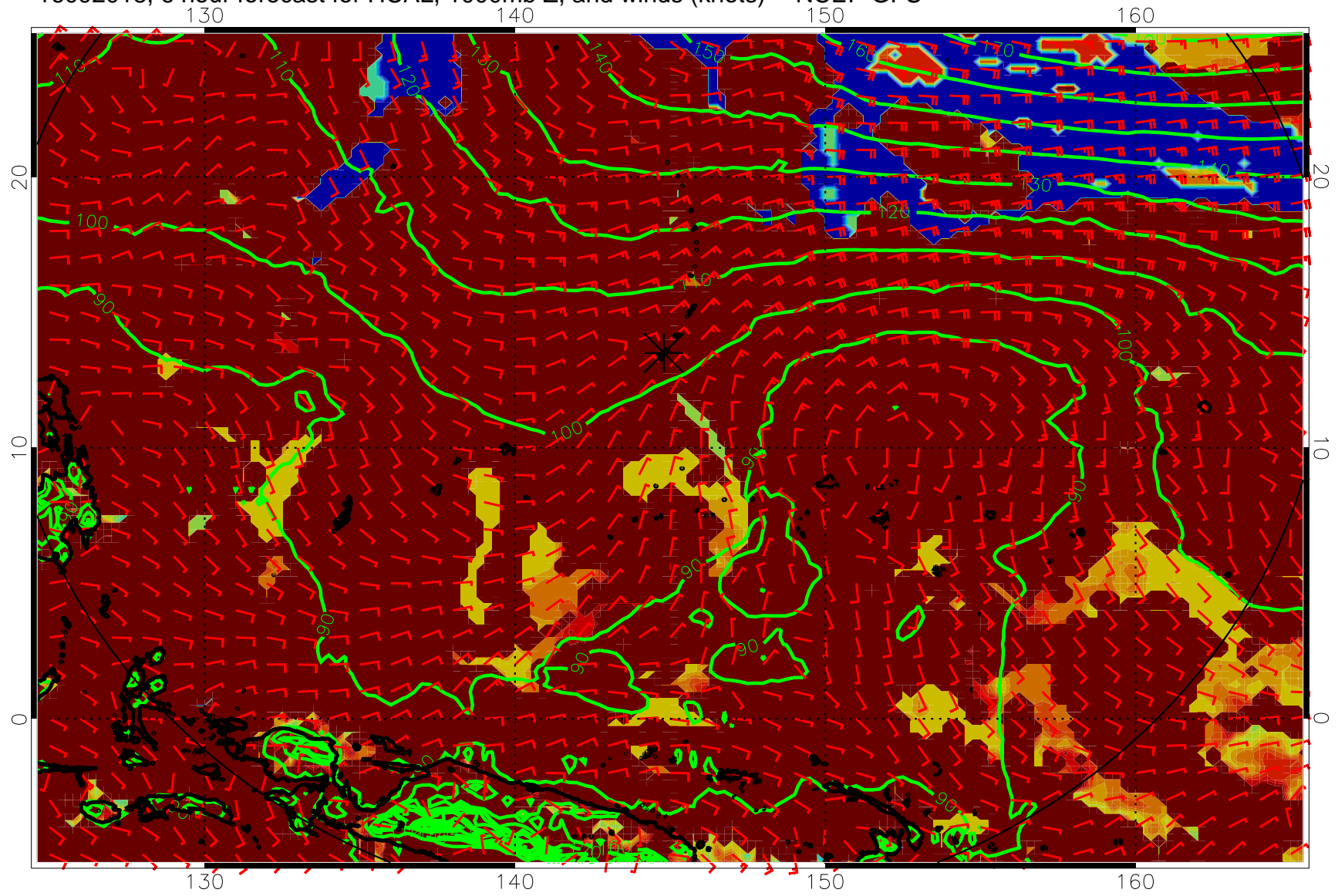
16092018, 6 hour forecast for HCAL, 1000mb Z, and winds (knots) -- NCEP GFS
