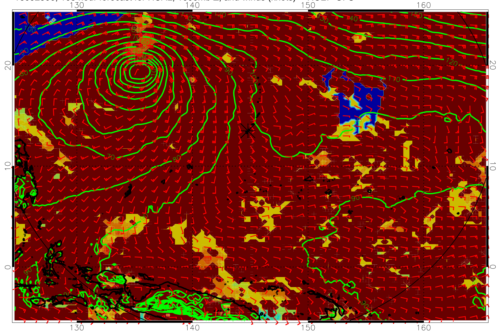
16092500, 108 hour forecast for HCAL, 1000mb Z, and winds (knots) -- NCEP GFS
