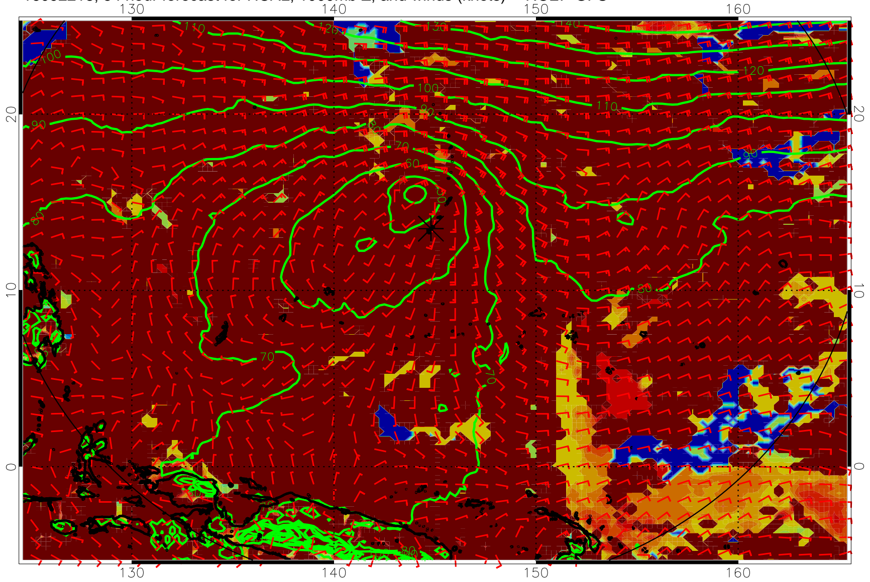
16092218, 54 hour forecast for HCAL, 1000mb Z, and winds (knots) -- NCEP GFS
