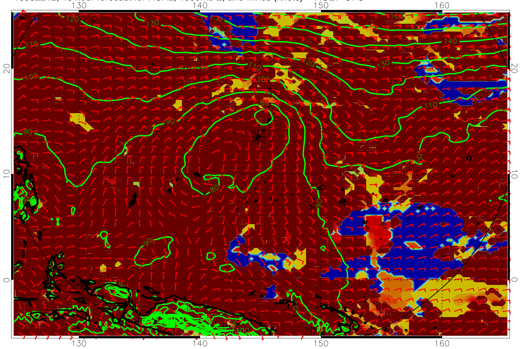
16092212, 48 hour forecast for HCAL, 1000mb Z, and winds (knots) -- NCEP GFS
