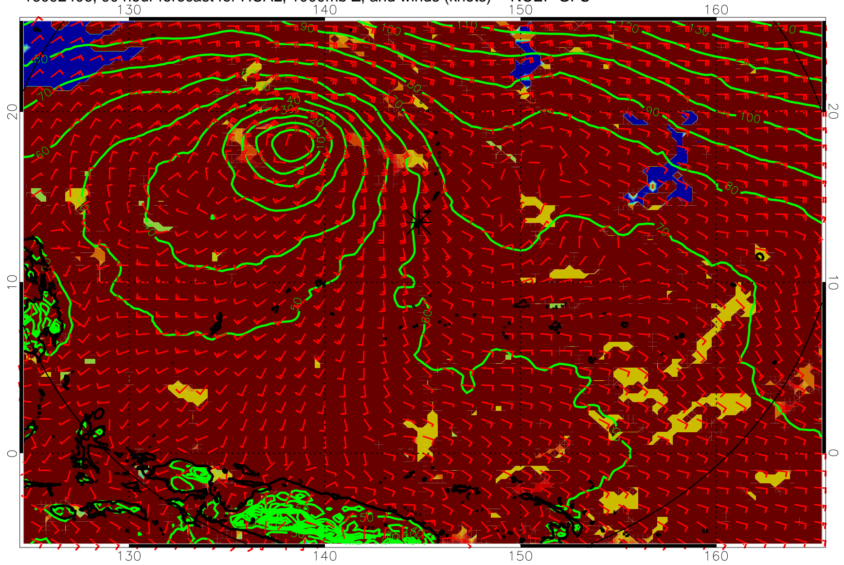
16092406, 90 hour forecast for HCAL, 1000mb Z, and winds (knots) -- NCEP GFS
