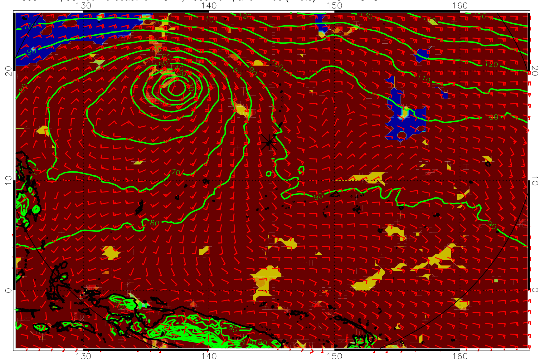
16092412, 96 hour forecast for HCAL, 1000mb Z, and winds (knots) -- NCEP GFS
