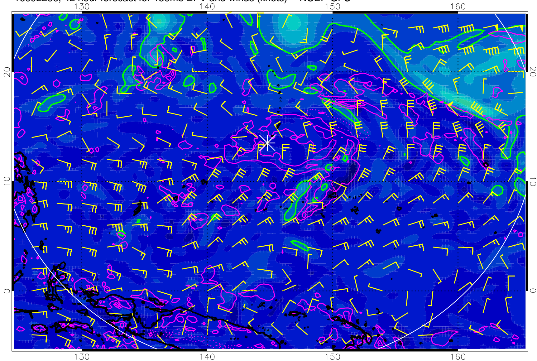
16092206, 42 hour forecast for 150mb EPV and winds (knots) -- NCEP GFS
