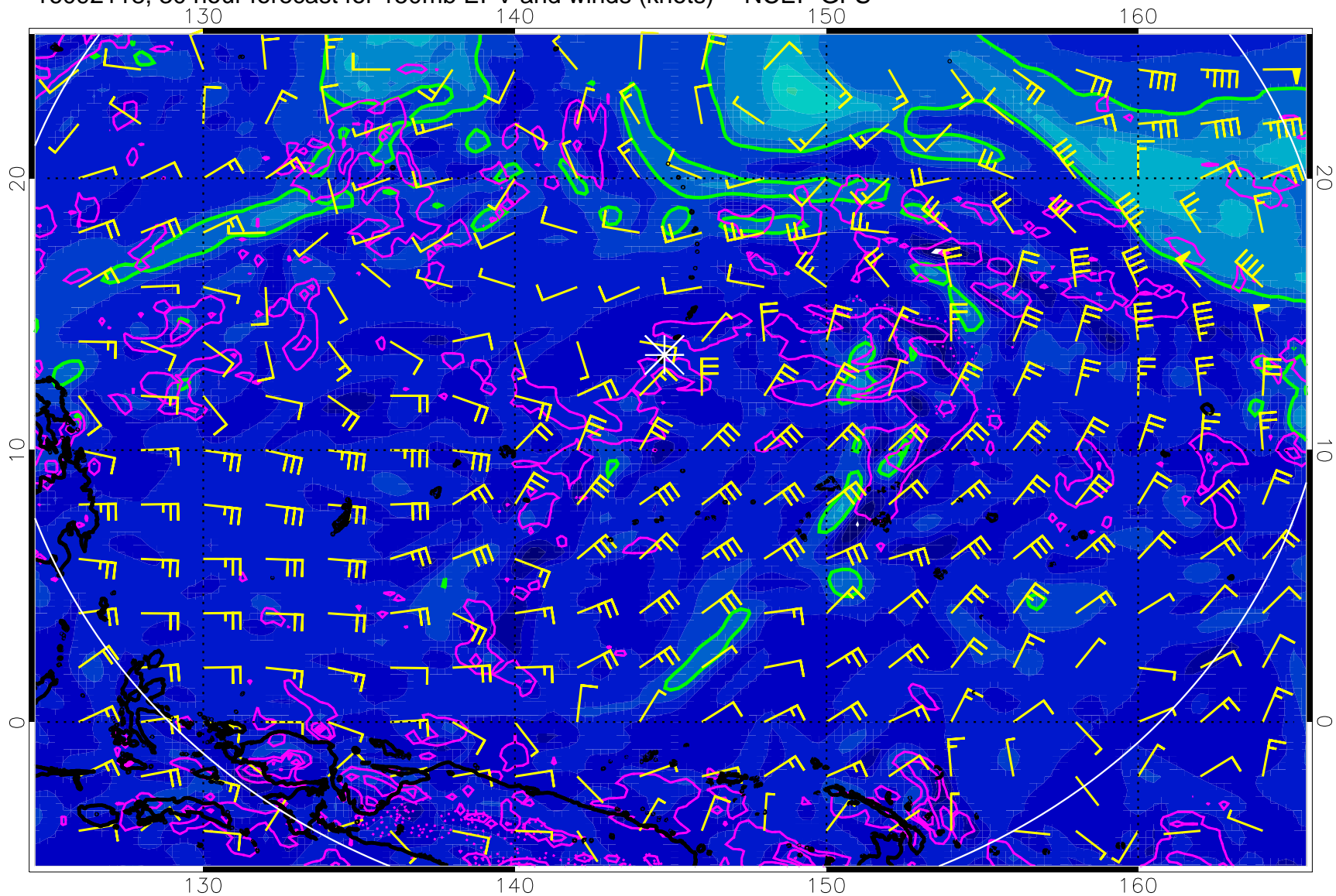
16092118, 30 hour forecast for 150mb EPV and winds (knots) -- NCEP GFS
