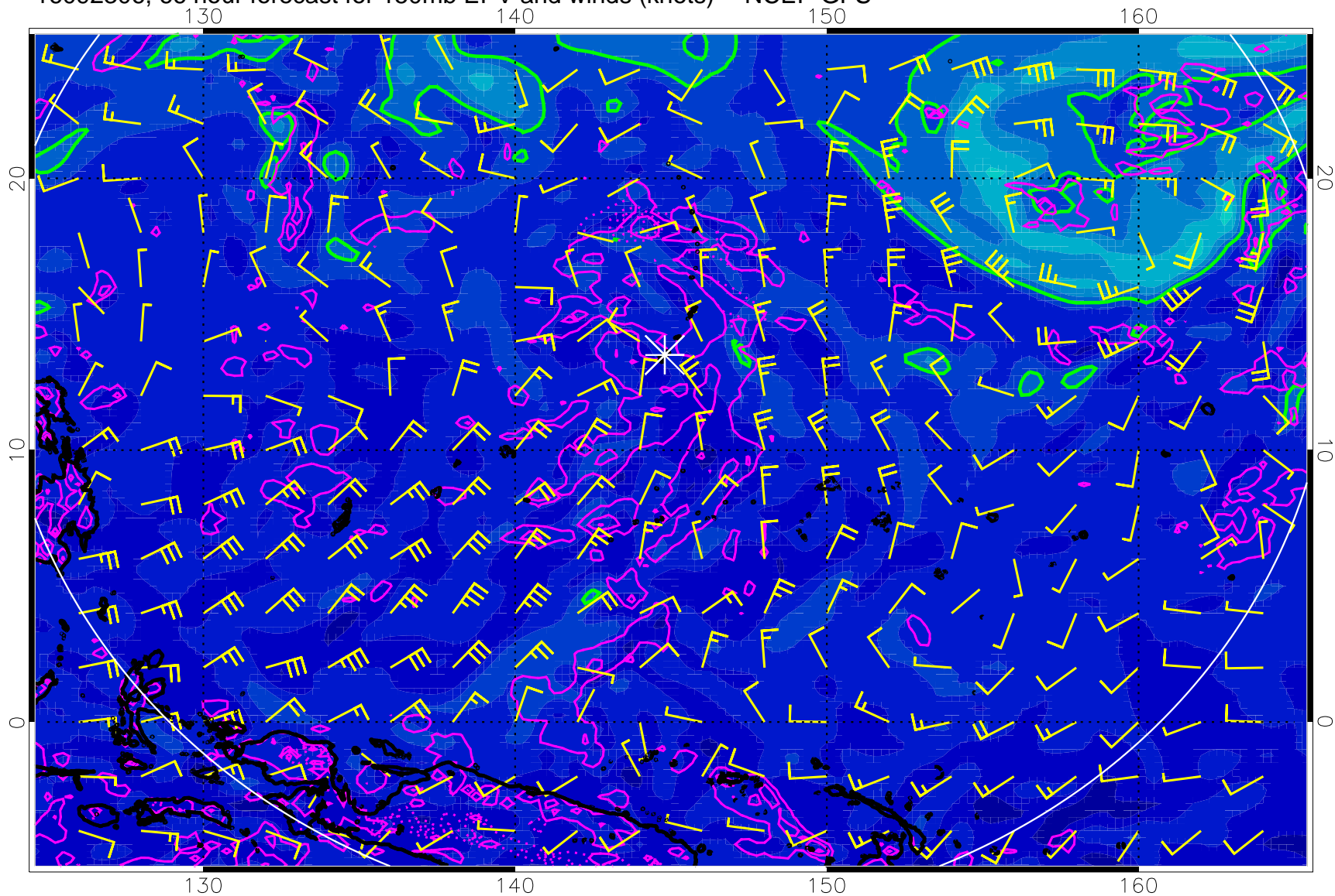
16092306, 66 hour forecast for 150mb EPV and winds (knots) -- NCEP GFS
