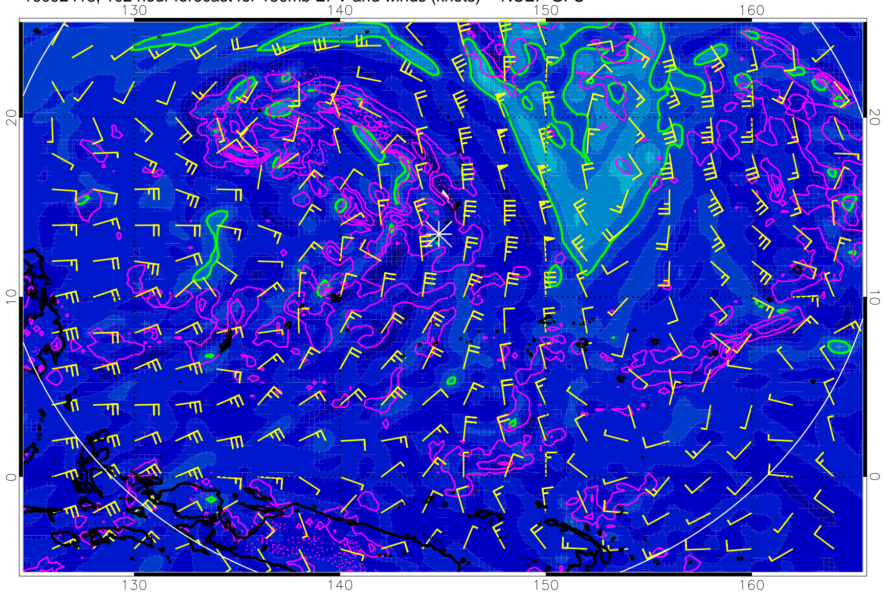
16092418, 102 hour forecast for 150mb EPV and winds (knots) -- NCEP GFS
