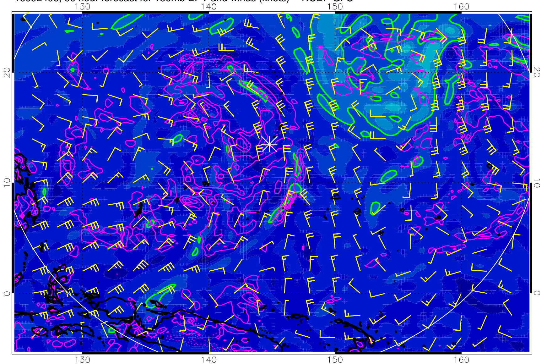
16092406, 90 hour forecast for 150mb EPV and winds (knots) -- NCEP GFS
