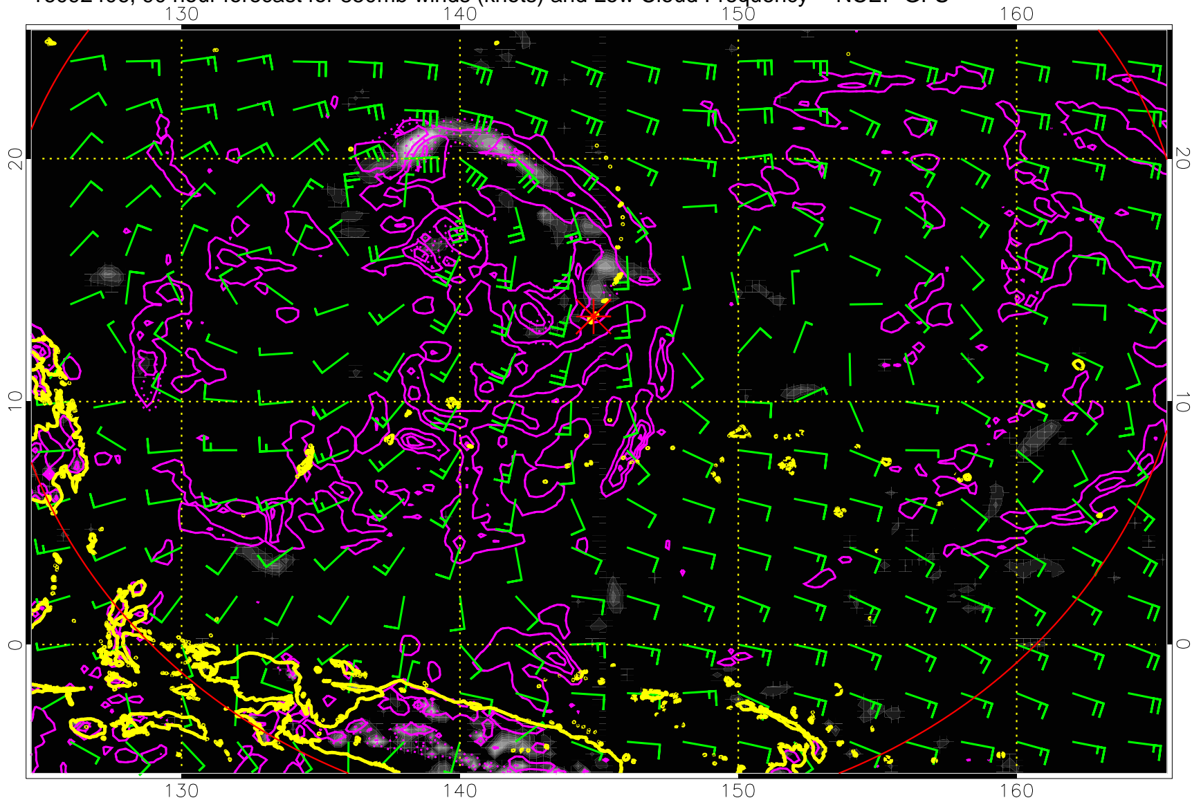
16092406, 90 hour forecast for 850mb winds (knots) and Low Cloud Frequency -- NCEP GFS
