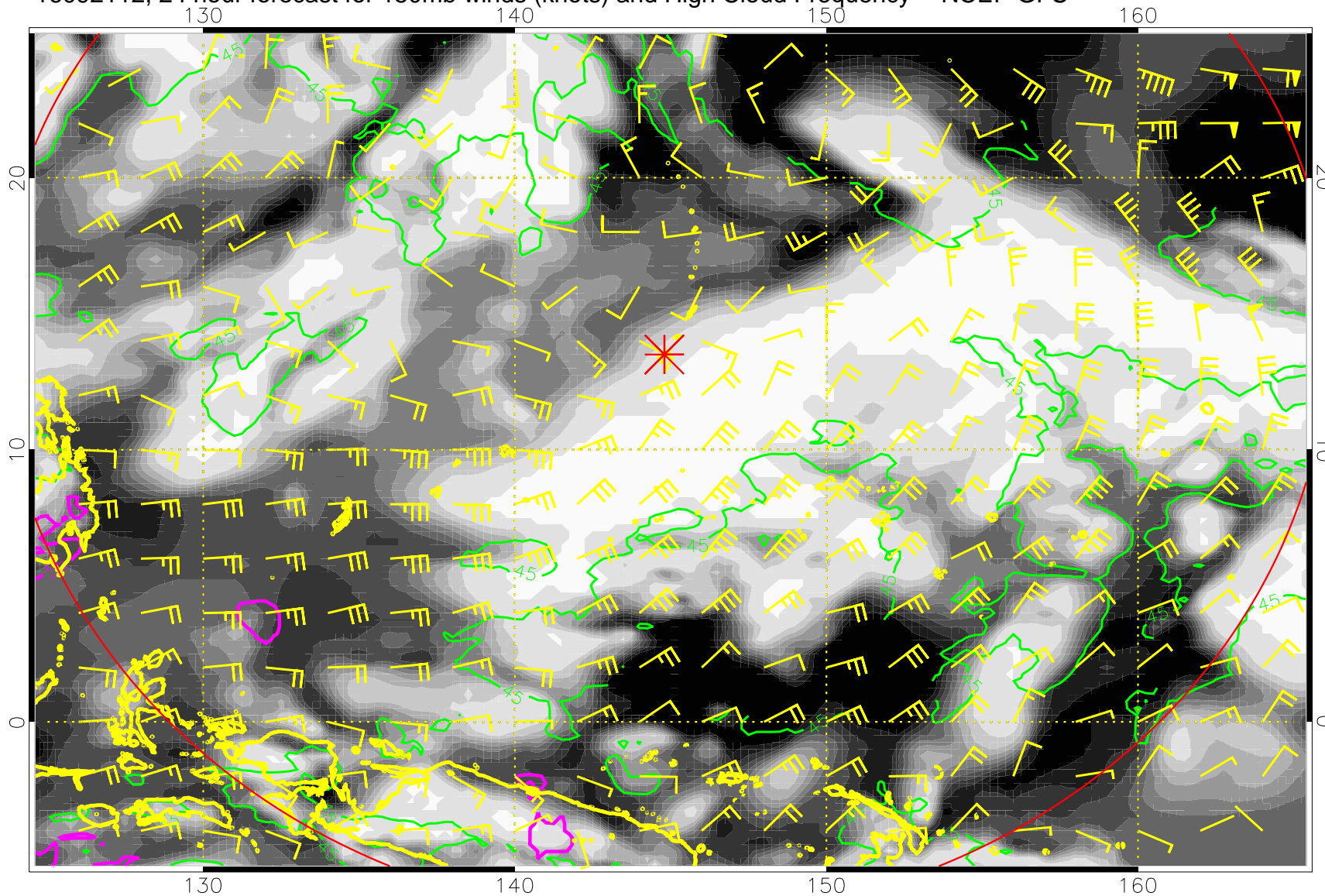
16092112, 24 hour forecast for 150mb winds (knots) and High Cloud Frequency -- NCEP GFS
