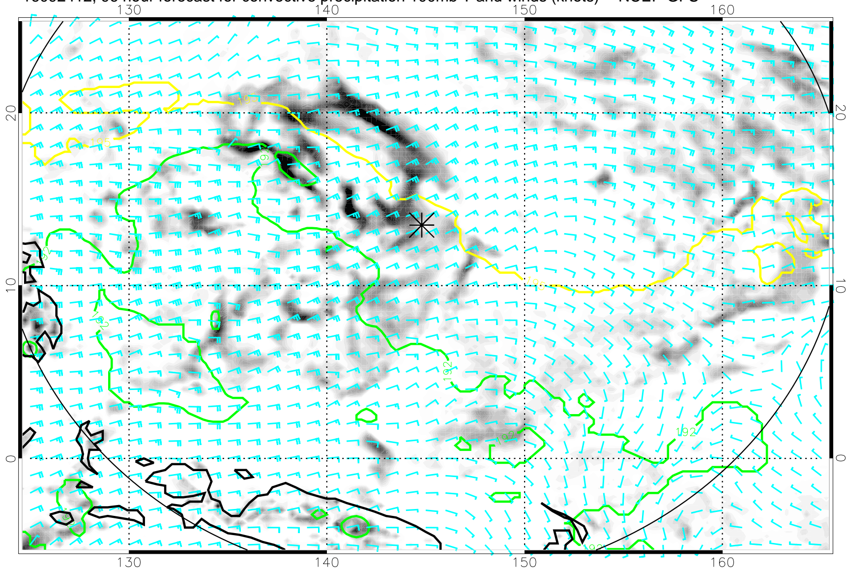
16092412, 96 hour forecast for convective precipitation 100mb T and winds (knots) -- NCEP GFS
