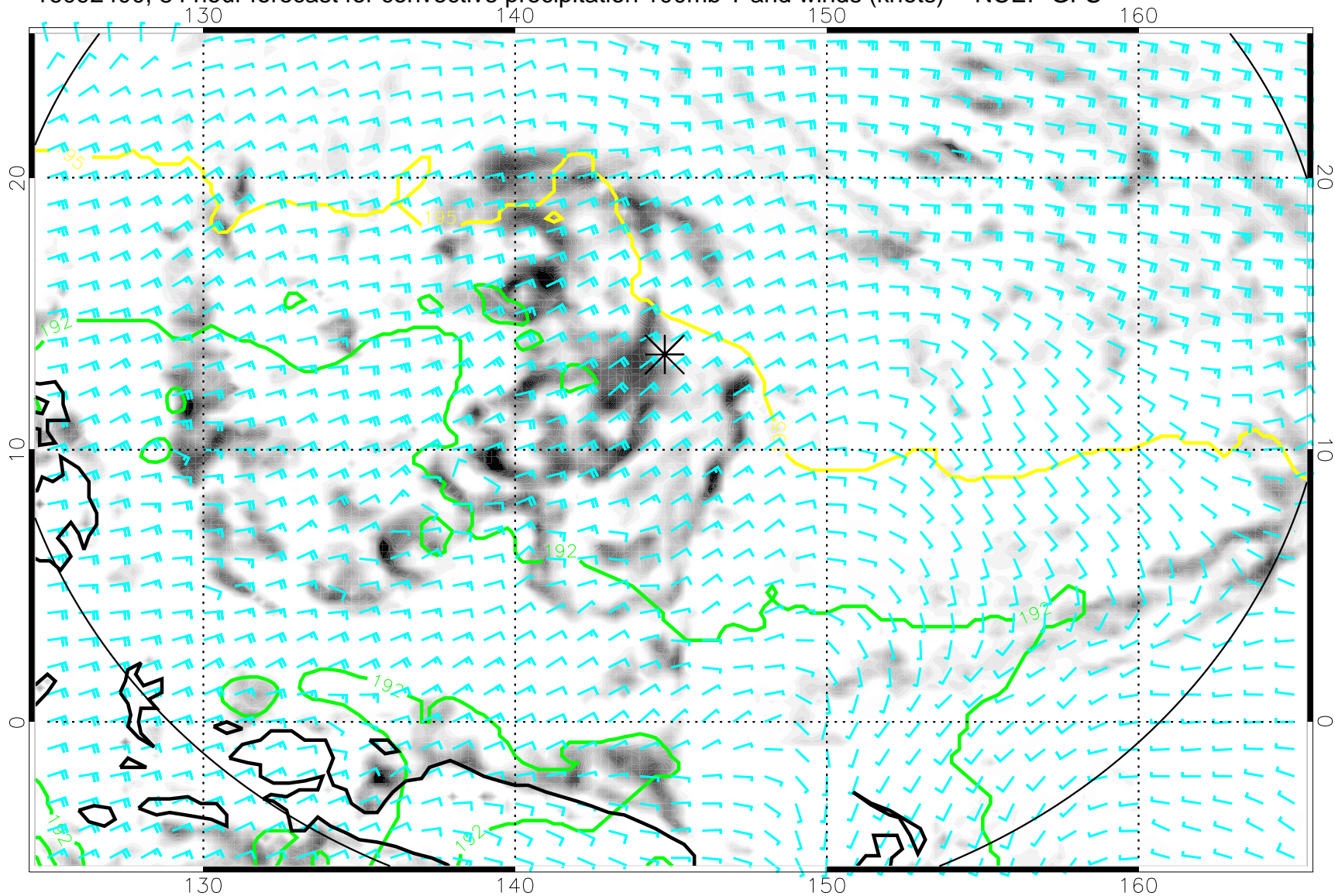
16092400, 84 hour forecast for convective precipitation 100mb T and winds (knots) -- NCEP GFS
