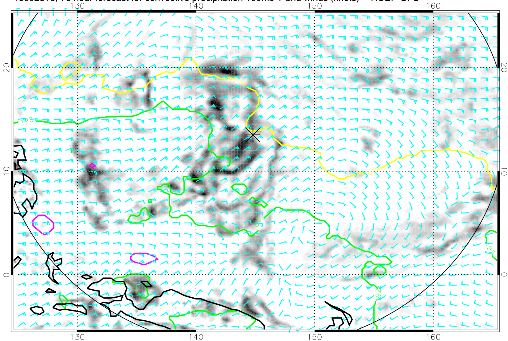
16092318, 78 hour forecast for convective precipitation 100mb T and winds (knots) -- NCEP GFS
