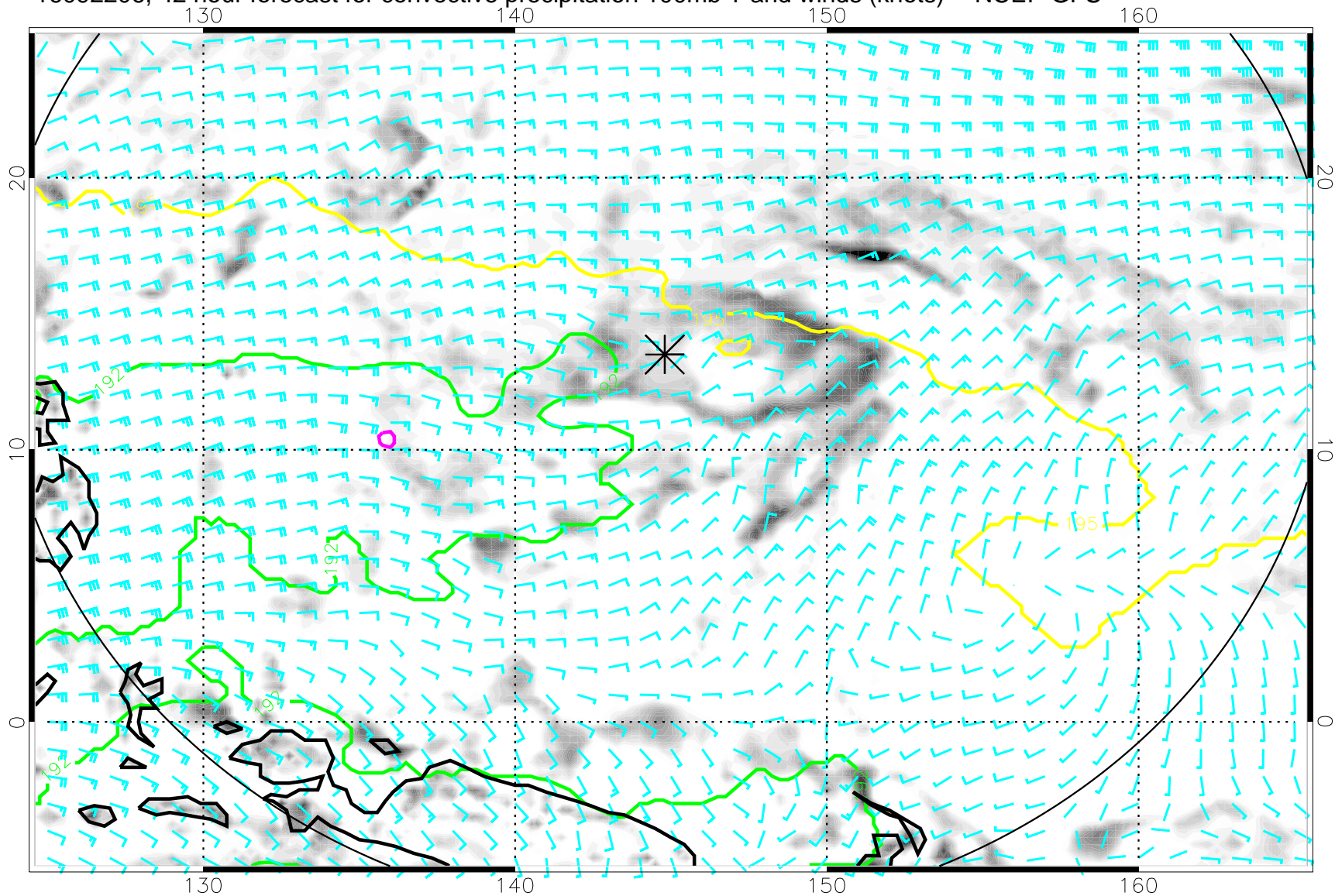
16092206, 42 hour forecast for convective precipitation 100mb T and winds (knots) -- NCEP GFS
