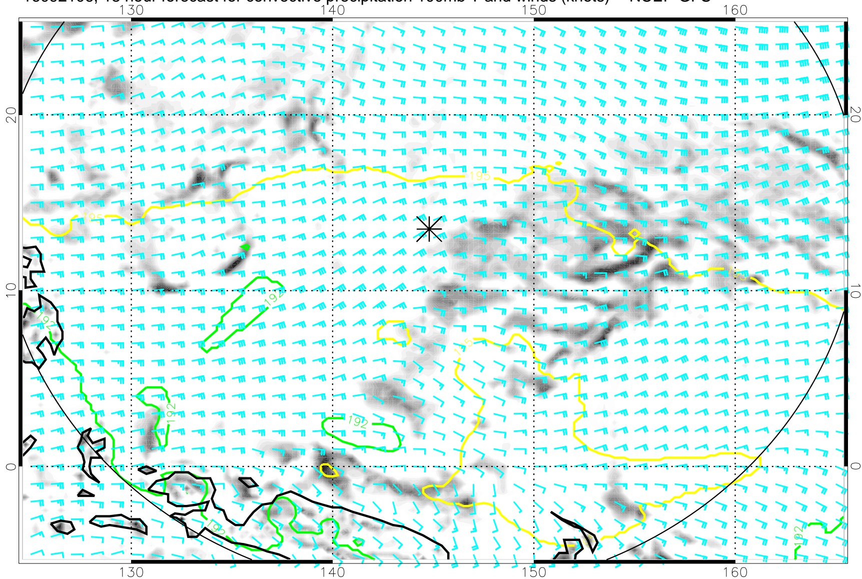
16092106, 18 hour forecast for convective precipitation 100mb T and winds (knots) -- NCEP GFS
