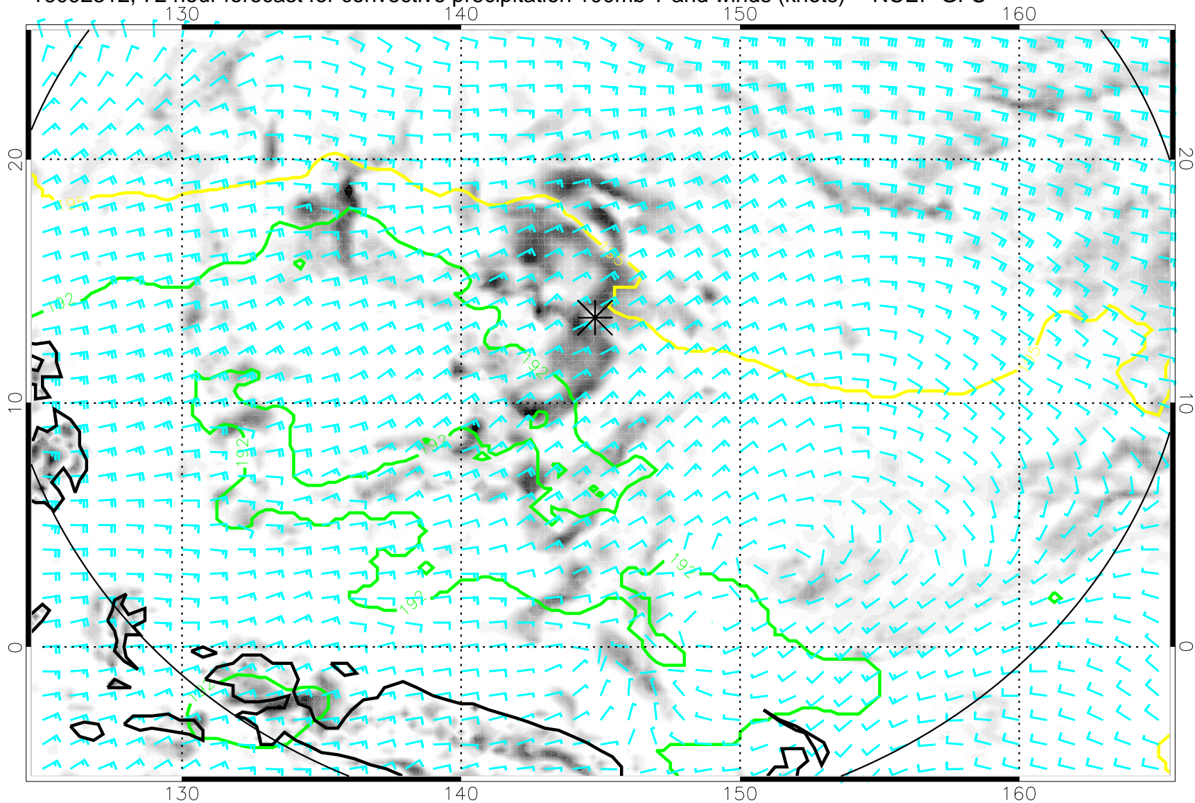
16092312, 72 hour forecast for convective precipitation 100mb T and winds (knots) -- NCEP GFS
