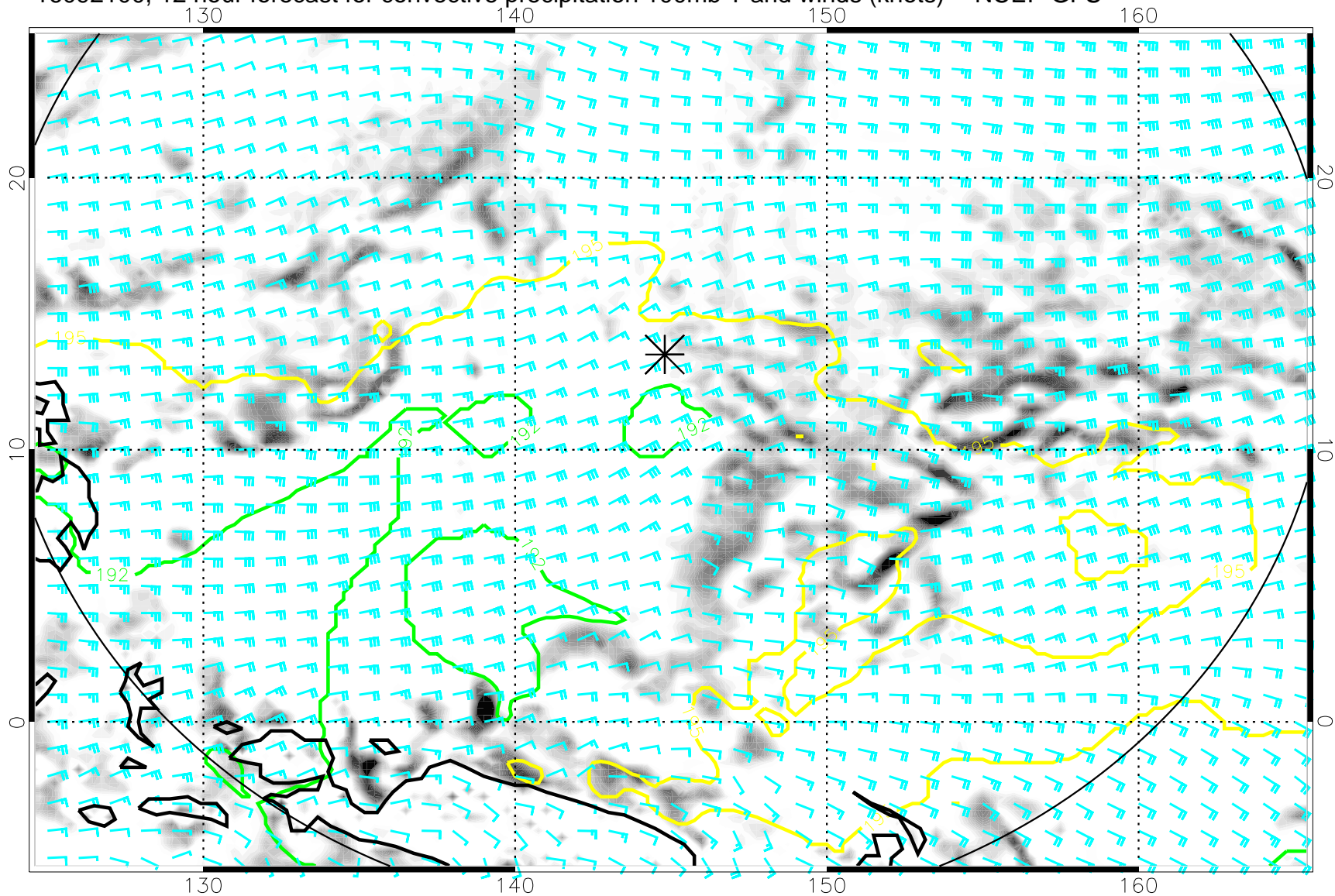
16092100, 12 hour forecast for convective precipitation 100mb T and winds (knots) -- NCEP GFS
