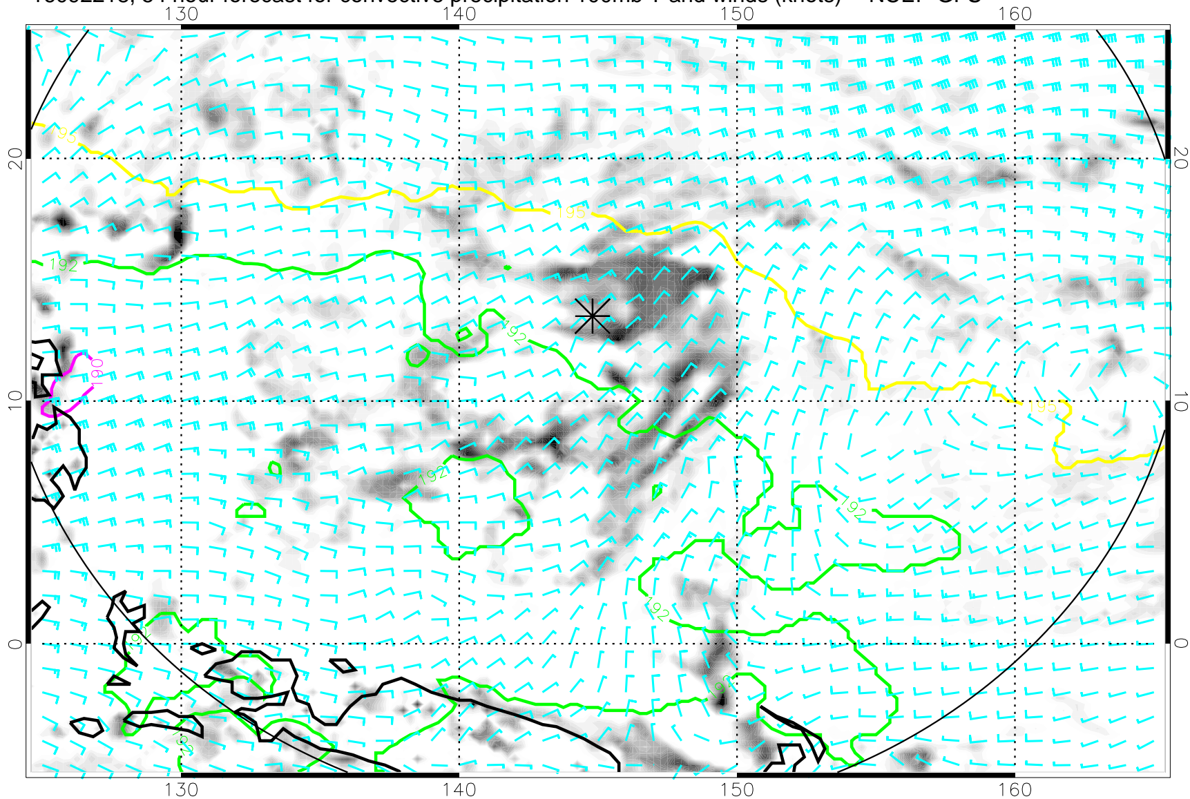
16092218, 54 hour forecast for convective precipitation 100mb T and winds (knots) -- NCEP GFS
