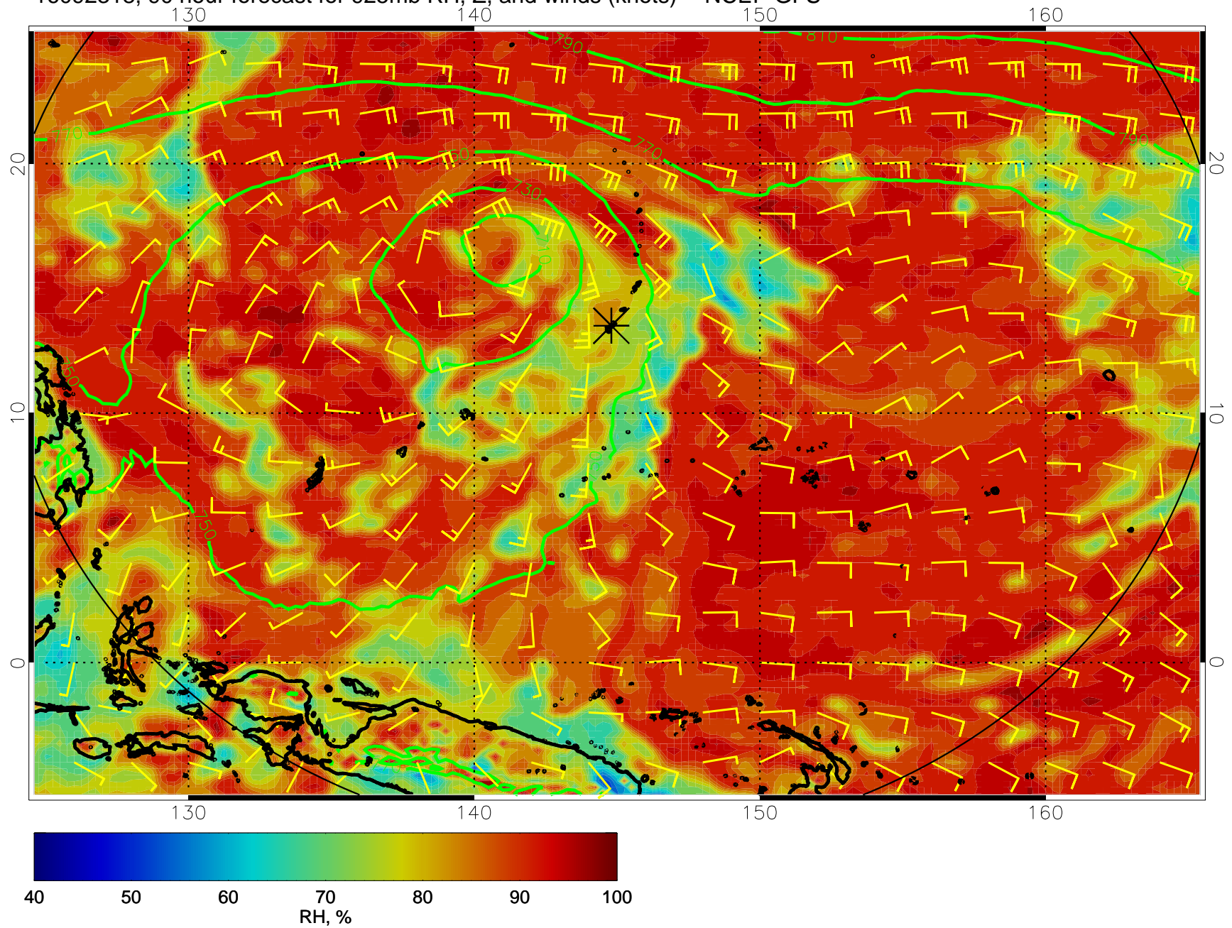
16092318, 90 hour forecast for 925mb RH, Z, and winds (knots) -- NCEP GFS
