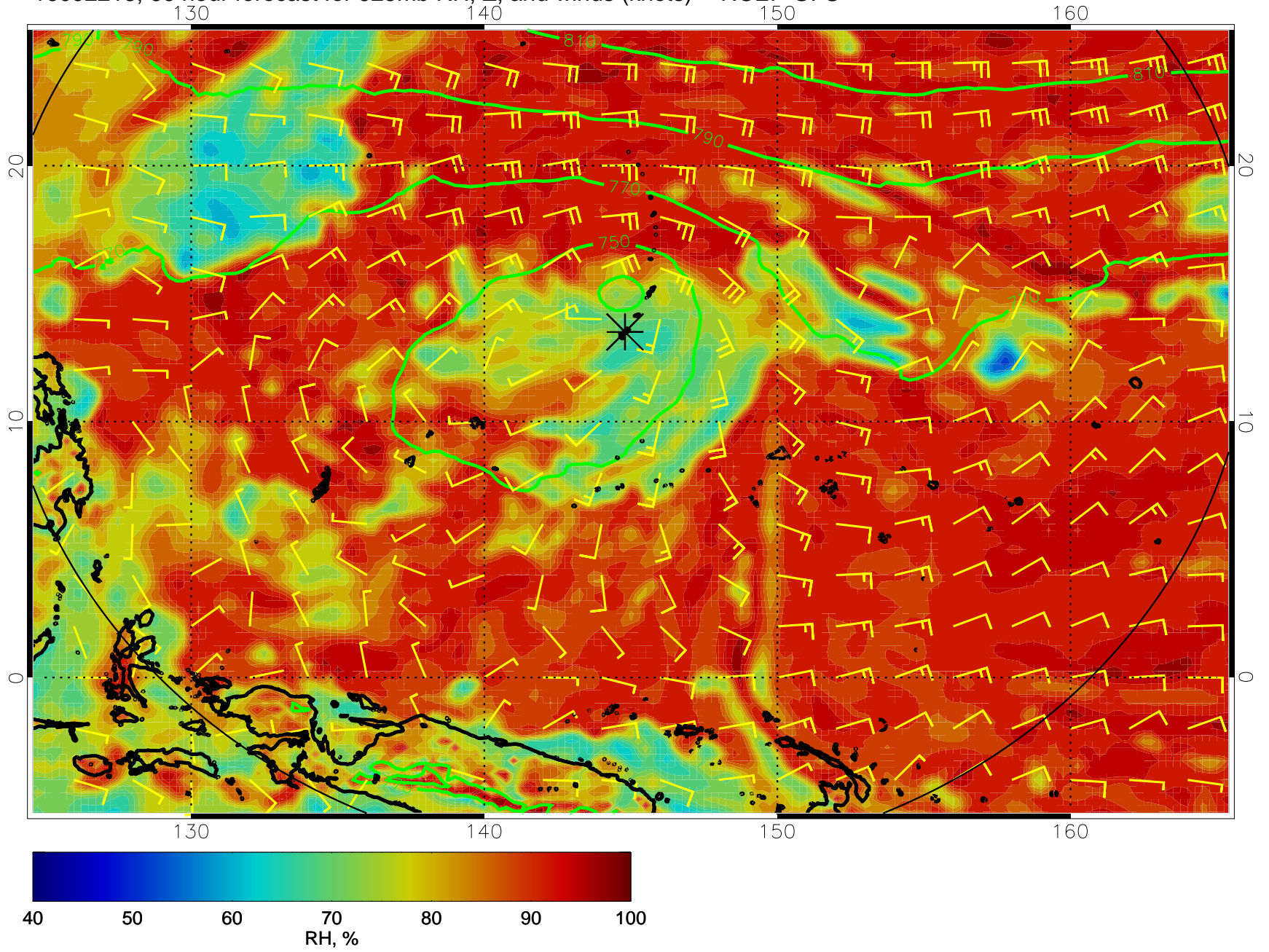
16092218, 66 hour forecast for 925mb RH, Z, and winds (knots) -- NCEP GFS
