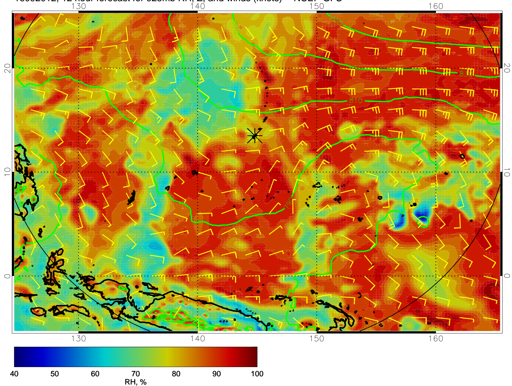
16092012, 12 hour forecast for 925mb RH, Z, and winds (knots) -- NCEP GFS
