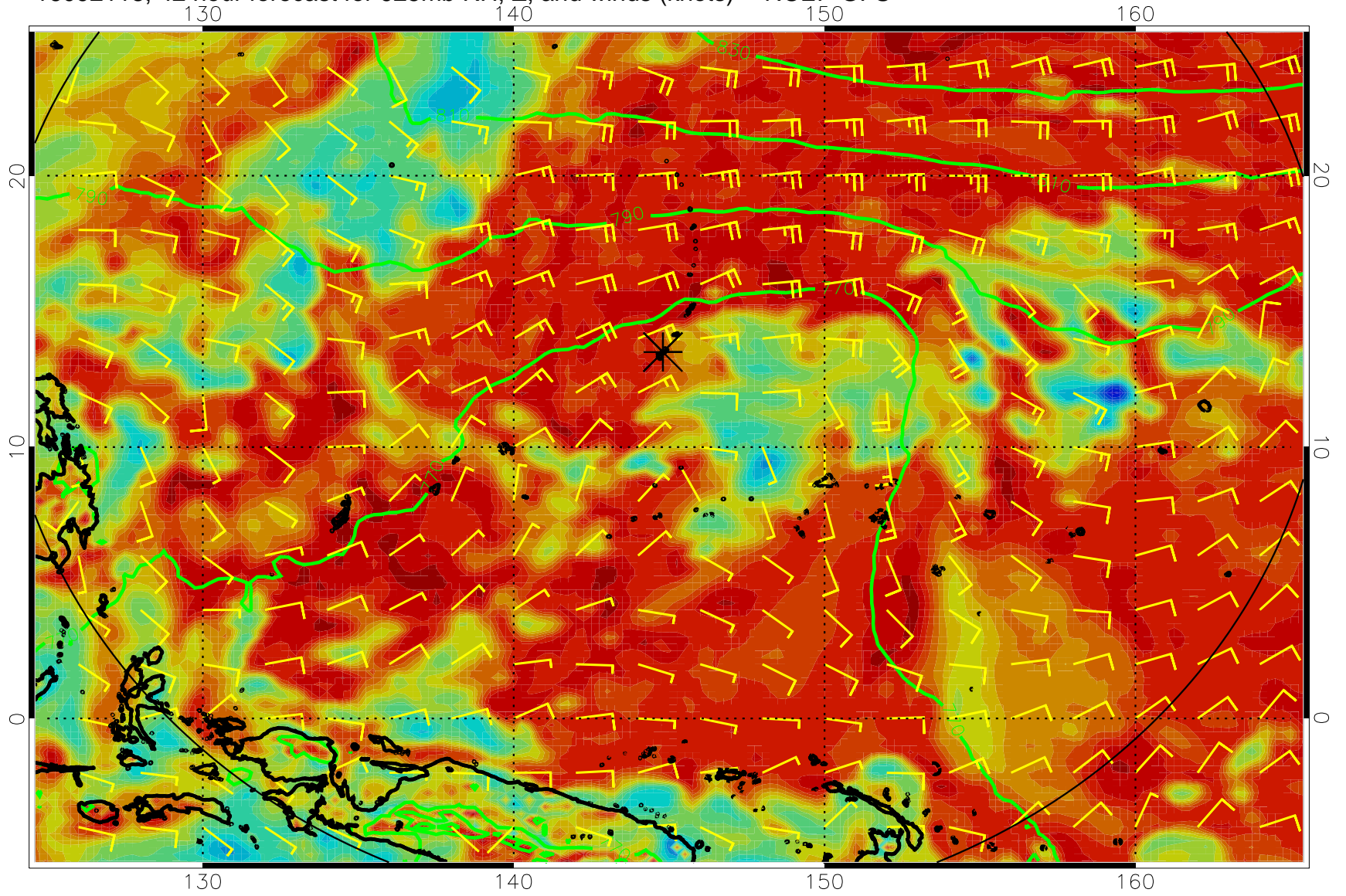
16092118, 42 hour forecast for 925mb RH, Z, and winds (knots) -- NCEP GFS
