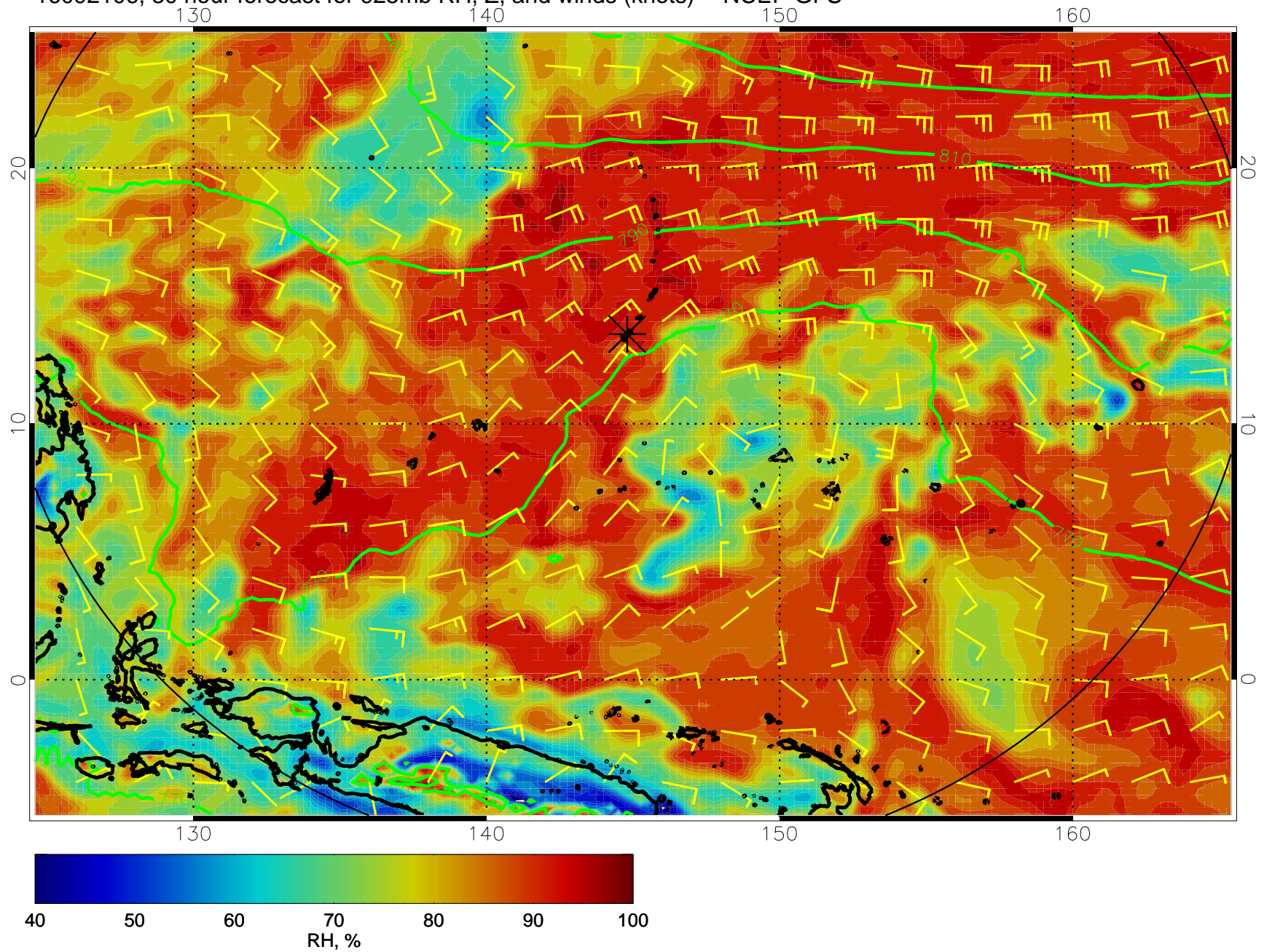
16092106, 30 hour forecast for 925mb RH, Z, and winds (knots) -- NCEP GFS
