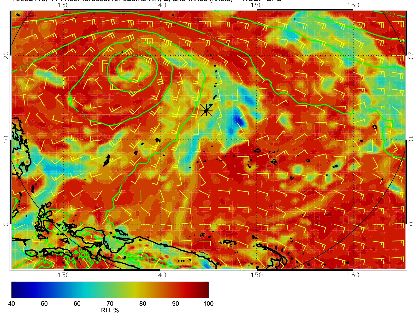
16092418, 114 hour forecast for 925mb RH, Z, and winds (knots) -- NCEP GFS
