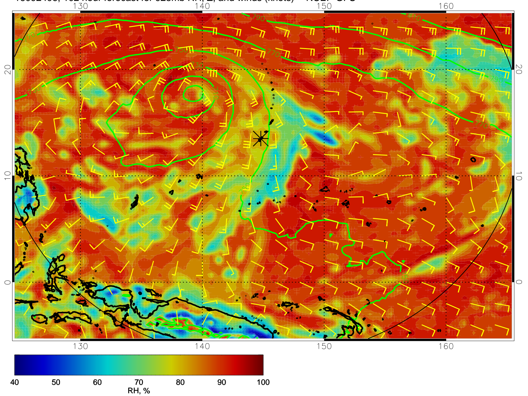
16092406, 102 hour forecast for 925mb RH, Z, and winds (knots) -- NCEP GFS
