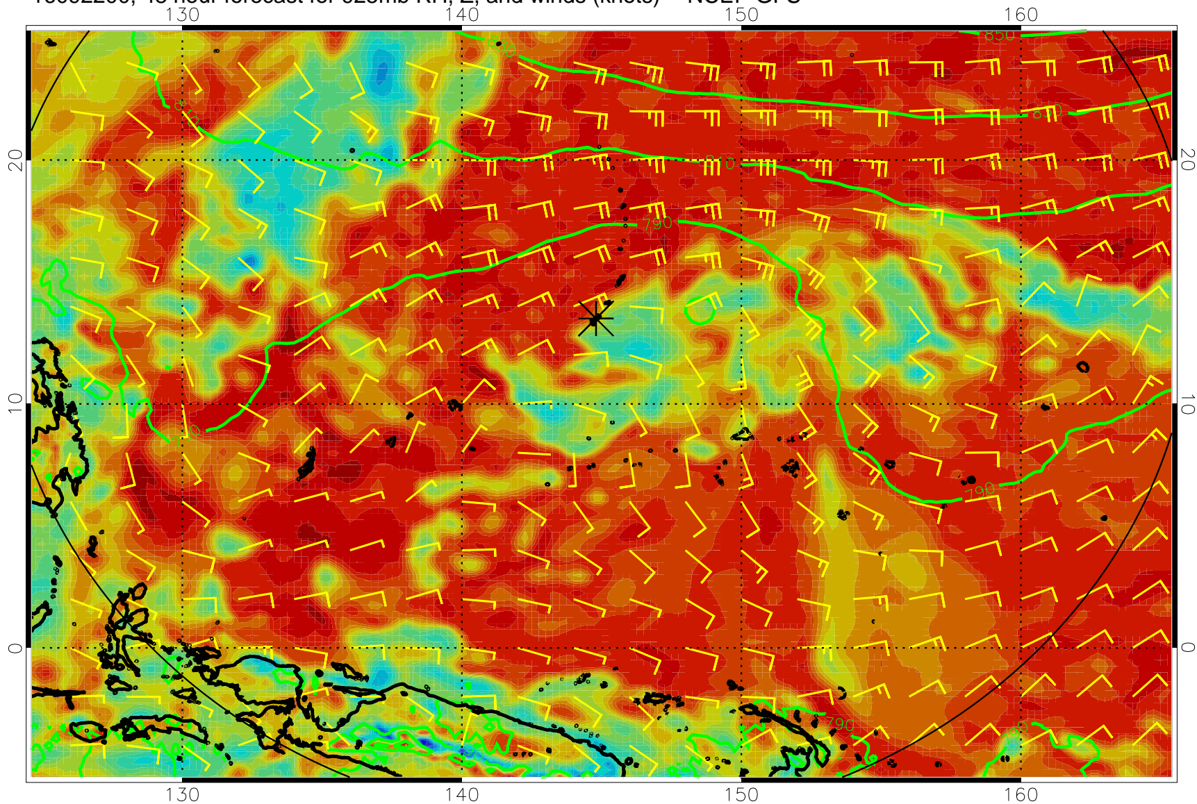
16092200, 48 hour forecast for 925mb RH, Z, and winds (knots) -- NCEP GFS
