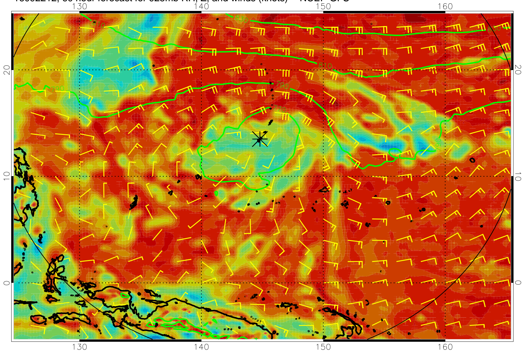
16092212, 60 hour forecast for 925mb RH, Z, and winds (knots) -- NCEP GFS
