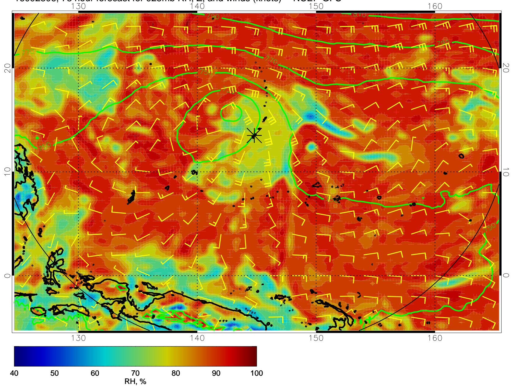
16092306, 78 hour forecast for 925mb RH, Z, and winds (knots) -- NCEP GFS
