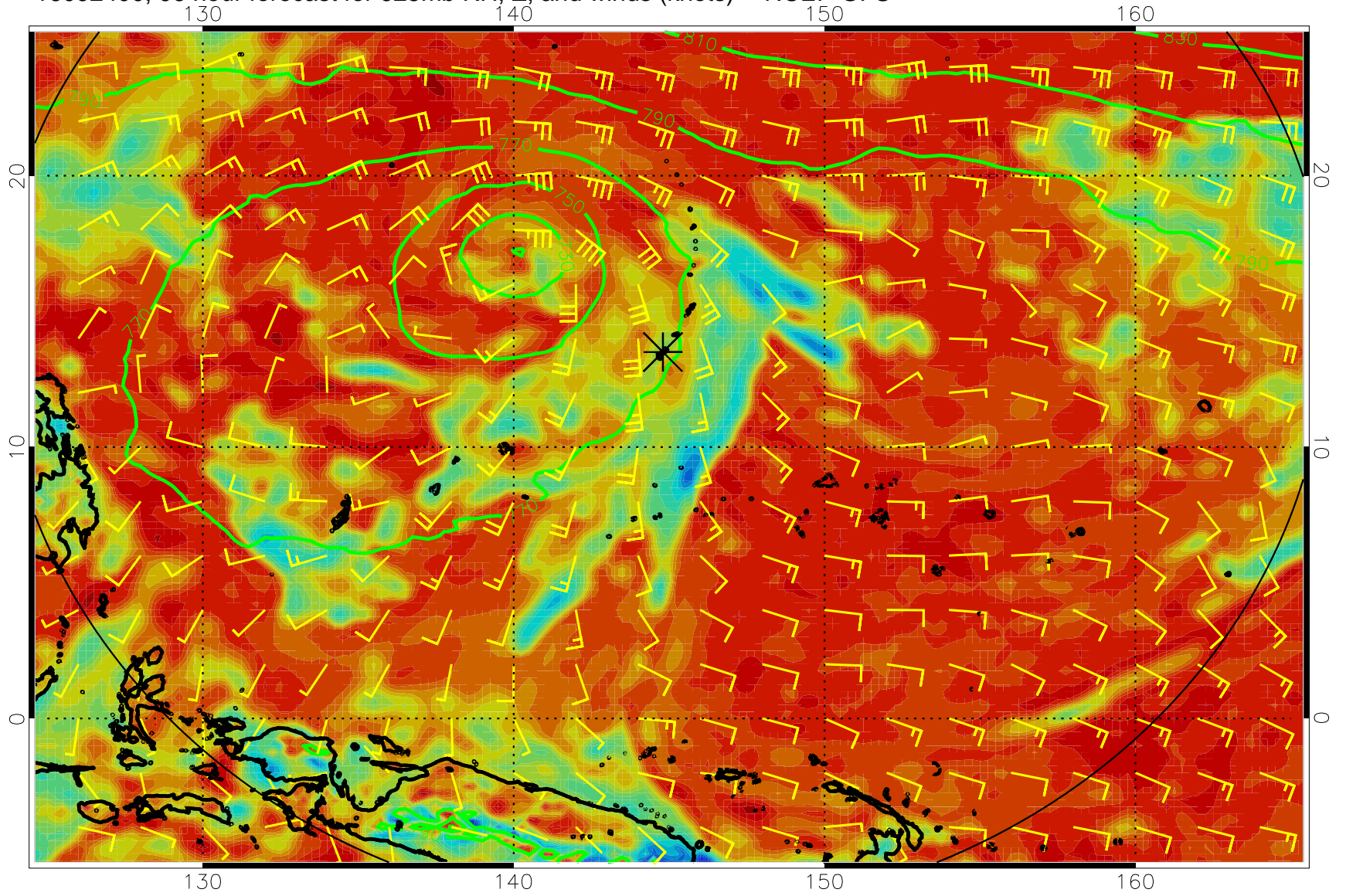
16092400, 96 hour forecast for 925mb RH, Z, and winds (knots) -- NCEP GFS
