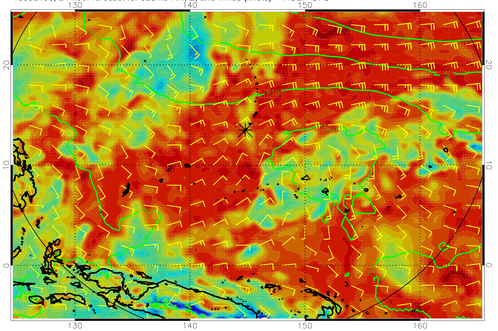
16092100, 24 hour forecast for 925mb RH, Z, and winds (knots) -- NCEP GFS
