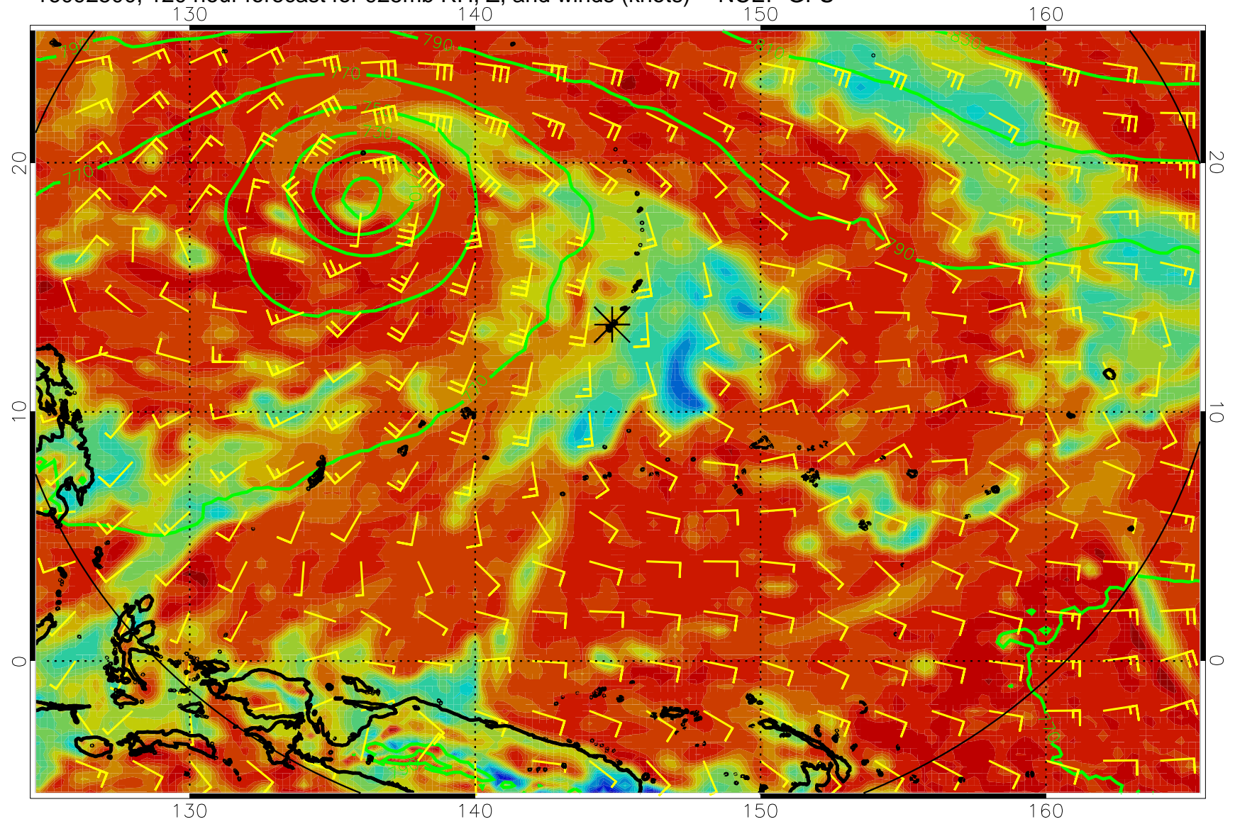
16092500, 120 hour forecast for 925mb RH, Z, and winds (knots) -- NCEP GFS
