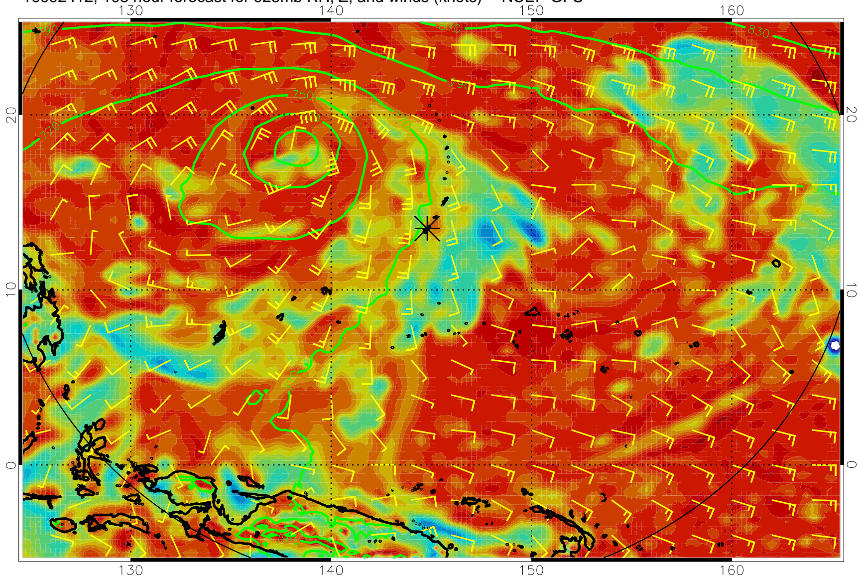
16092412, 108 hour forecast for 925mb RH, Z, and winds (knots) -- NCEP GFS
