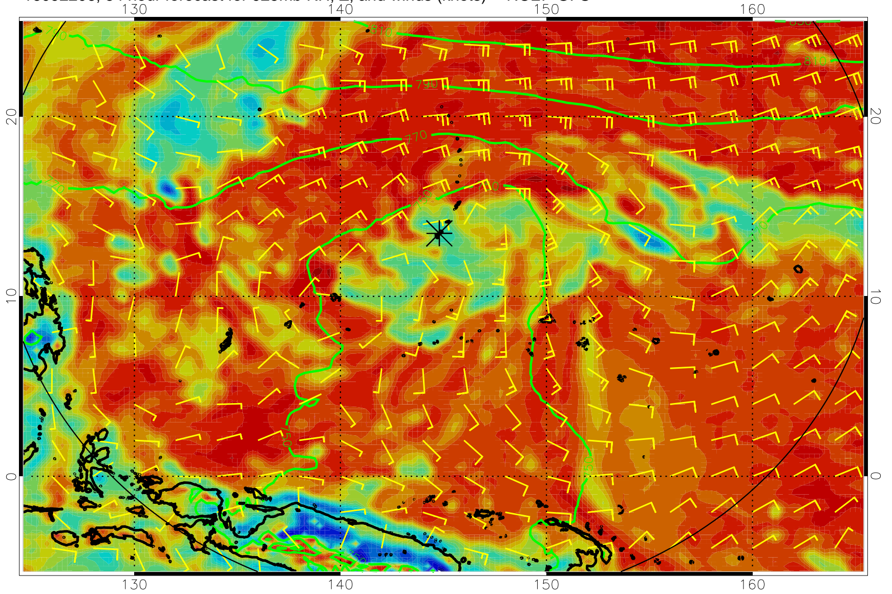
16092206, 54 hour forecast for 925mb RH, Z, and winds (knots) -- NCEP GFS
