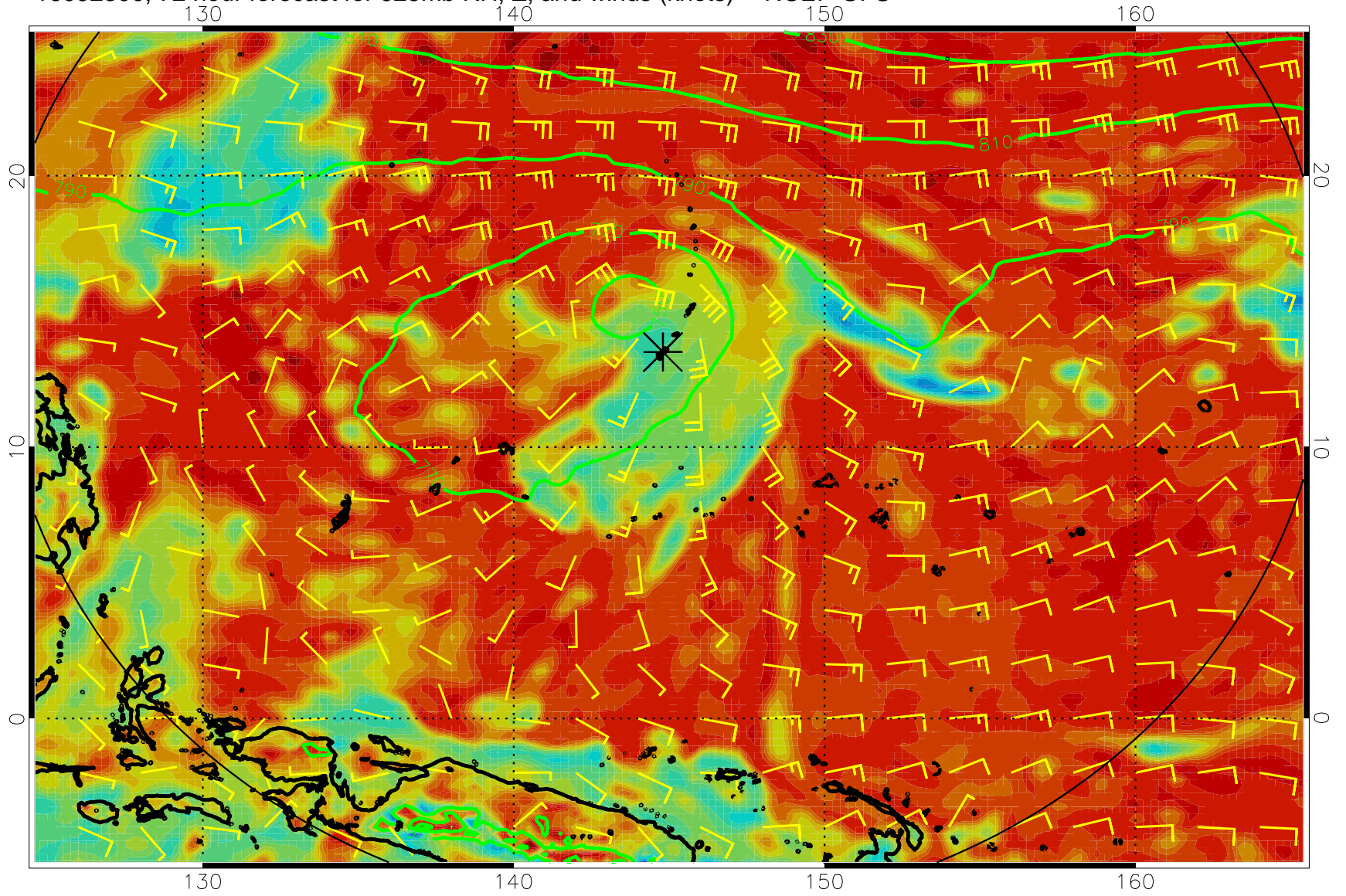
16092300, 72 hour forecast for 925mb RH, Z, and winds (knots) -- NCEP GFS
