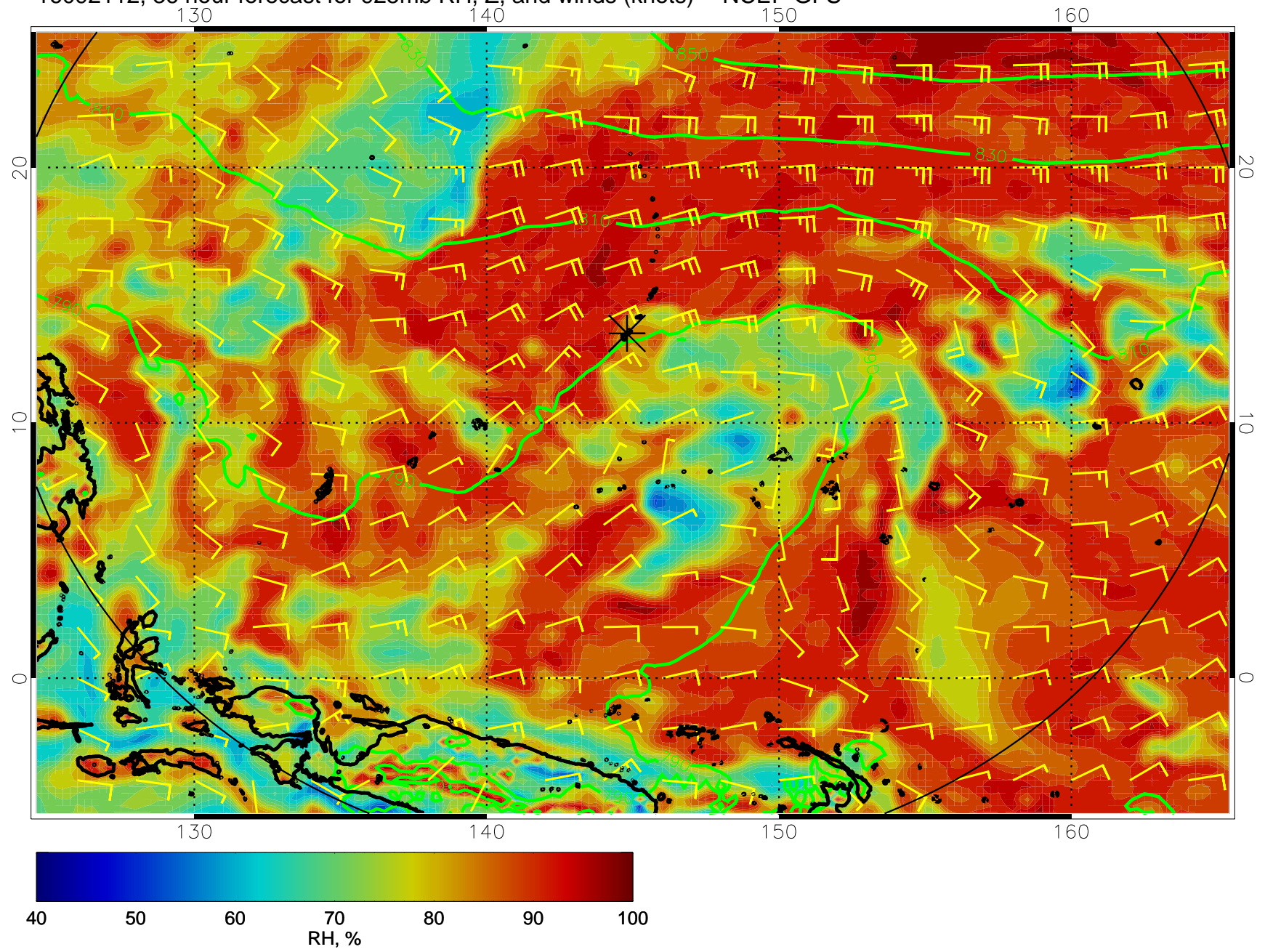
16092112, 36 hour forecast for 925mb RH, Z, and winds (knots) -- NCEP GFS
