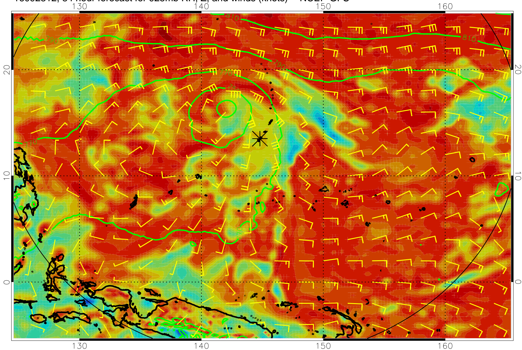
16092312, 84 hour forecast for 925mb RH, Z, and winds (knots) -- NCEP GFS
