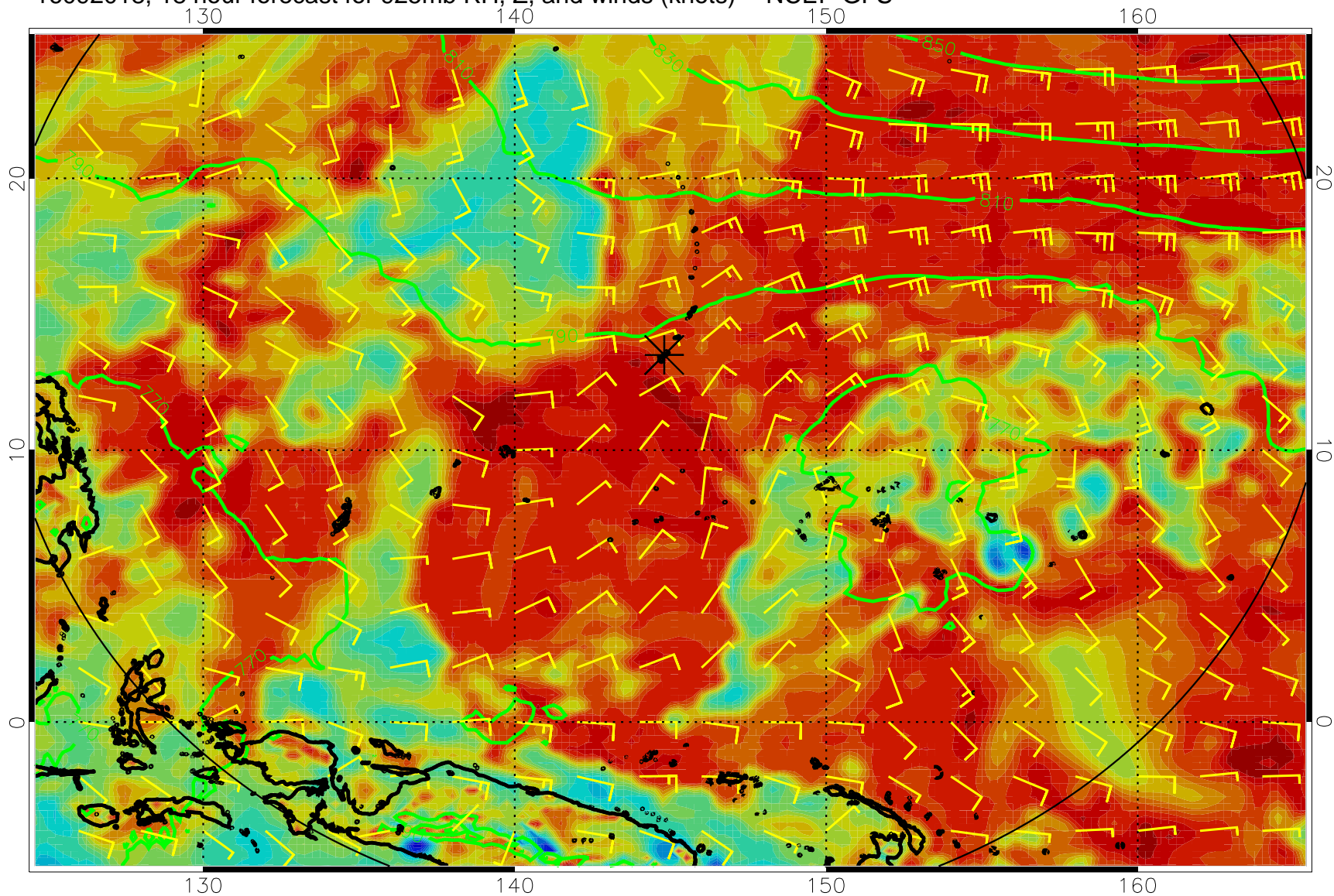
16092018, 18 hour forecast for 925mb RH, Z, and winds (knots) -- NCEP GFS
