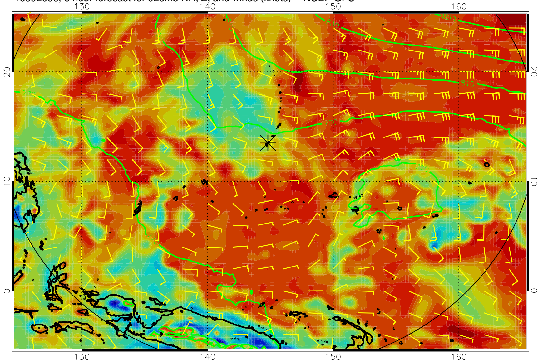
16092006, 6 hour forecast for 925mb RH, Z, and winds (knots) -- NCEP GFS
