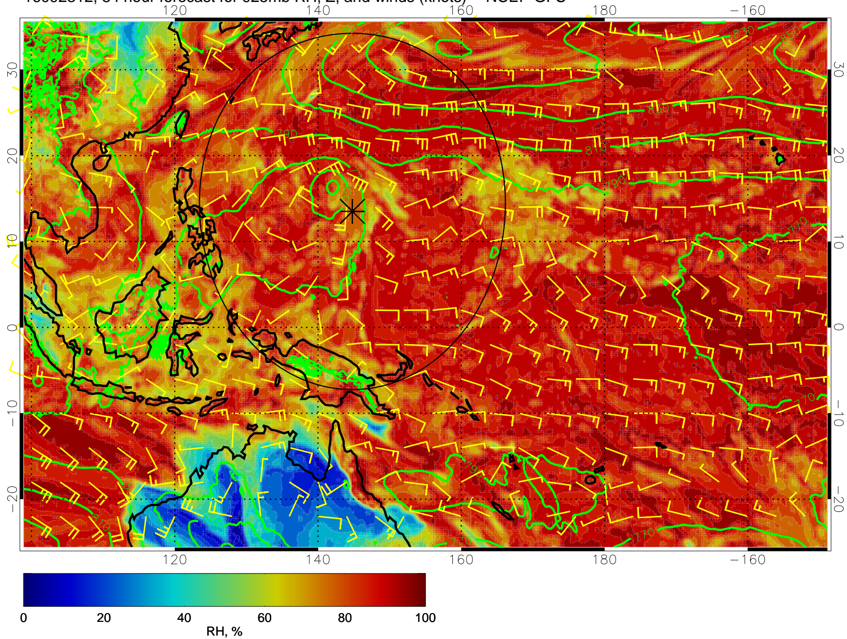
16092312, 84 hour forecast for 925mb RH, Z, and winds (knots) -- NCEP GFS
