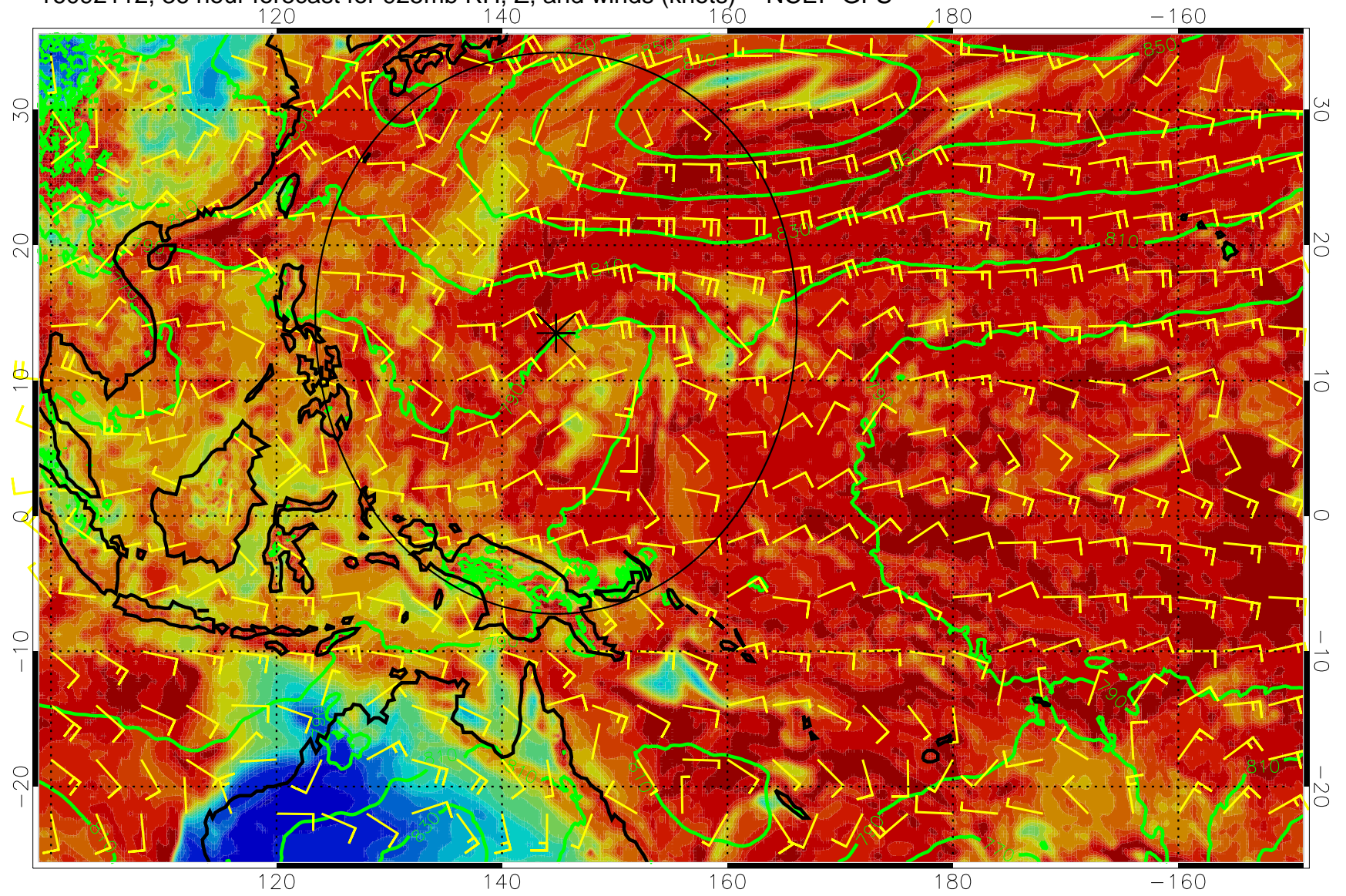
16092112, 36 hour forecast for 925mb RH, Z, and winds (knots) -- NCEP GFS
