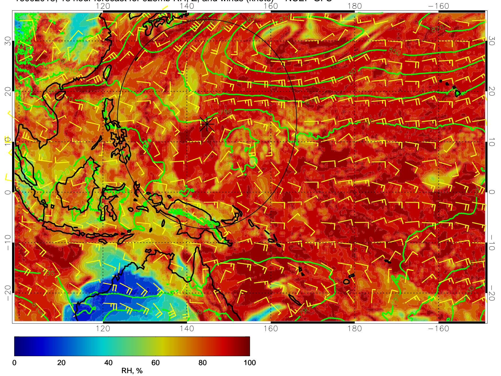
16092018, 18 hour forecast for 925mb RH, Z, and winds (knots) -- NCEP GFS
