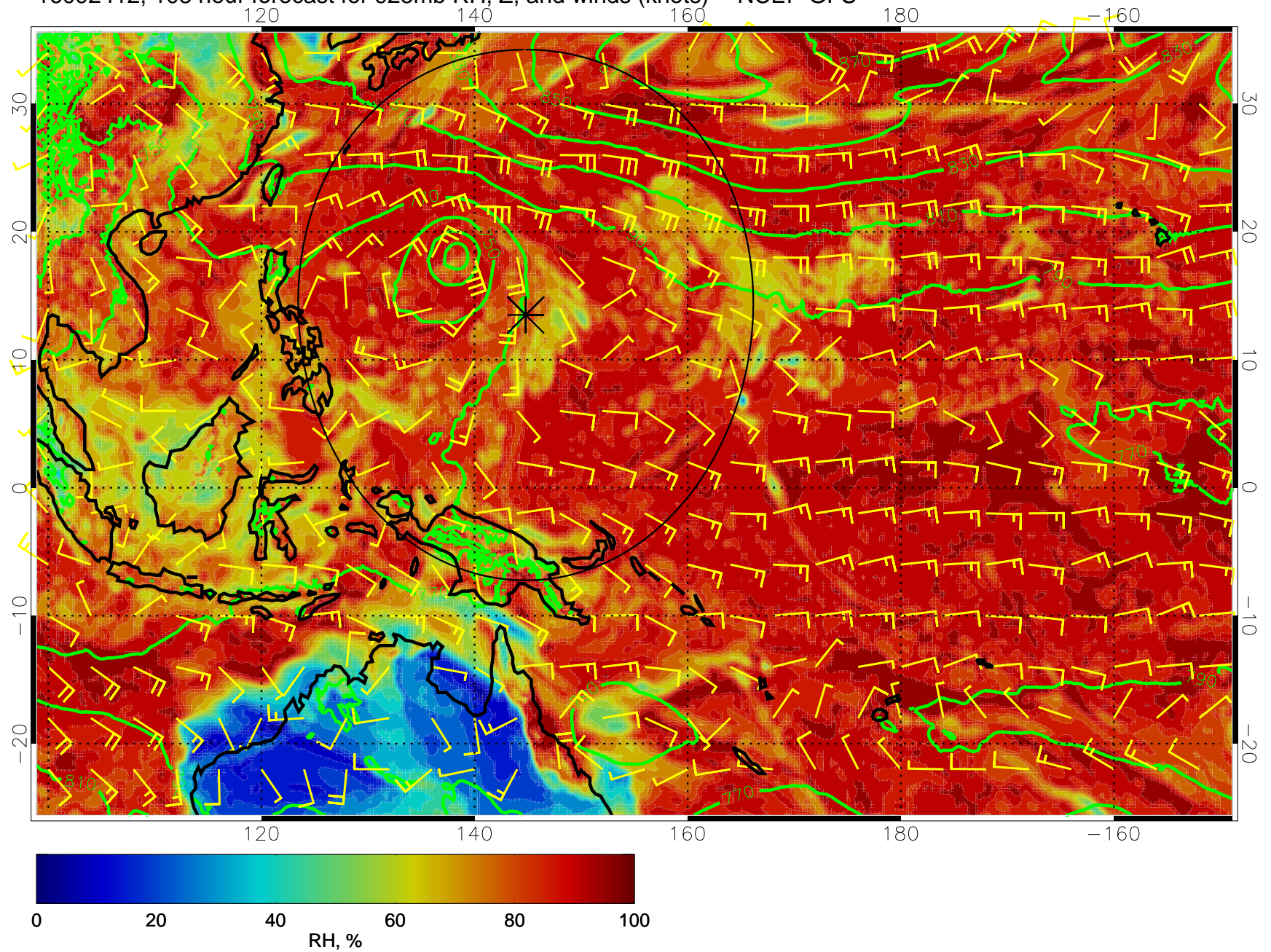
16092412, 108 hour forecast for 925mb RH, Z, and winds (knots) -- NCEP GFS
