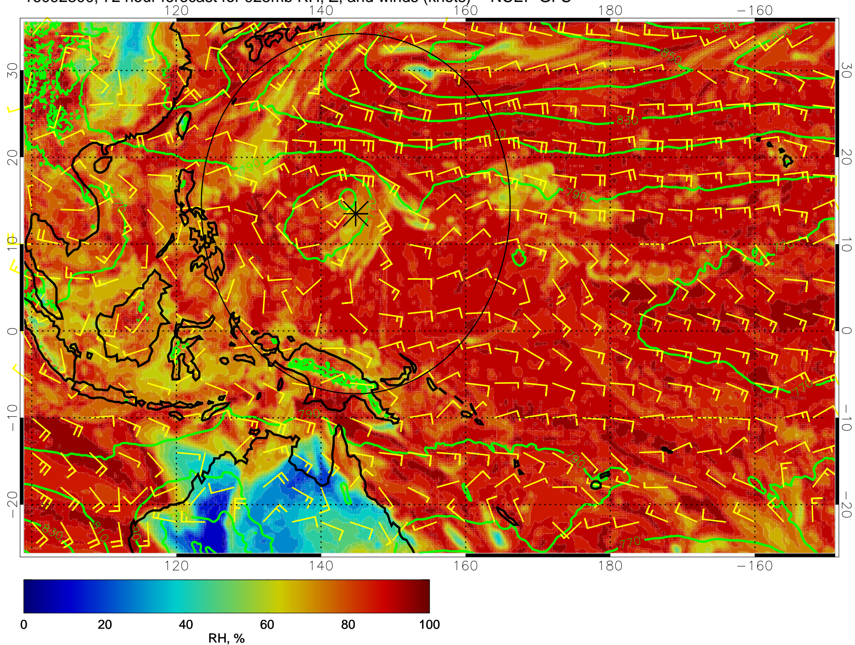
16092300, 72 hour forecast for 925mb RH, Z, and winds (knots) -- NCEP GFS
