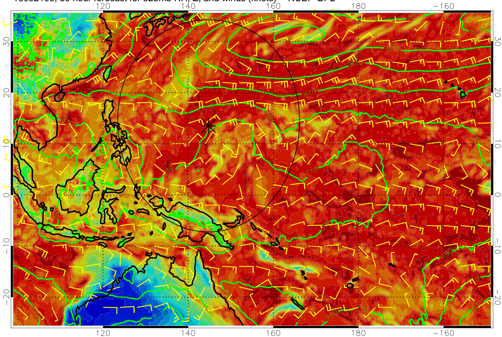
16092106, 30 hour forecast for 925mb RH, Z, and winds (knots) -- NCEP GFS
