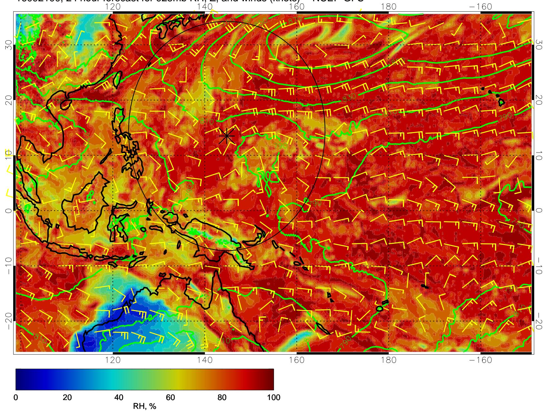
16092100, 24 hour forecast for 925mb RH, Z, and winds (knots) -- NCEP GFS
