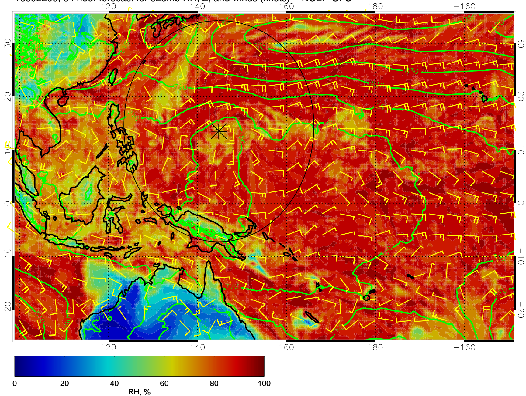
16092206, 54 hour forecast for 925mb RH, Z, and winds (knots) -- NCEP GFS
