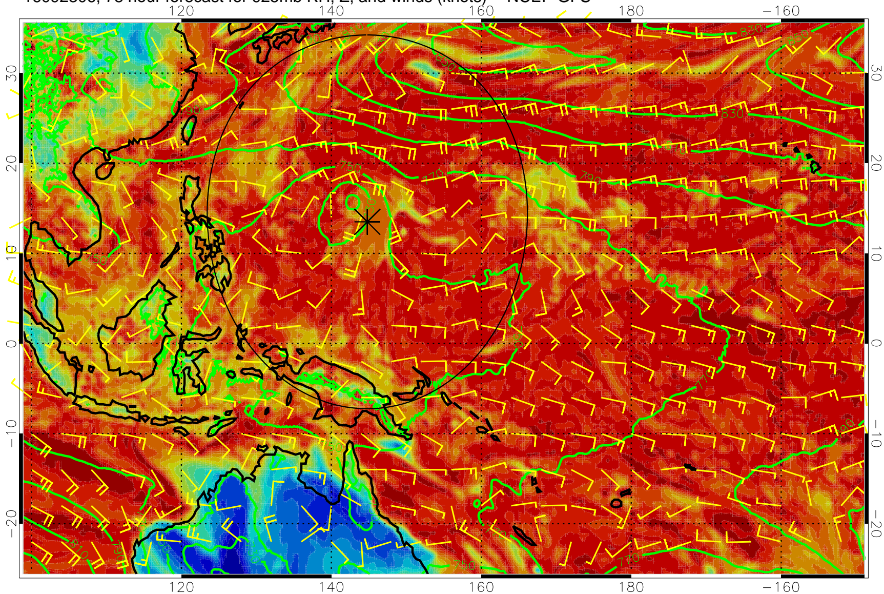
16092306, 78 hour forecast for 925mb RH, Z, and winds (knots) -- NCEP GFS
