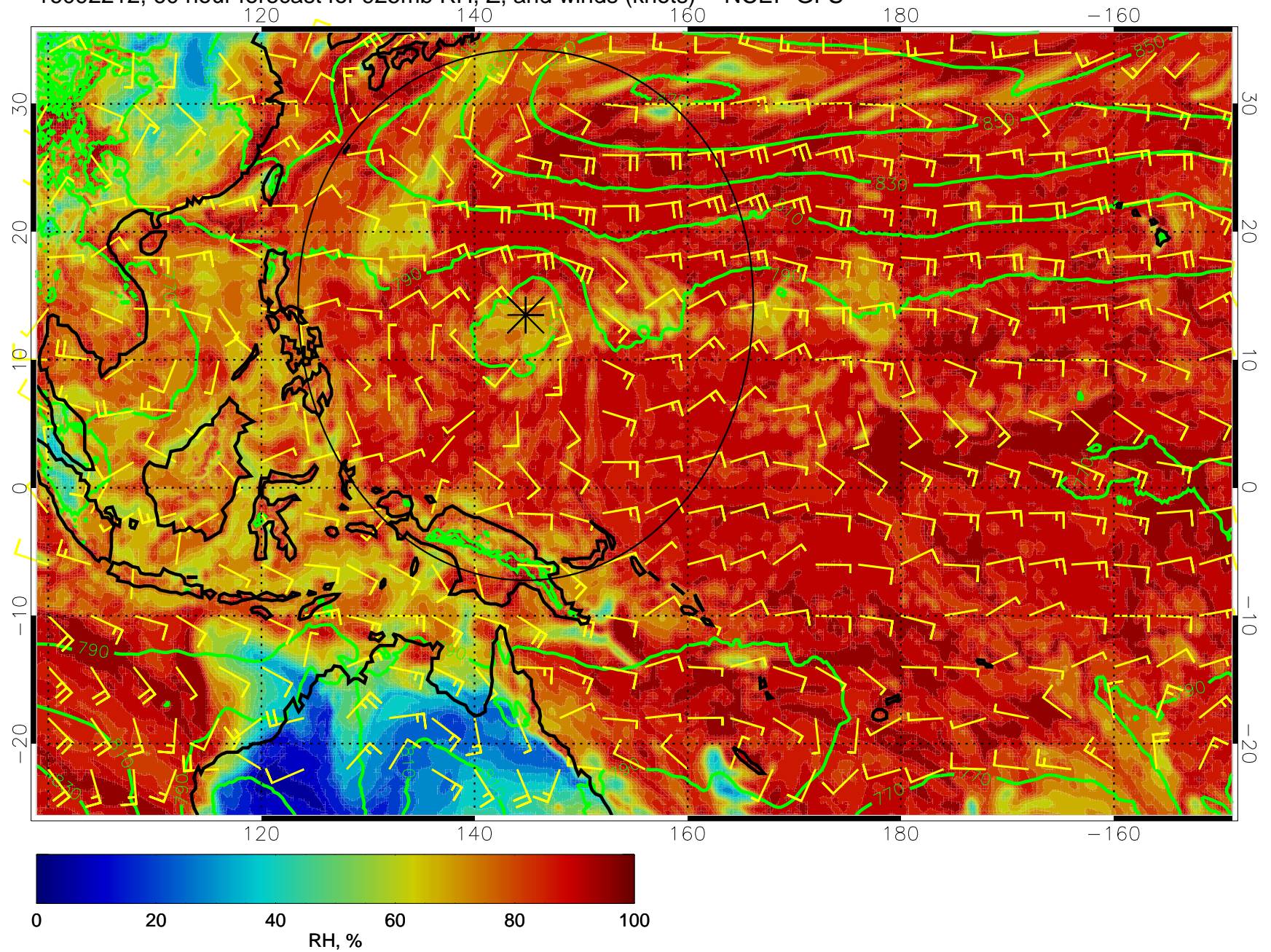
16092212, 60 hour forecast for 925mb RH, Z, and winds (knots) -- NCEP GFS
