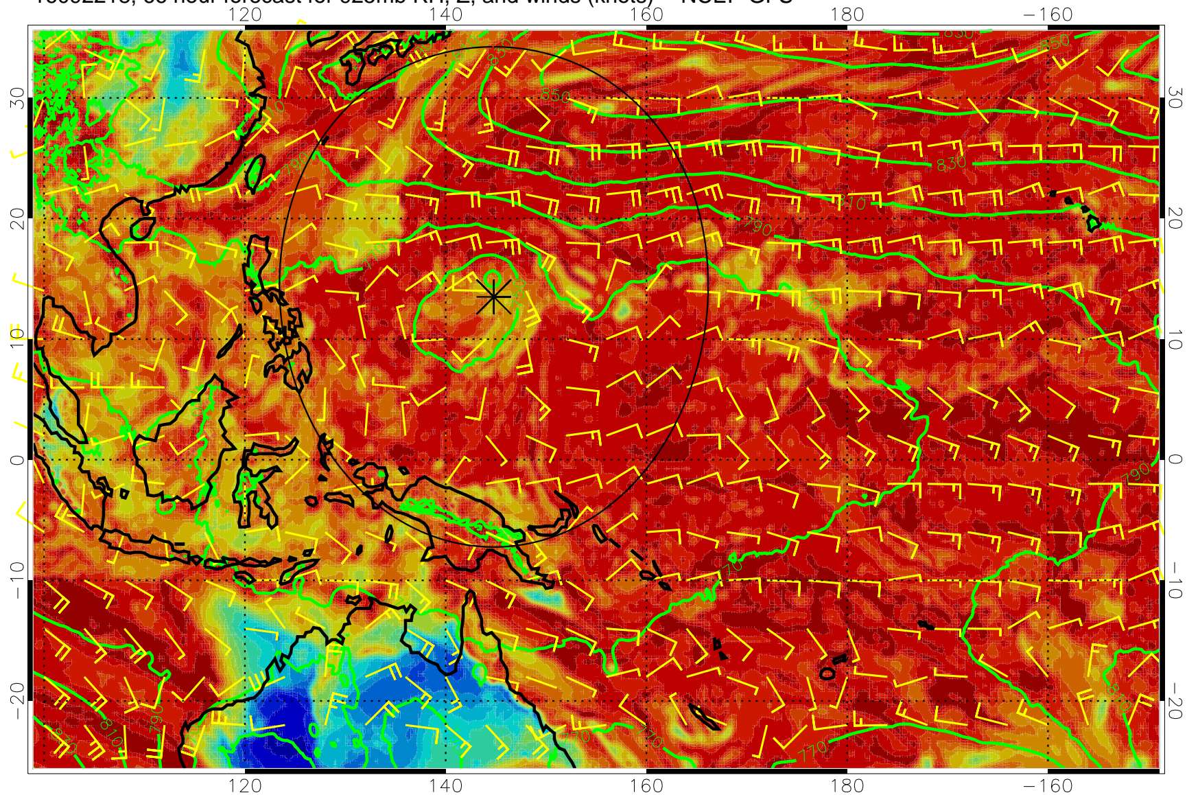
16092218, 66 hour forecast for 925mb RH, Z, and winds (knots) -- NCEP GFS
