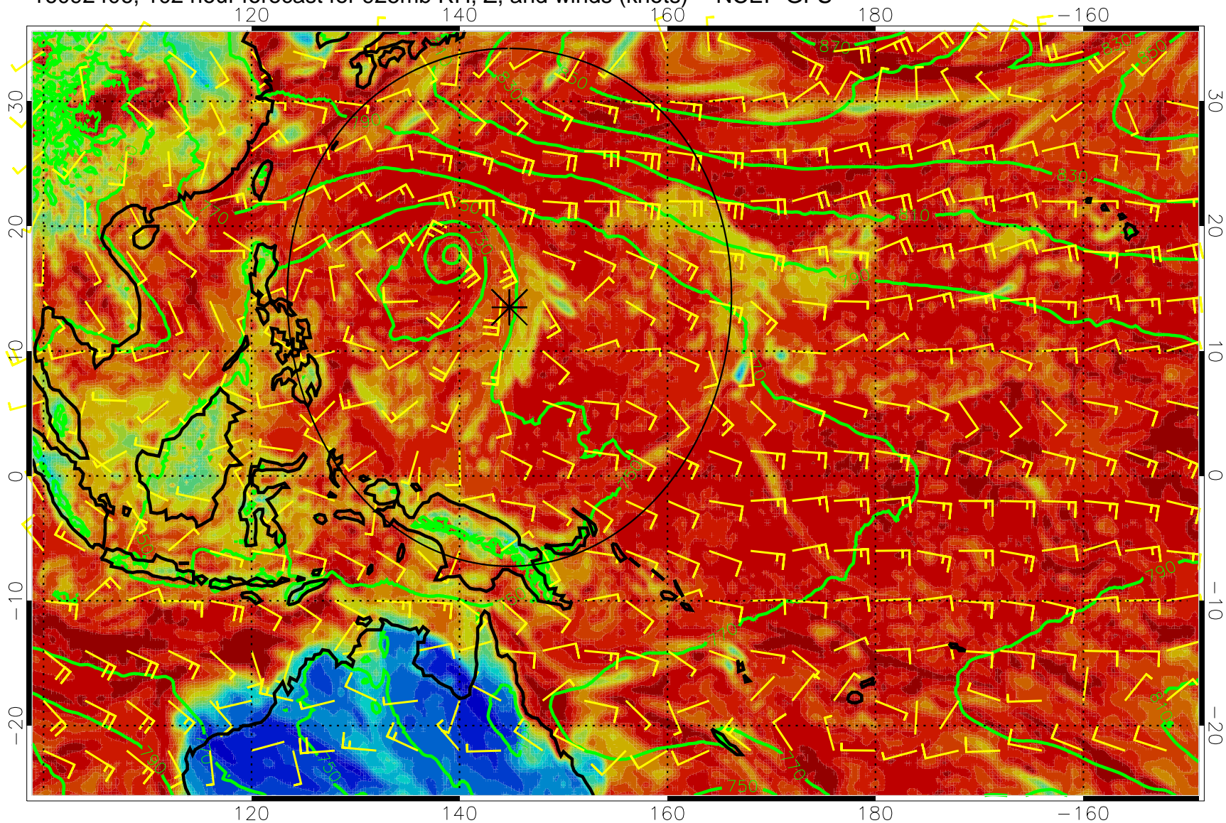
16092406, 102 hour forecast for 925mb RH, Z, and winds (knots) -- NCEP GFS
