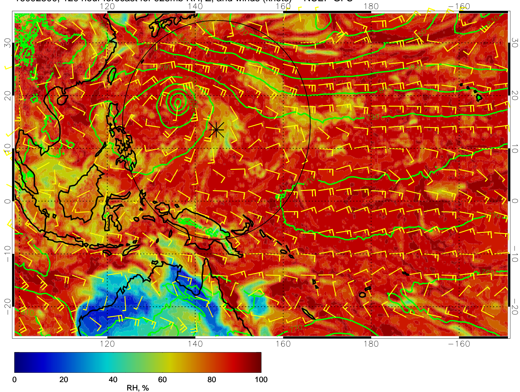
16092500, 120 hour forecast for 925mb RH, Z, and winds (knots) -- NCEP GFS
