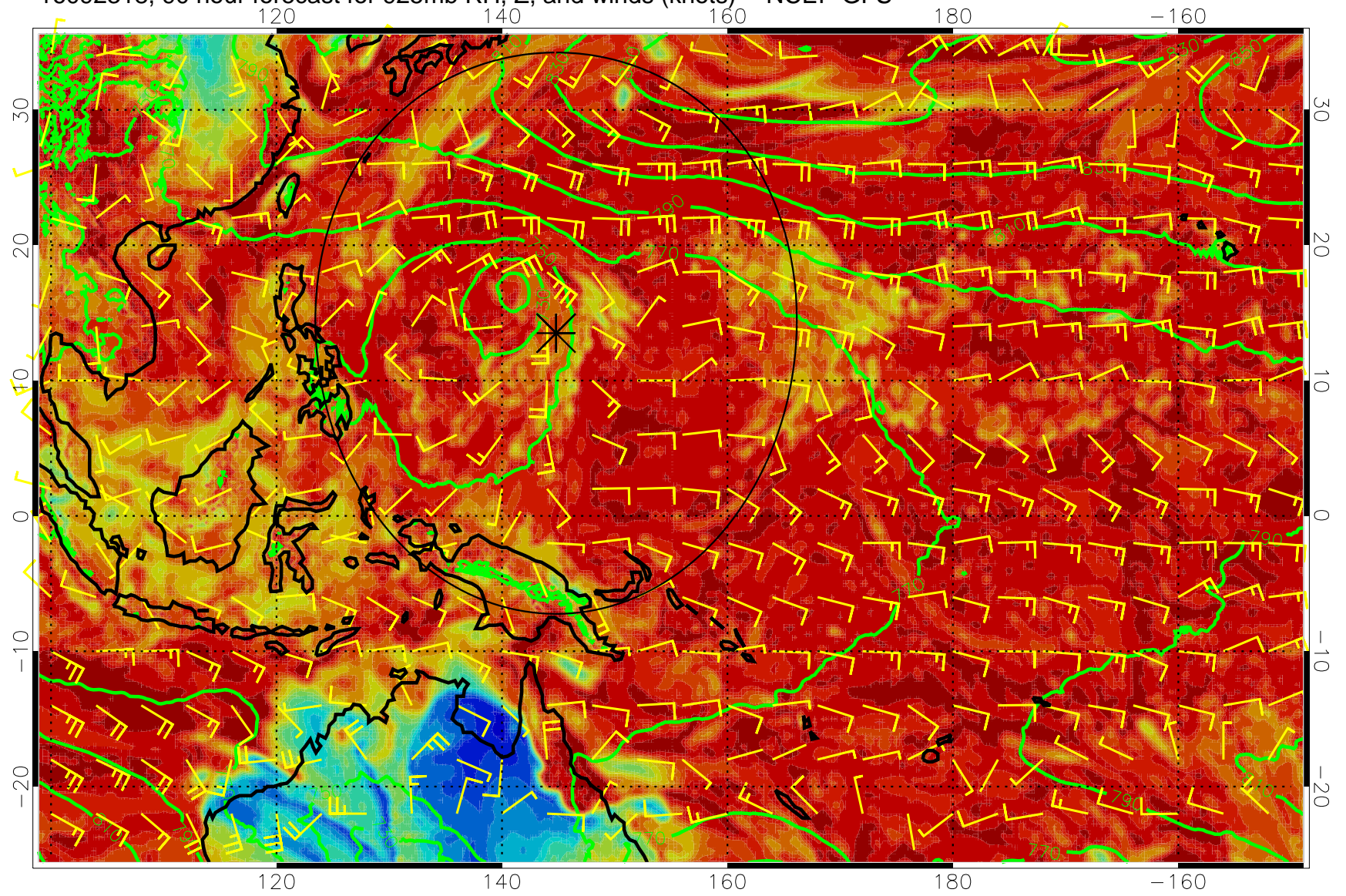
16092318, 90 hour forecast for 925mb RH, Z, and winds (knots) -- NCEP GFS
