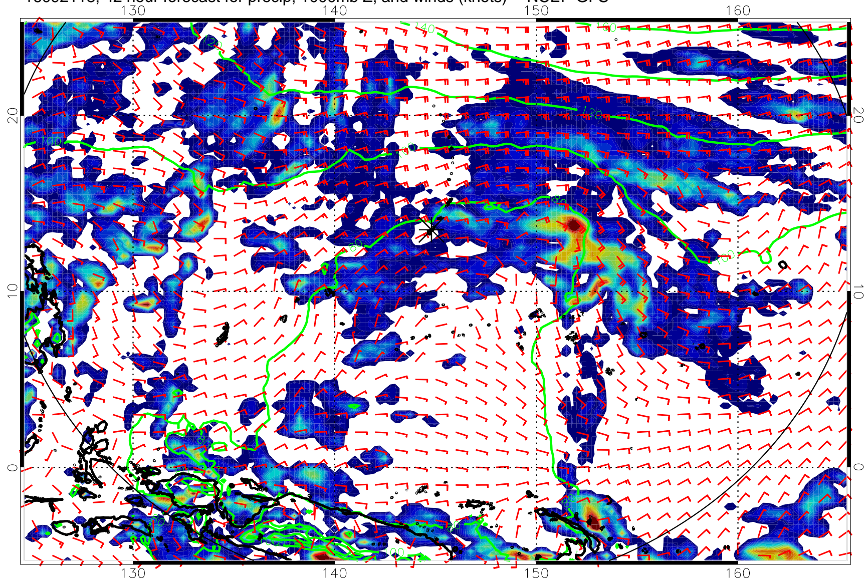
16092118, 42 hour forecast for precip, 1000mb Z, and winds (knots) -- NCEP GFS
