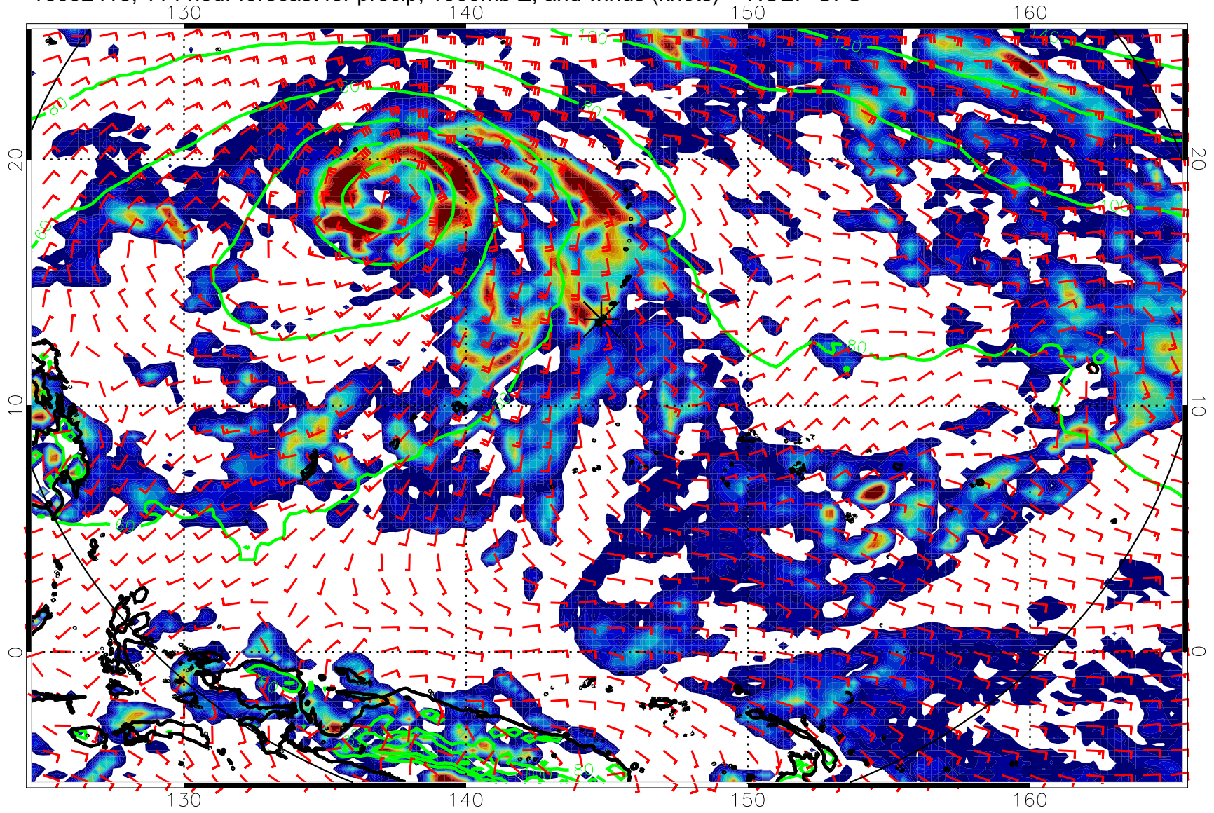
16092418, 114 hour forecast for precip, 1000mb Z, and winds (knots) -- NCEP GFS
