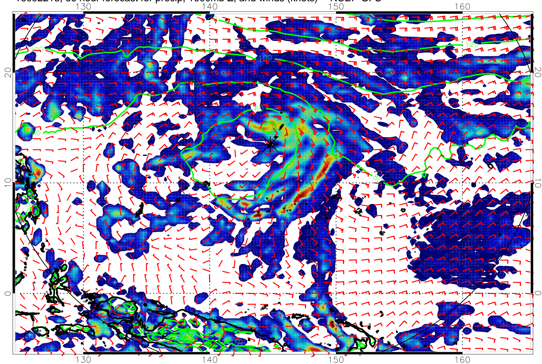
16092218, 66 hour forecast for precip, 1000mb Z, and winds (knots) -- NCEP GFS
