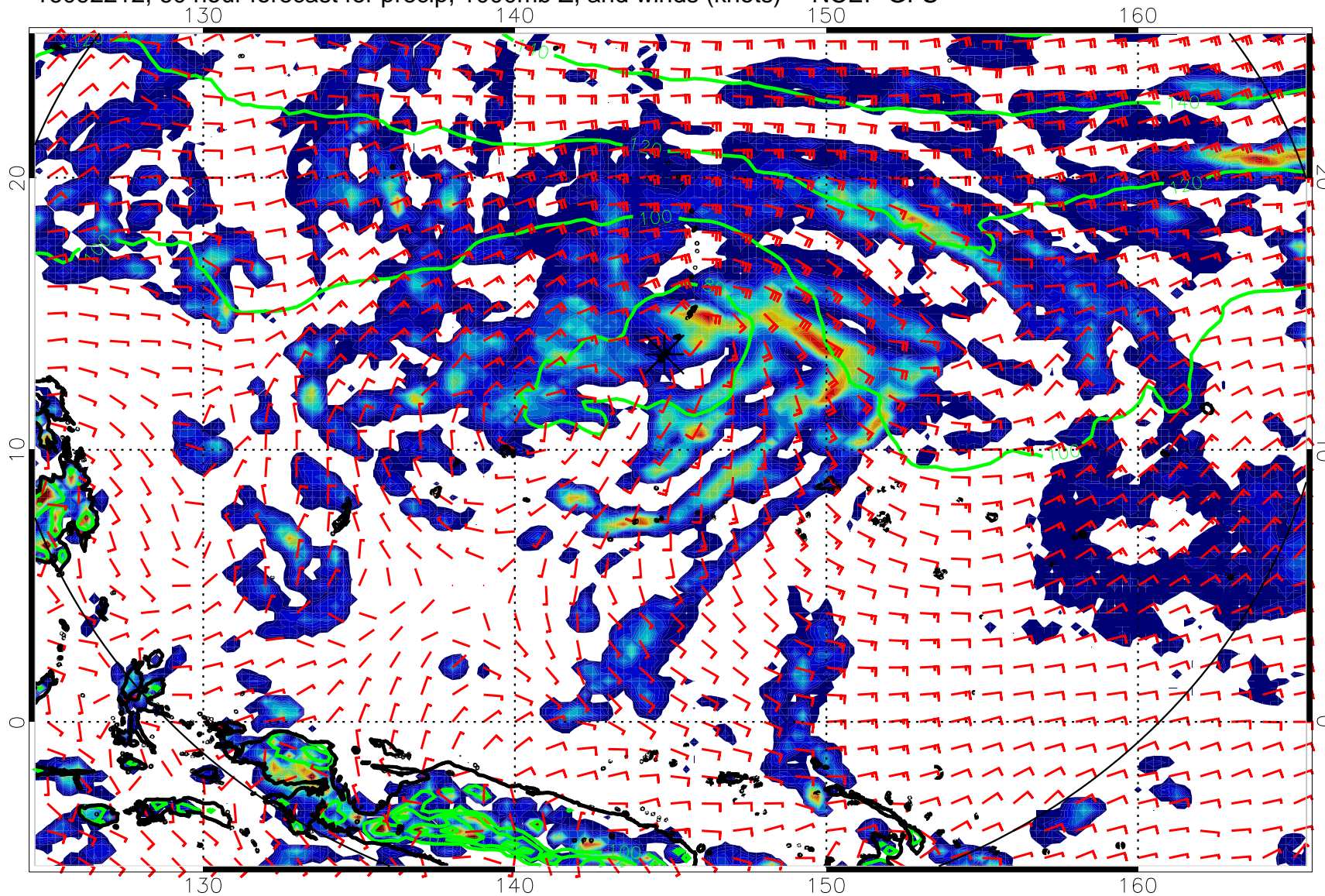
16092212, 60 hour forecast for precip, 1000mb Z, and winds (knots) -- NCEP GFS
