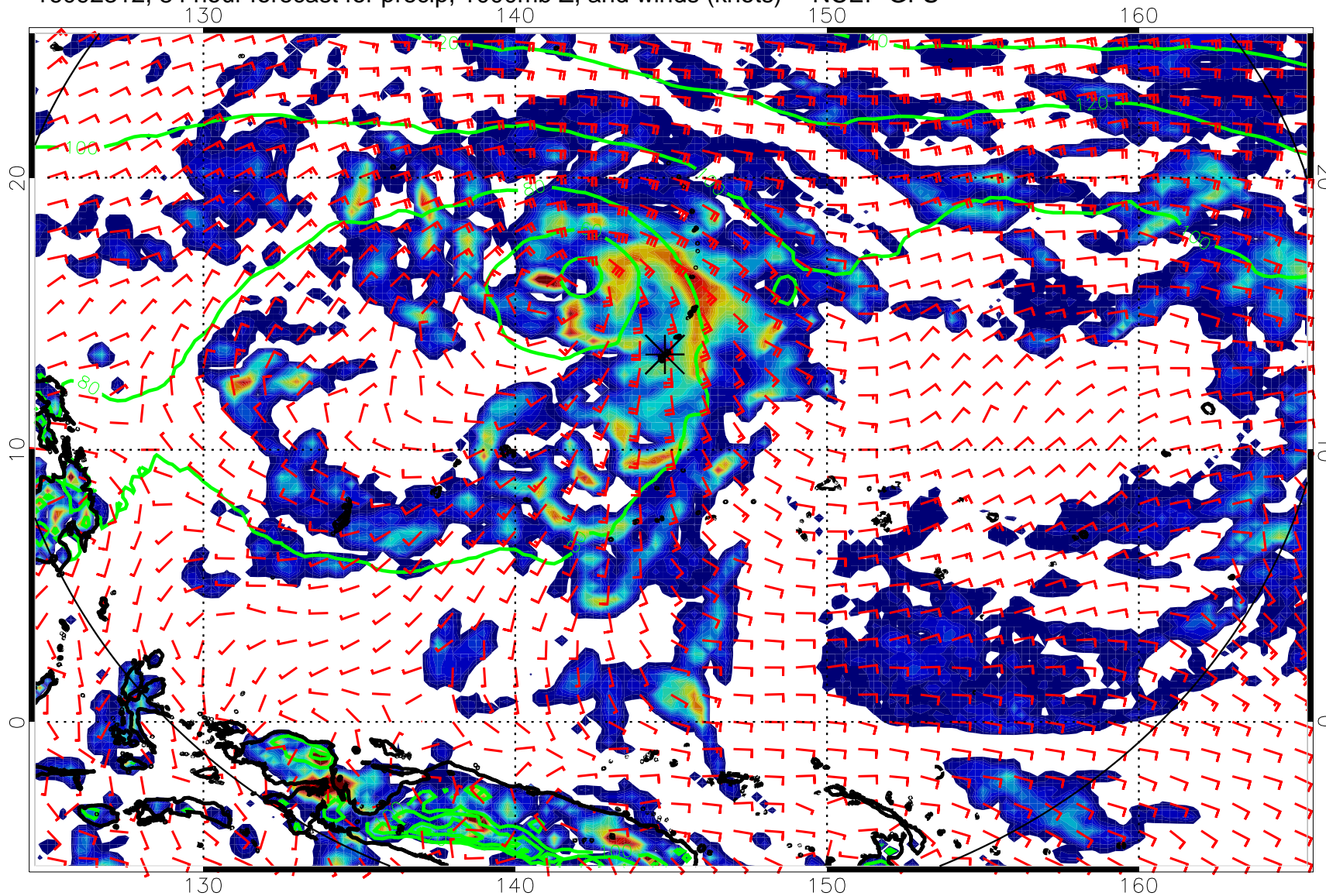
16092312, 84 hour forecast for precip, 1000mb Z, and winds (knots) -- NCEP GFS
