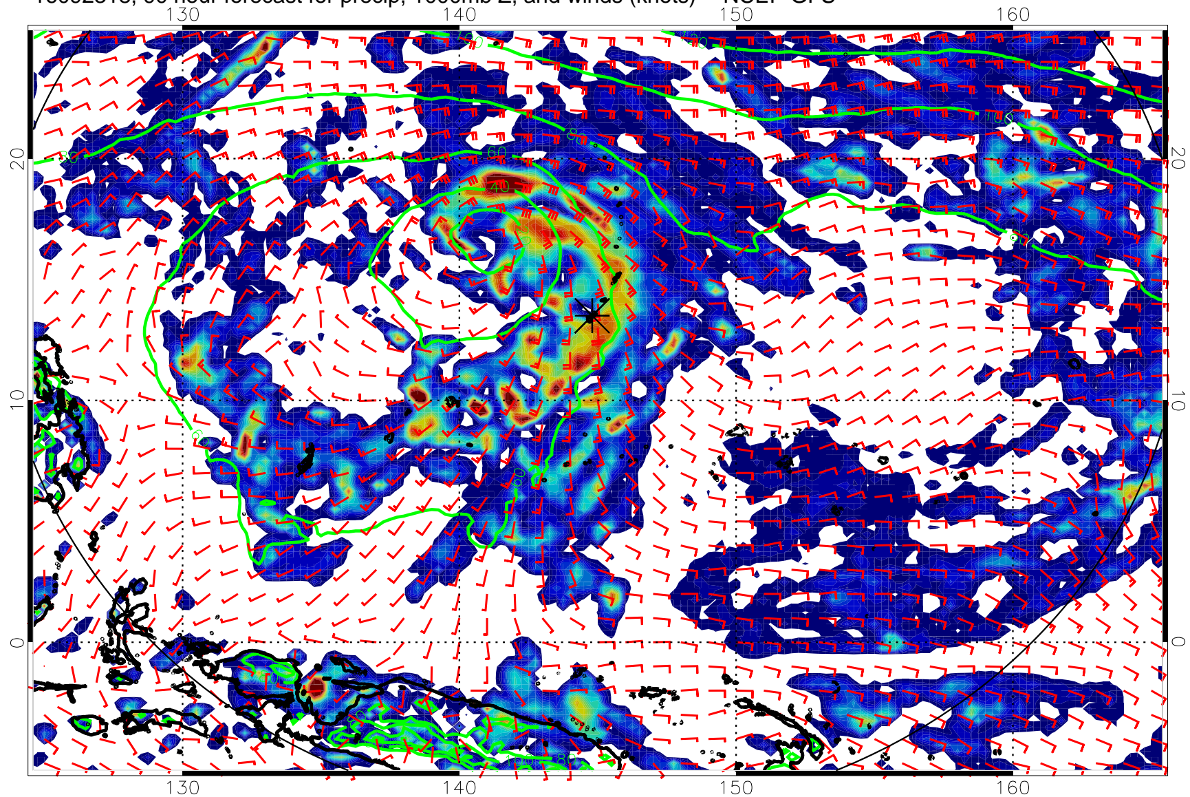
16092318, 90 hour forecast for precip, 1000mb Z, and winds (knots) -- NCEP GFS
