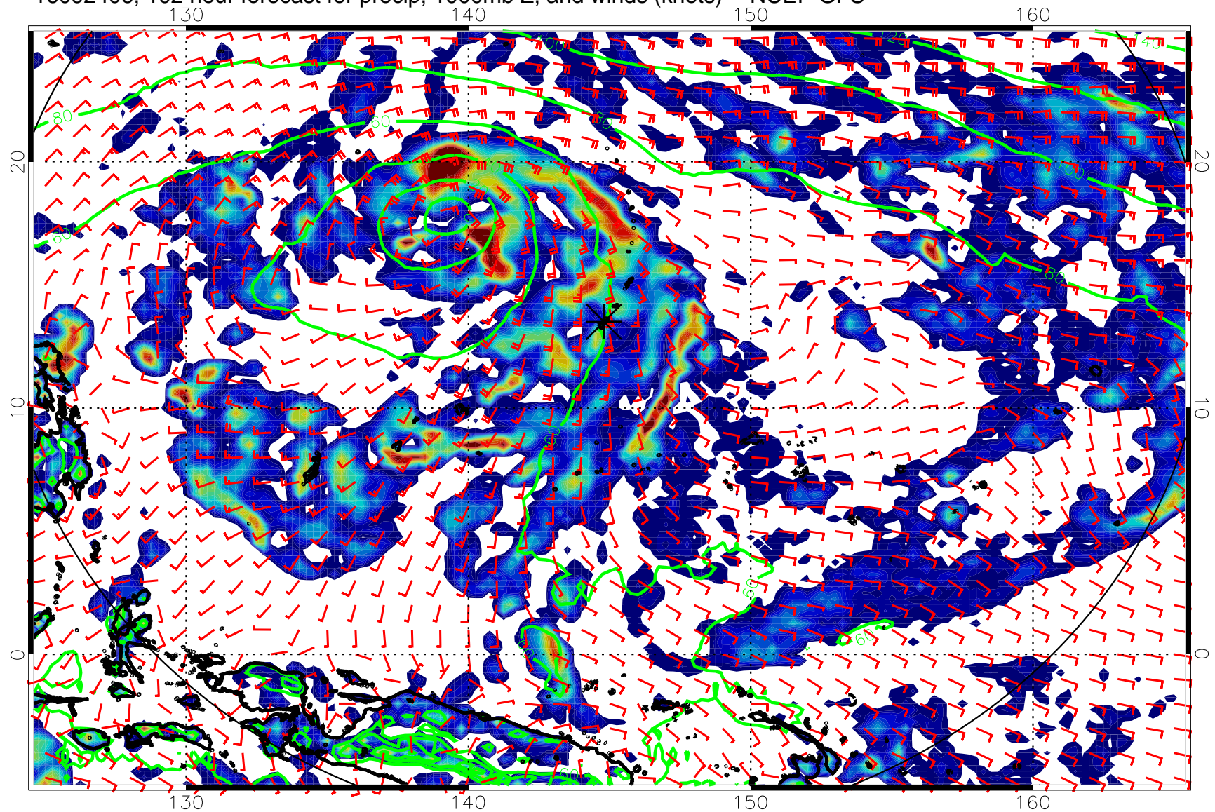
16092406, 102 hour forecast for precip, 1000mb Z, and winds (knots) -- NCEP GFS
