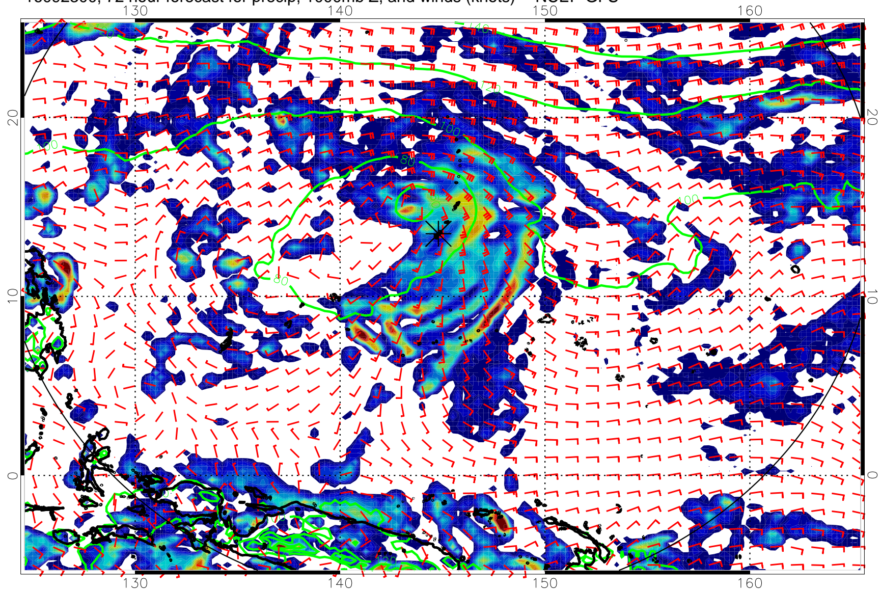
16092300, 72 hour forecast for precip, 1000mb Z, and winds (knots) -- NCEP GFS
