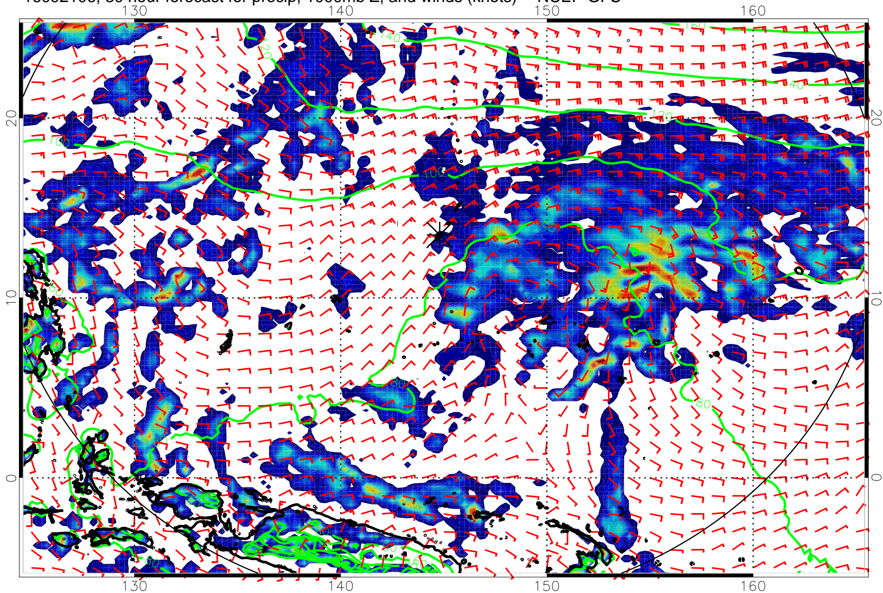
16092106, 30 hour forecast for precip, 1000mb Z, and winds (knots) -- NCEP GFS
