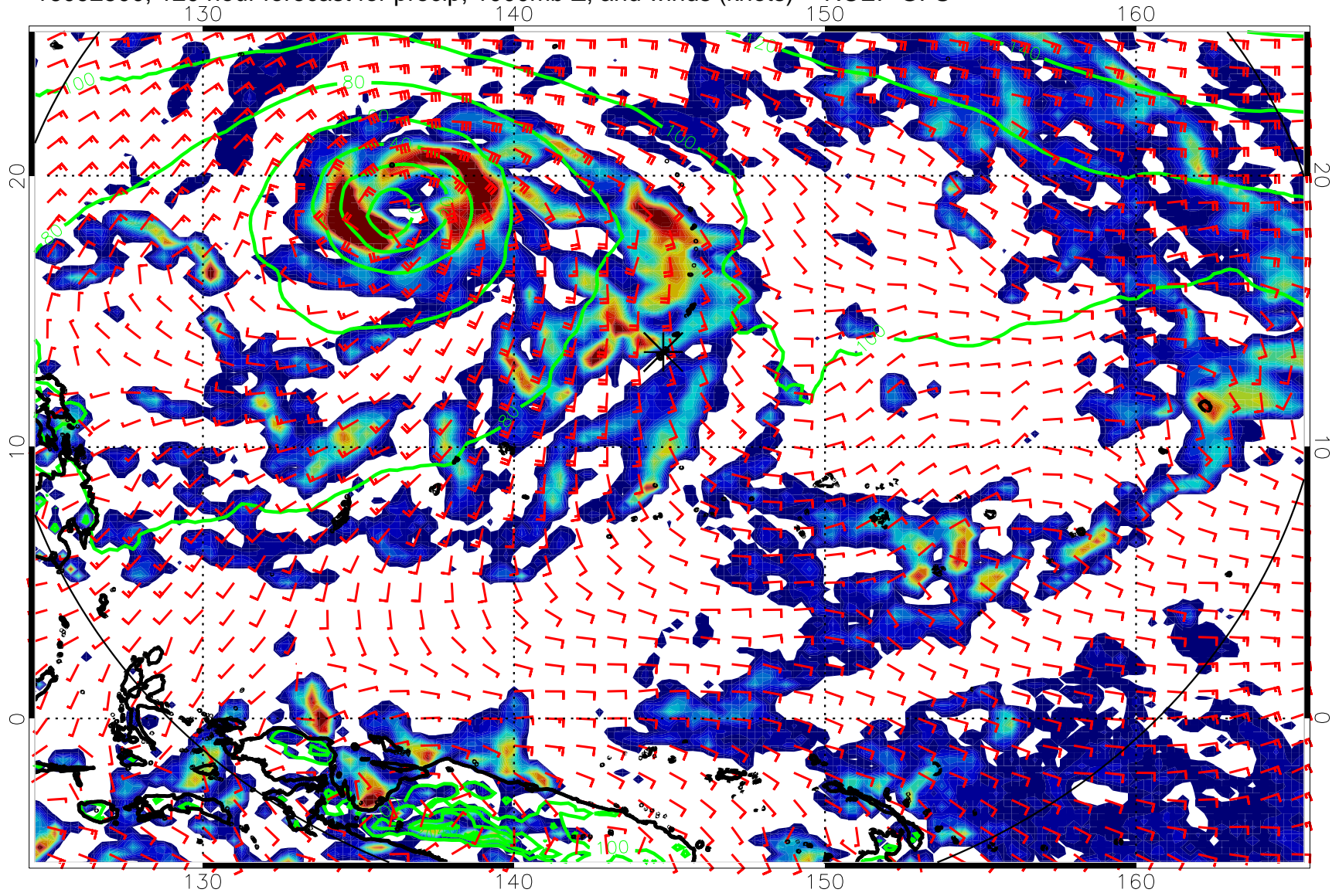
16092500, 120 hour forecast for precip, 1000mb Z, and winds (knots) -- NCEP GFS
