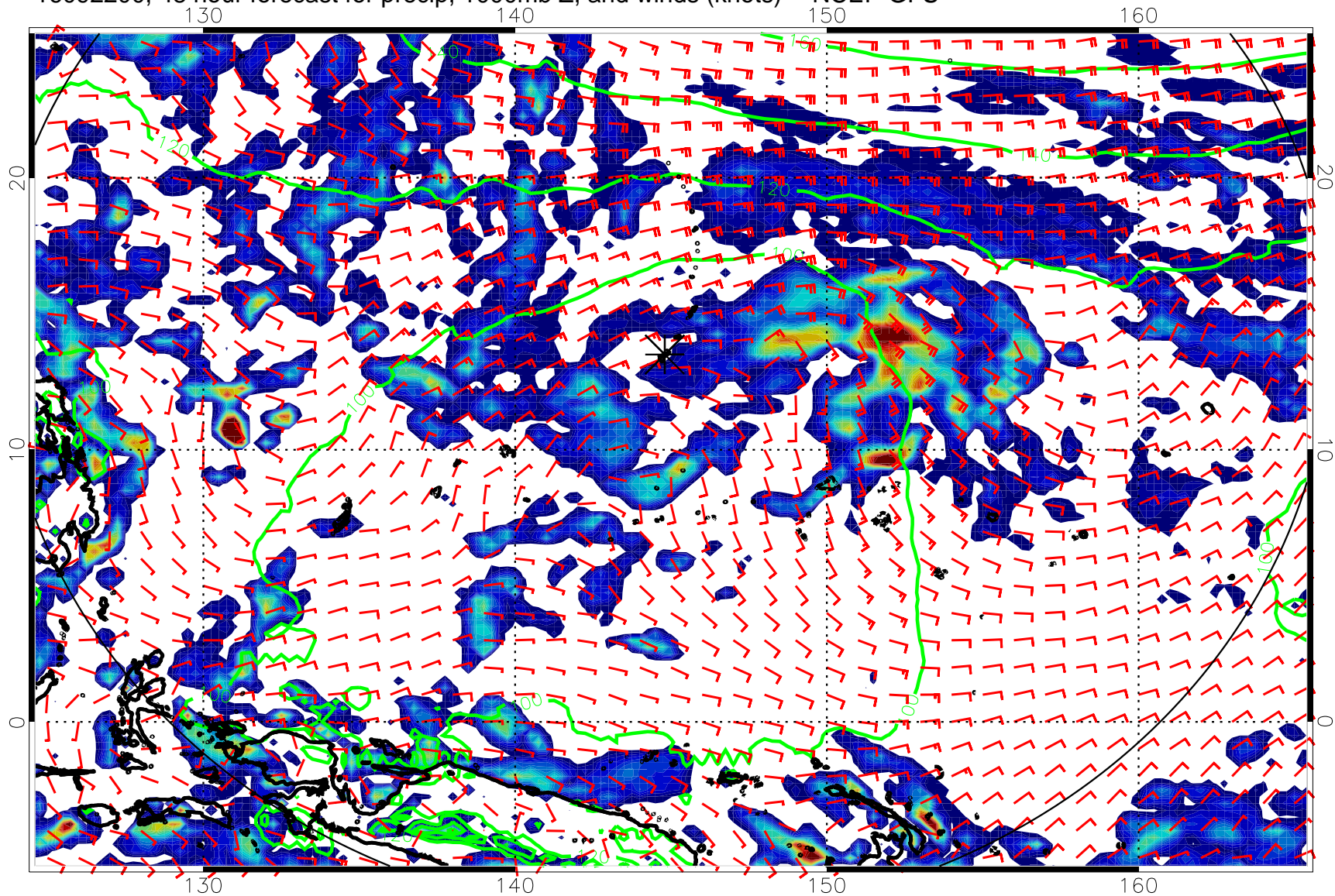
16092200, 48 hour forecast for precip, 1000mb Z, and winds (knots) -- NCEP GFS
