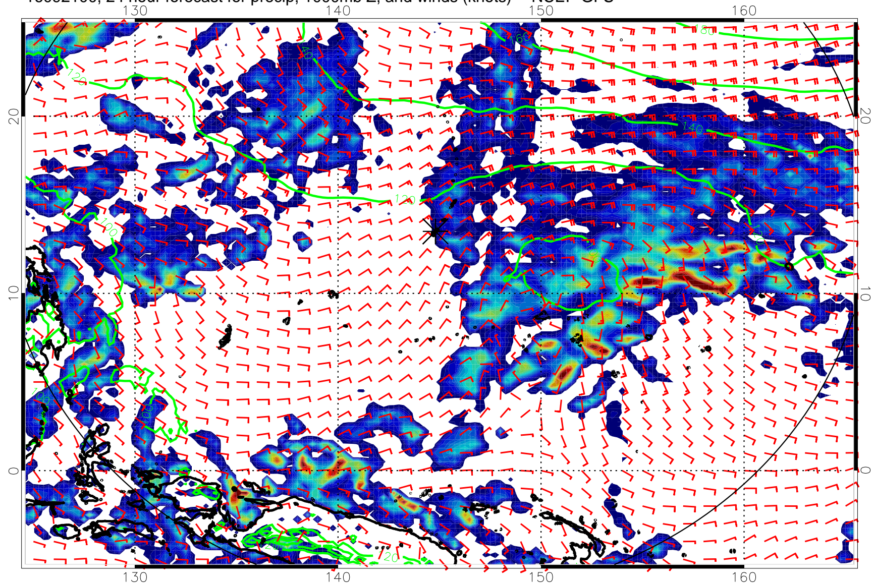
16092100, 24 hour forecast for precip, 1000mb Z, and winds (knots) -- NCEP GFS
