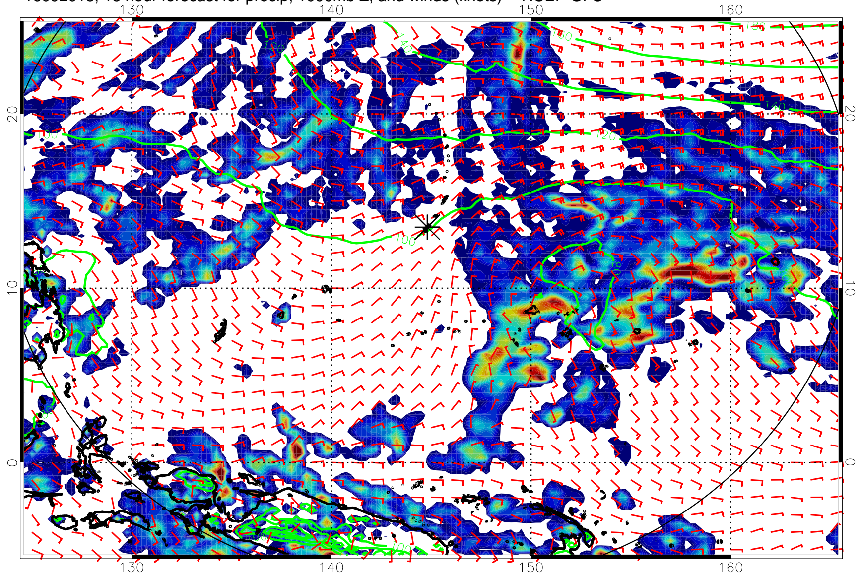
16092018, 18 hour forecast for precip, 1000mb Z, and winds (knots) -- NCEP GFS
