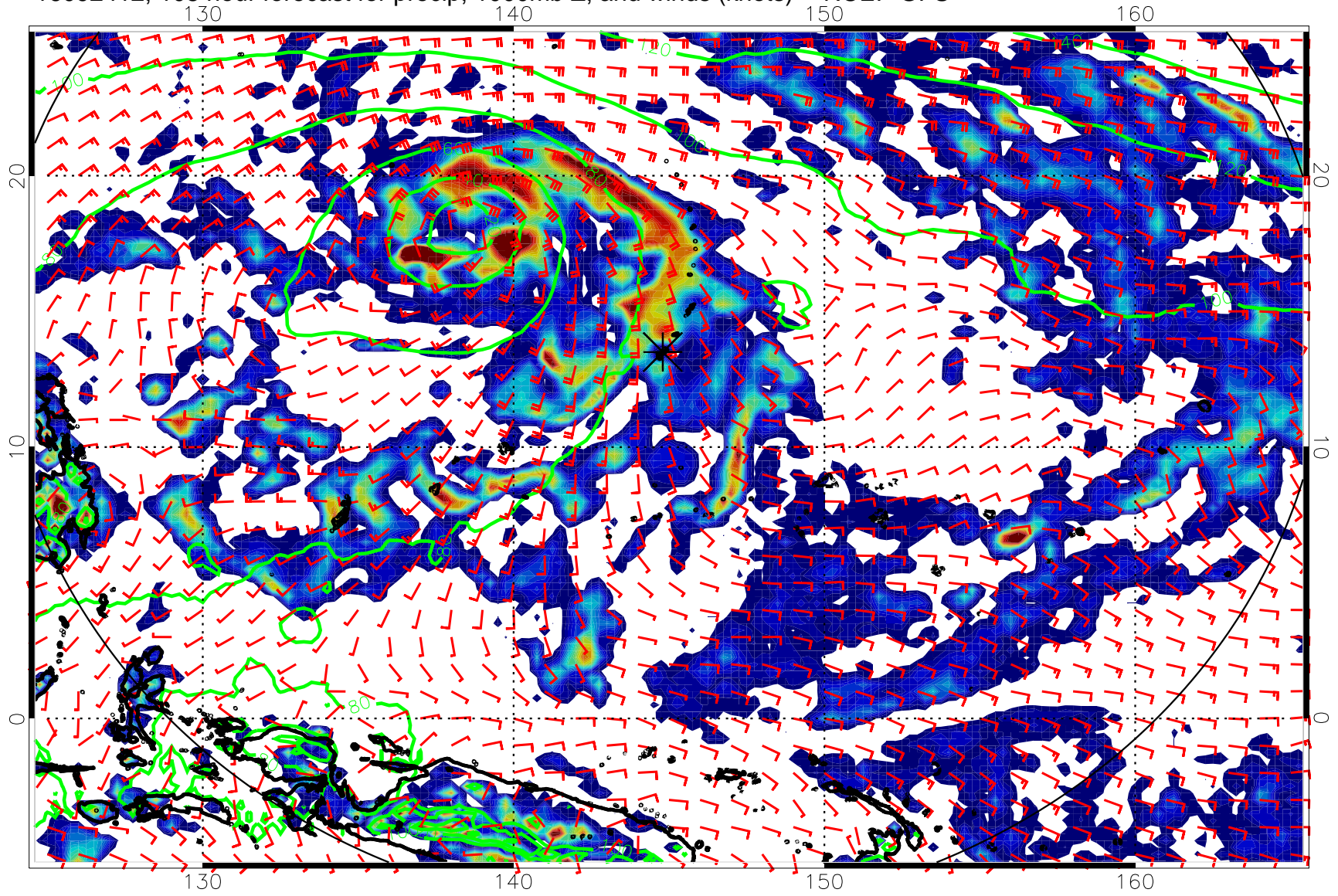
16092412, 108 hour forecast for precip, 1000mb Z, and winds (knots) -- NCEP GFS
