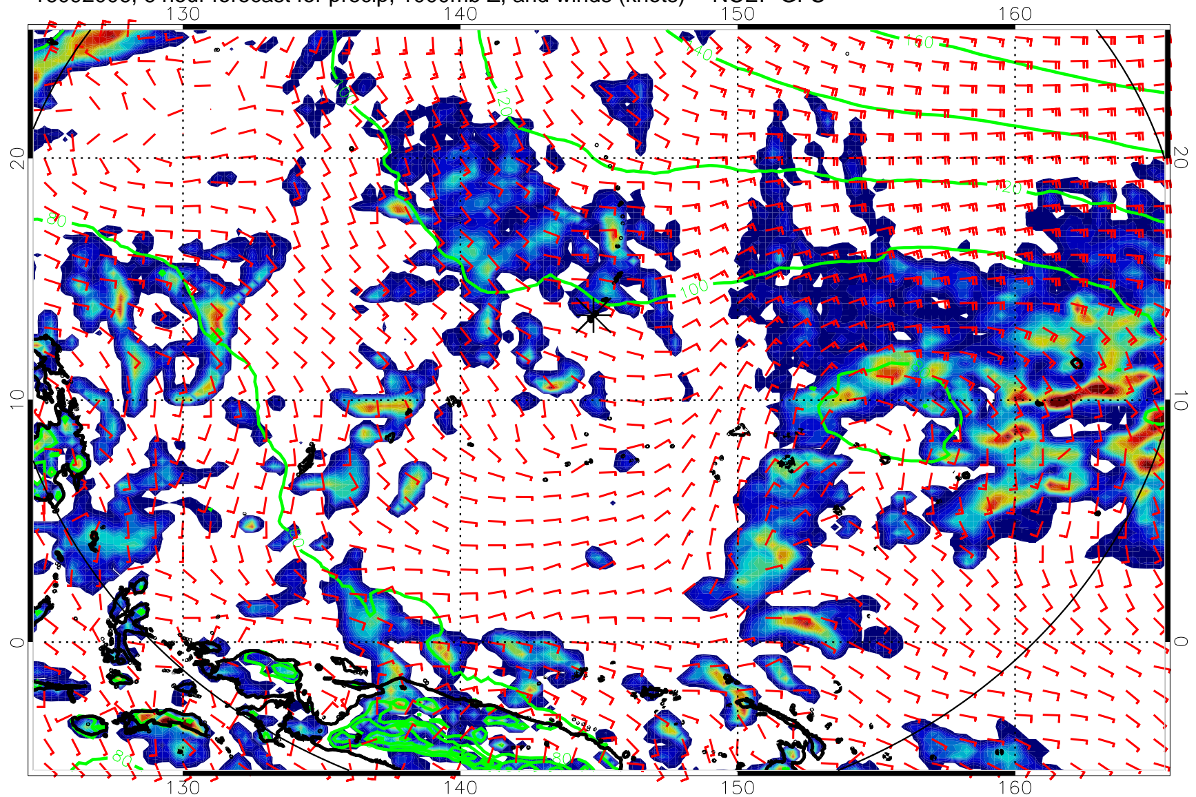
16092006, 6 hour forecast for precip, 1000mb Z, and winds (knots) -- NCEP GFS
