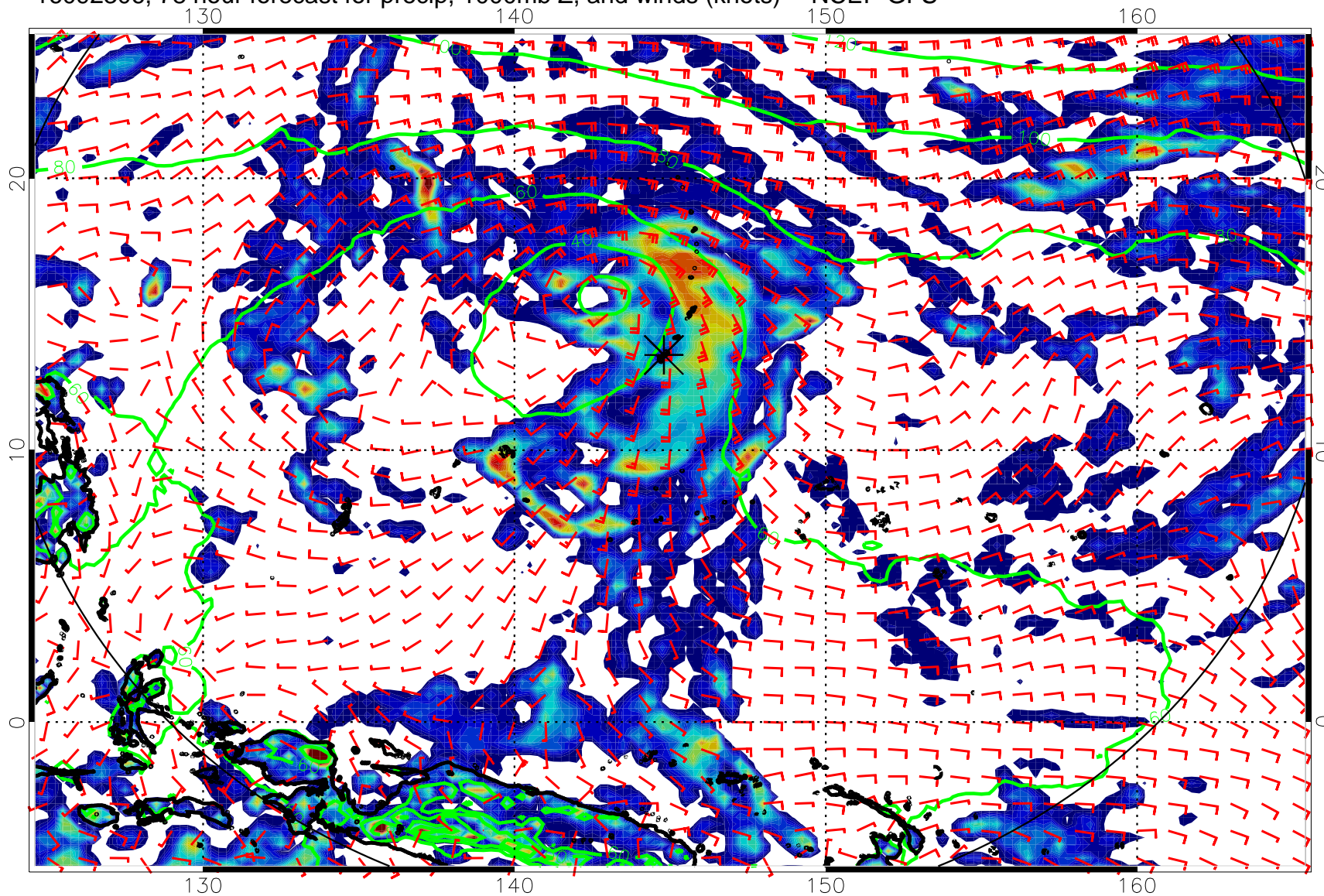
16092306, 78 hour forecast for precip, 1000mb Z, and winds (knots) -- NCEP GFS
