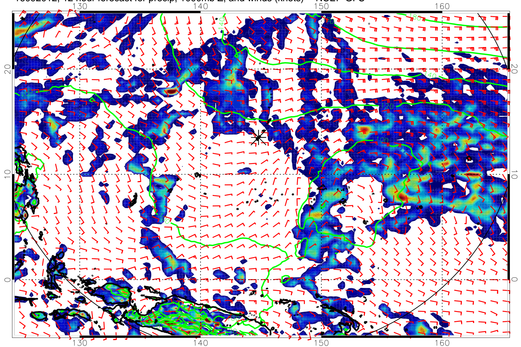
16092012, 12 hour forecast for precip, 1000mb Z, and winds (knots) -- NCEP GFS
