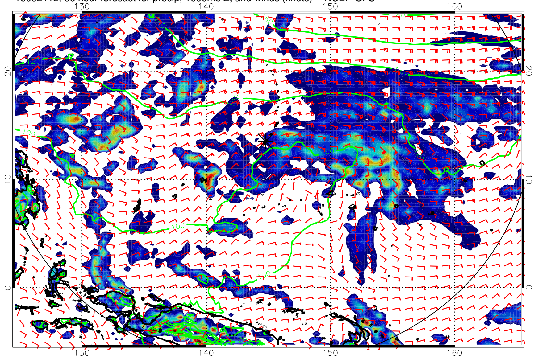
16092112, 36 hour forecast for precip, 1000mb Z, and winds (knots) -- NCEP GFS
