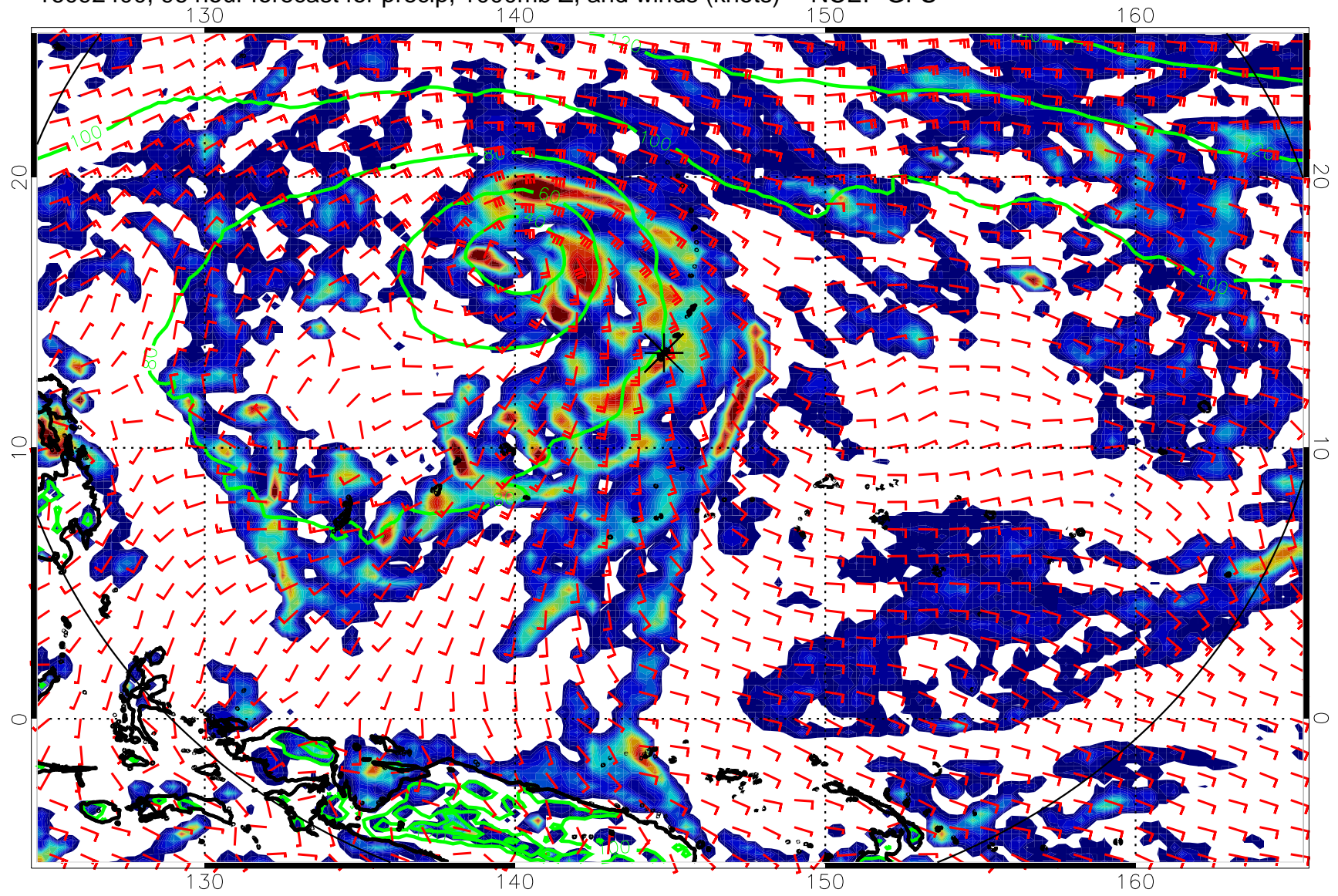
16092400, 96 hour forecast for precip, 1000mb Z, and winds (knots) -- NCEP GFS
