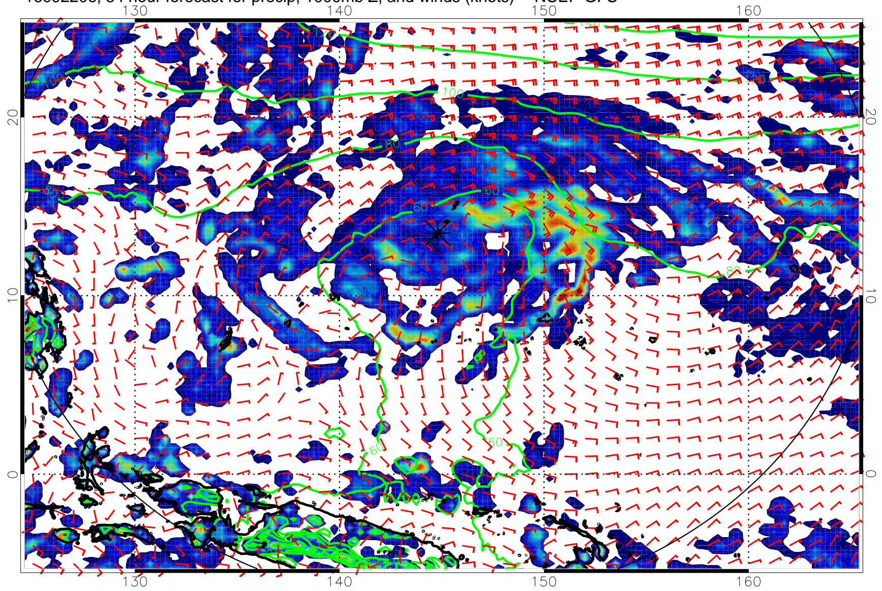
16092206, 54 hour forecast for precip, 1000mb Z, and winds (knots) -- NCEP GFS
