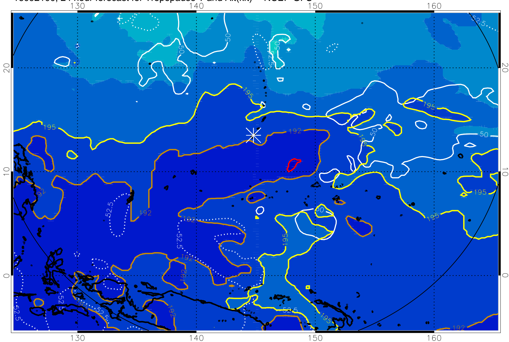
16092100, 24 hour forecast for Tropopause T and Alt(kft) -- NCEP GFS
