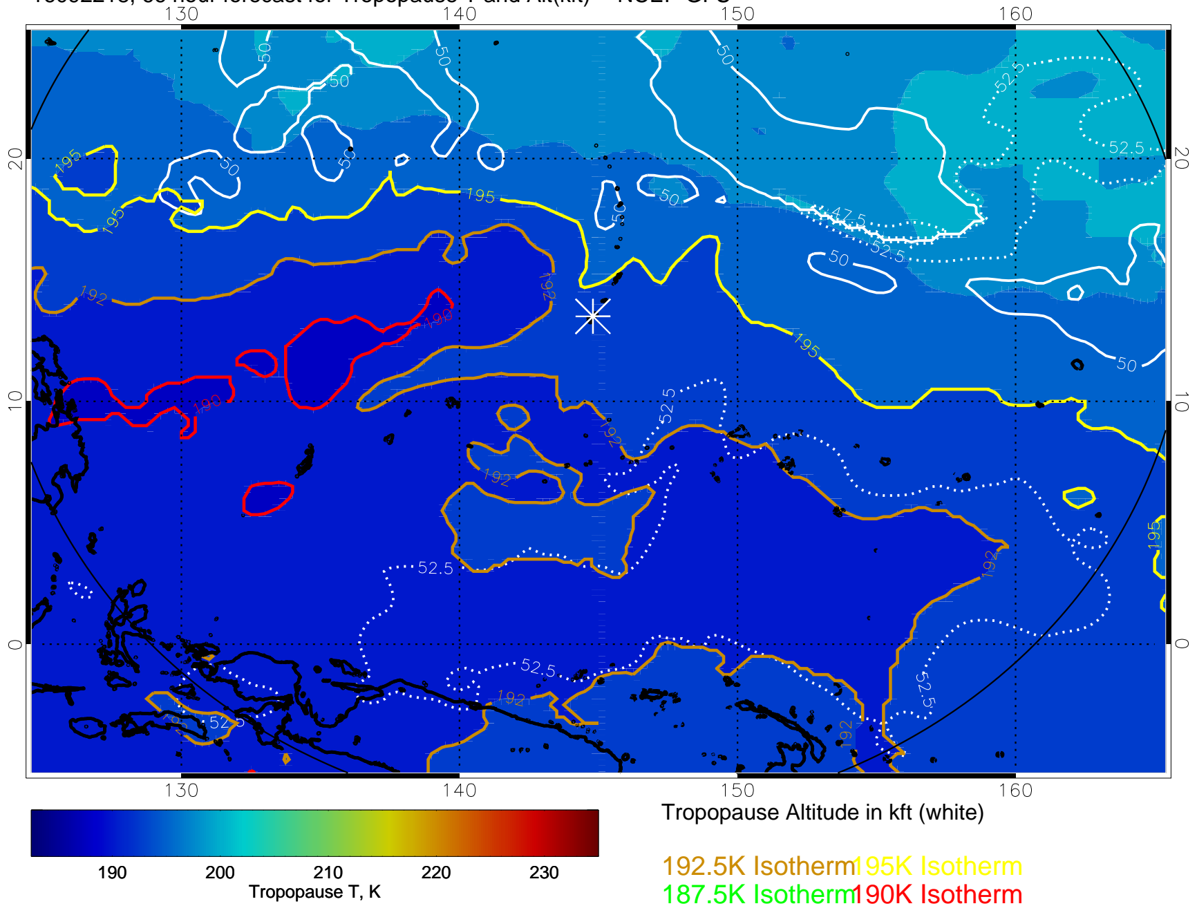
16092218, 66 hour forecast for Tropopause T and Alt(kft) -- NCEP GFS
