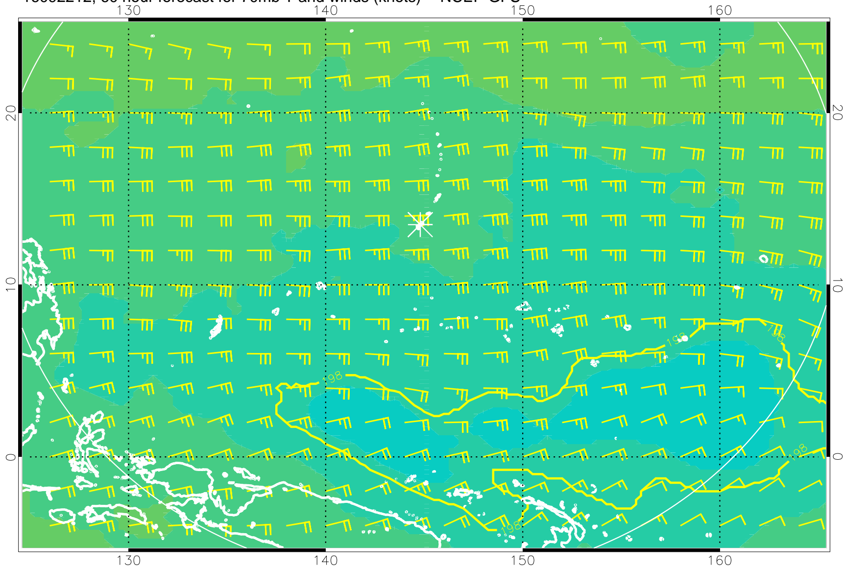
16092212, 60 hour forecast for 70mb T and winds (knots) -- NCEP GFS
