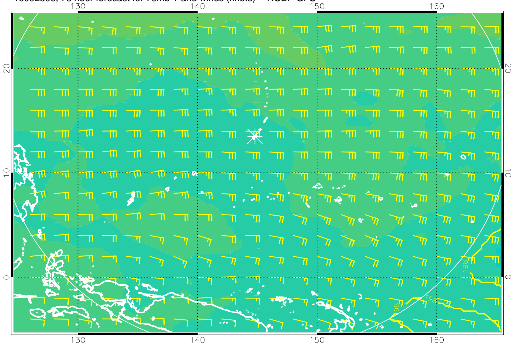
16092306, 78 hour forecast for 70mb T and winds (knots) -- NCEP GFS
