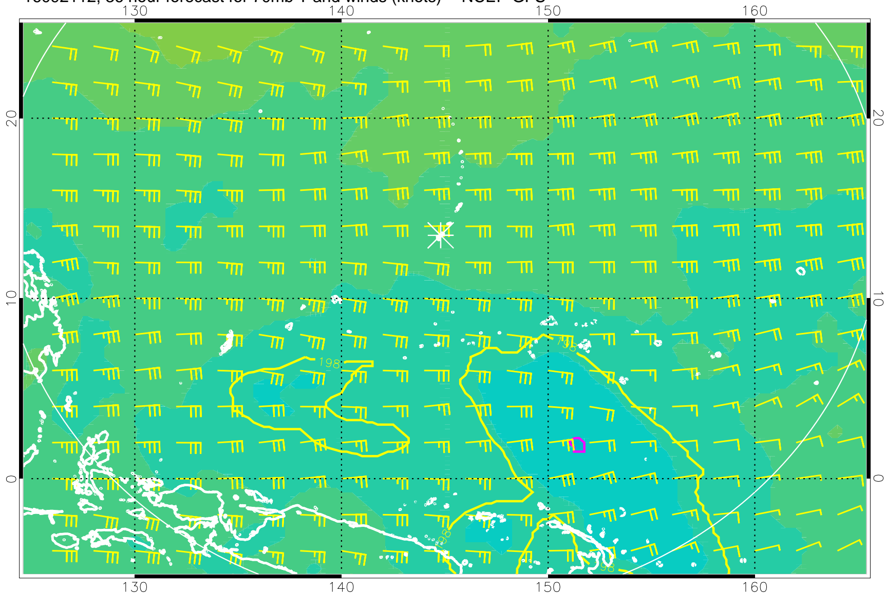
16092112, 36 hour forecast for 70mb T and winds (knots) -- NCEP GFS
