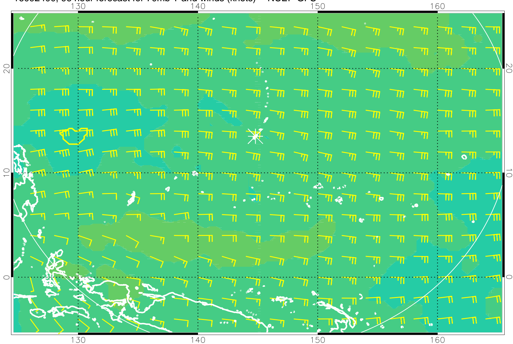
16092400, 96 hour forecast for 70mb T and winds (knots) -- NCEP GFS
