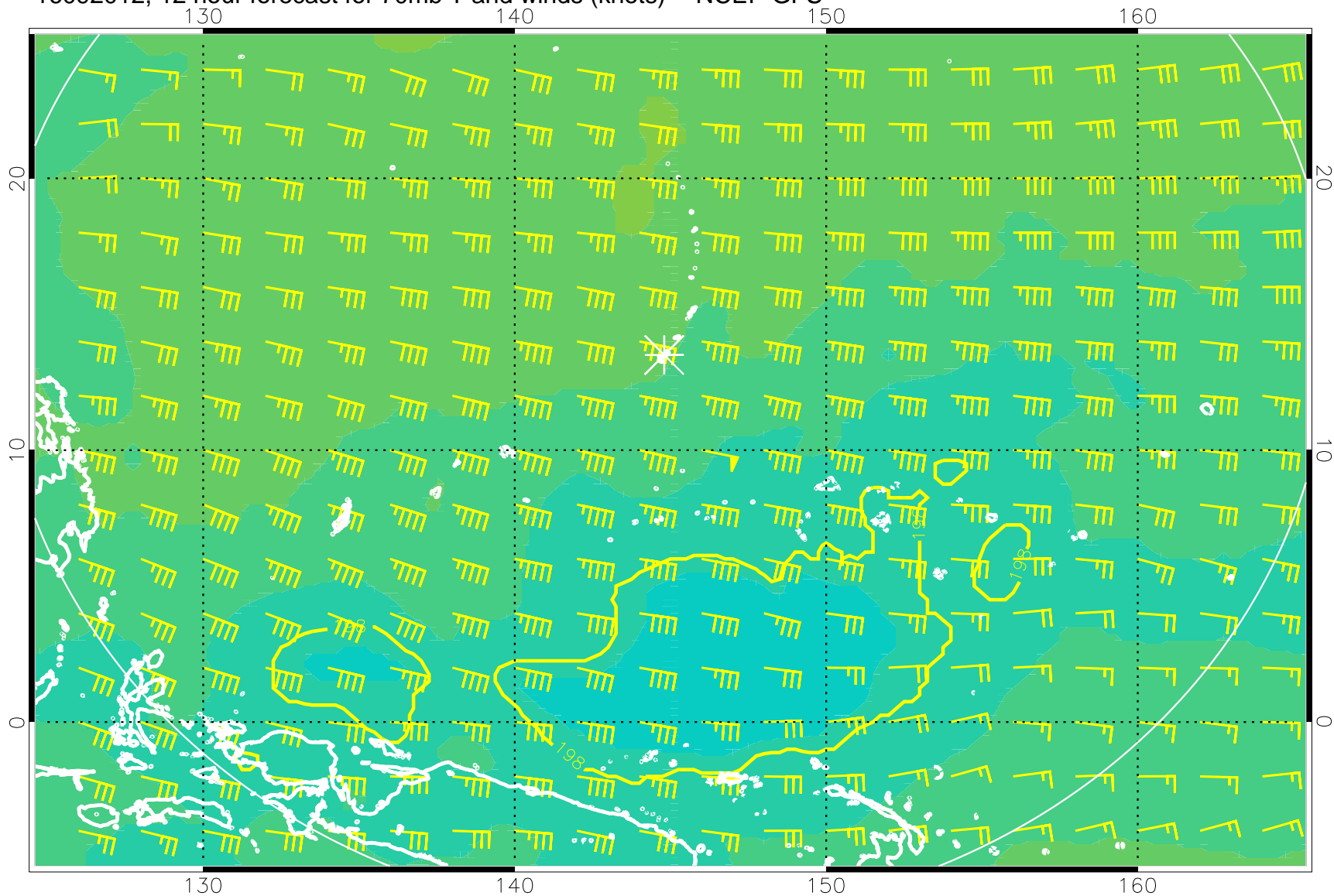
16092012, 12 hour forecast for 70mb T and winds (knots) -- NCEP GFS
