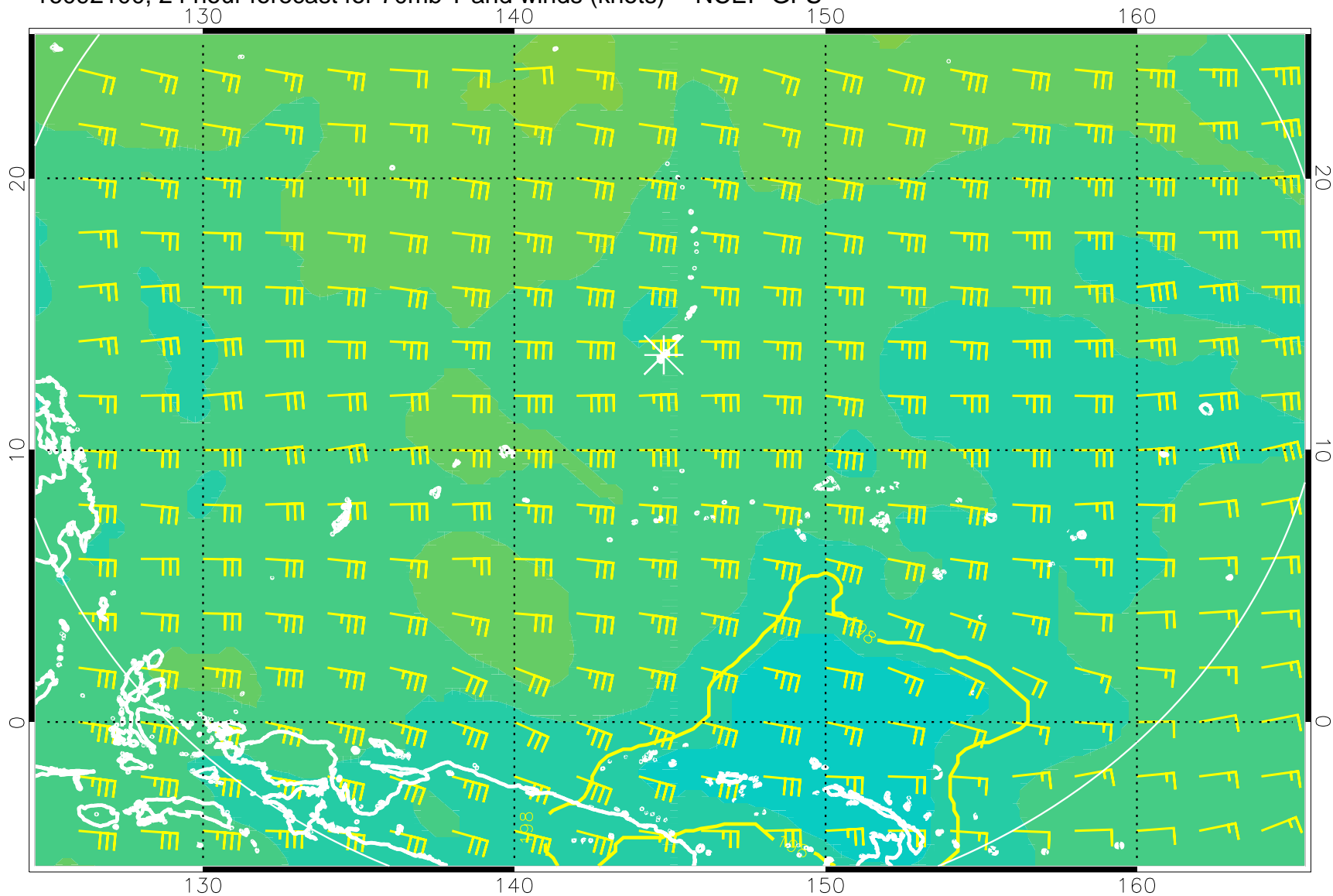
16092100, 24 hour forecast for 70mb T and winds (knots) -- NCEP GFS
