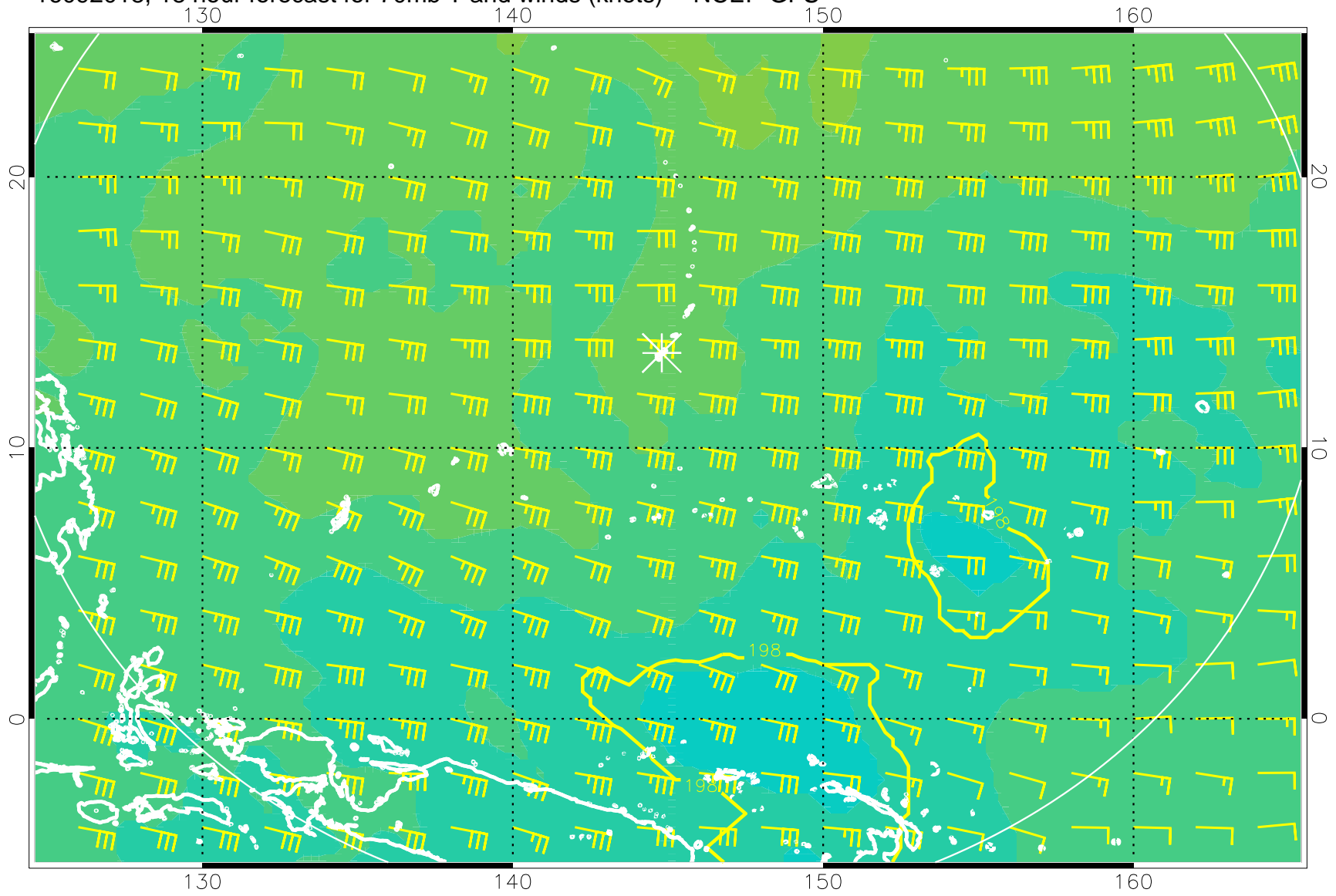
16092018, 18 hour forecast for 70mb T and winds (knots) -- NCEP GFS
