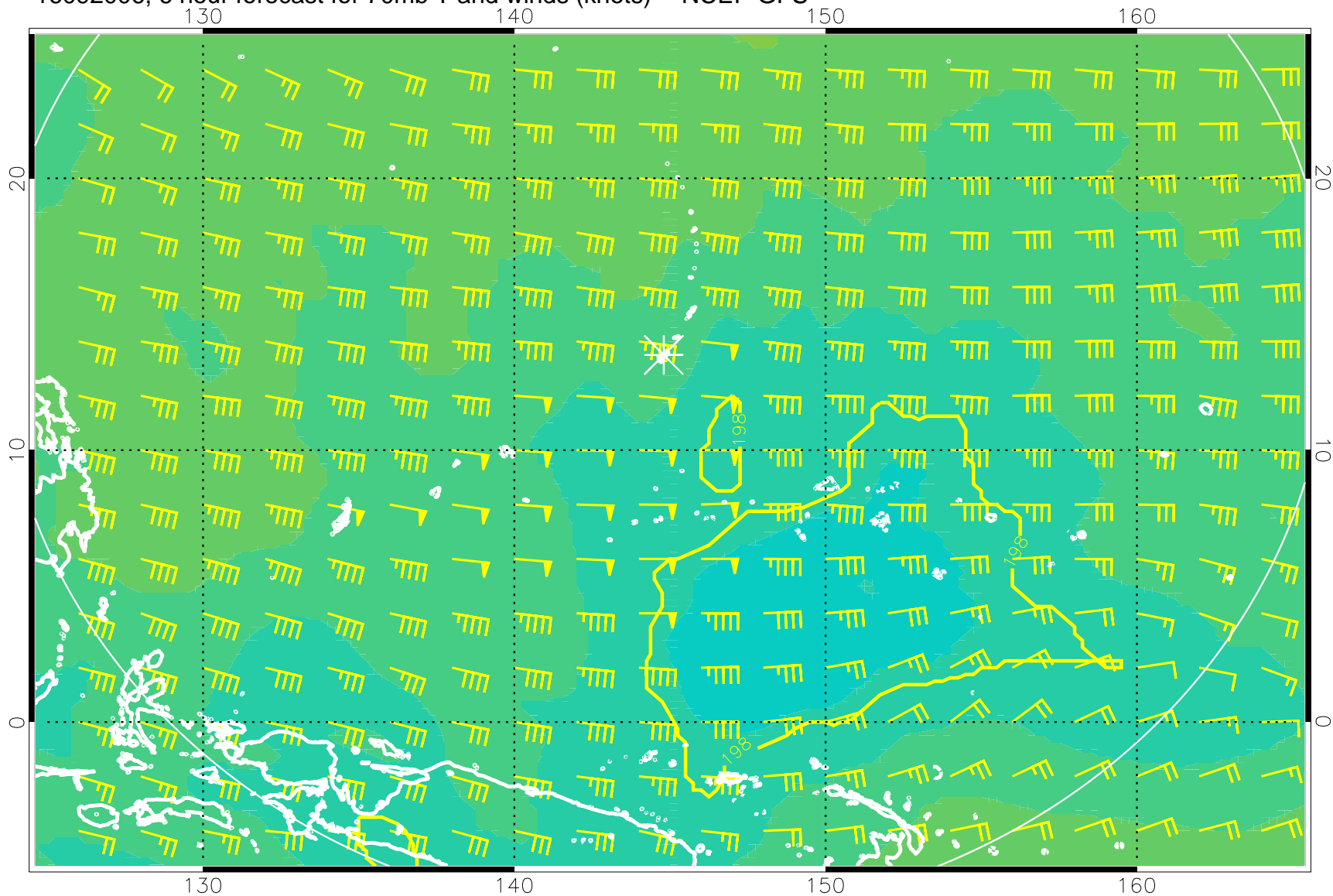
16092006, 6 hour forecast for 70mb T and winds (knots) -- NCEP GFS
