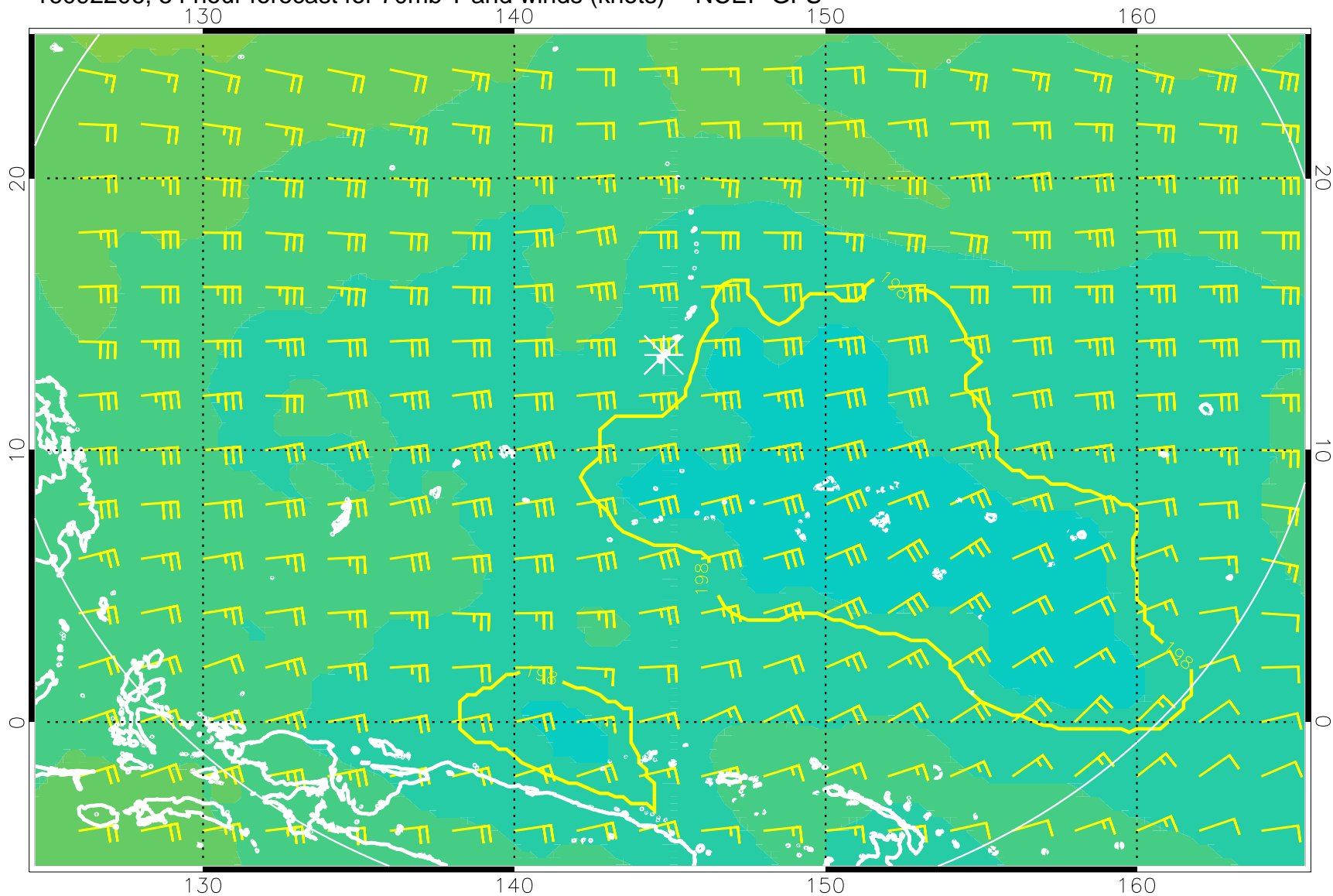
16092206, 54 hour forecast for 70mb T and winds (knots) -- NCEP GFS
