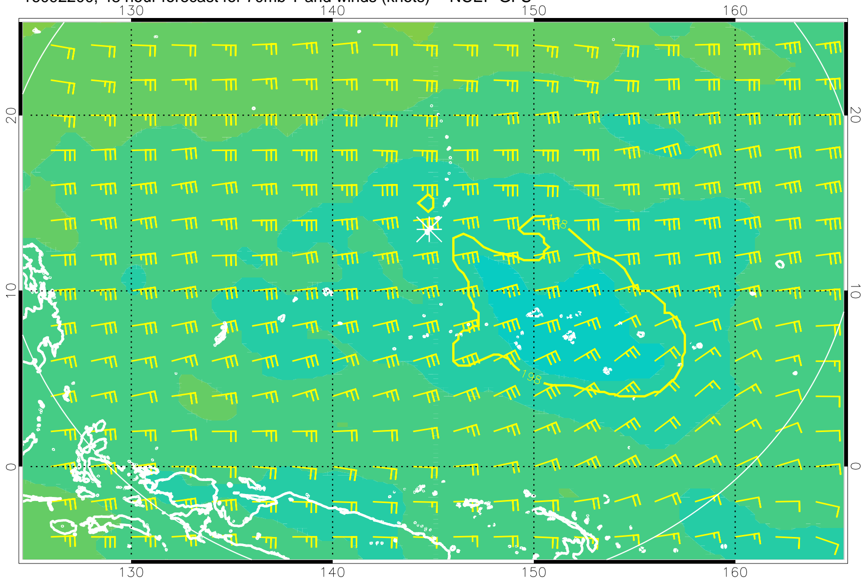
16092200, 48 hour forecast for 70mb T and winds (knots) -- NCEP GFS
