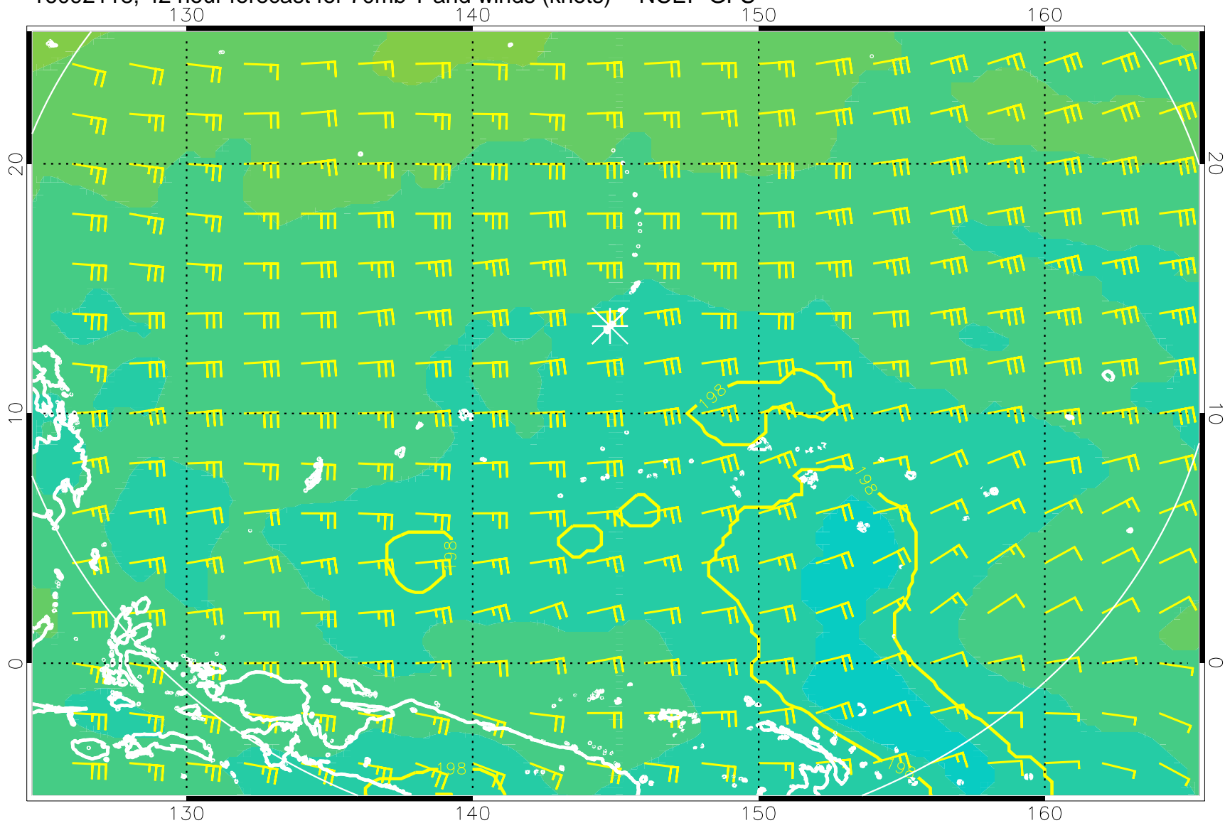
16092118, 42 hour forecast for 70mb T and winds (knots) -- NCEP GFS
