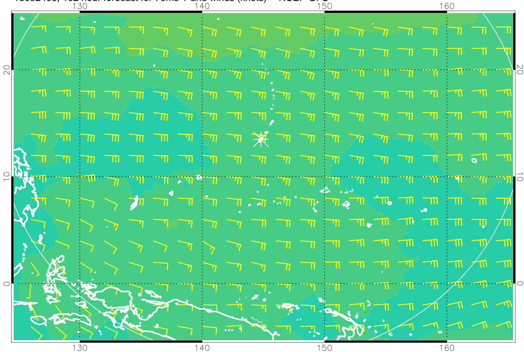
16092406, 102 hour forecast for 70mb T and winds (knots) -- NCEP GFS
