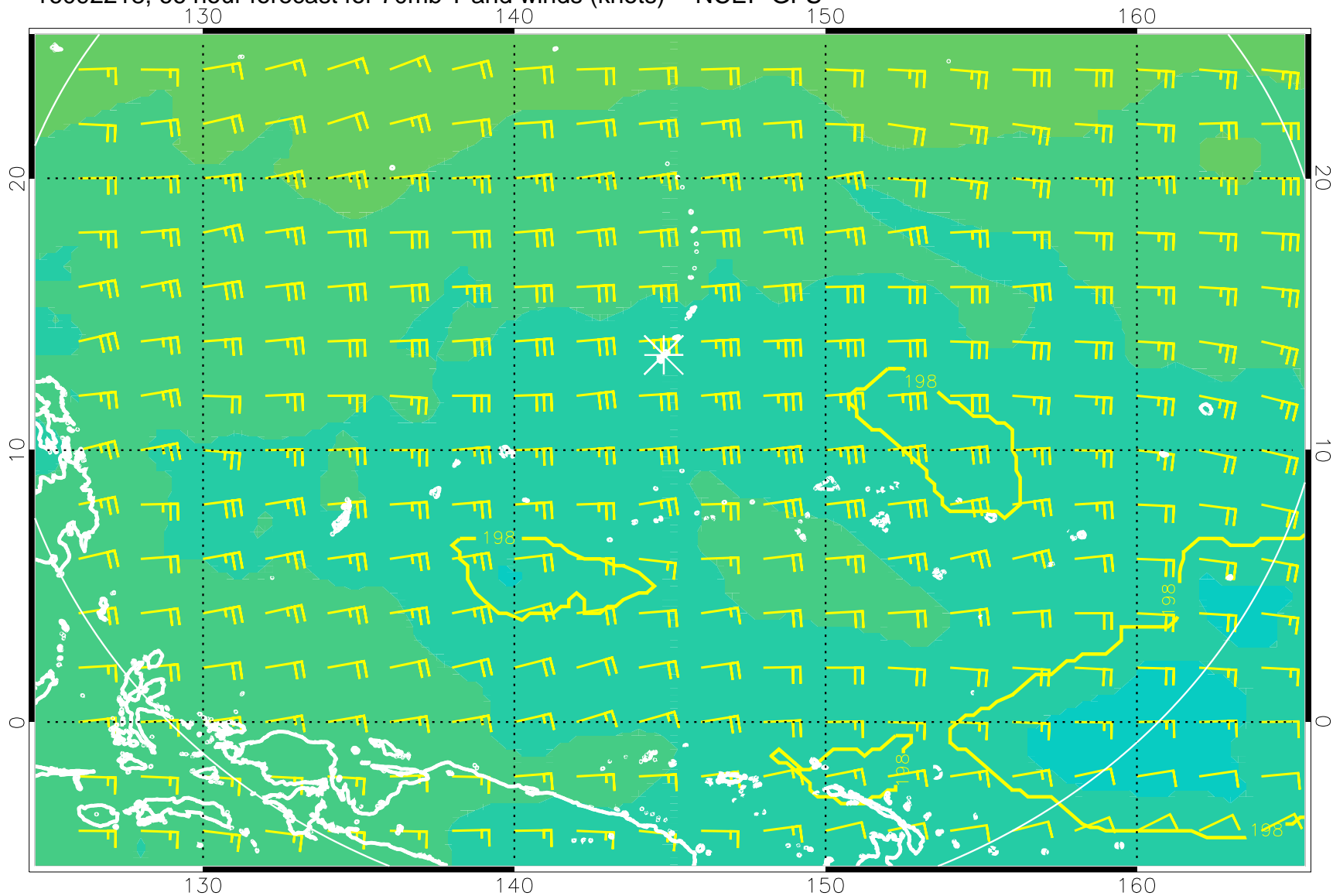
16092218, 66 hour forecast for 70mb T and winds (knots) -- NCEP GFS
