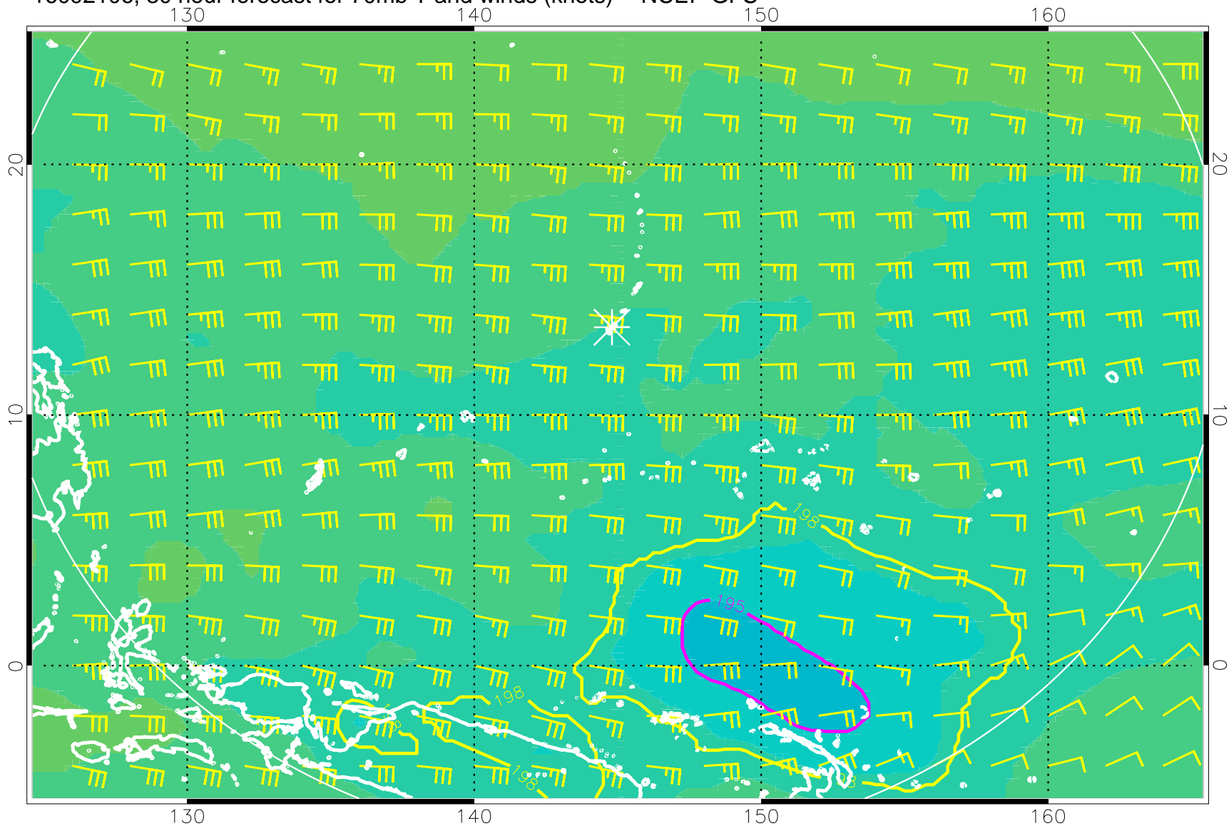
16092106, 30 hour forecast for 70mb T and winds (knots) -- NCEP GFS
