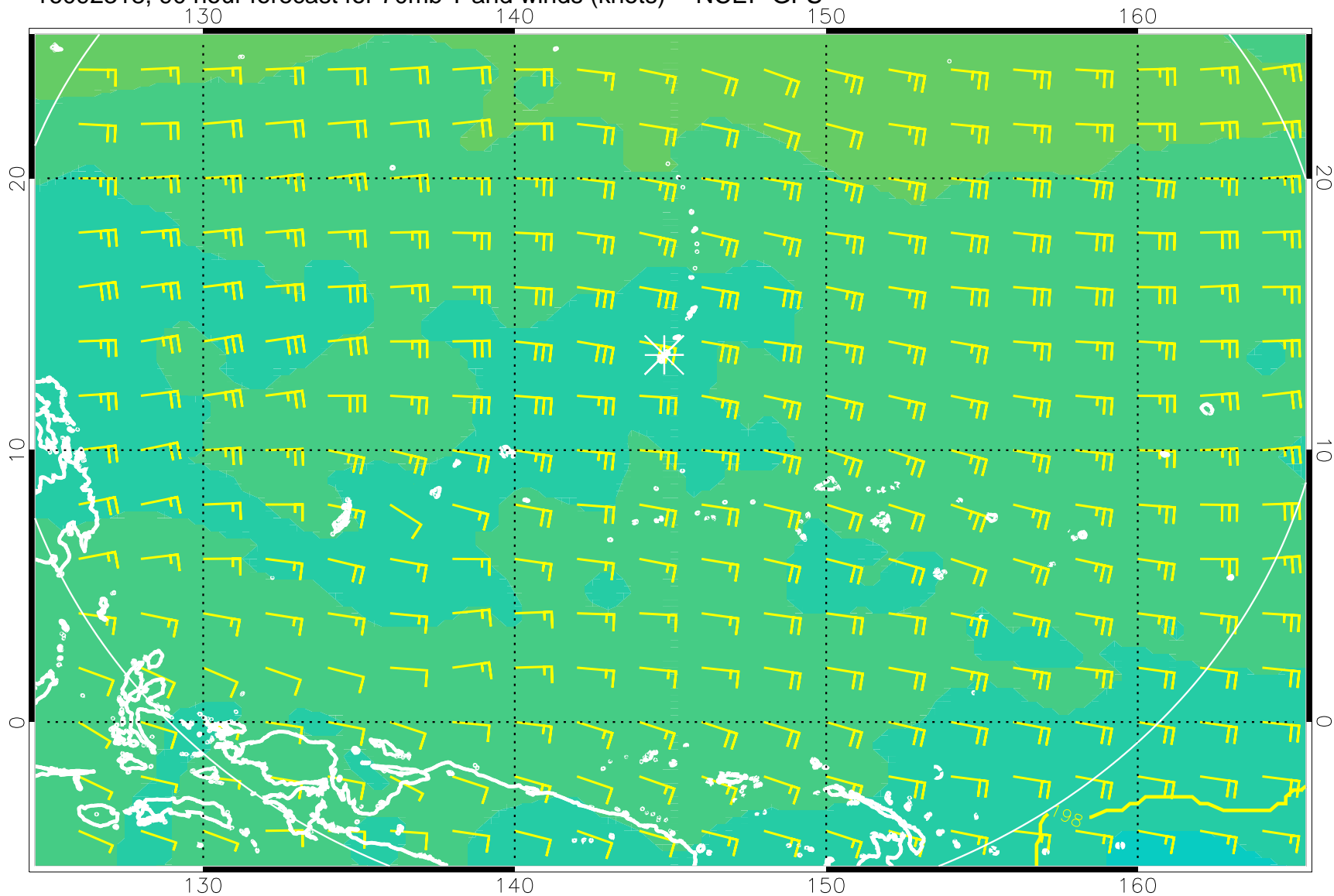
16092318, 90 hour forecast for 70mb T and winds (knots) -- NCEP GFS
