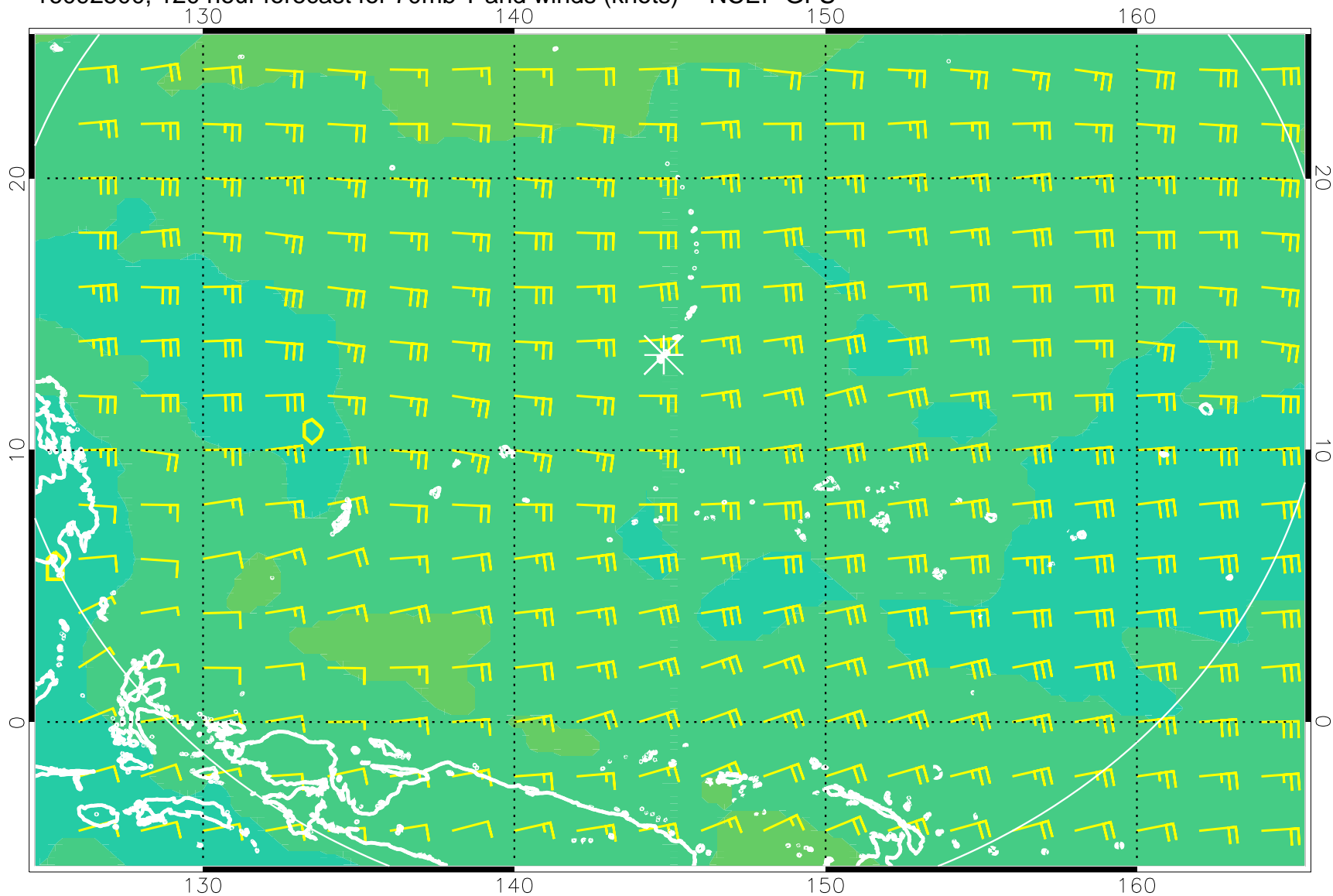
16092500, 120 hour forecast for 70mb T and winds (knots) -- NCEP GFS
