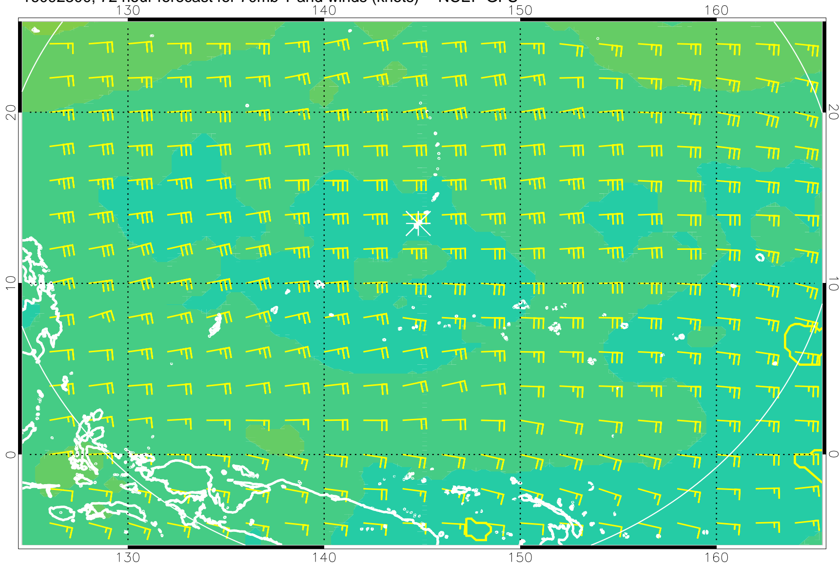
16092300, 72 hour forecast for 70mb T and winds (knots) -- NCEP GFS
