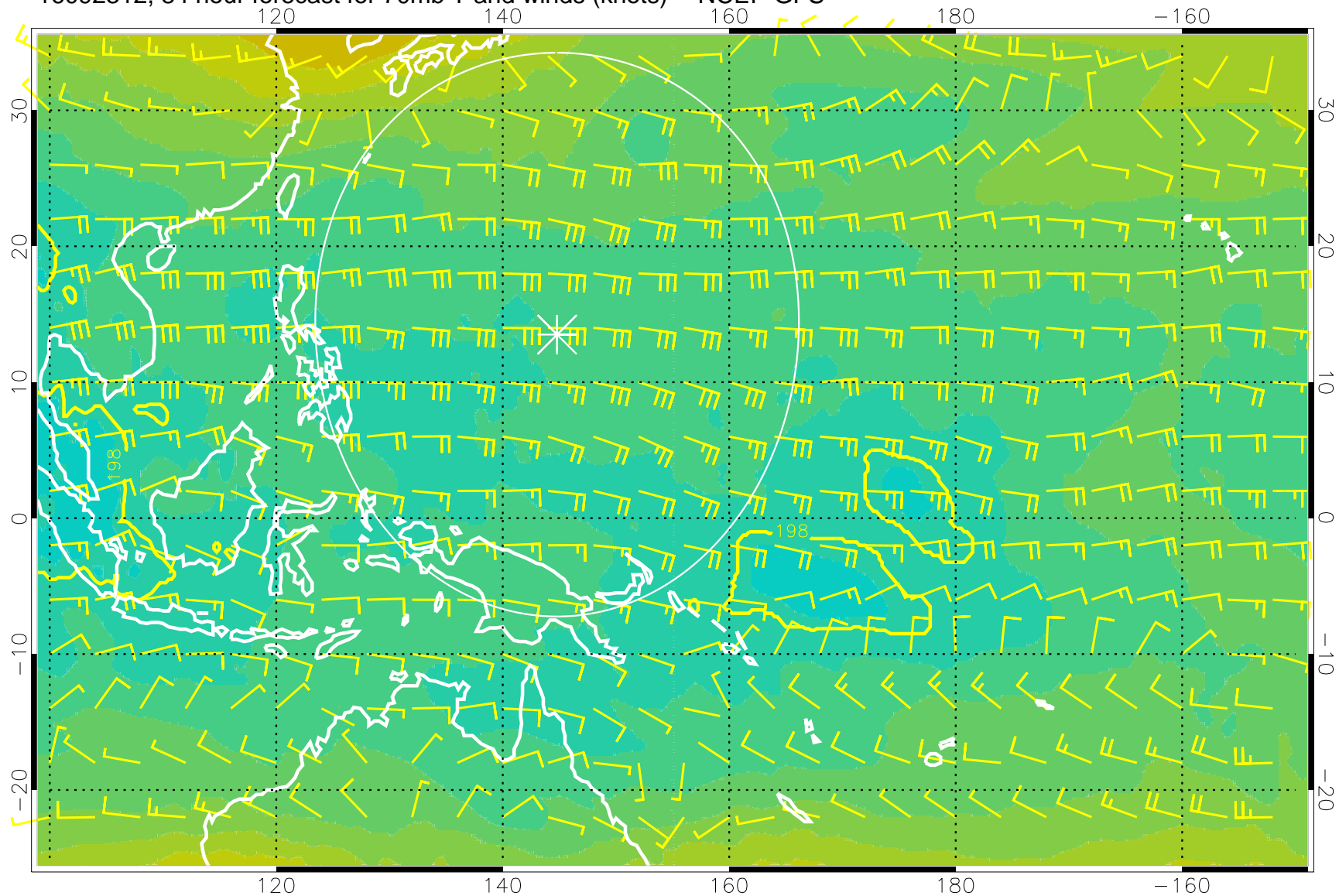
16092312, 84 hour forecast for 70mb T and winds (knots) -- NCEP GFS
