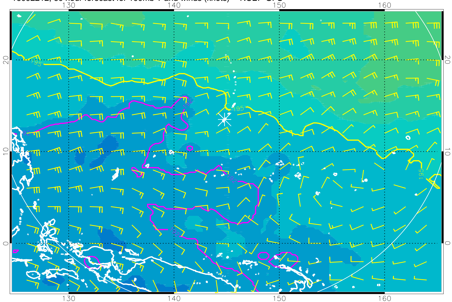
16092212, 60 hour forecast for 100mb T and winds (knots) -- NCEP GFS
