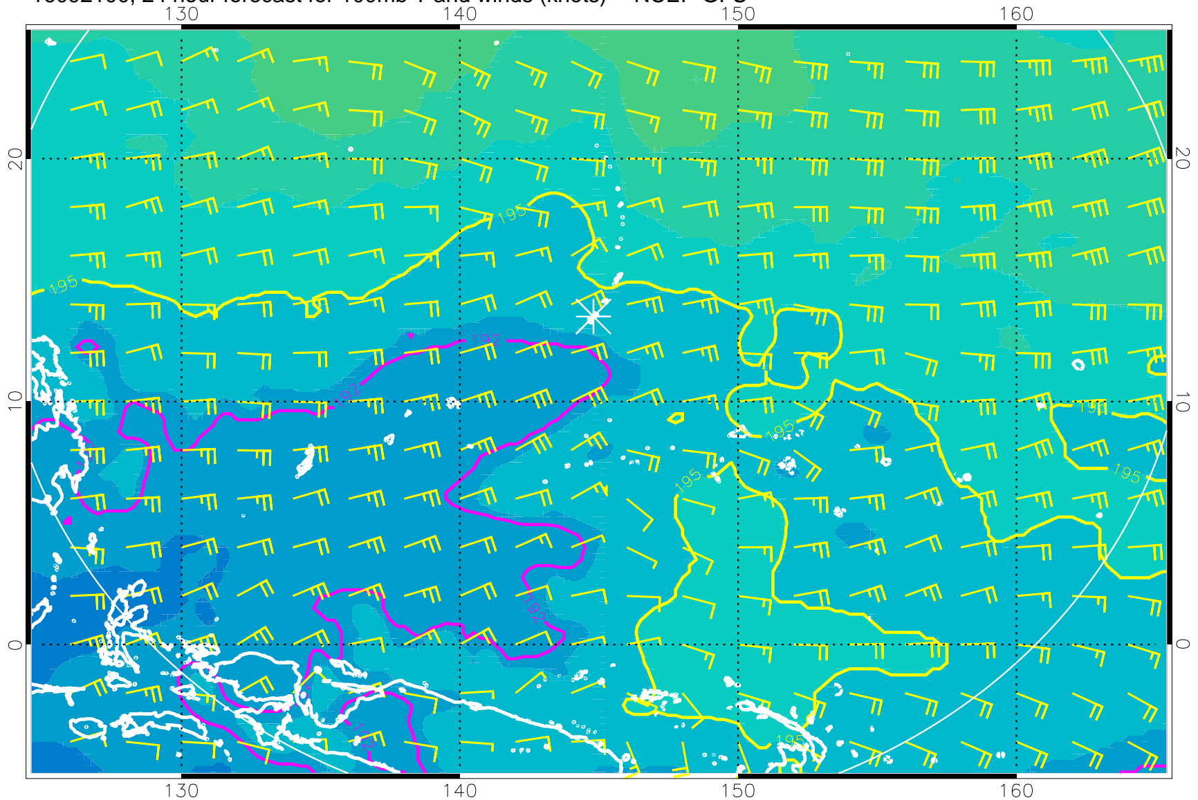
16092100, 24 hour forecast for 100mb T and winds (knots) -- NCEP GFS
