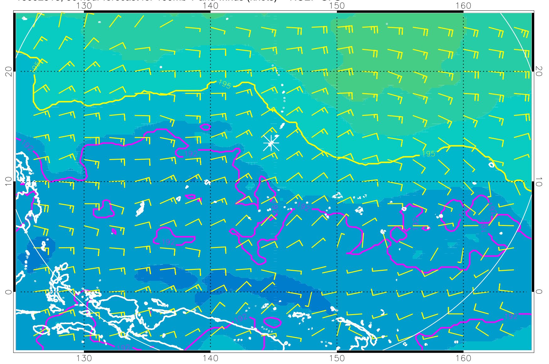
16092318, 90 hour forecast for 100mb T and winds (knots) -- NCEP GFS
