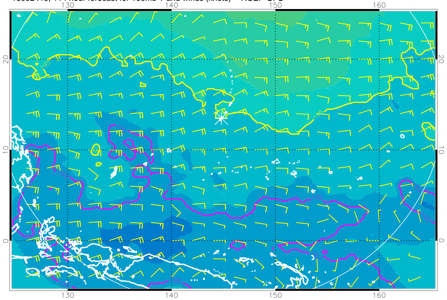
16092418, 114 hour forecast for 100mb T and winds (knots) -- NCEP GFS
