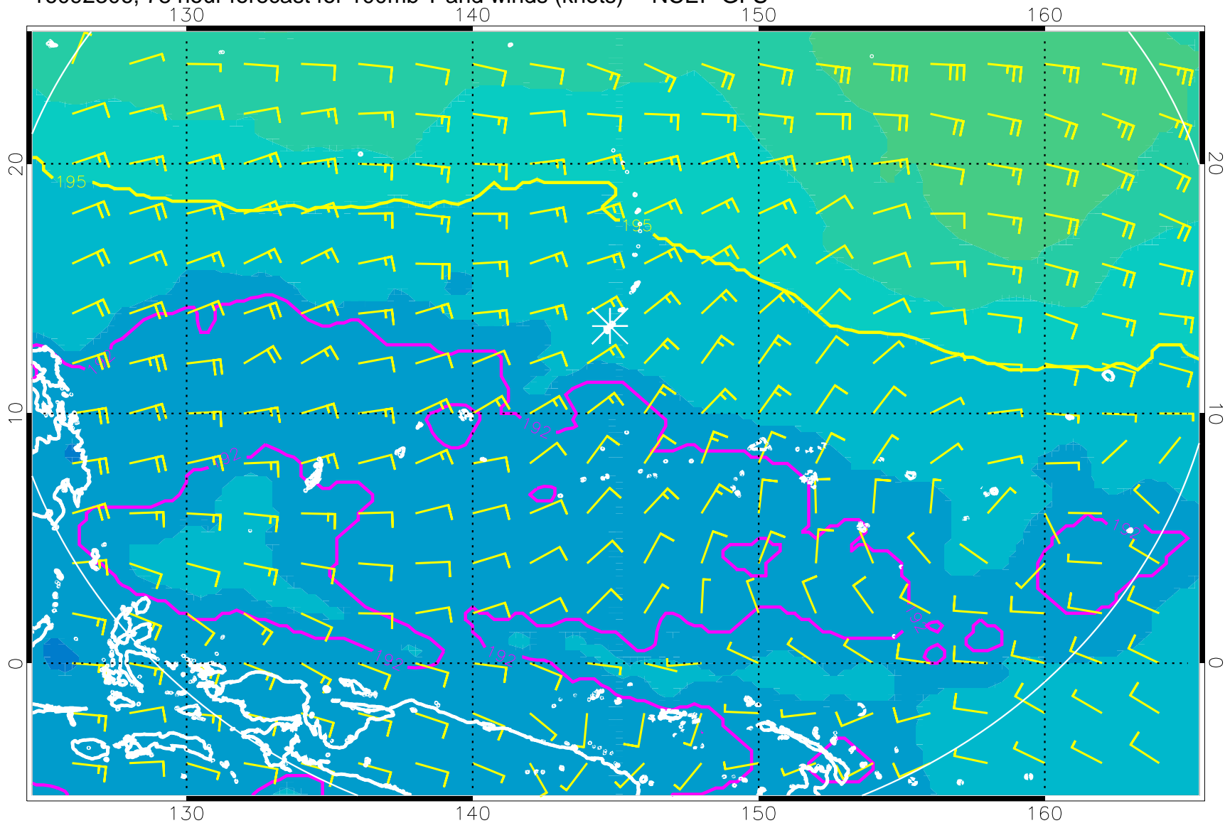
16092306, 78 hour forecast for 100mb T and winds (knots) -- NCEP GFS
