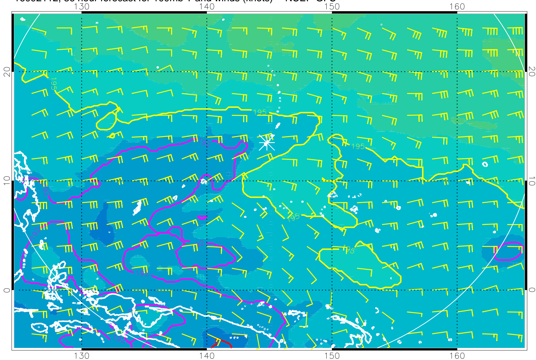
16092112, 36 hour forecast for 100mb T and winds (knots) -- NCEP GFS
