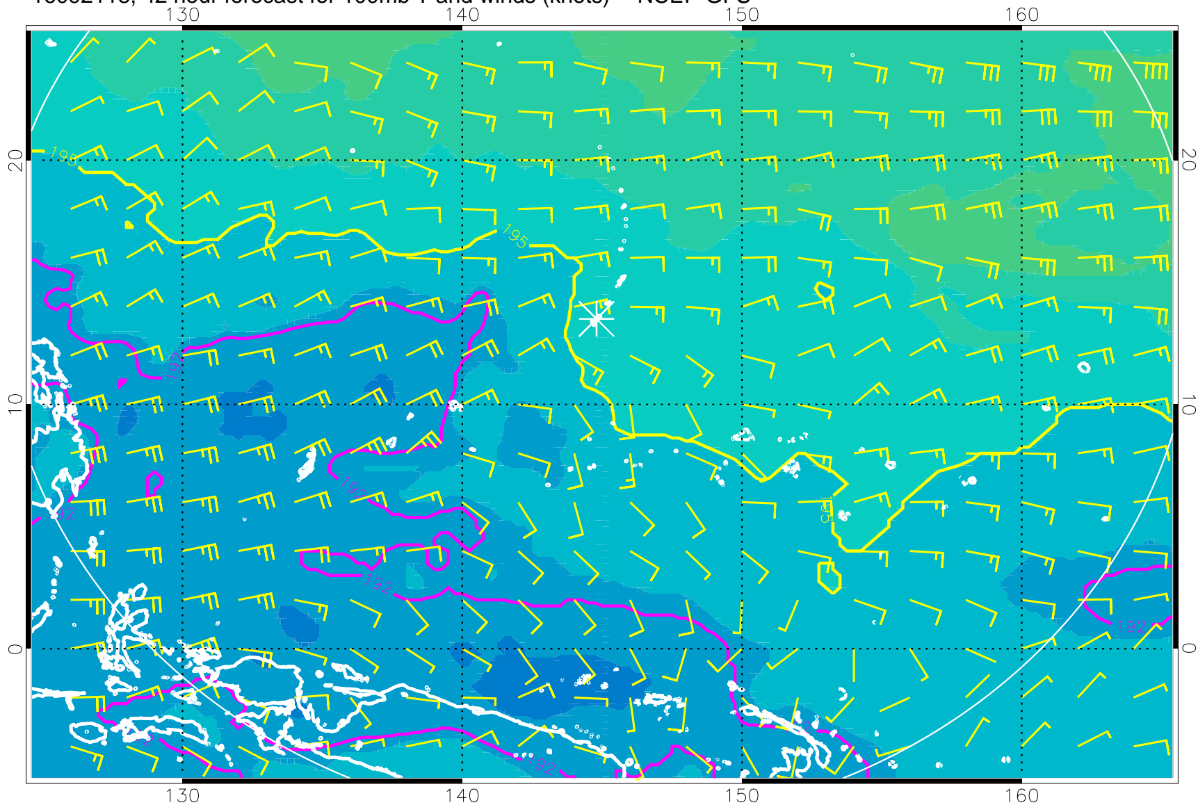
16092118, 42 hour forecast for 100mb T and winds (knots) -- NCEP GFS
