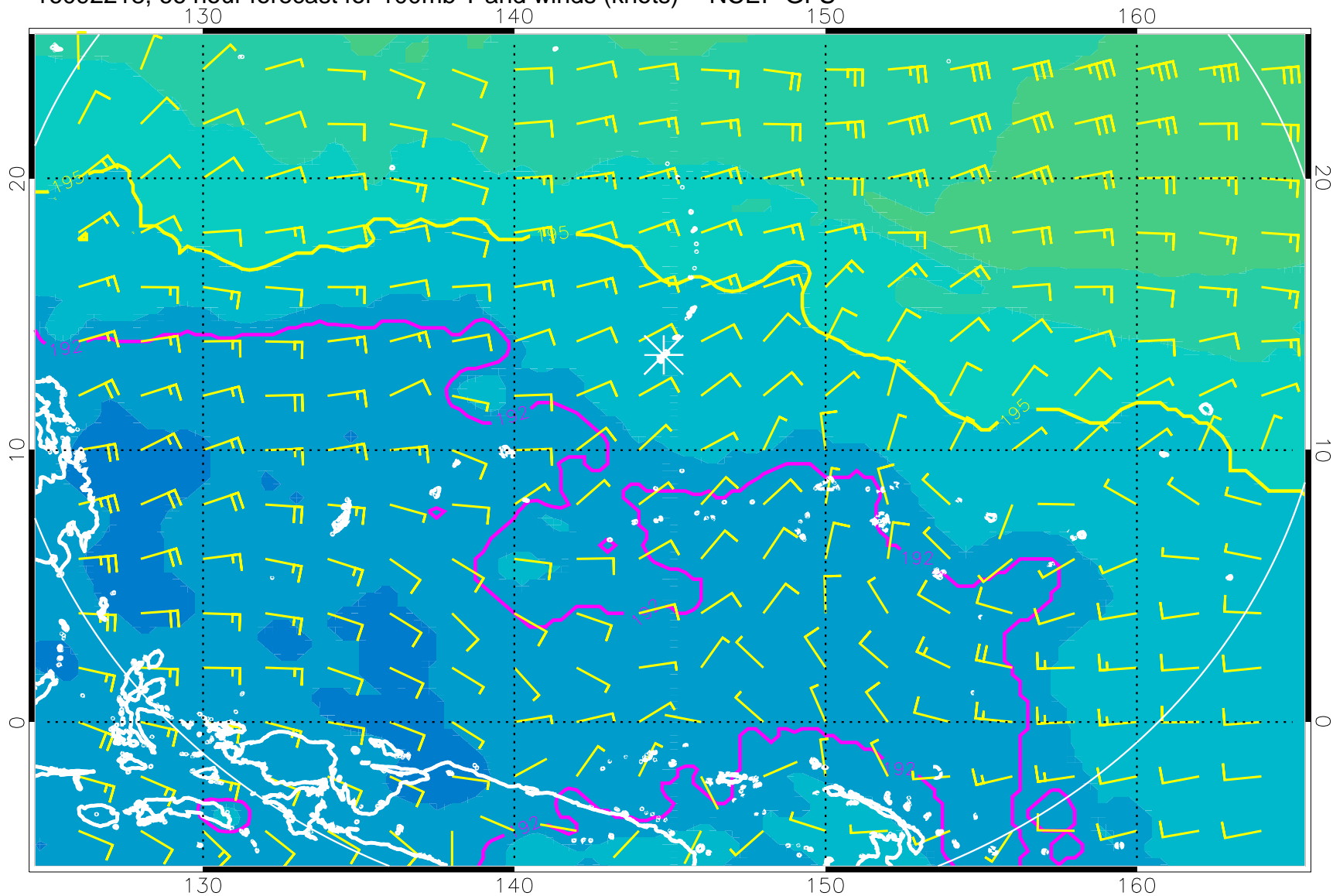
16092218, 66 hour forecast for 100mb T and winds (knots) -- NCEP GFS
