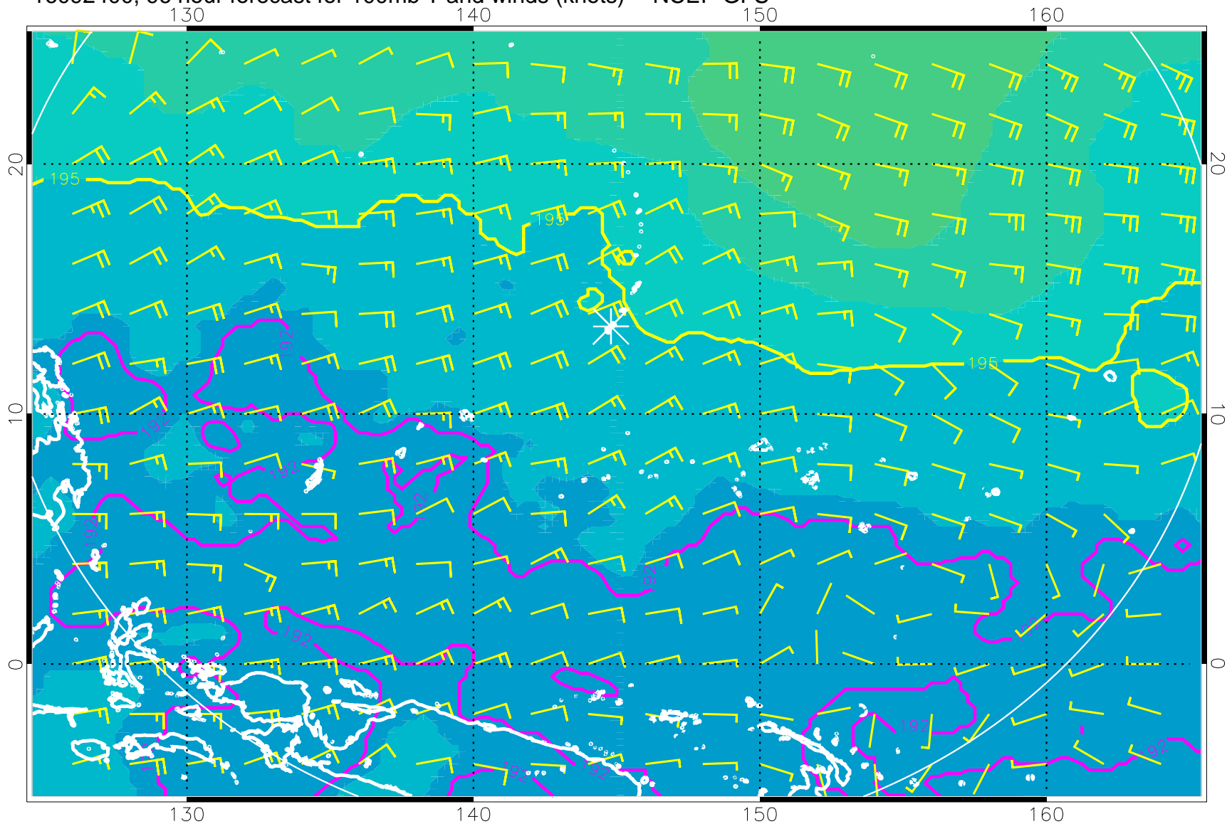
16092400, 96 hour forecast for 100mb T and winds (knots) -- NCEP GFS
