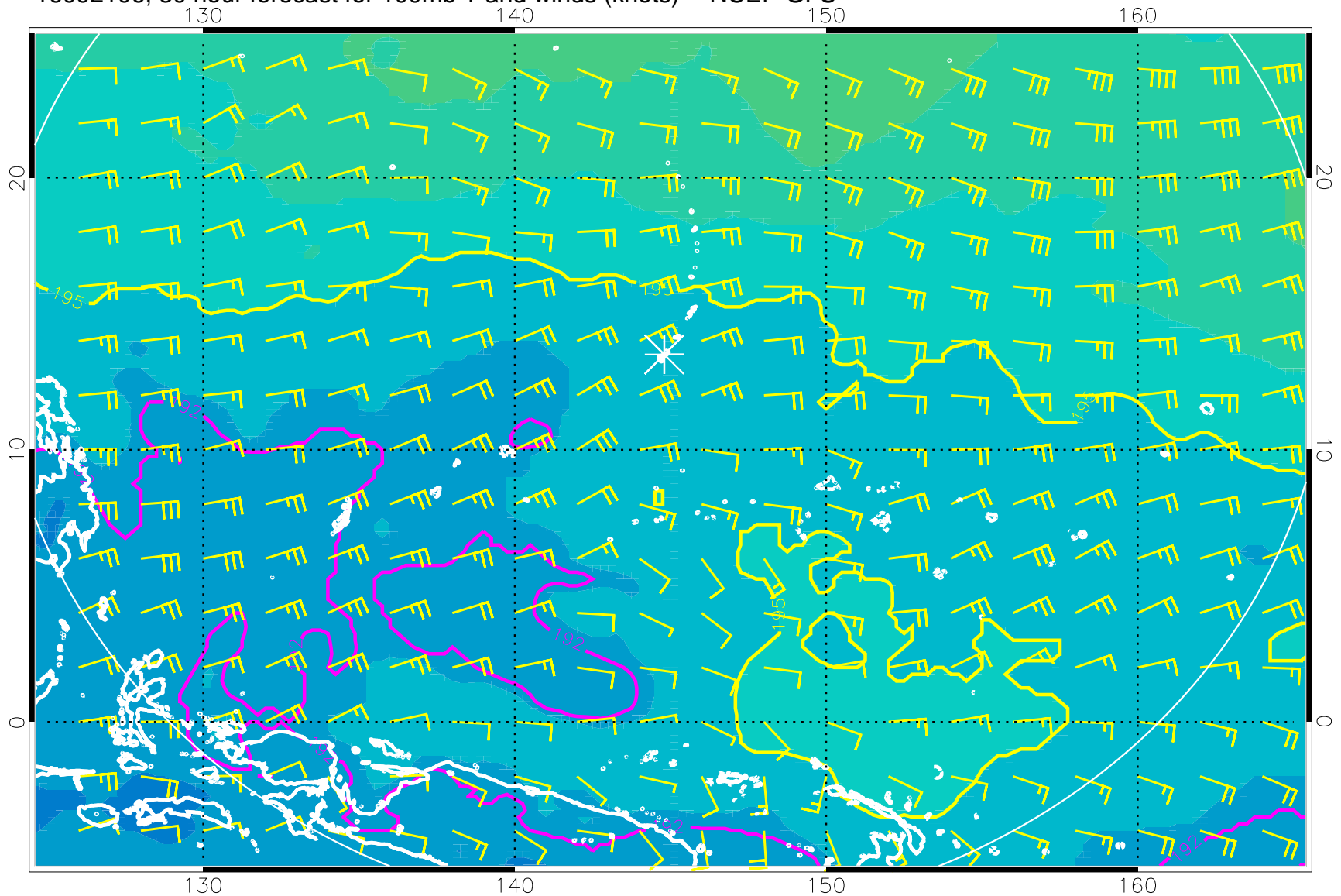
16092106, 30 hour forecast for 100mb T and winds (knots) -- NCEP GFS
