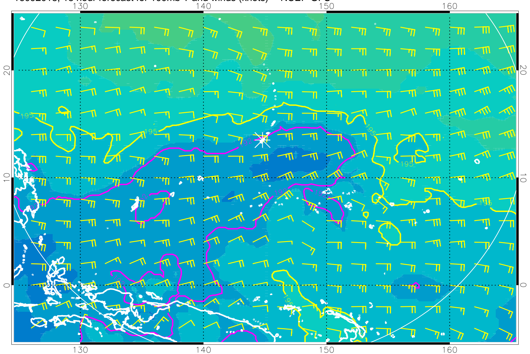
16092018, 18 hour forecast for 100mb T and winds (knots) -- NCEP GFS
