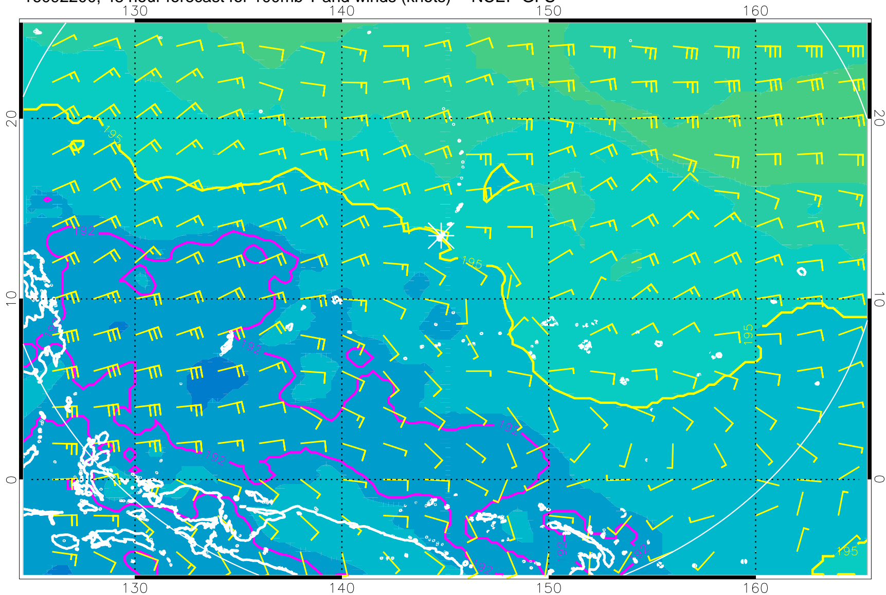
16092200, 48 hour forecast for 100mb T and winds (knots) -- NCEP GFS
