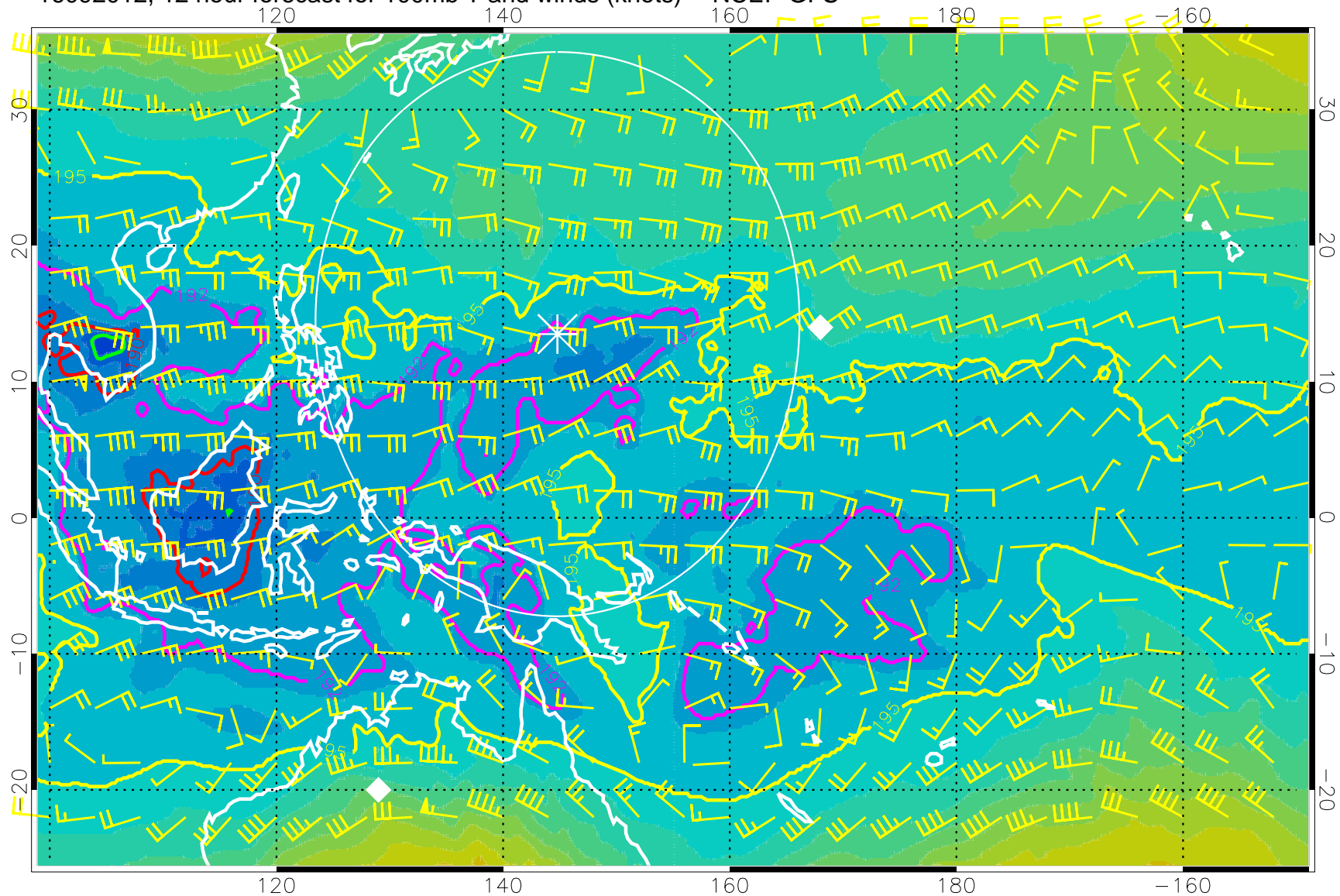
16092012, 12 hour forecast for 100mb T and winds (knots) -- NCEP GFS
