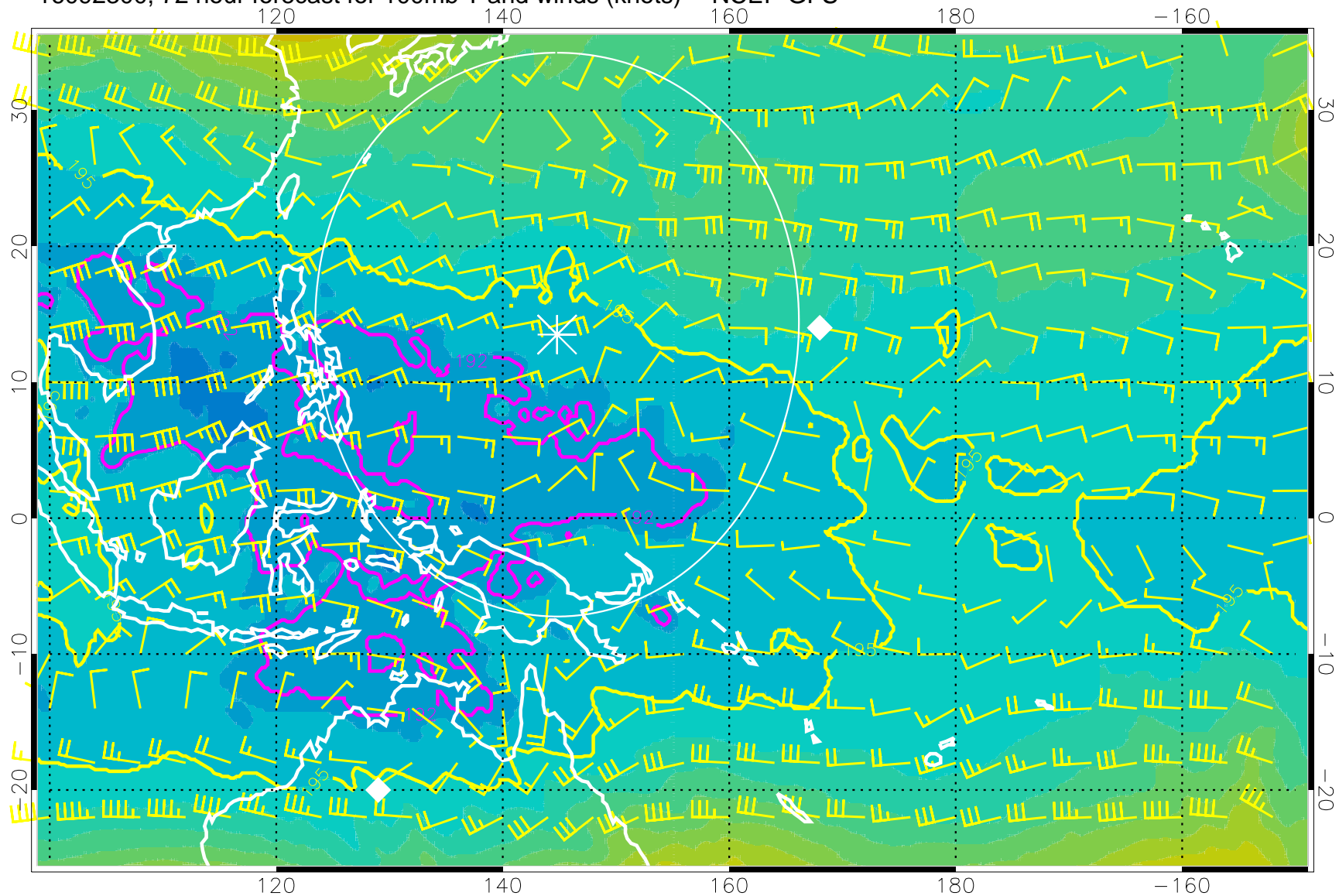
16092300, 72 hour forecast for 100mb T and winds (knots) -- NCEP GFS
