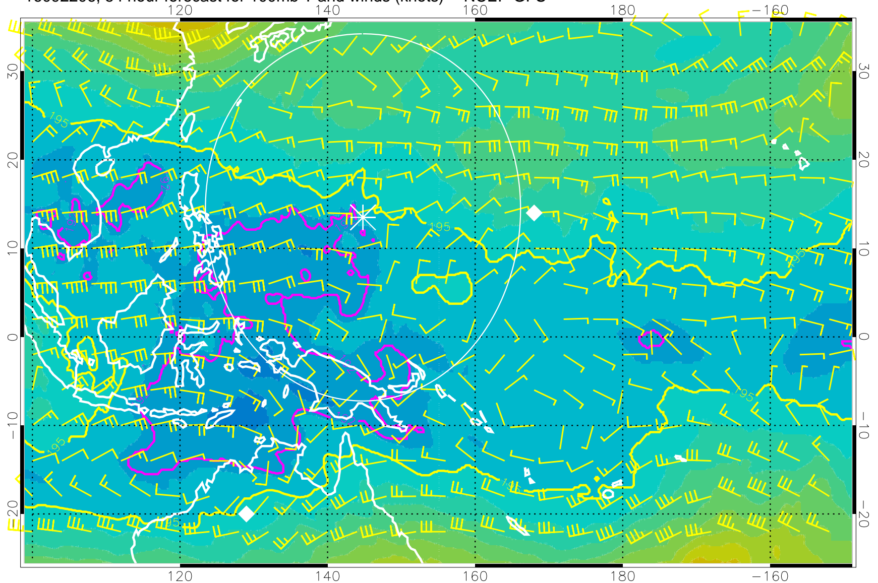
16092206, 54 hour forecast for 100mb T and winds (knots) -- NCEP GFS
