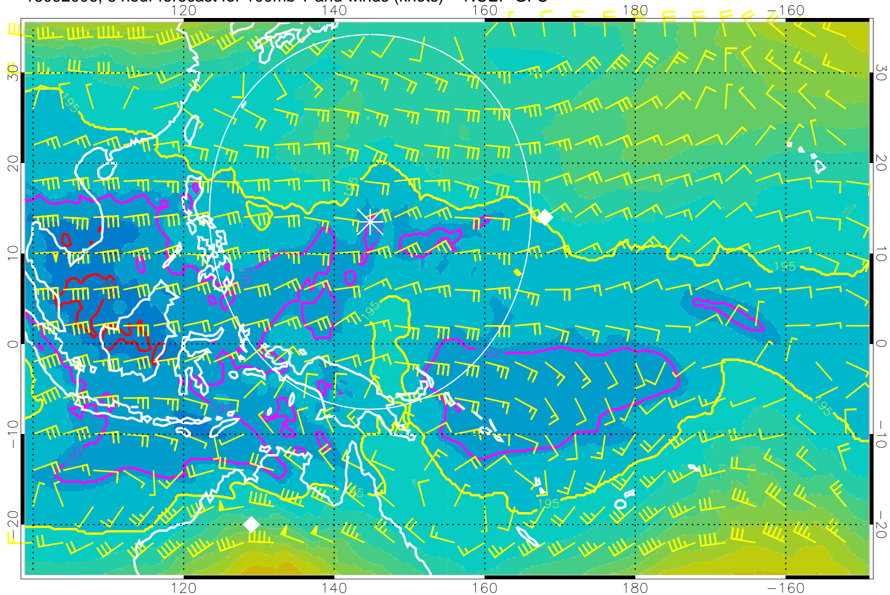
16092006, 6 hour forecast for 100mb T and winds (knots) -- NCEP GFS
