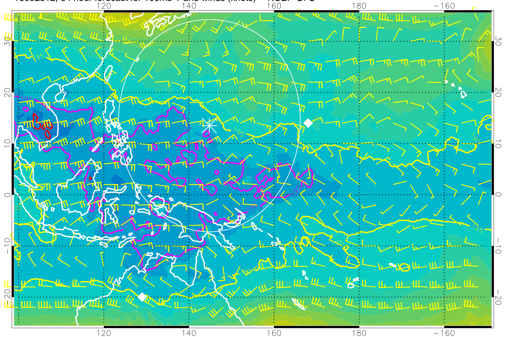
16092312, 84 hour forecast for 100mb T and winds (knots) -- NCEP GFS
