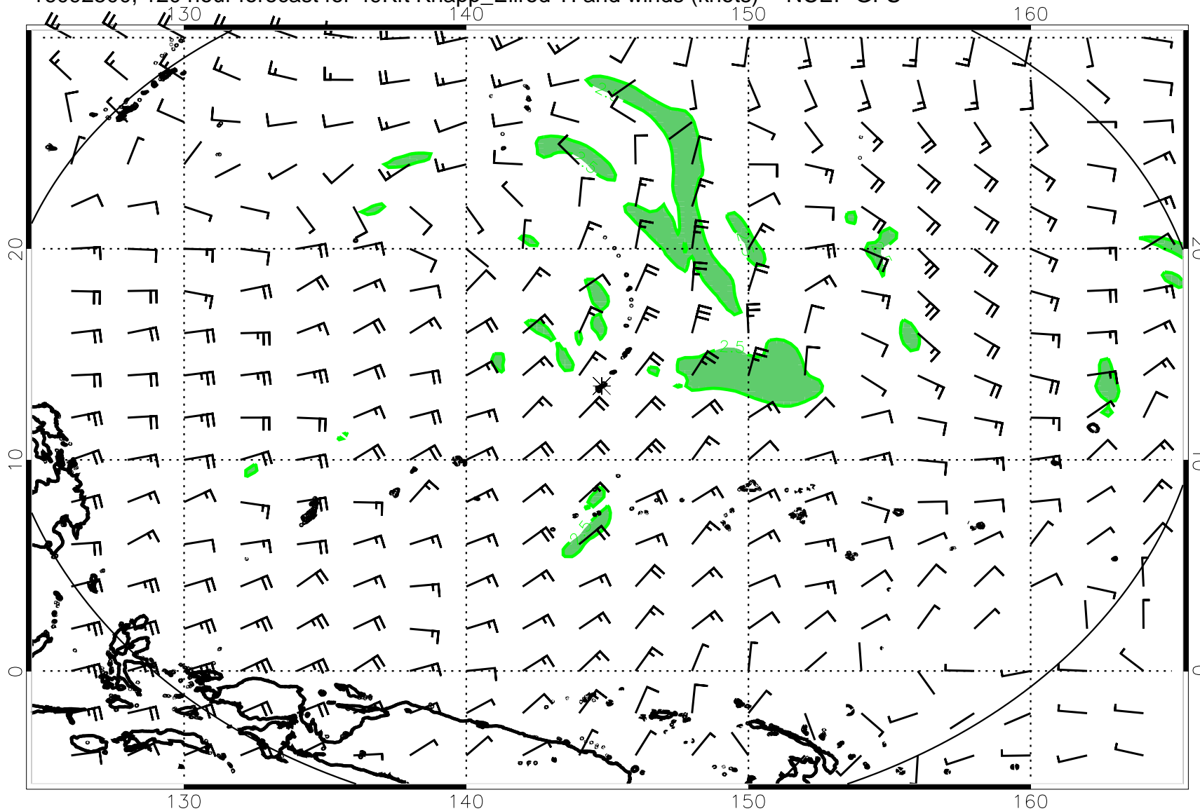
16092500, 120 hour forecast for 49Kft Knapp_Ellrod TI and winds (knots) -- NCEP GFS
