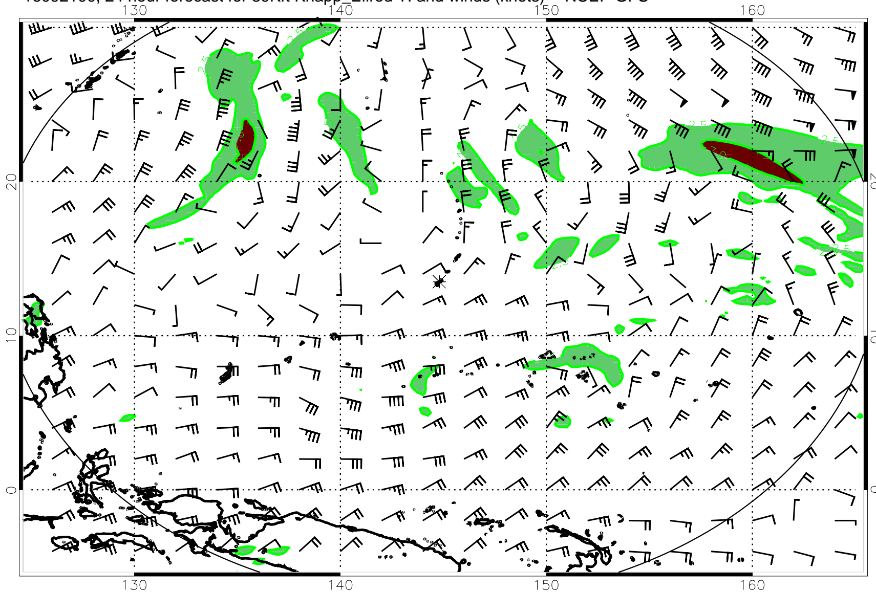
16092100, 24 hour forecast for 39Kft Knapp_Ellrod TI and winds (knots) -- NCEP GFS
