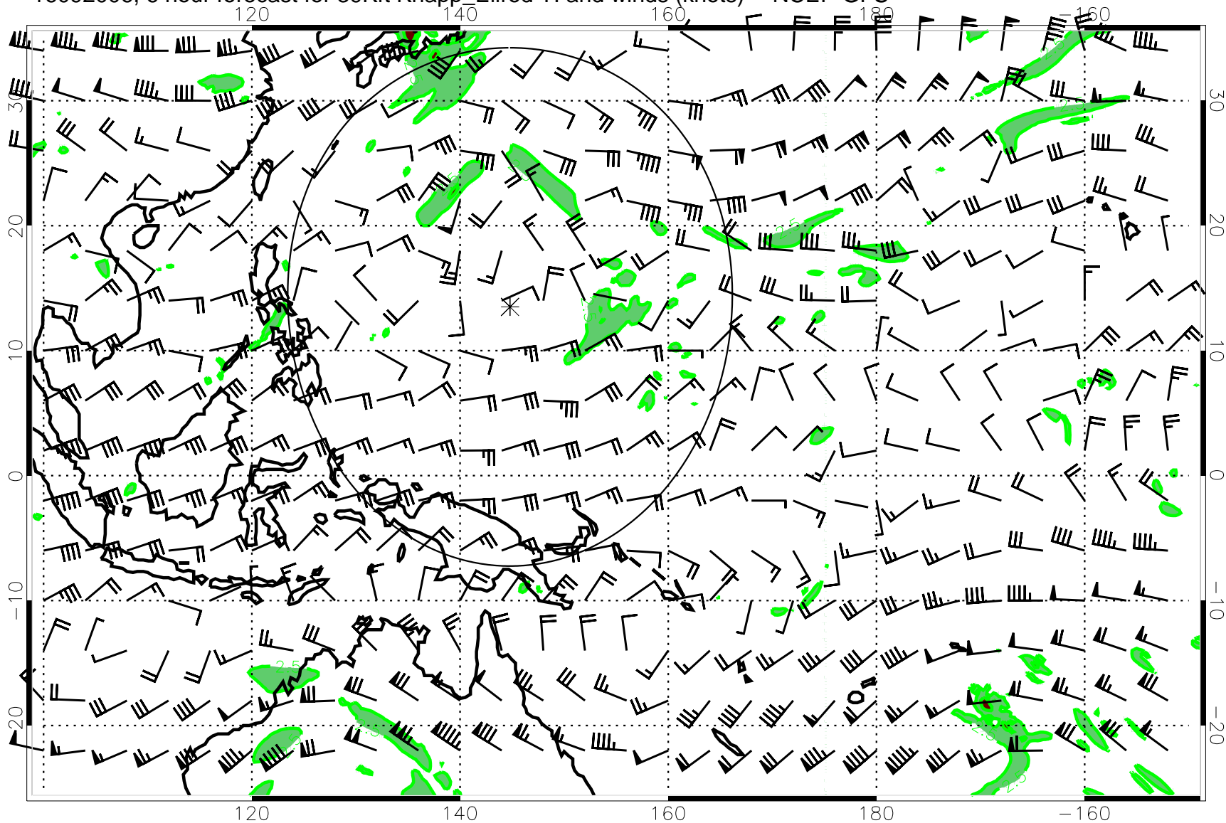
16092006, 6 hour forecast for 39Kft Knapp_Ellrod TI and winds (knots) -- NCEP GFS
