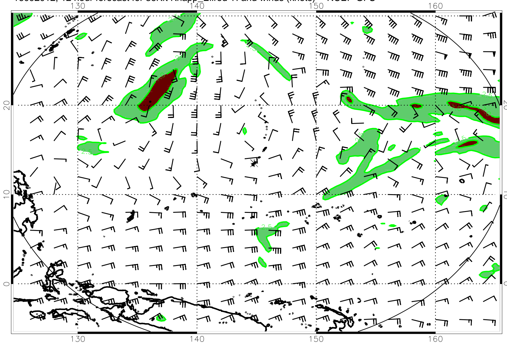
16092012, 12 hour forecast for 36Kft Knapp_Ellrod TI and winds (knots) -- NCEP GFS
