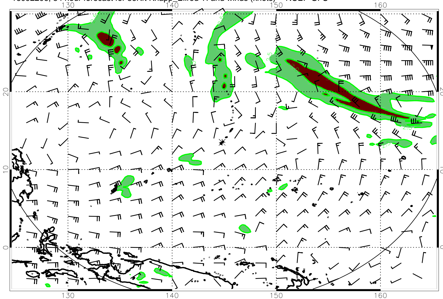
16092206, 54 hour forecast for 36Kft Knapp_Ellrod TI and winds (knots) -- NCEP GFS
