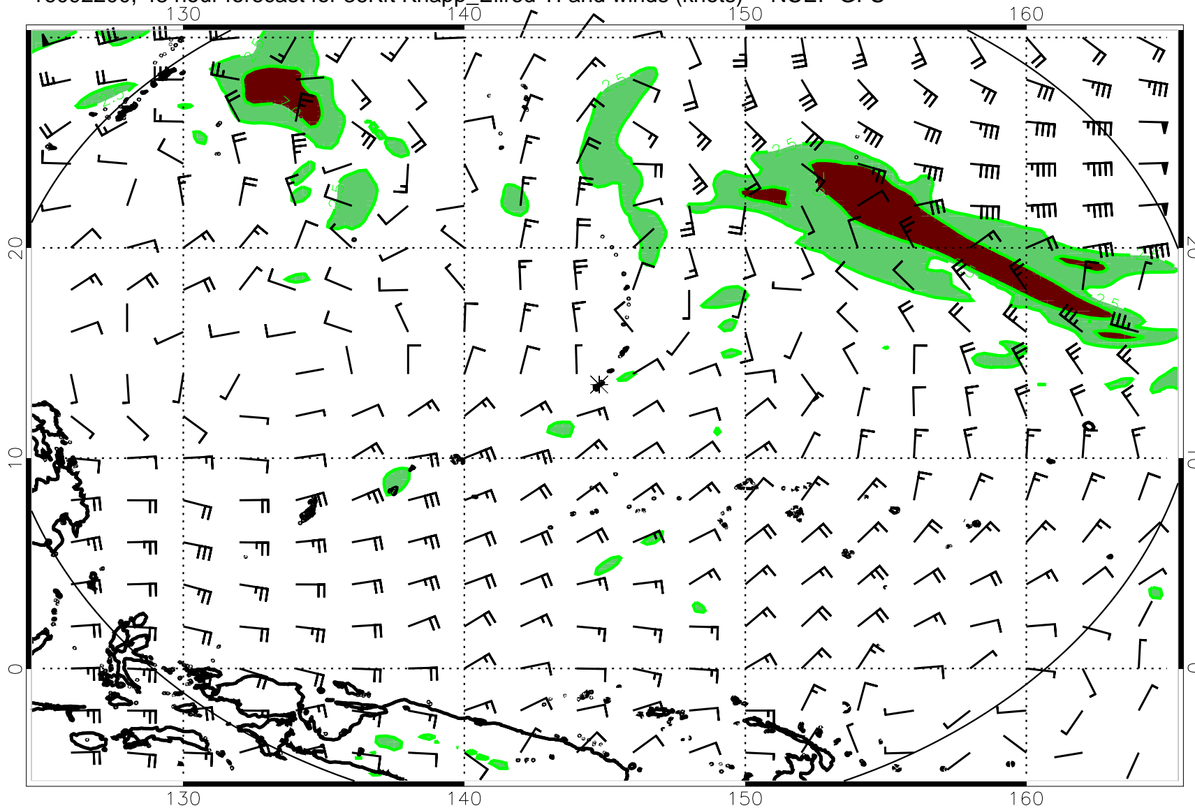
16092200, 48 hour forecast for 36Kft Knapp_Ellrod TI and winds (knots) -- NCEP GFS
