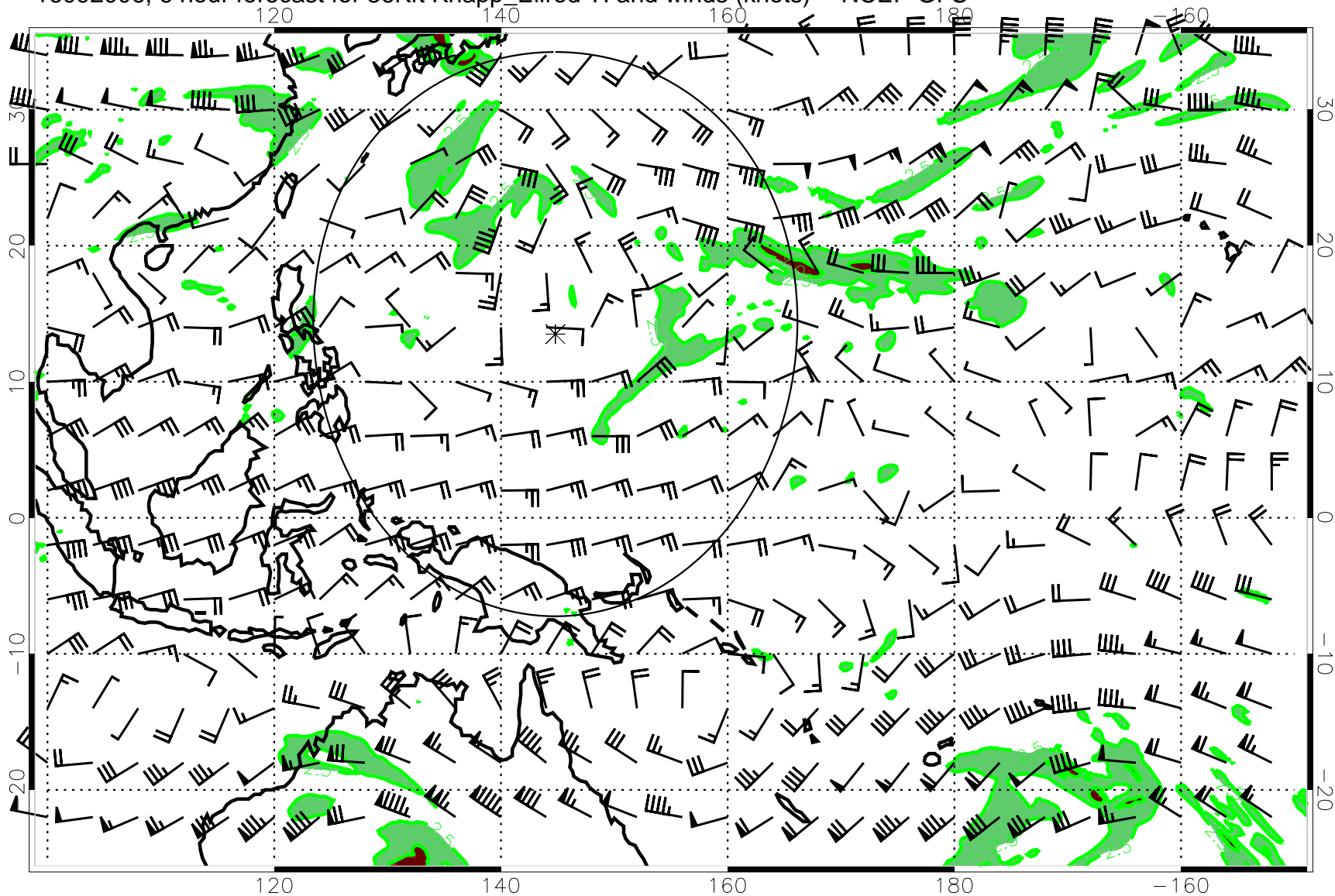
16092006, 6 hour forecast for 36Kft Knapp_Ellrod TI and winds (knots) -- NCEP GFS
