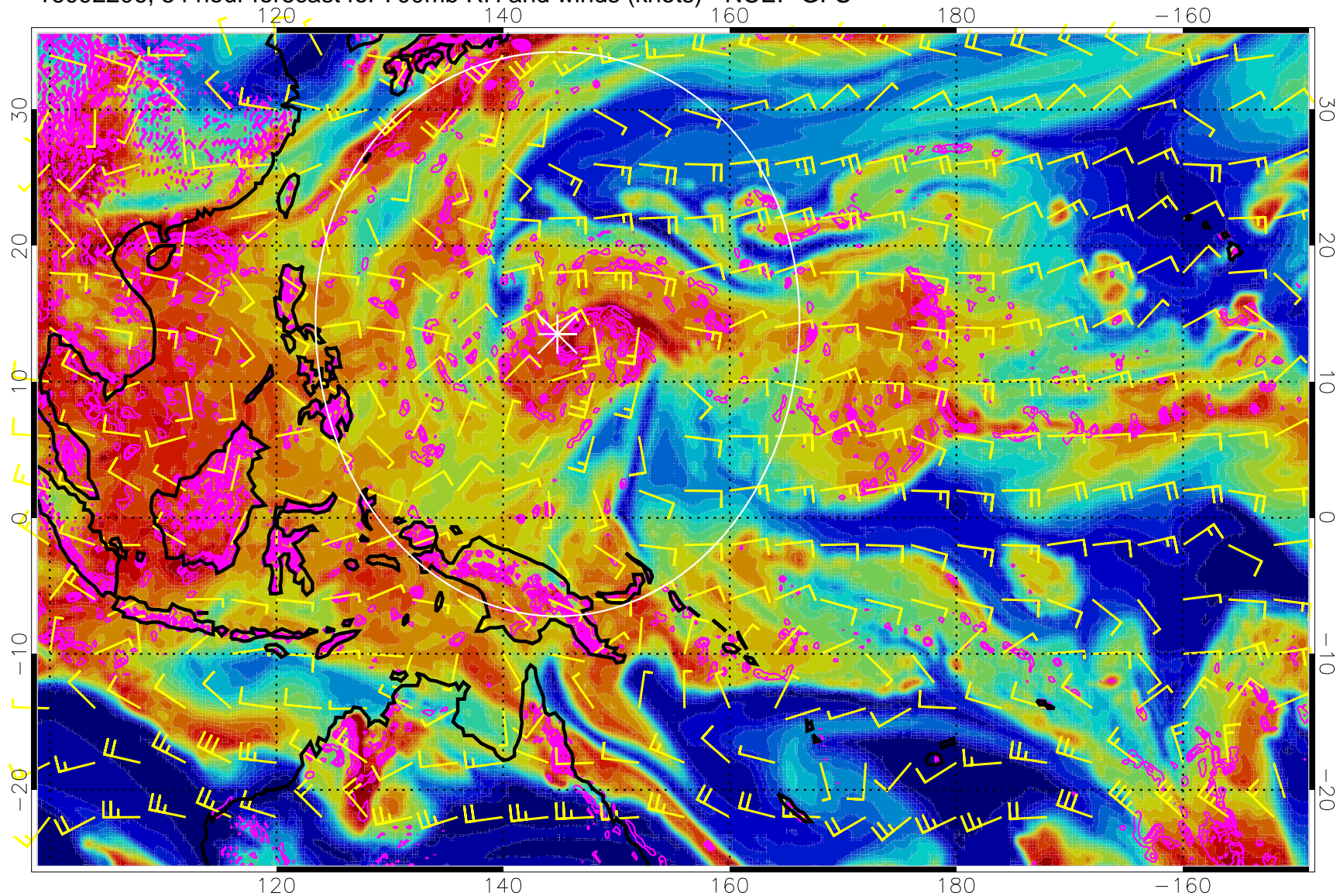
16092206, 54 hour forecast for 700mb RH and winds (knots) - NCEP GFS
