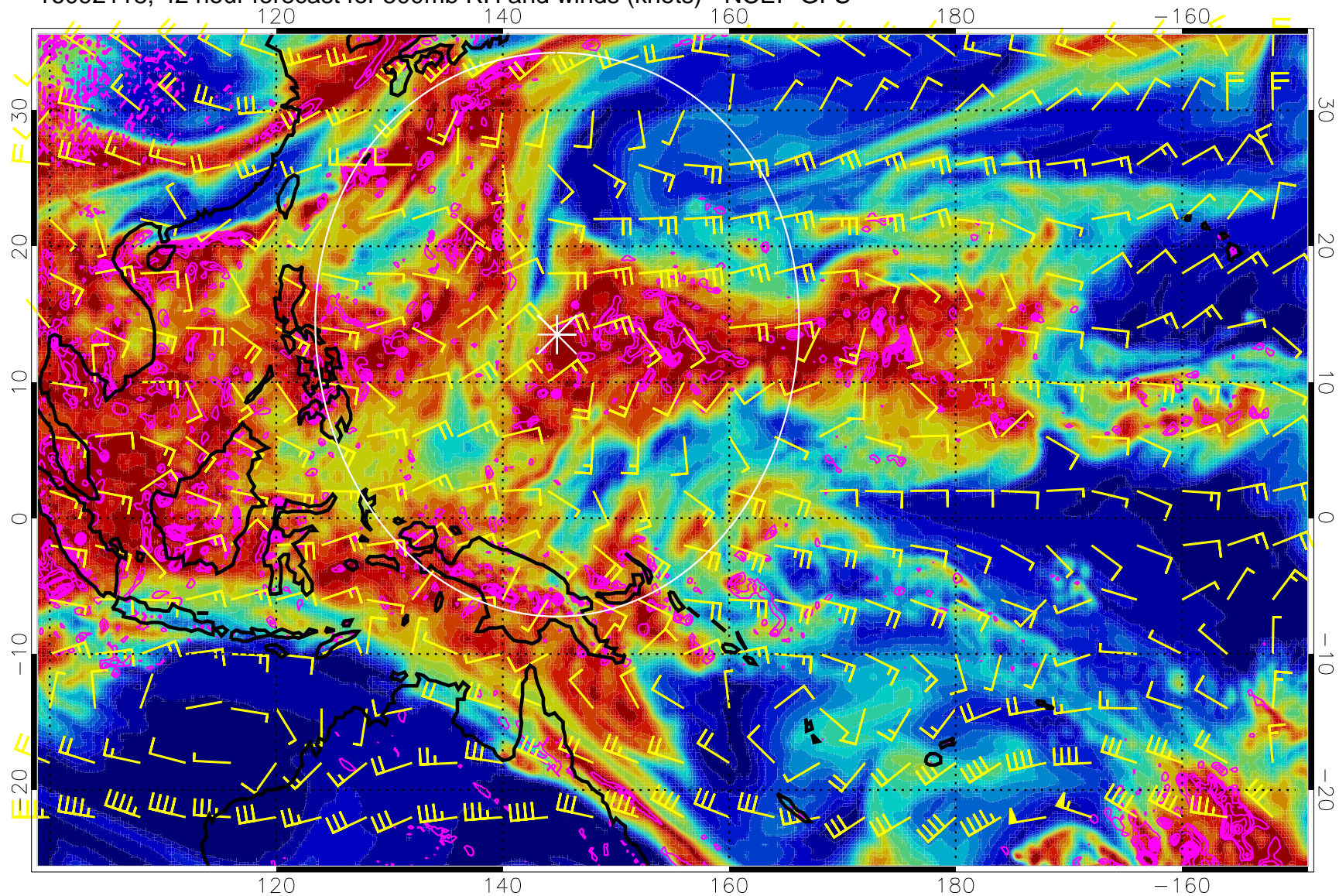
16092118, 42 hour forecast for 500mb RH and winds (knots) - NCEP GFS
