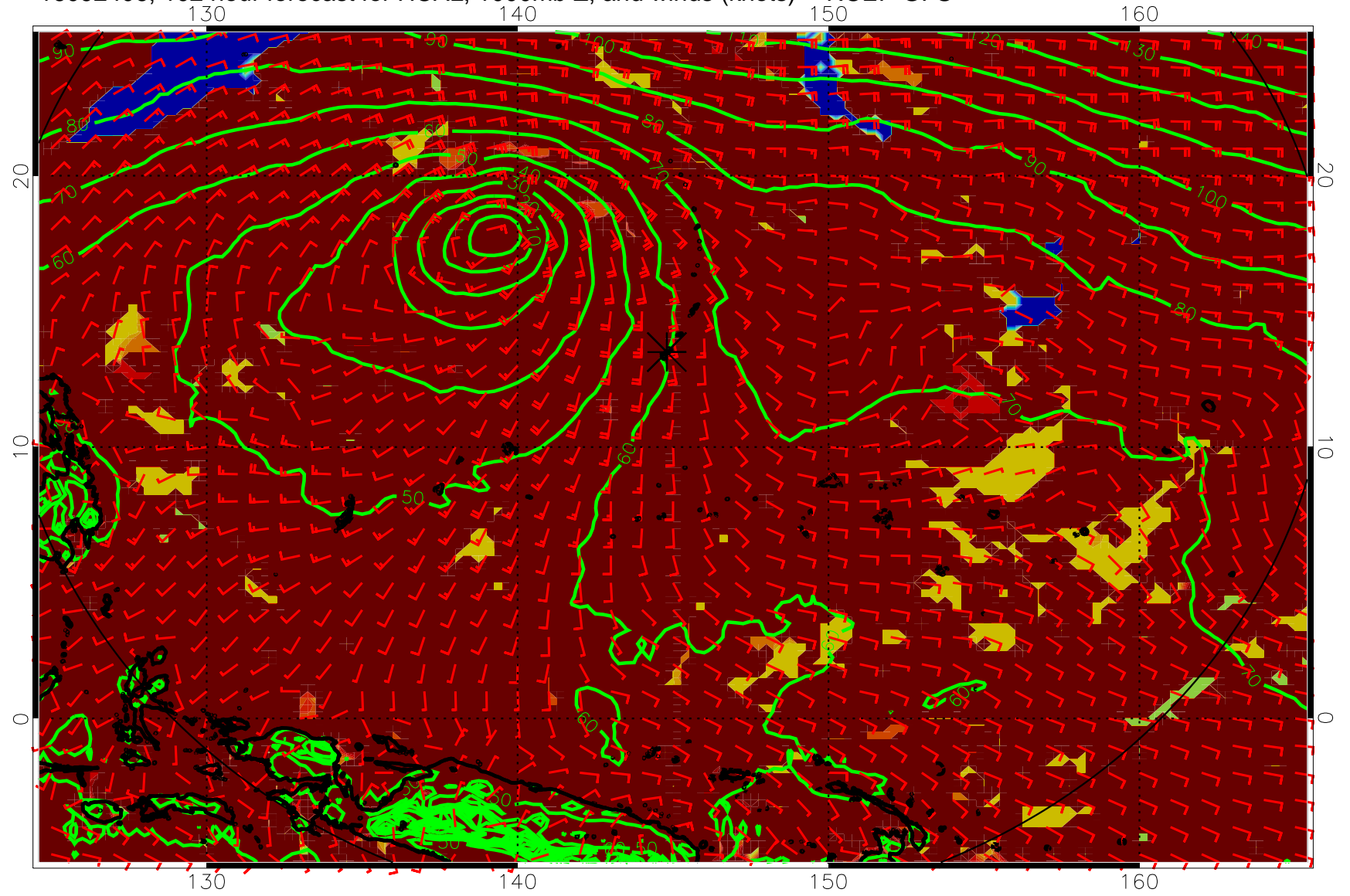
16092406, 102 hour forecast for HCAL, 1000mb Z, and winds (knots) -- NCEP GFS
