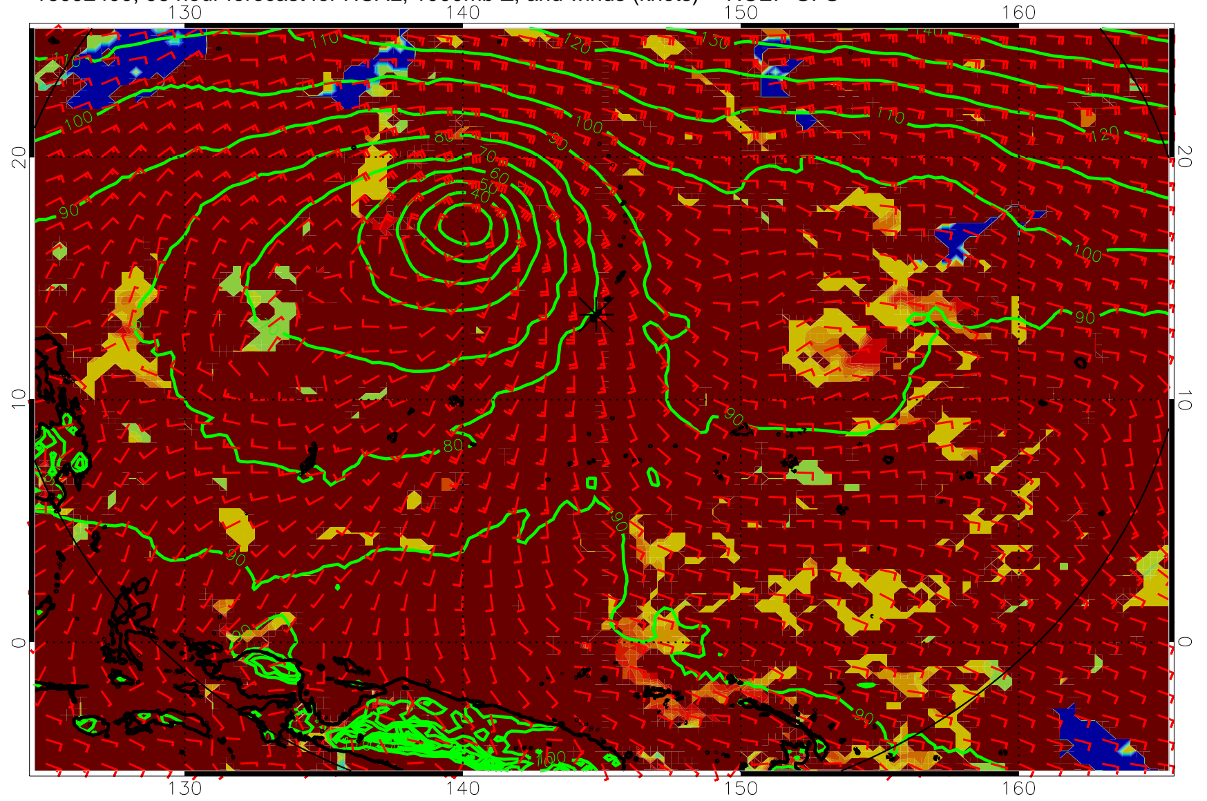
16092400, 96 hour forecast for HCAL, 1000mb Z, and winds (knots) -- NCEP GFS
