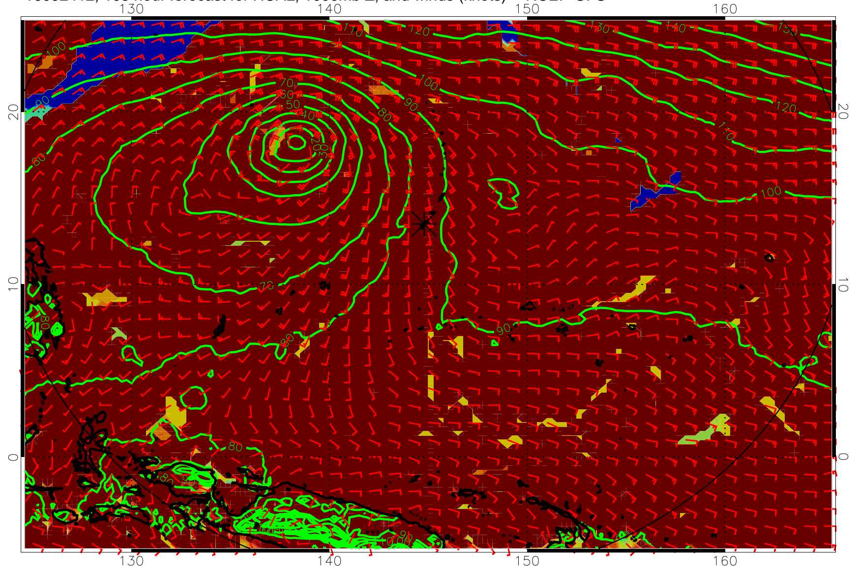
16092412, 108 hour forecast for HCAL, 1000mb Z, and winds (knots) -- NCEP GFS
