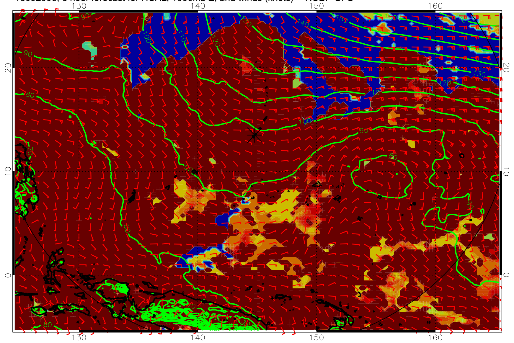
16092006, 6 hour forecast for HCAL, 1000mb Z, and winds (knots) -- NCEP GFS
