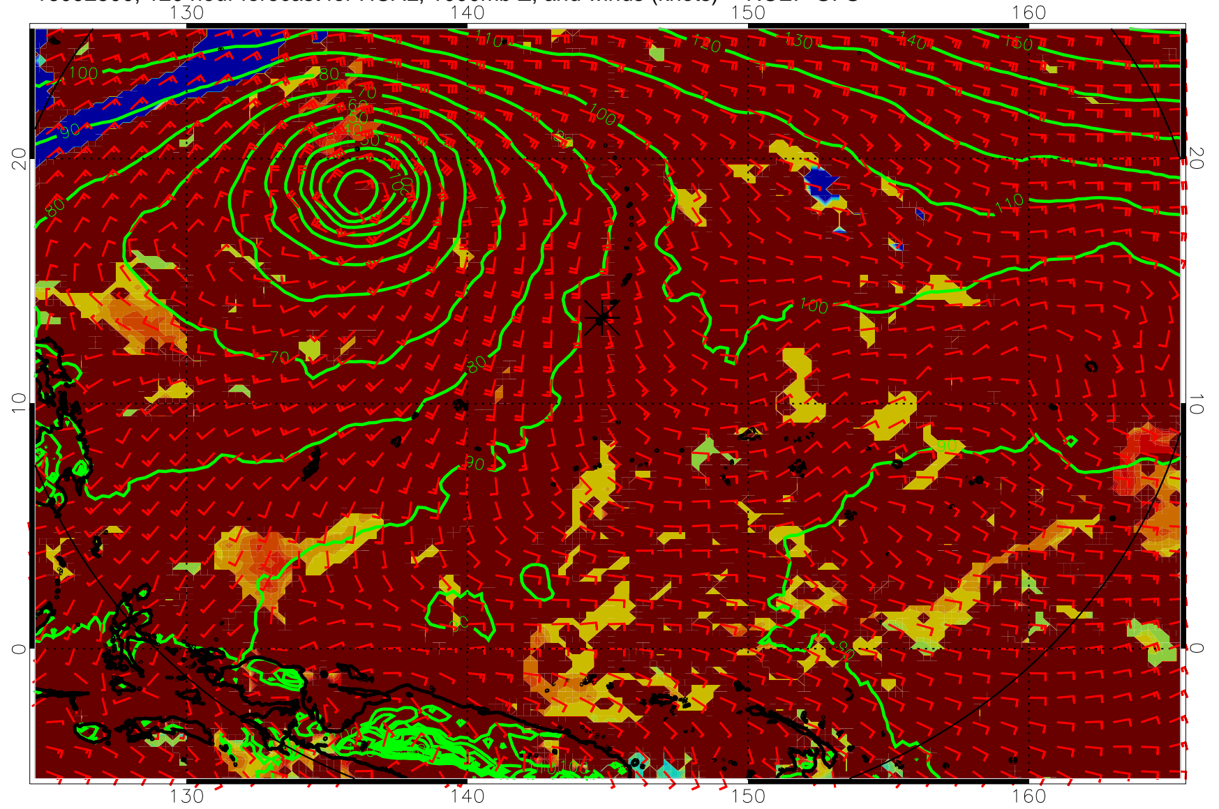
16092500, 120 hour forecast for HCAL, 1000mb Z, and winds (knots) -- NCEP GFS
