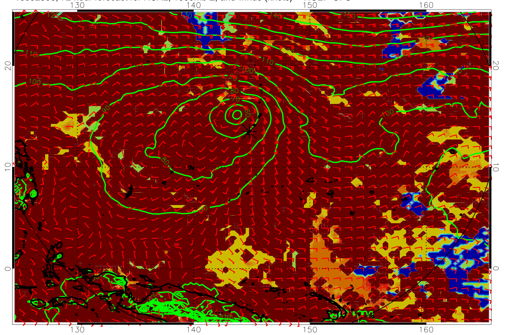
16092300, 72 hour forecast for HCAL, 1000mb Z, and winds (knots) -- NCEP GFS
