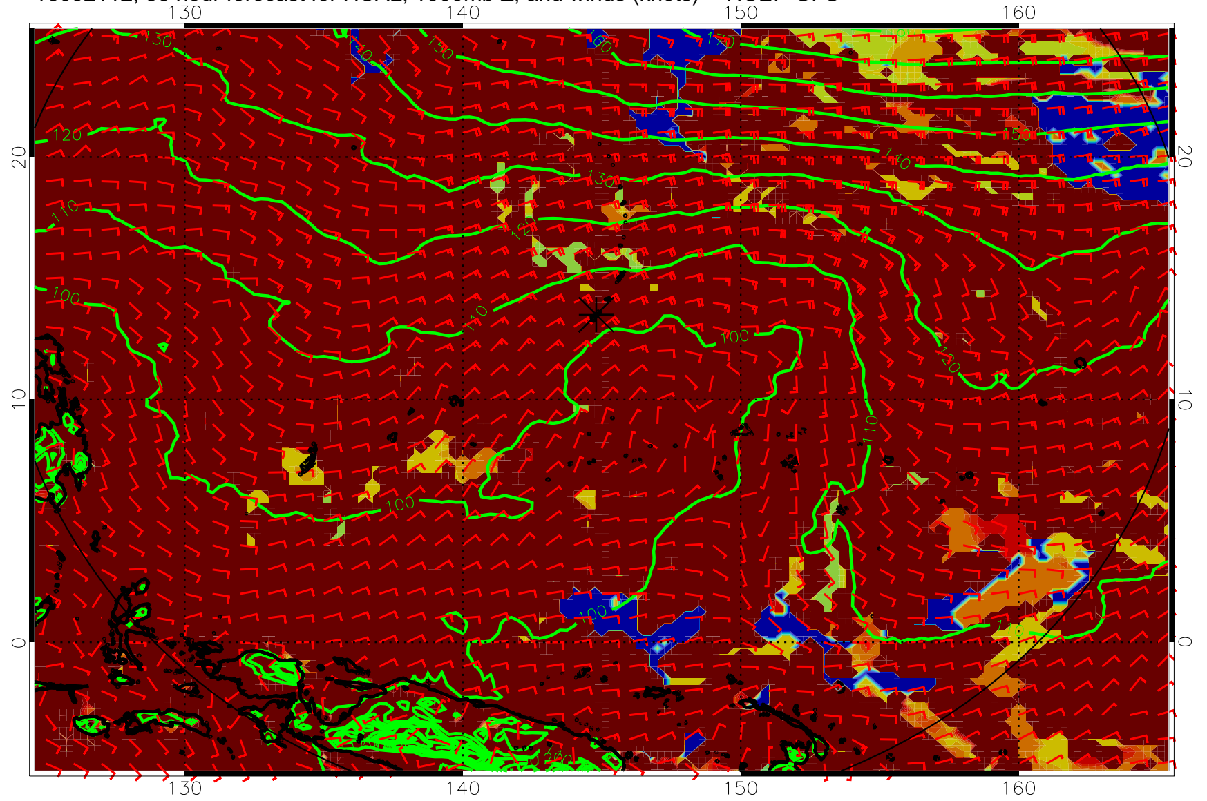
16092112, 36 hour forecast for HCAL, 1000mb Z, and winds (knots) -- NCEP GFS
