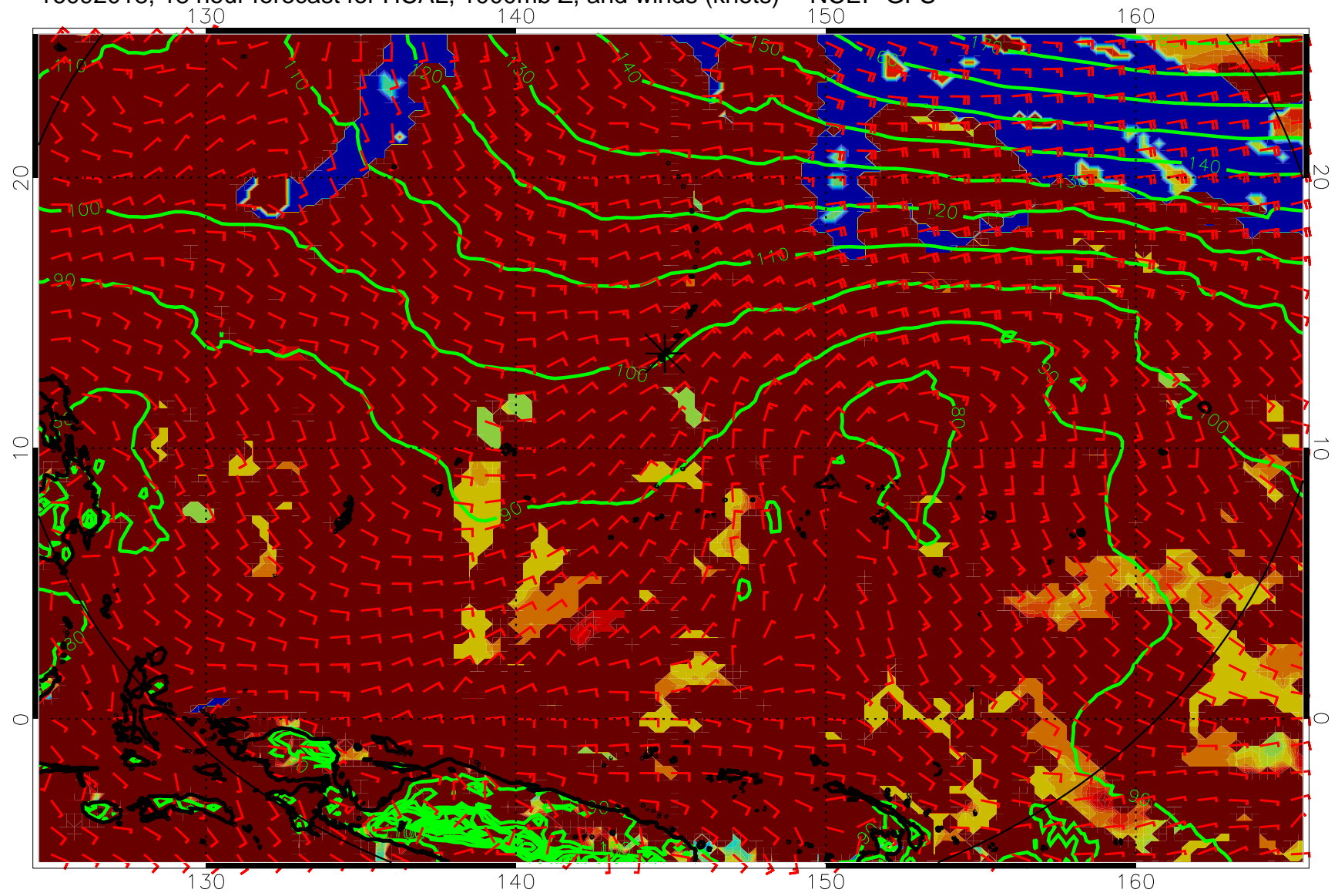
16092018, 18 hour forecast for HCAL, 1000mb Z, and winds (knots) -- NCEP GFS
