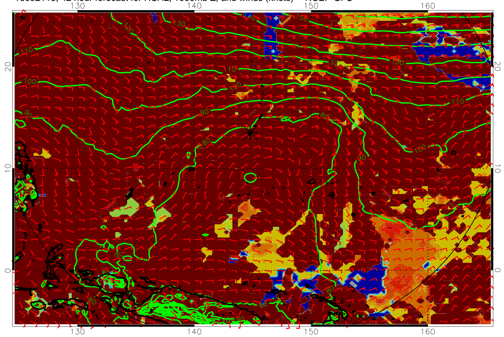
16092118, 42 hour forecast for HCAL, 1000mb Z, and winds (knots) -- NCEP GFS
