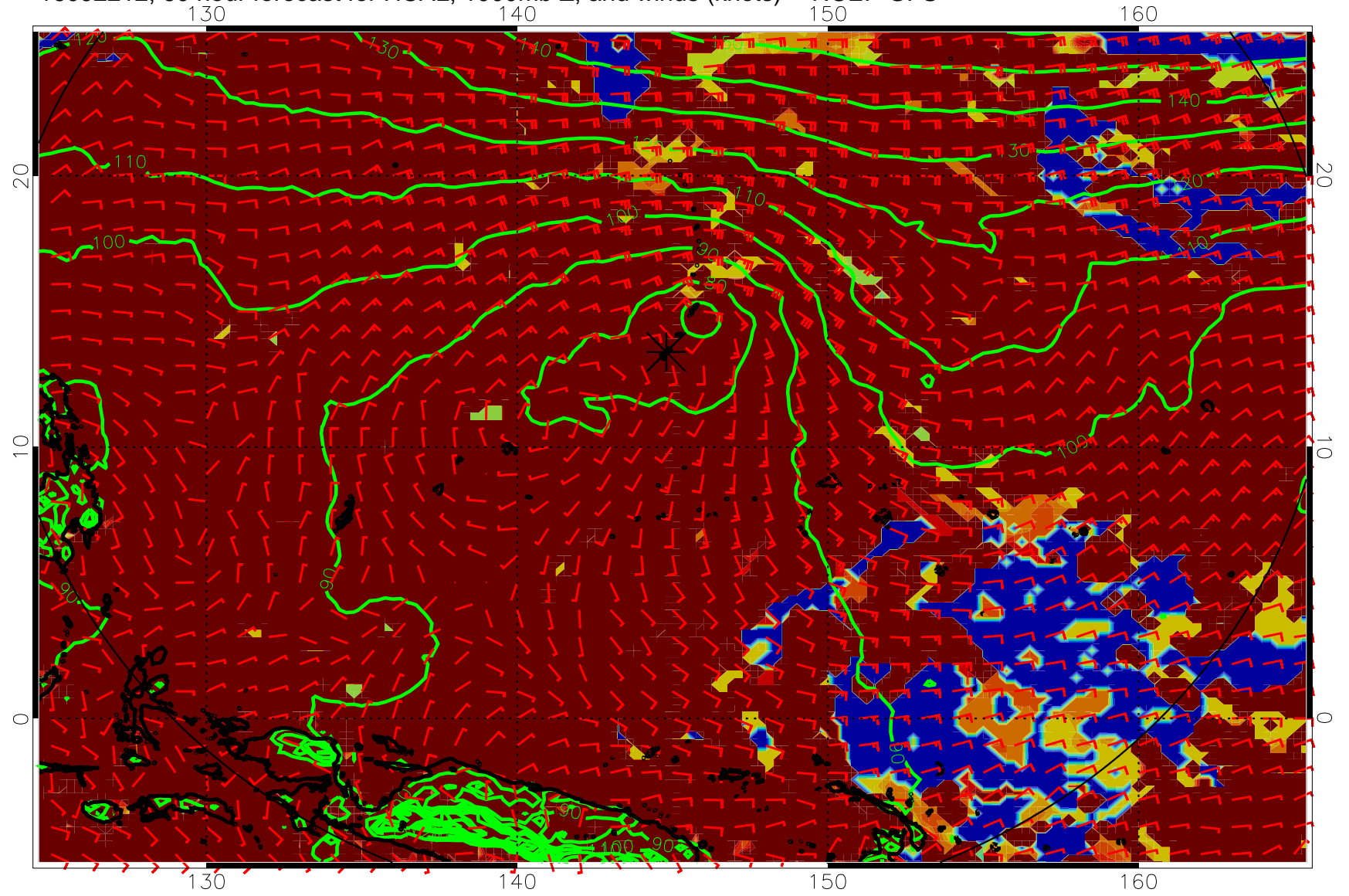
16092212, 60 hour forecast for HCAL, 1000mb Z, and winds (knots) -- NCEP GFS
