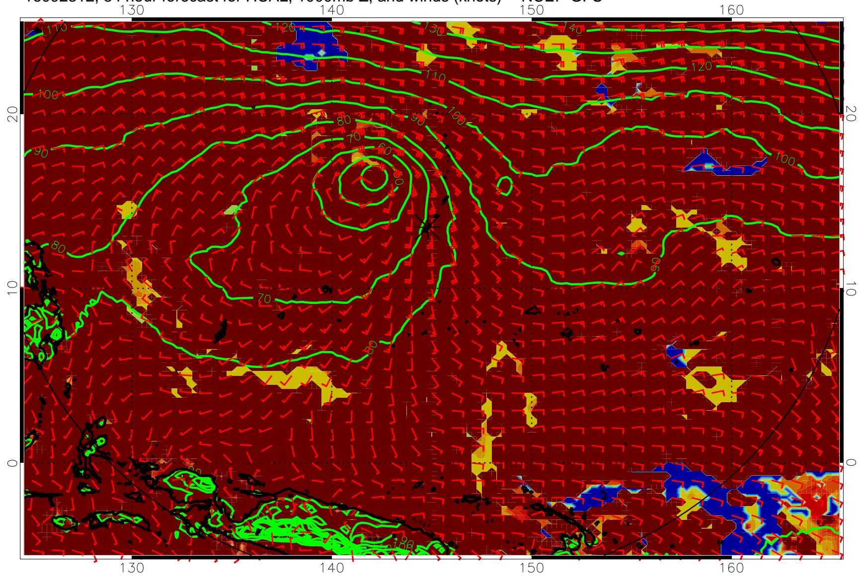
16092312, 84 hour forecast for HCAL, 1000mb Z, and winds (knots) -- NCEP GFS
