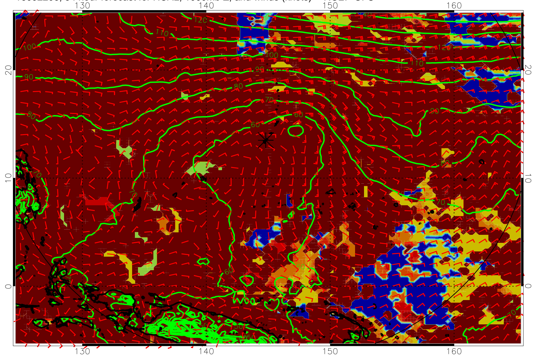
16092206, 54 hour forecast for HCAL, 1000mb Z, and winds (knots) -- NCEP GFS
