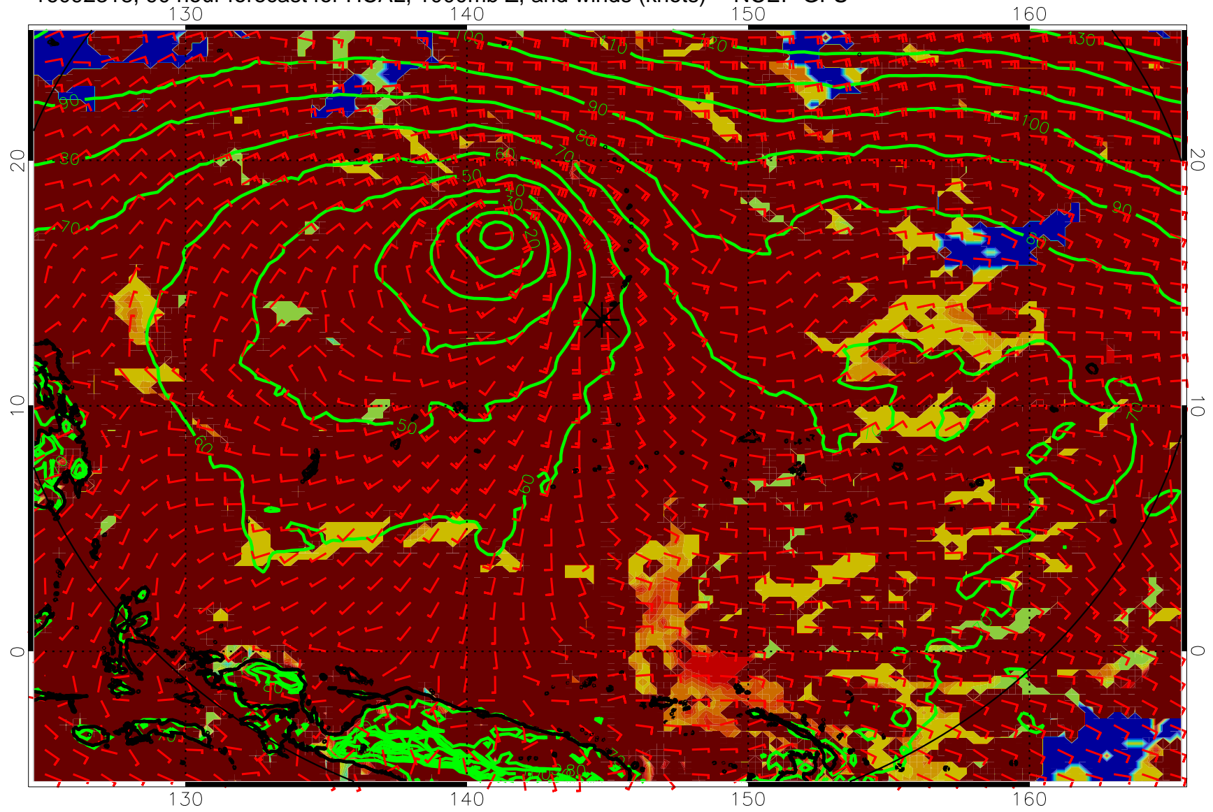
16092318, 90 hour forecast for HCAL, 1000mb Z, and winds (knots) -- NCEP GFS
