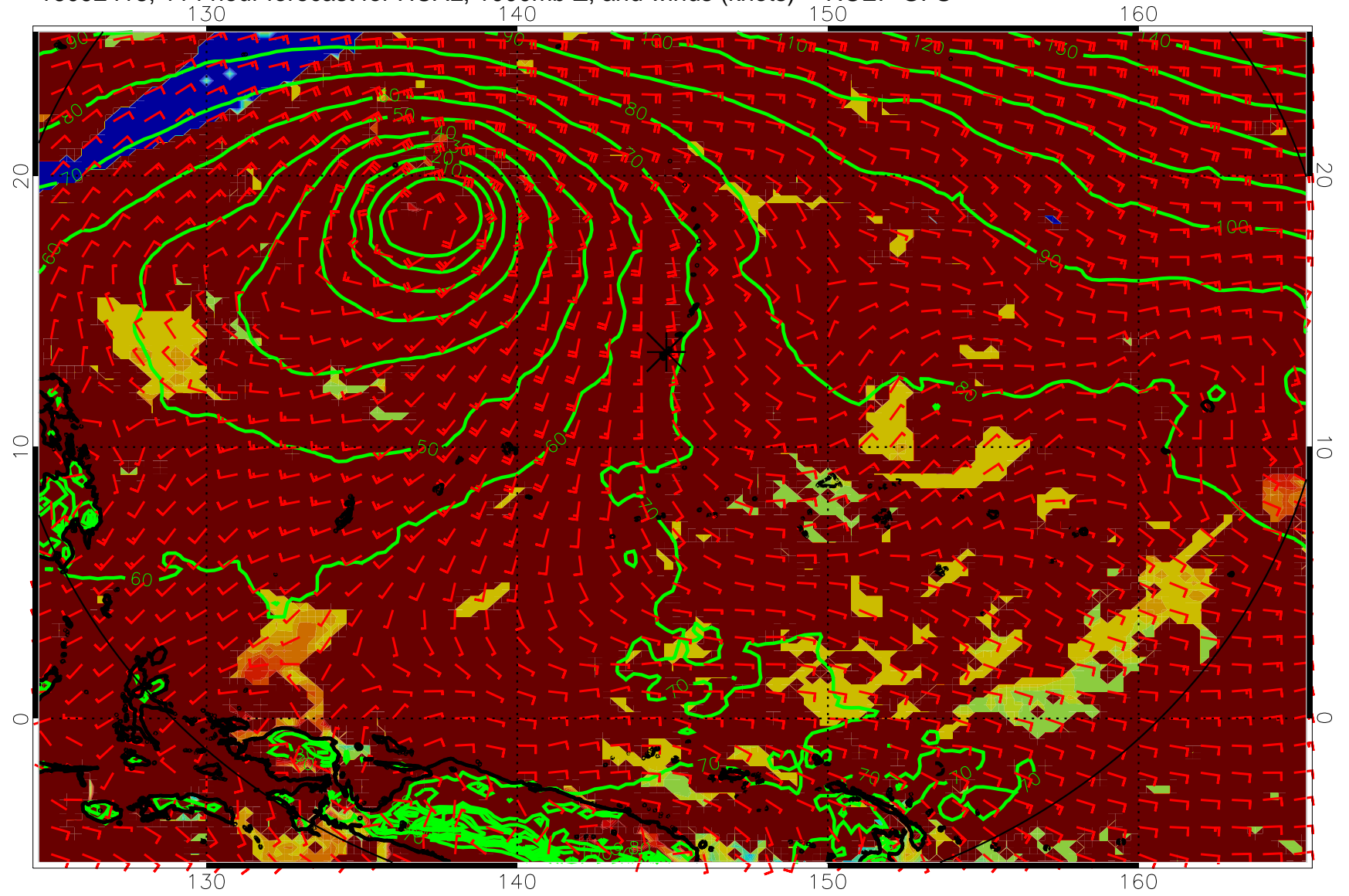
16092418, 114 hour forecast for HCAL, 1000mb Z, and winds (knots) -- NCEP GFS
