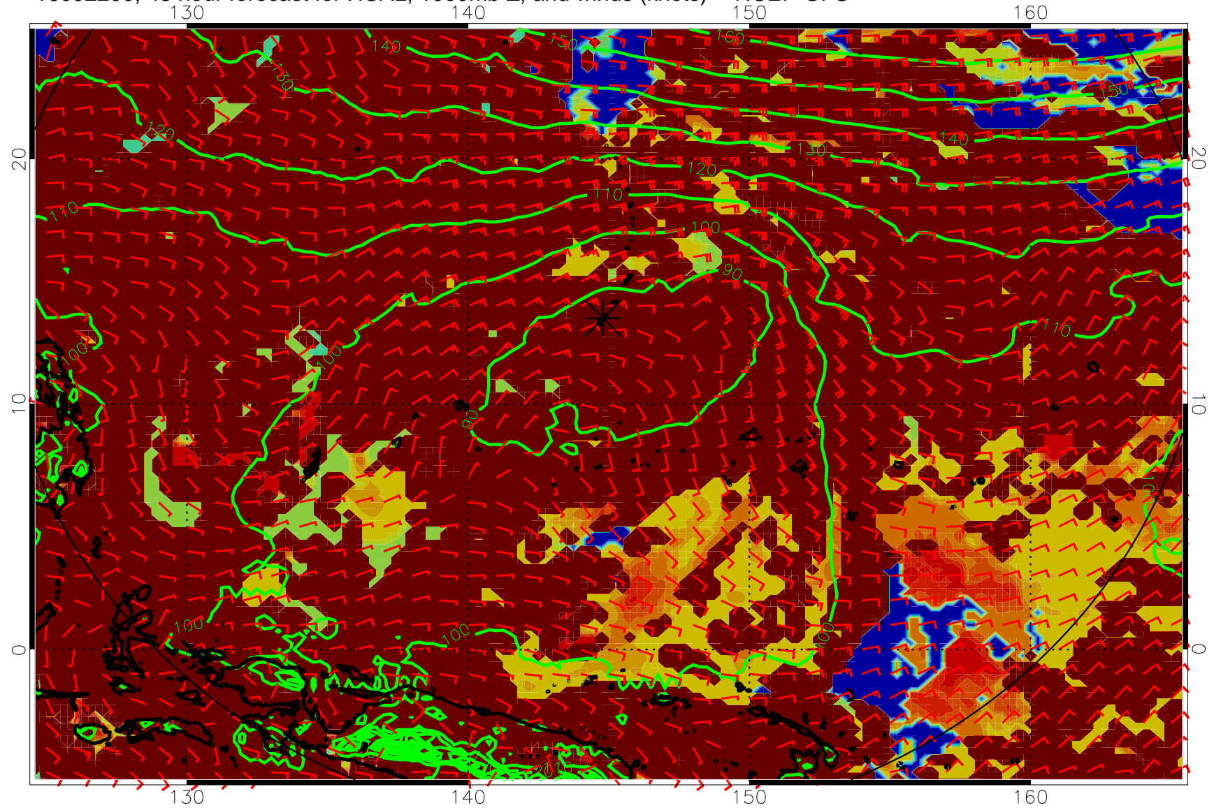
16092200, 48 hour forecast for HCAL, 1000mb Z, and winds (knots) -- NCEP GFS
