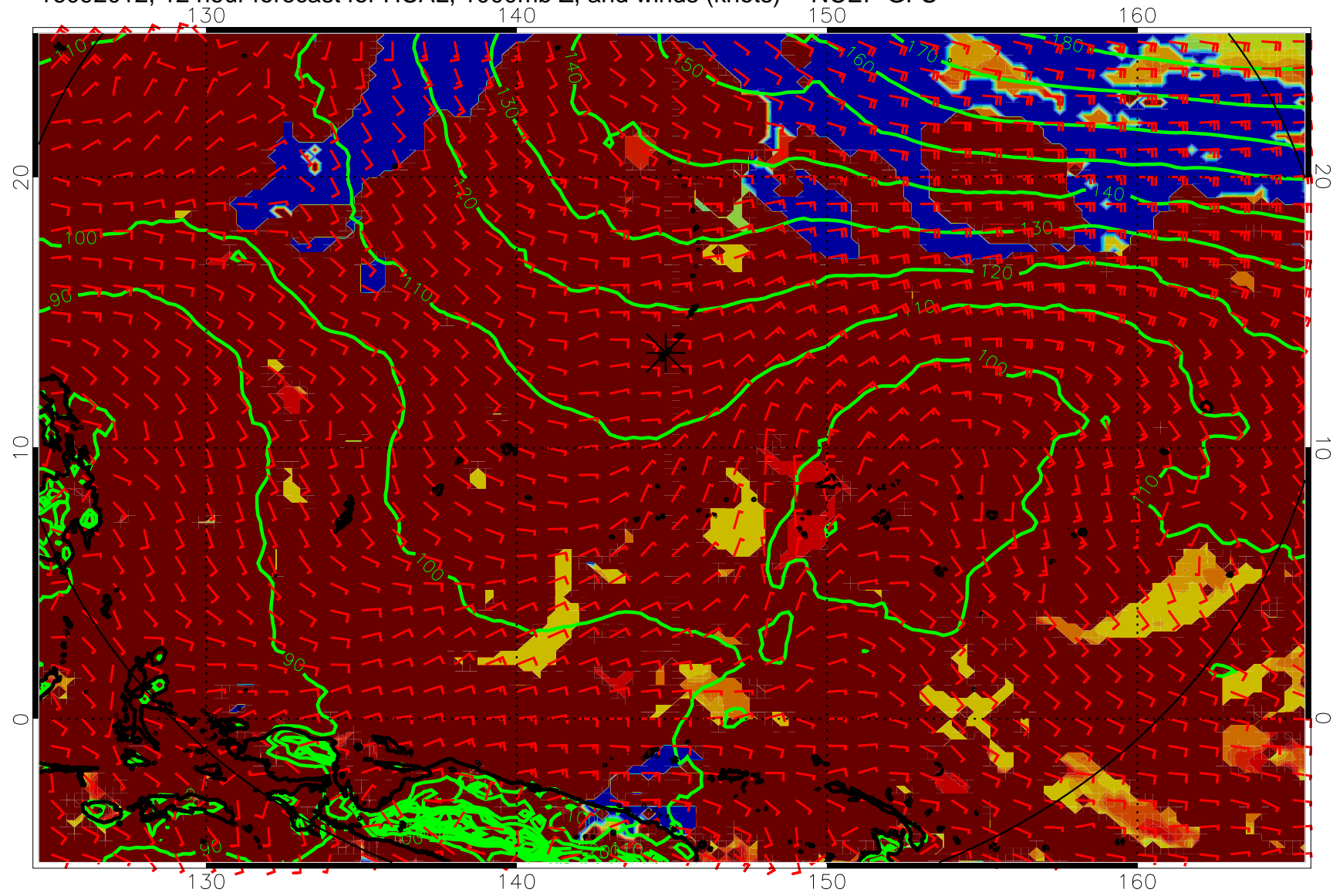
16092012, 12 hour forecast for HCAL, 1000mb Z, and winds (knots) -- NCEP GFS
