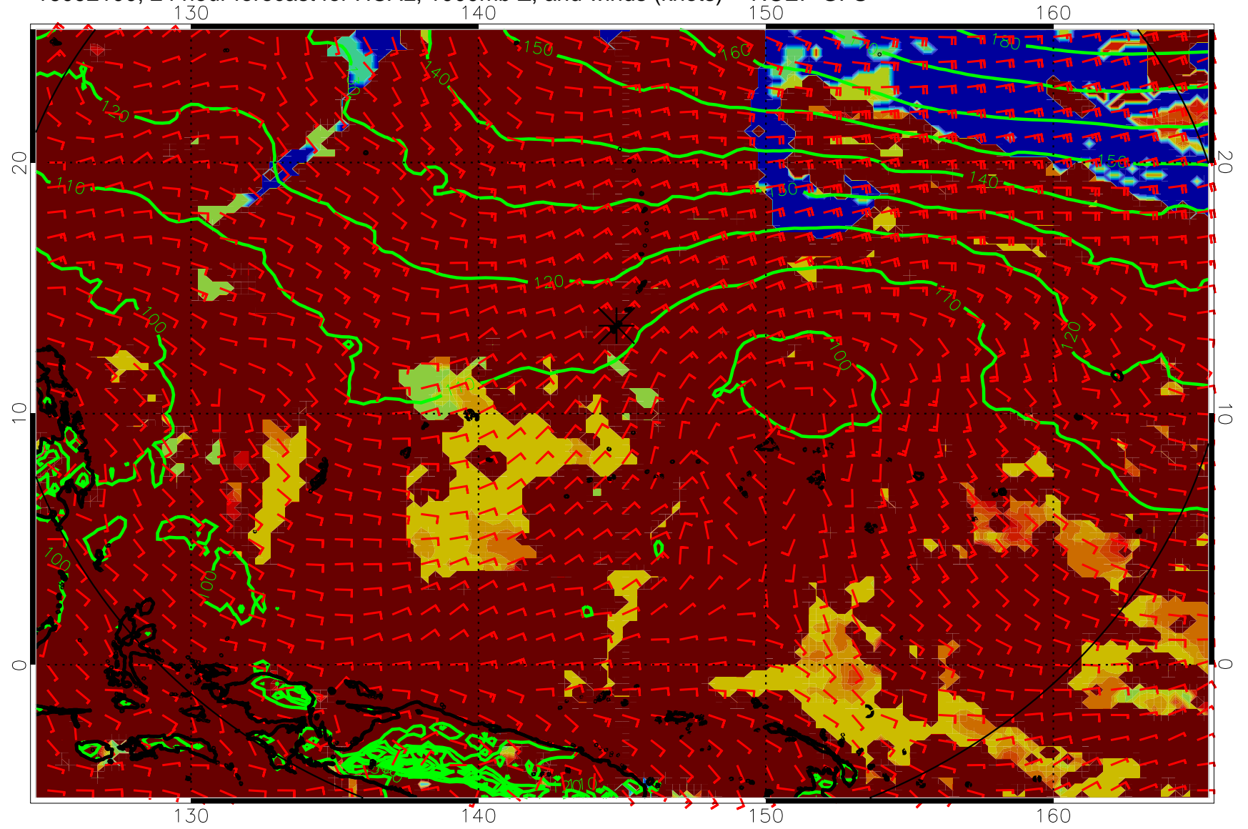
16092100, 24 hour forecast for HCAL, 1000mb Z, and winds (knots) -- NCEP GFS
