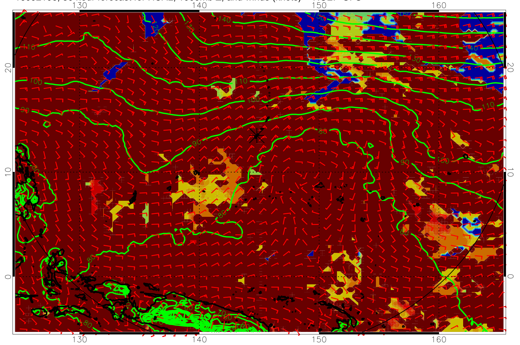
16092106, 30 hour forecast for HCAL, 1000mb Z, and winds (knots) -- NCEP GFS
