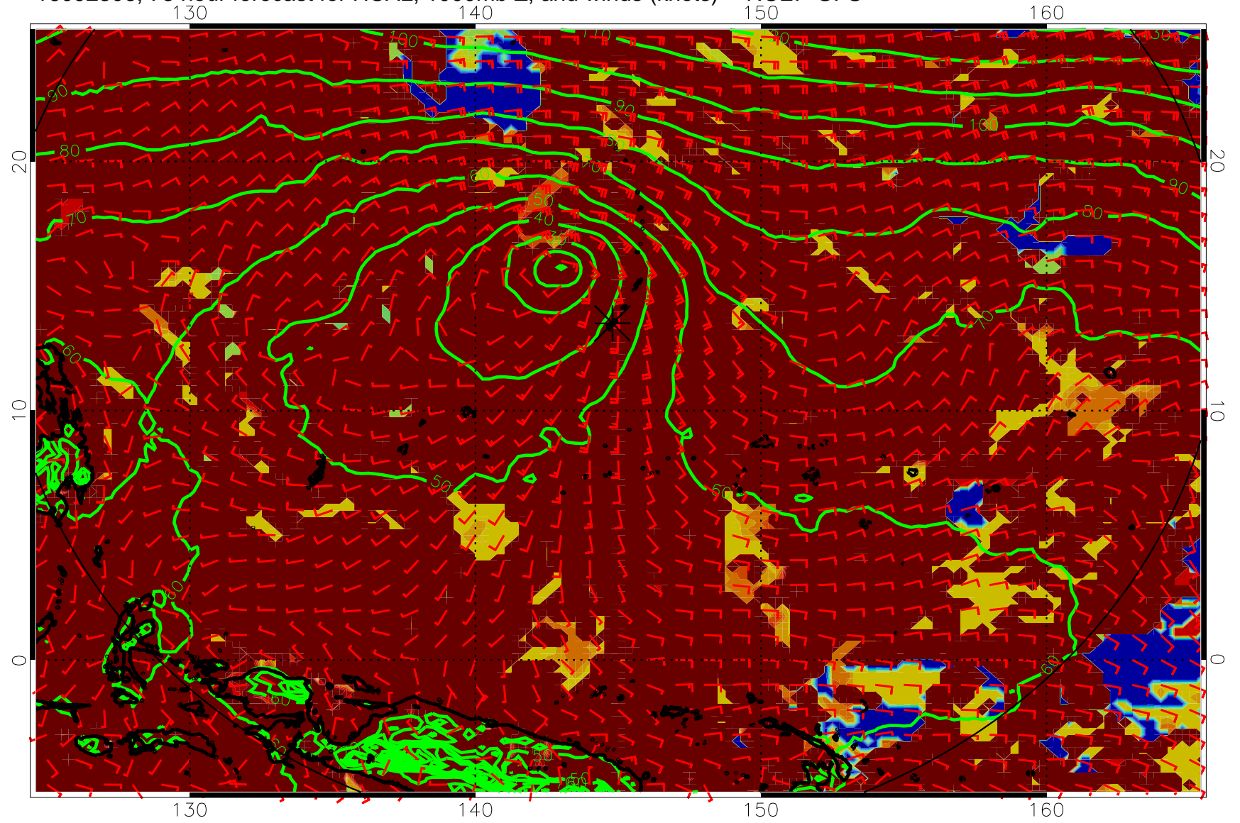
16092306, 78 hour forecast for HCAL, 1000mb Z, and winds (knots) -- NCEP GFS
