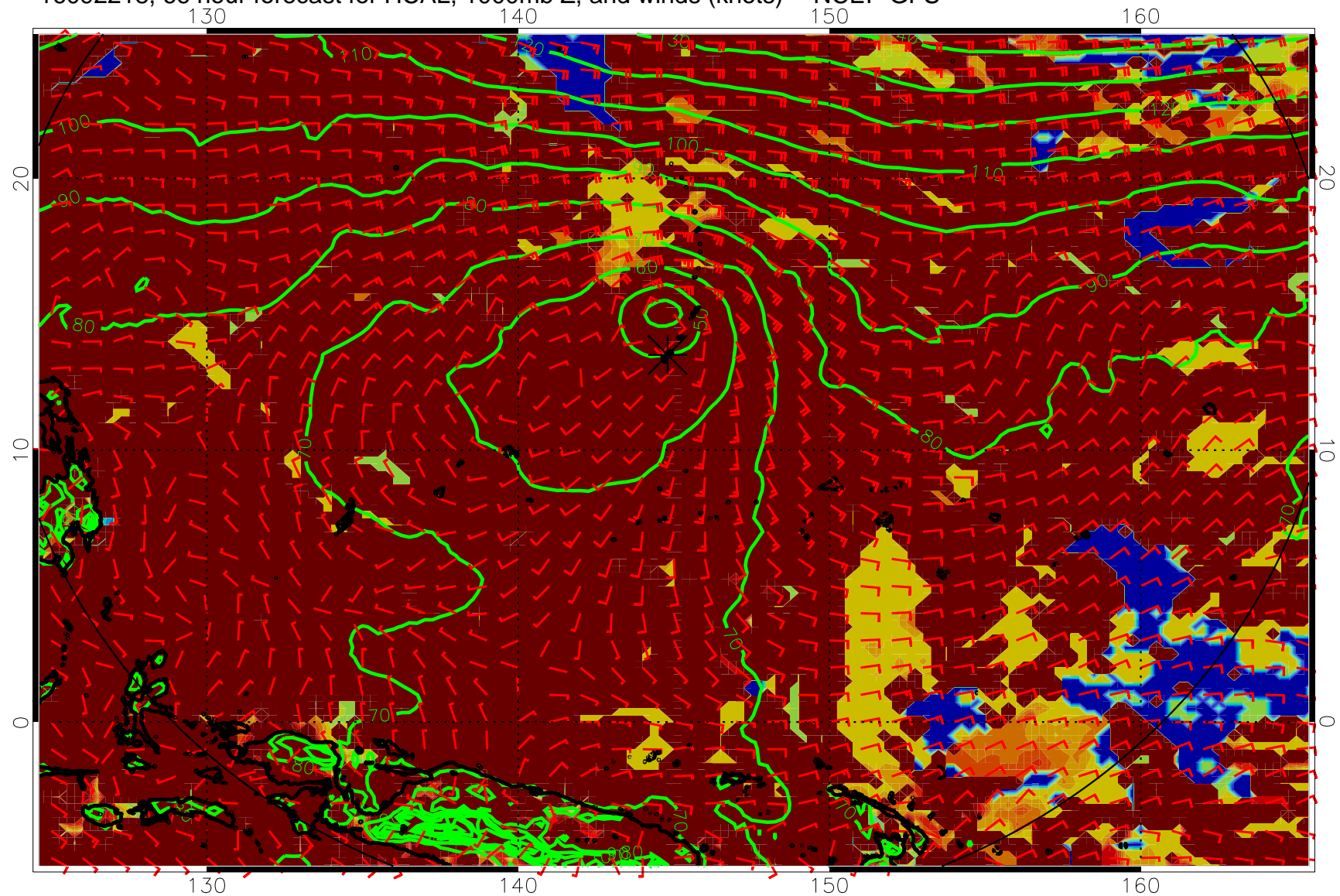
16092218, 66 hour forecast for HCAL, 1000mb Z, and winds (knots) -- NCEP GFS
