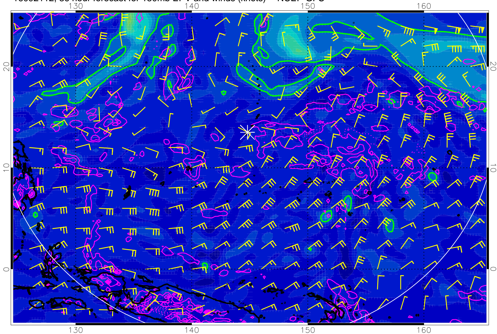
16092112, 36 hour forecast for 150mb EPV and winds (knots) -- NCEP GFS
