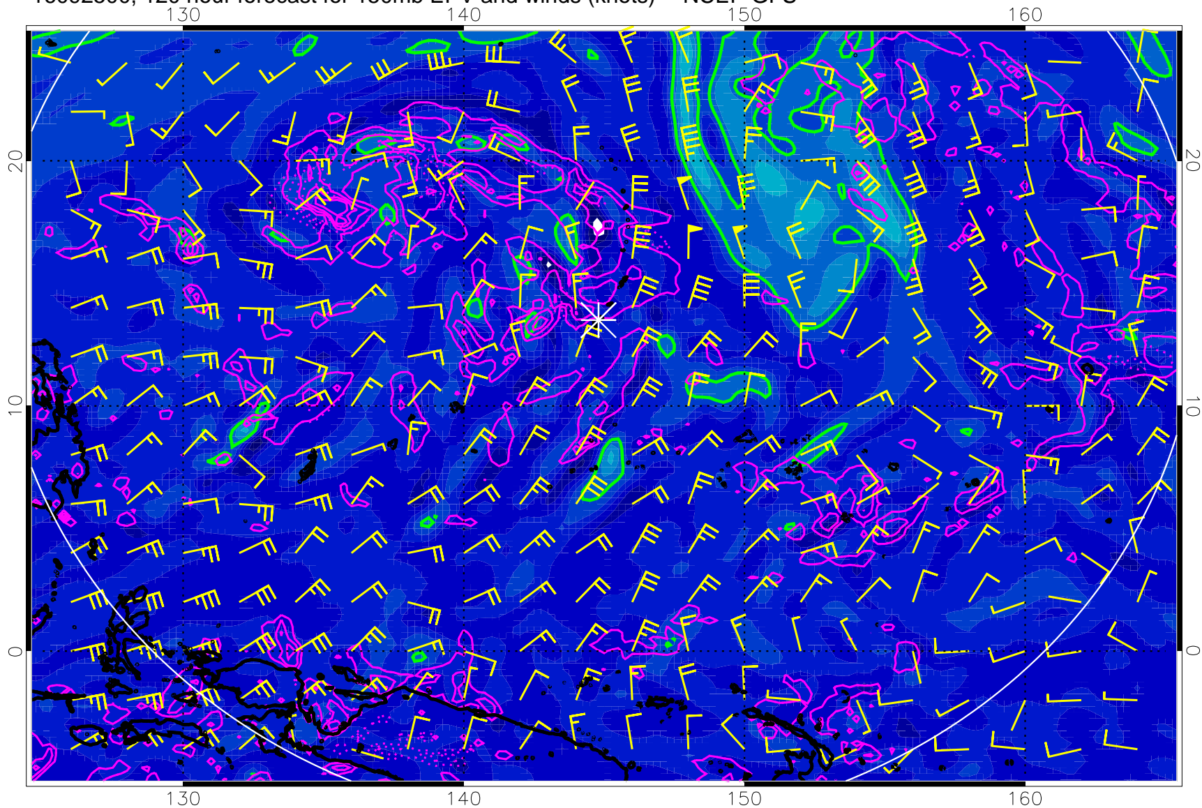
16092500, 120 hour forecast for 150mb EPV and winds (knots) -- NCEP GFS
