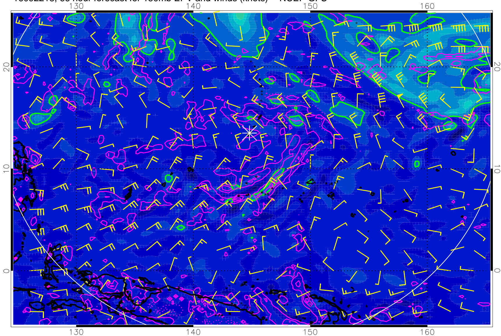
16092218, 66 hour forecast for 150mb EPV and winds (knots) -- NCEP GFS
