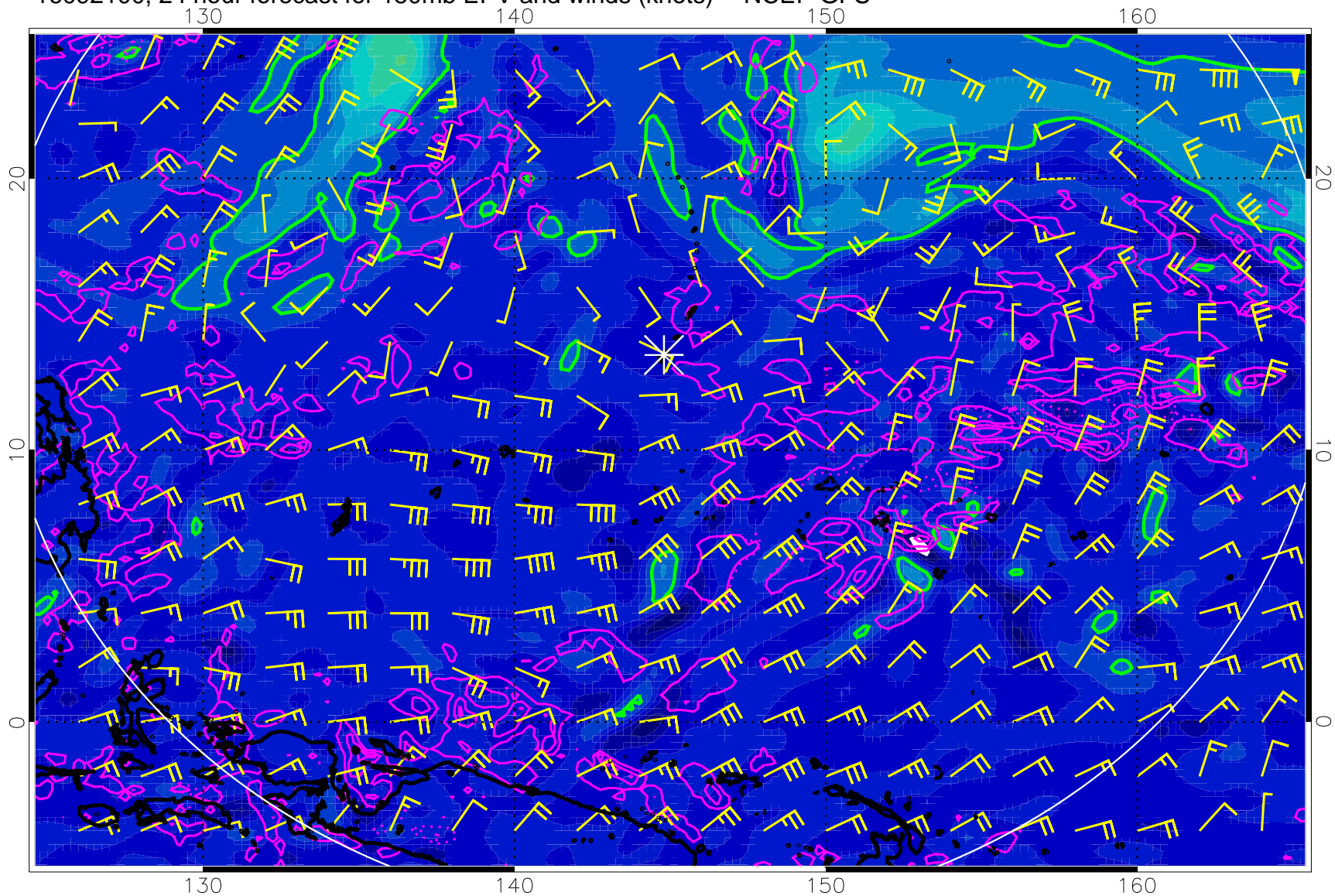
16092100, 24 hour forecast for 150mb EPV and winds (knots) -- NCEP GFS
