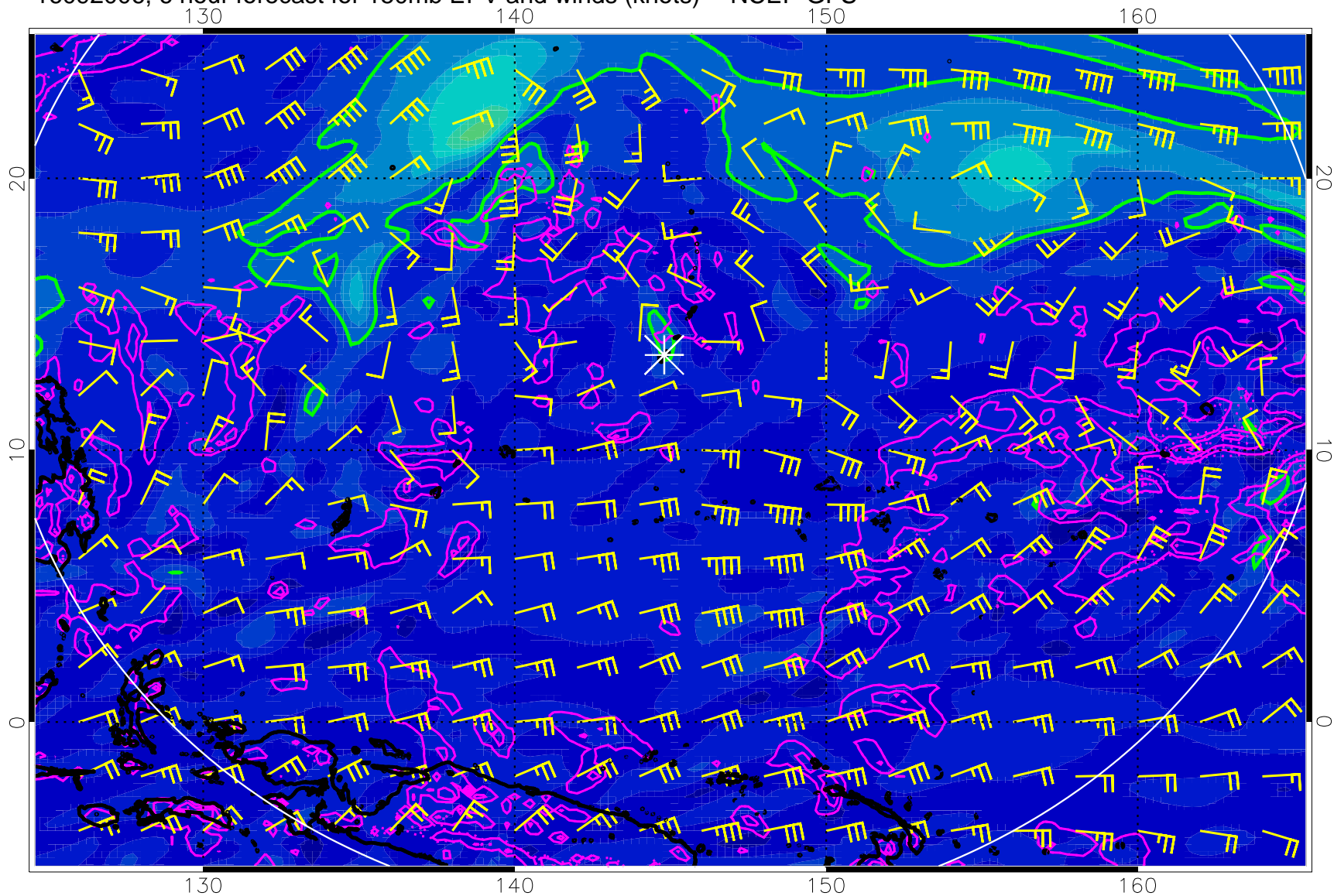
16092006, 6 hour forecast for 150mb EPV and winds (knots) -- NCEP GFS
