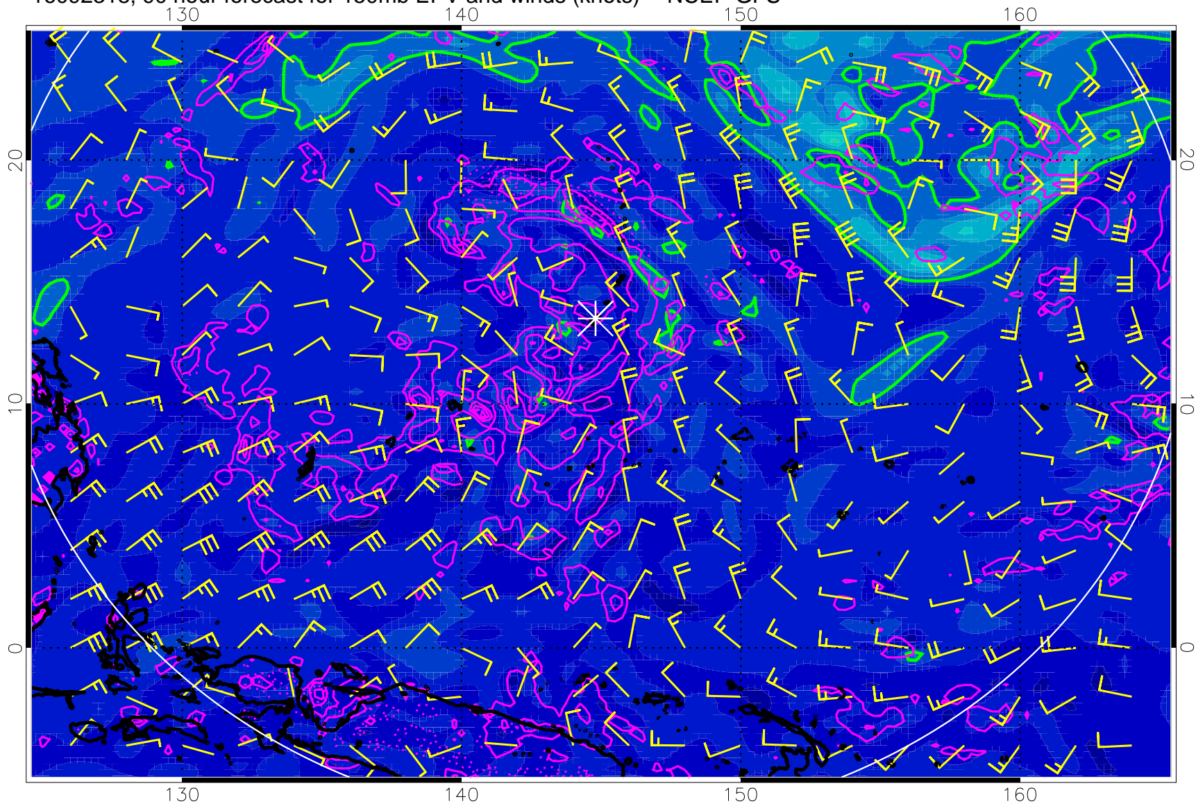
16092318, 90 hour forecast for 150mb EPV and winds (knots) -- NCEP GFS
