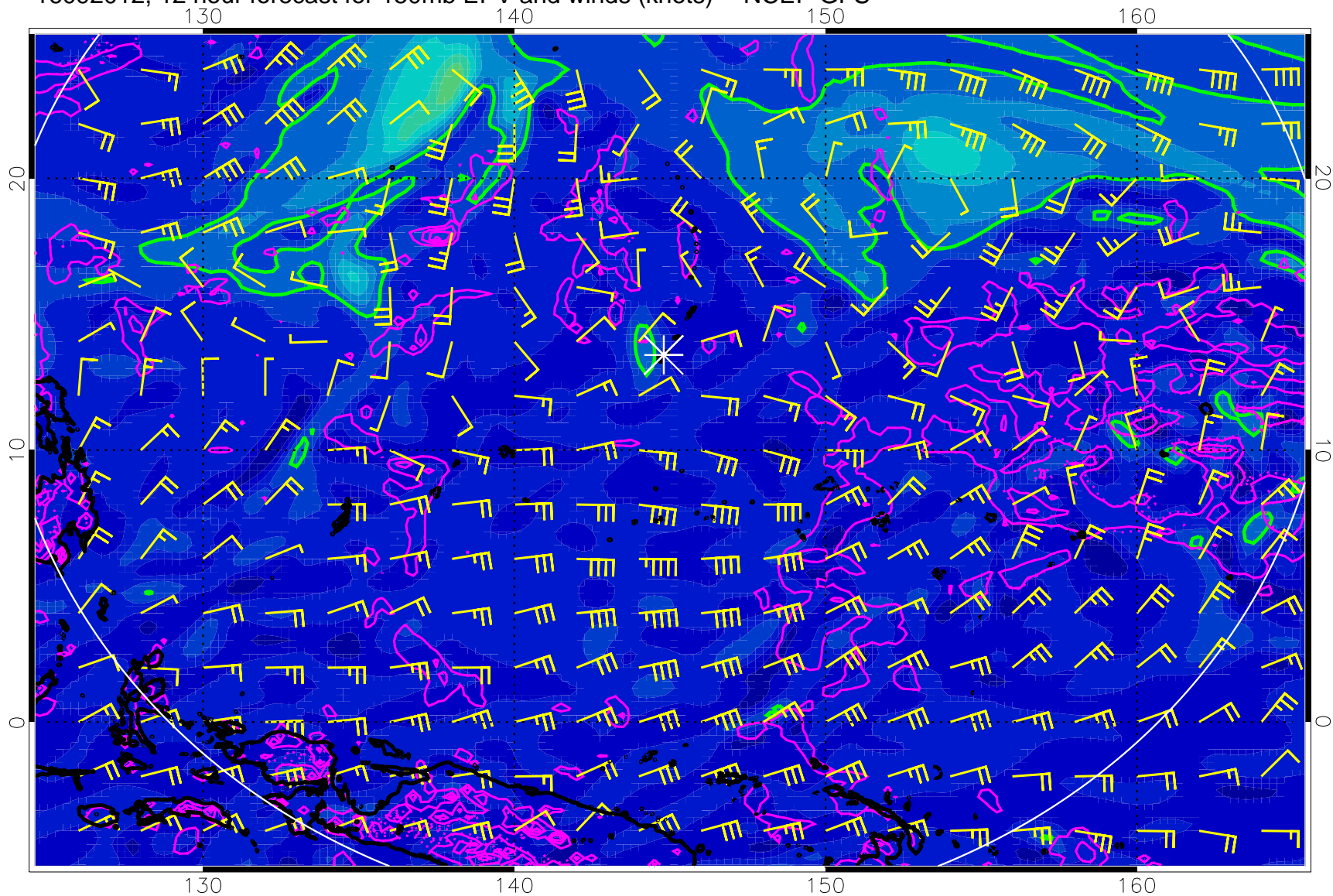
16092012, 12 hour forecast for 150mb EPV and winds (knots) -- NCEP GFS
