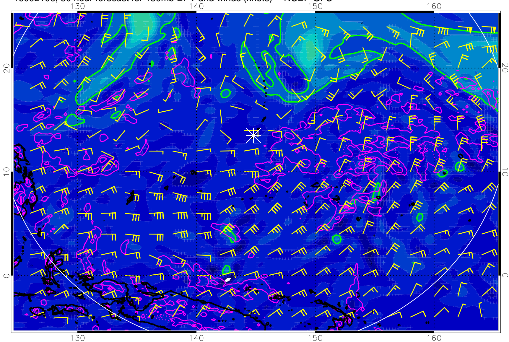
16092106, 30 hour forecast for 150mb EPV and winds (knots) -- NCEP GFS
