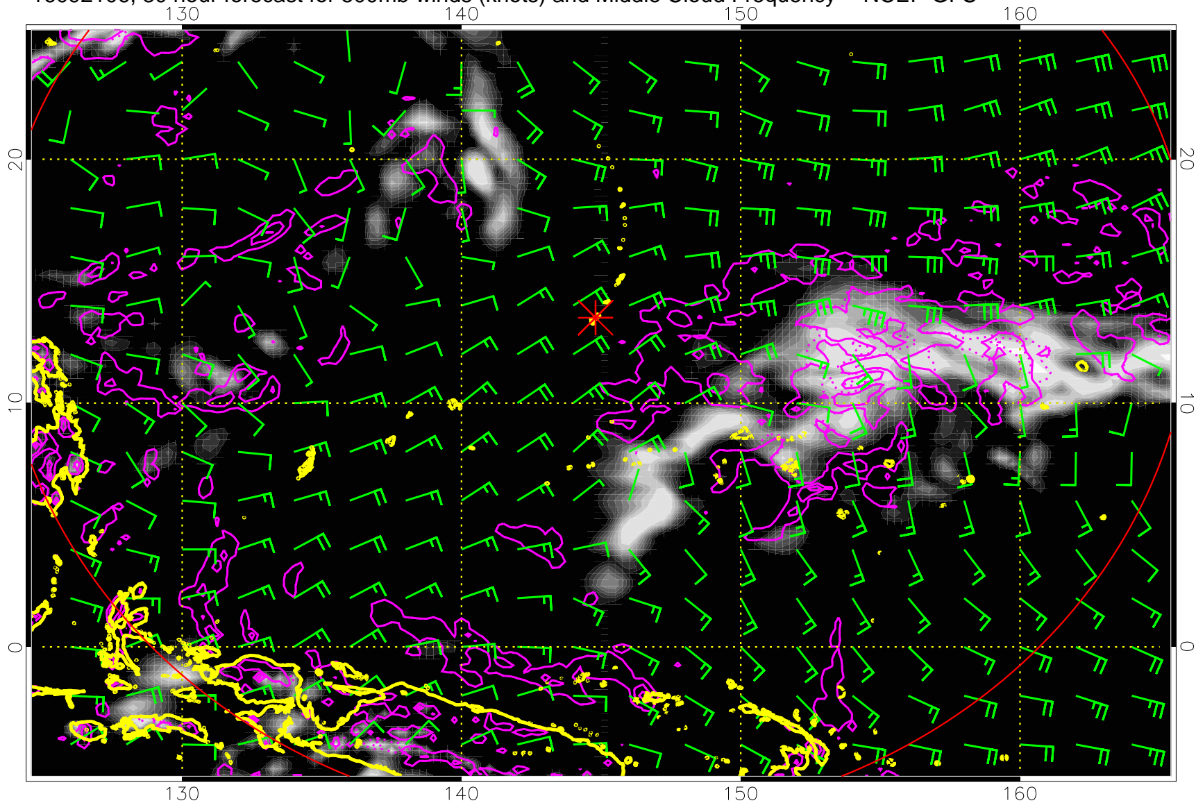
16092106, 30 hour forecast for 500mb winds (knots) and Middle Cloud Frequency -- NCEP GFS
