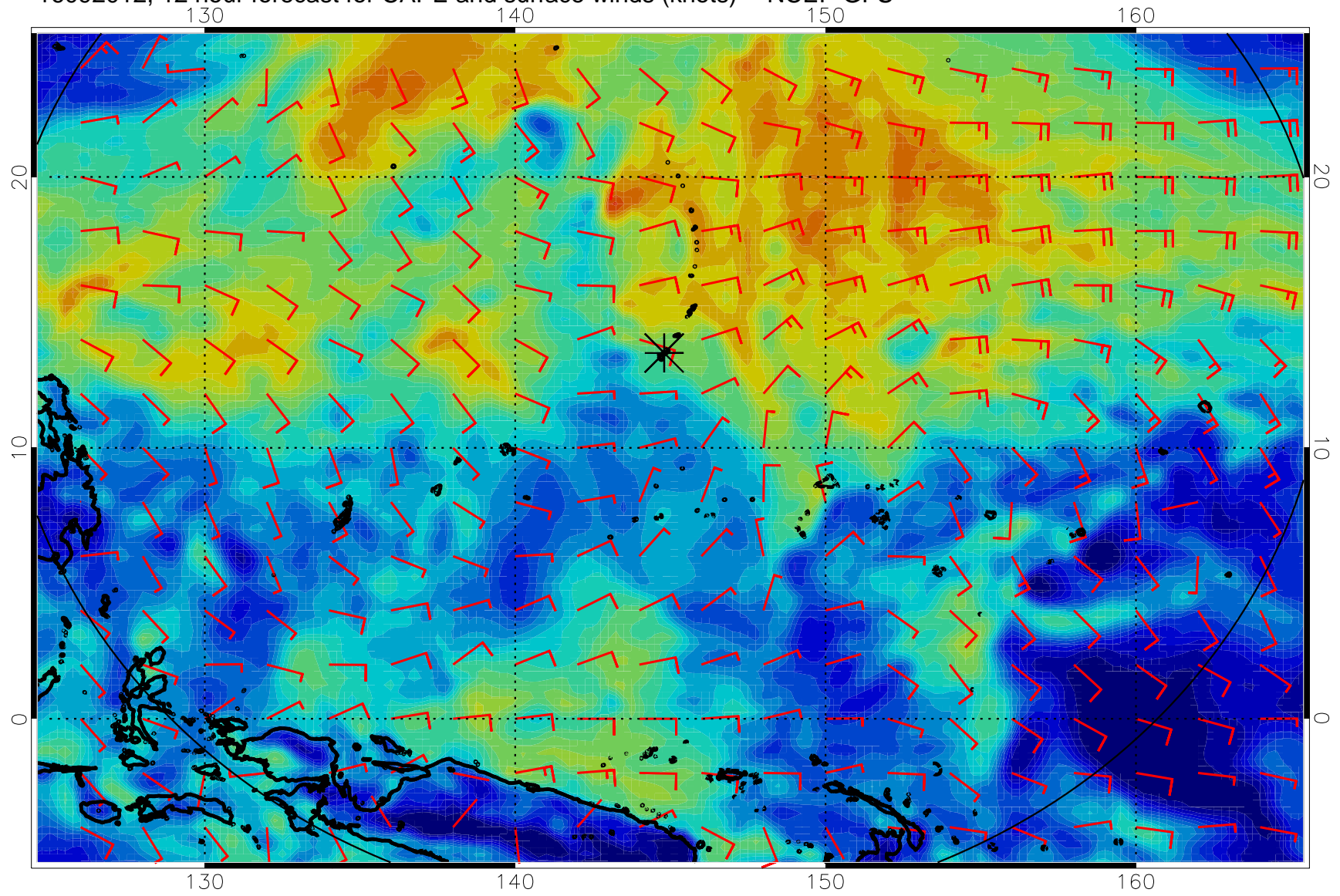
16092012, 12 hour forecast for CAPE and surface winds (knots) -- NCEP GFS
