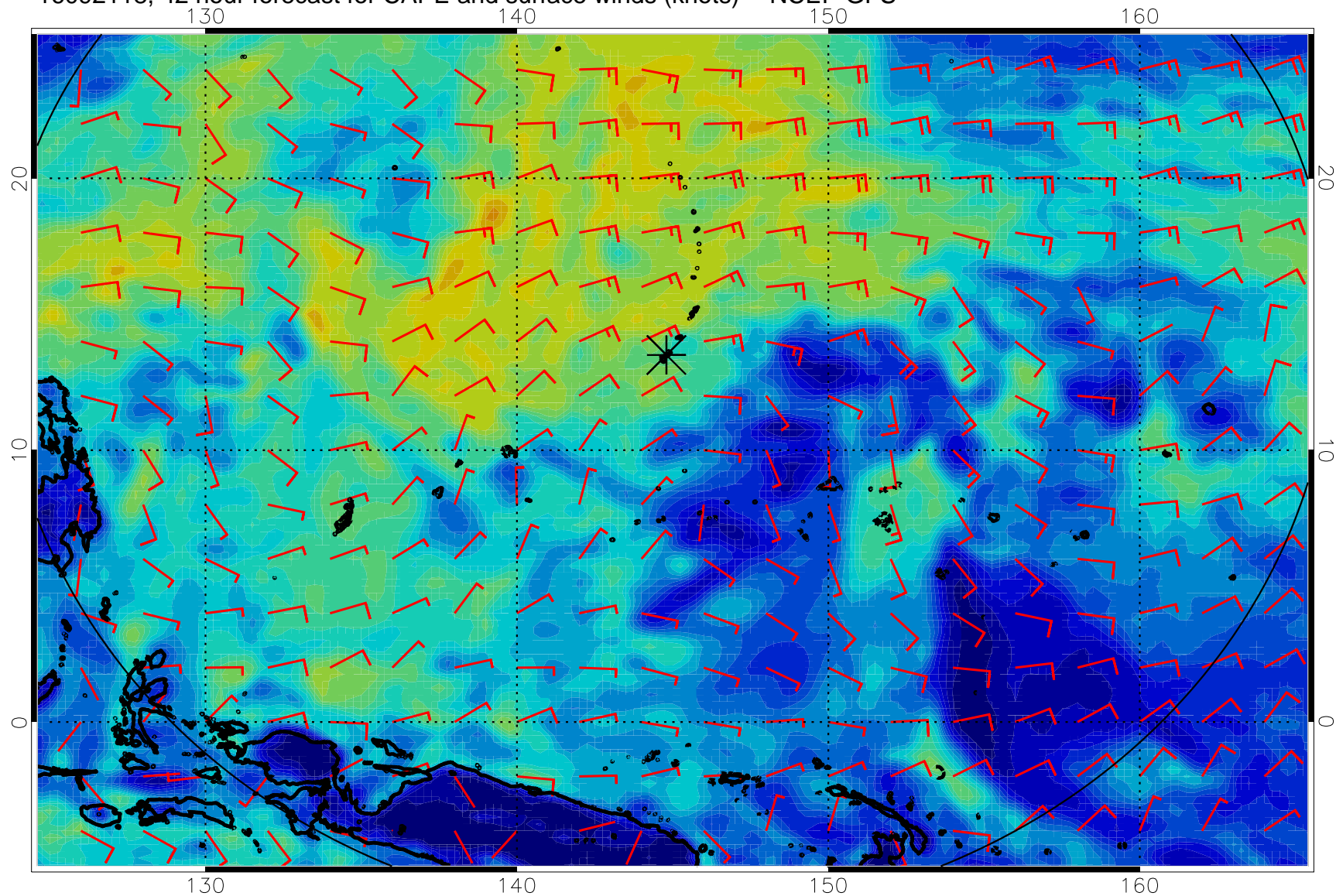
16092118, 42 hour forecast for CAPE and surface winds (knots) -- NCEP GFS
