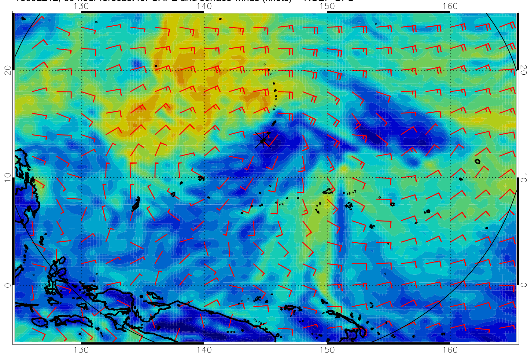
16092212, 60 hour forecast for CAPE and surface winds (knots) -- NCEP GFS
