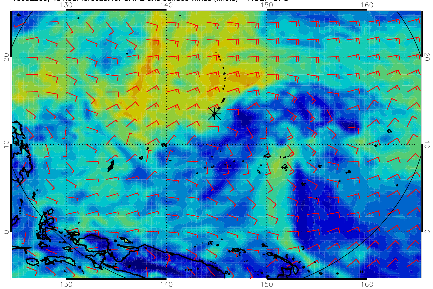
16092200, 48 hour forecast for CAPE and surface winds (knots) -- NCEP GFS
