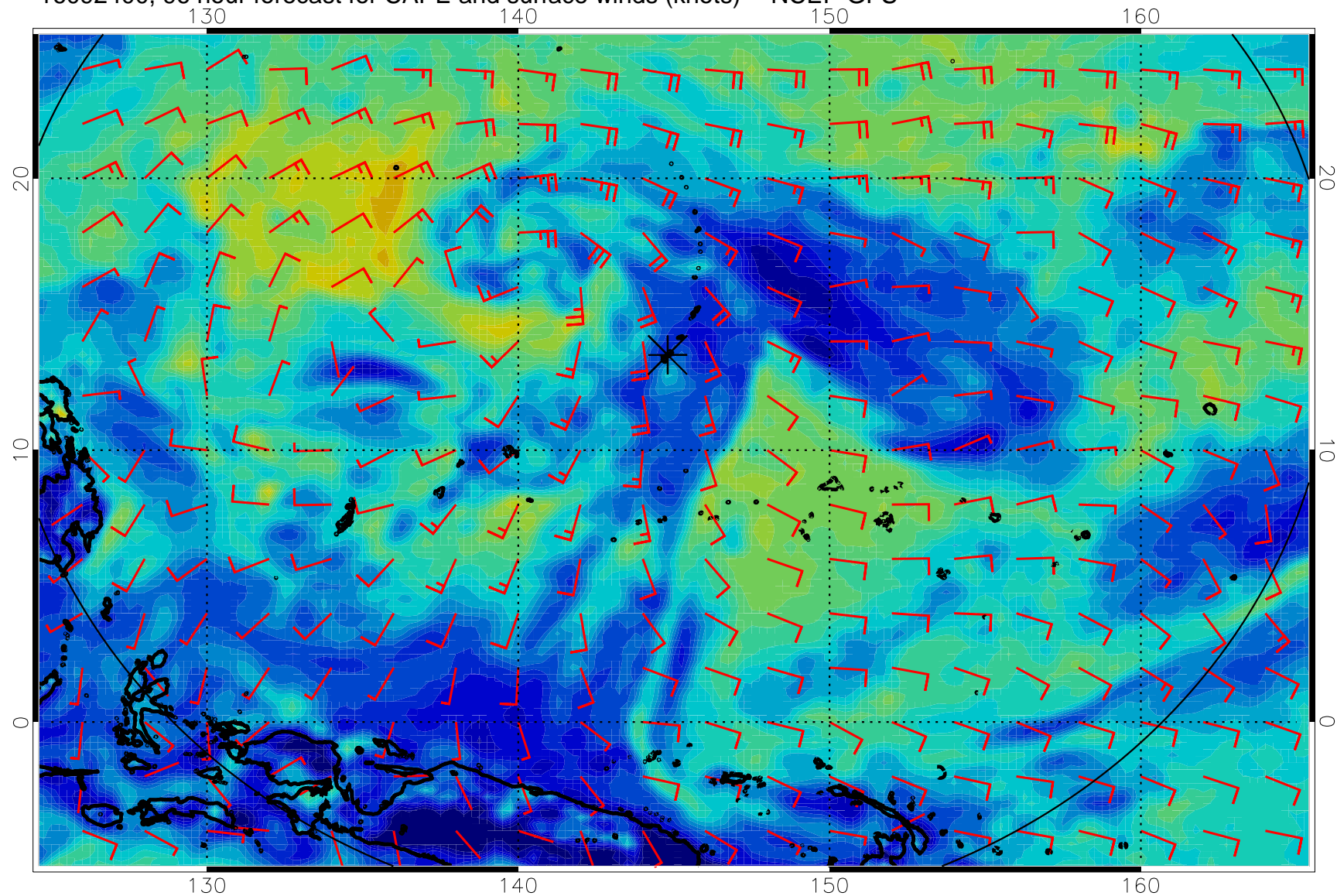
16092400, 96 hour forecast for CAPE and surface winds (knots) -- NCEP GFS
