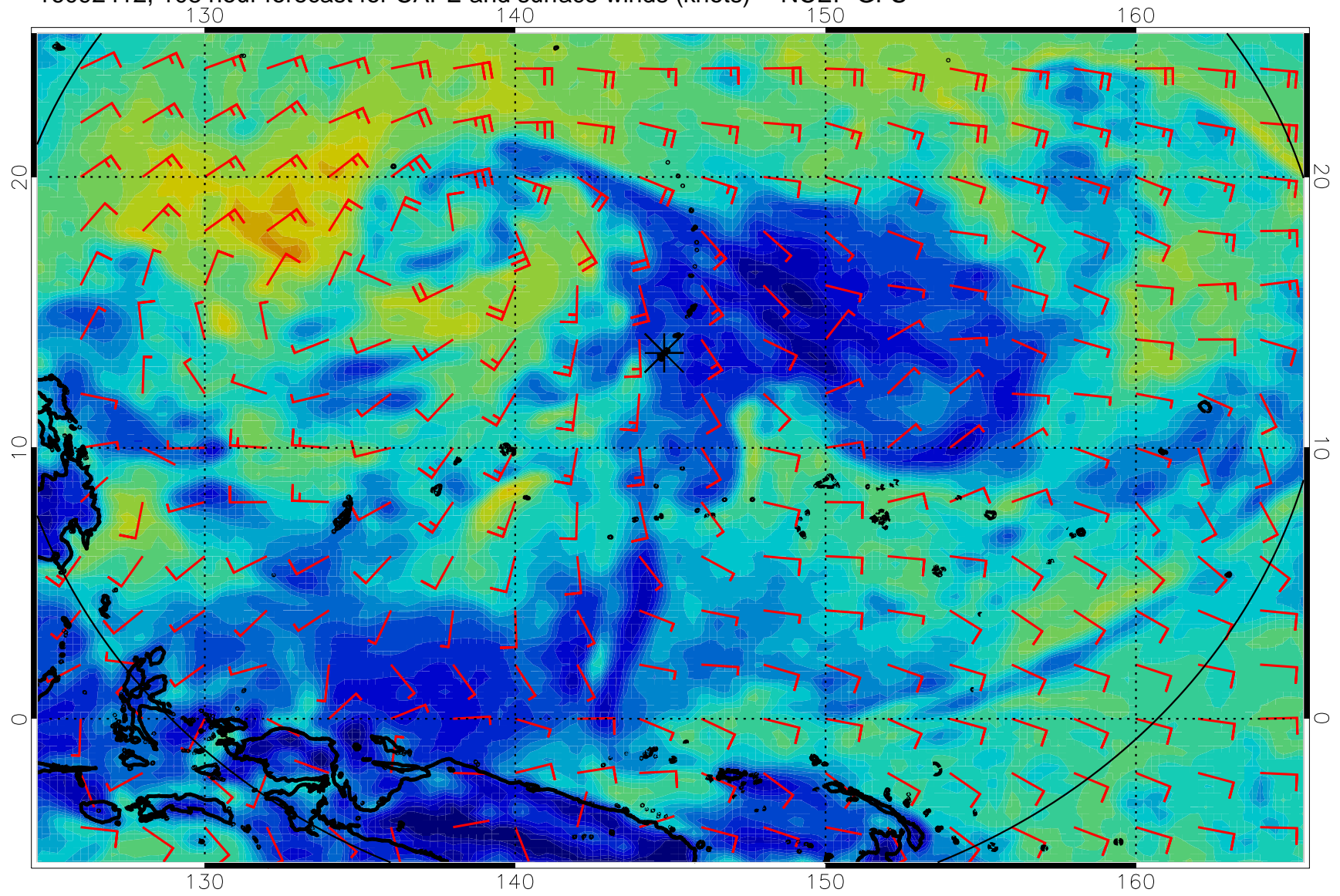
16092412, 108 hour forecast for CAPE and surface winds (knots) -- NCEP GFS
