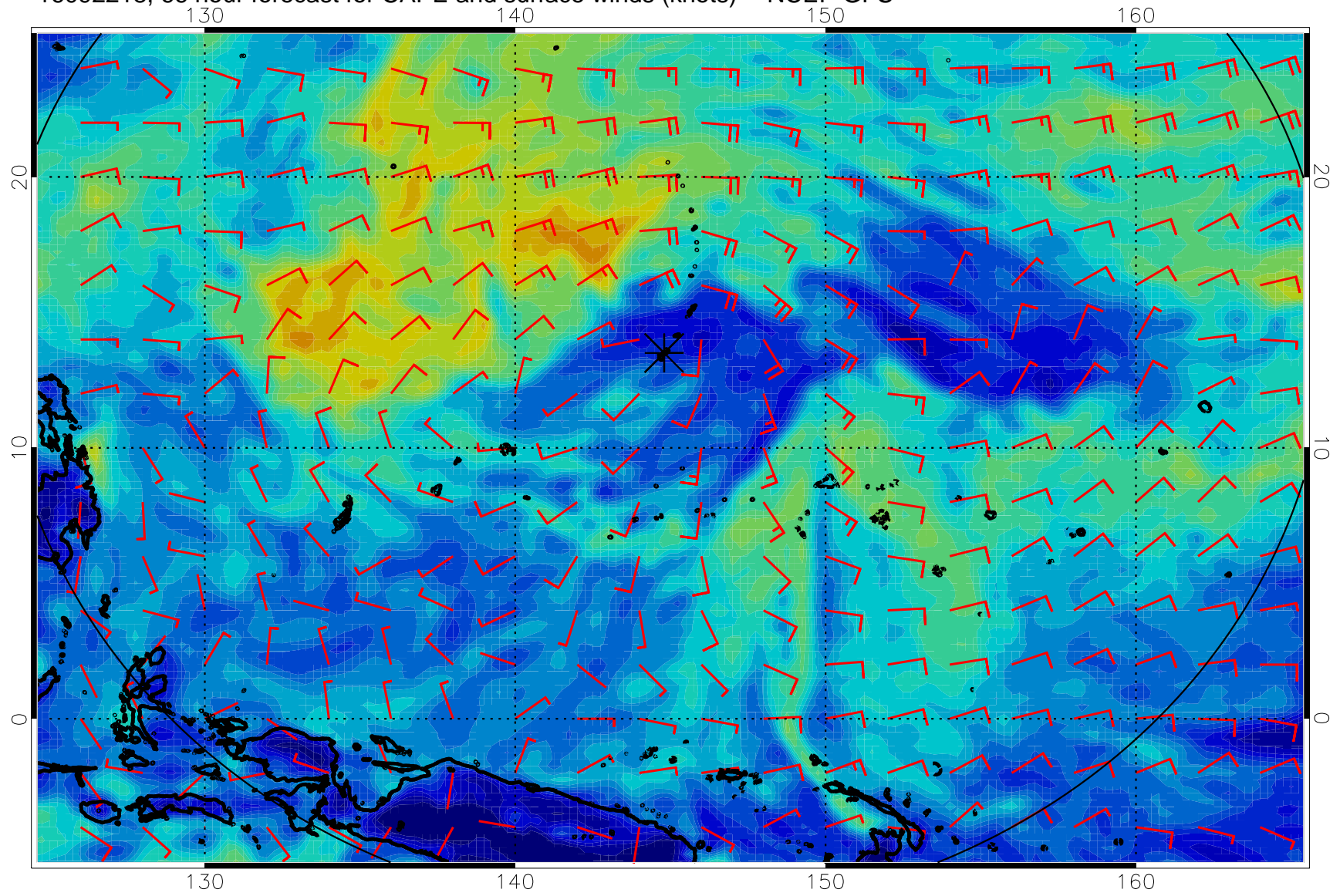
16092218, 66 hour forecast for CAPE and surface winds (knots) -- NCEP GFS
