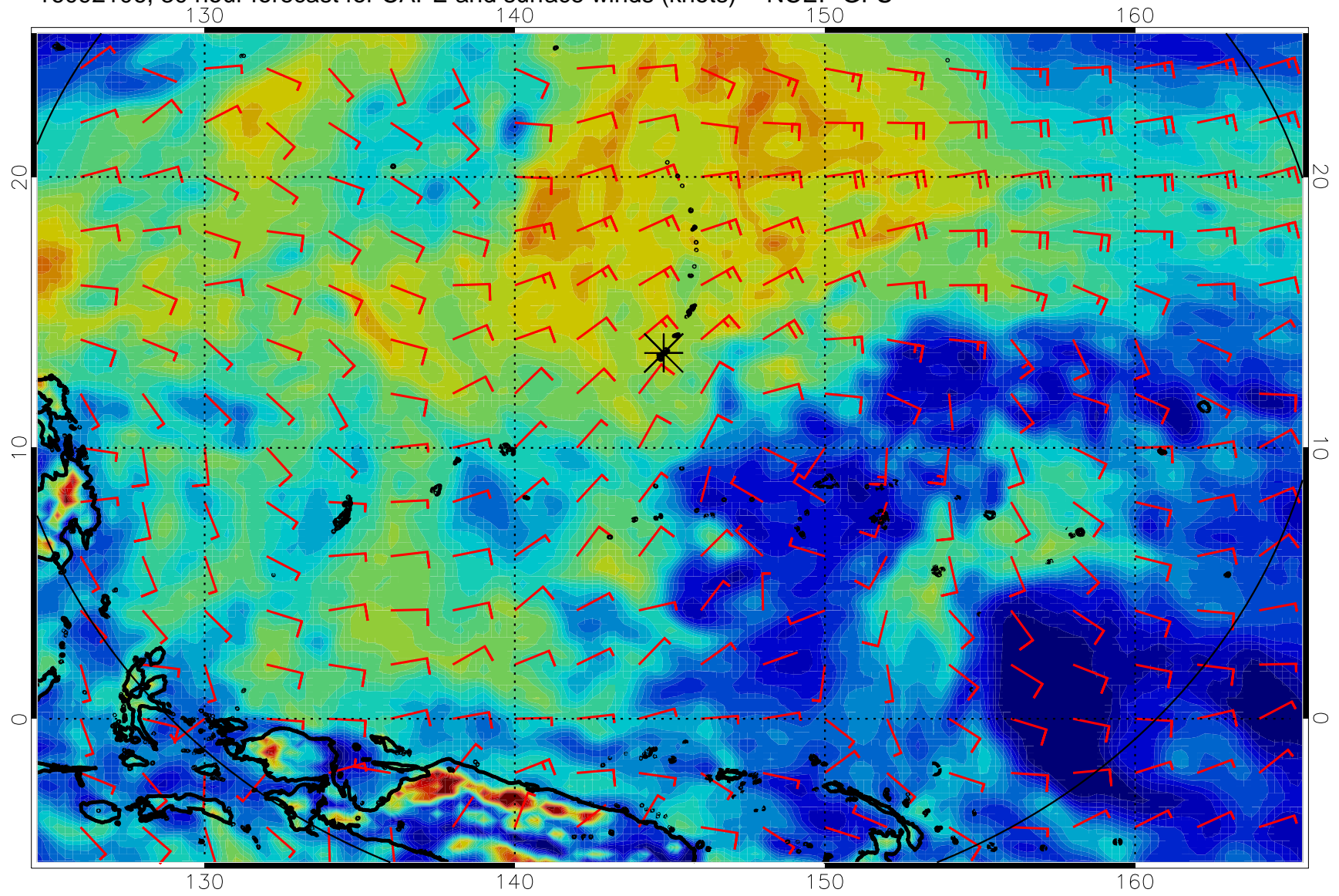
16092106, 30 hour forecast for CAPE and surface winds (knots) -- NCEP GFS
