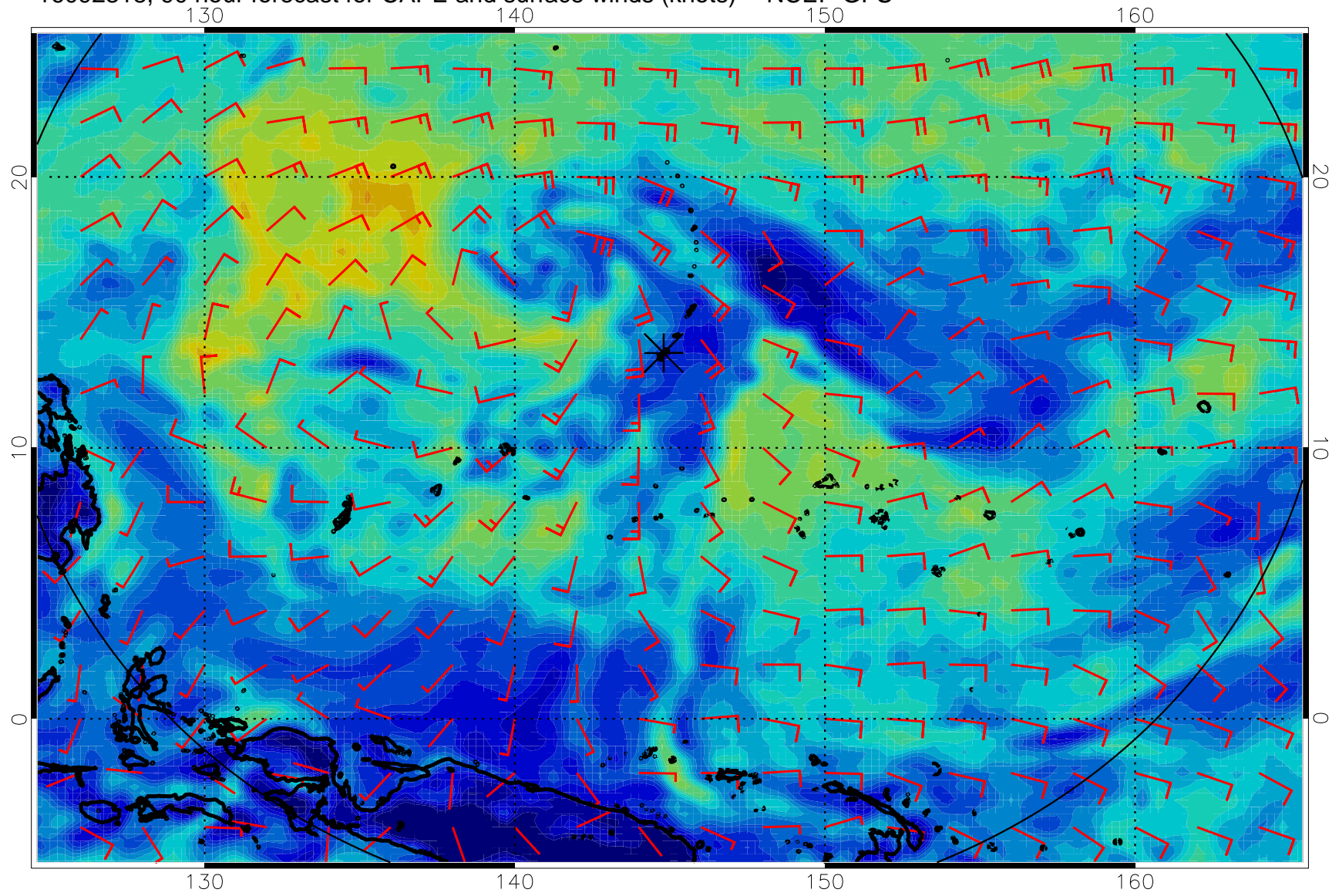
16092318, 90 hour forecast for CAPE and surface winds (knots) -- NCEP GFS
