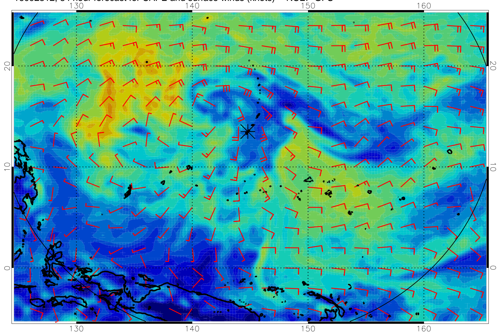
16092312, 84 hour forecast for CAPE and surface winds (knots) -- NCEP GFS
