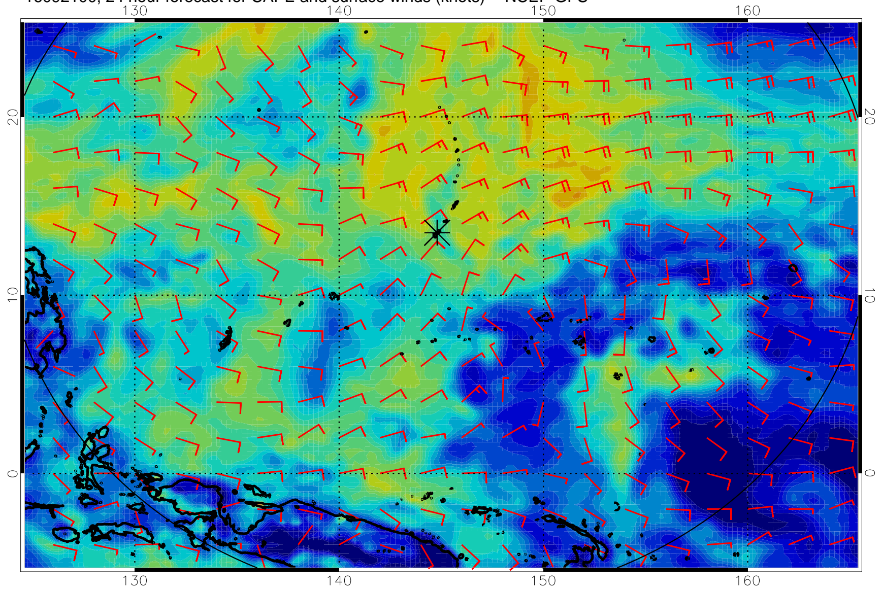
16092100, 24 hour forecast for CAPE and surface winds (knots) -- NCEP GFS
