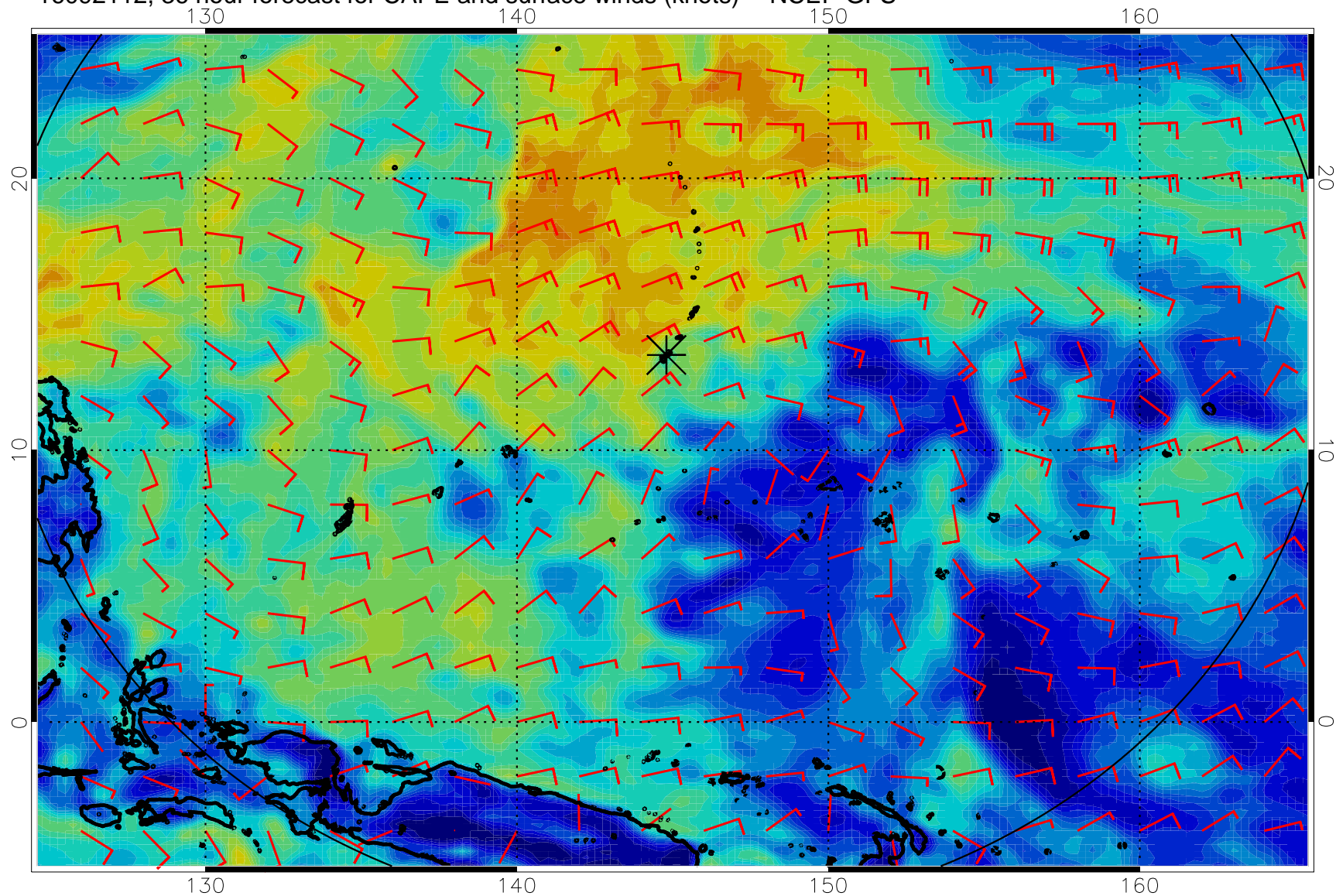
16092112, 36 hour forecast for CAPE and surface winds (knots) -- NCEP GFS
