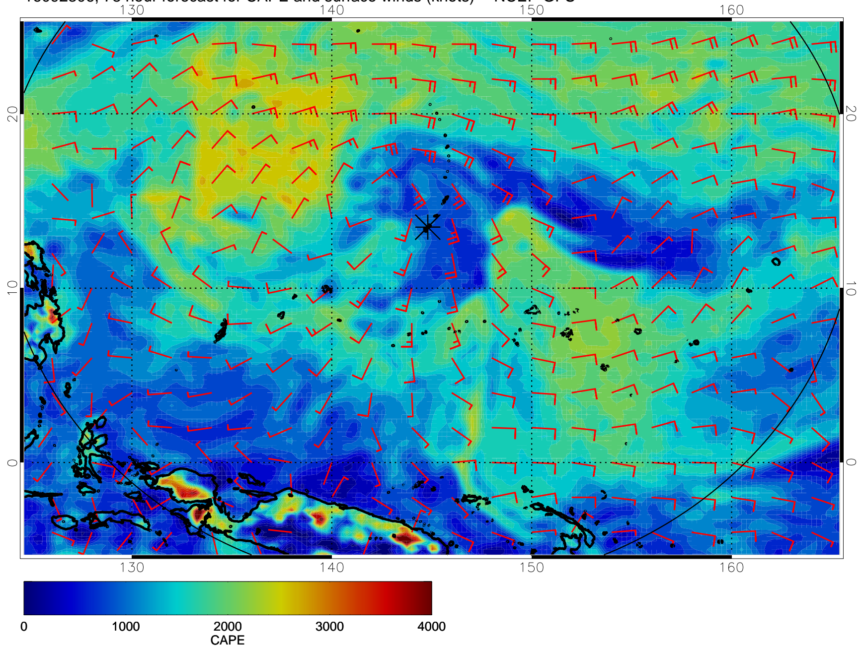
16092306, 78 hour forecast for CAPE and surface winds (knots) -- NCEP GFS
