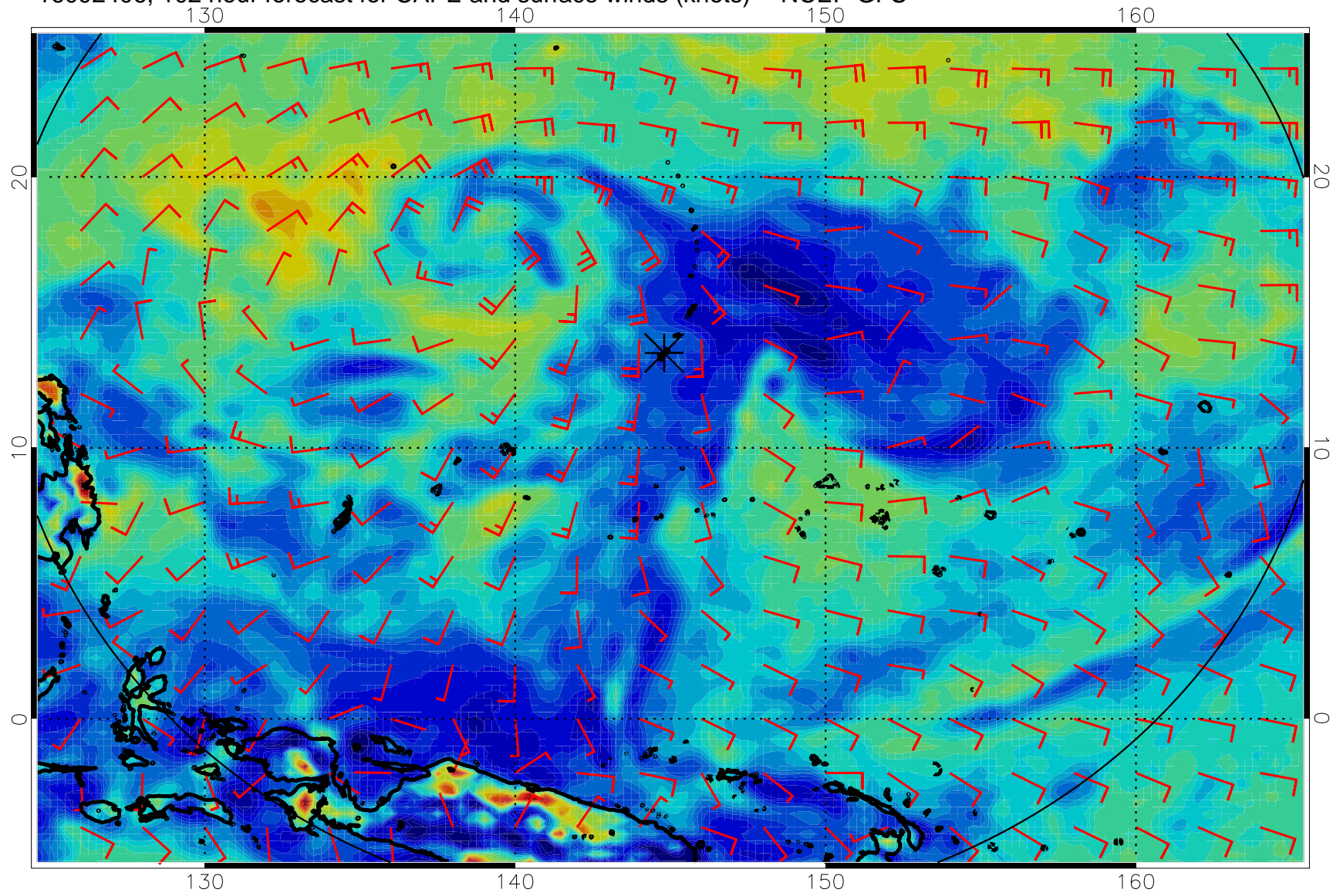
16092406, 102 hour forecast for CAPE and surface winds (knots) -- NCEP GFS
