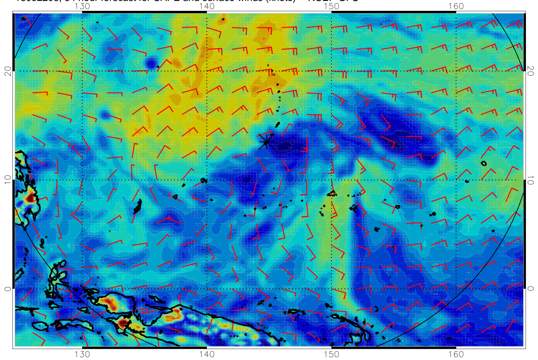
16092206, 54 hour forecast for CAPE and surface winds (knots) -- NCEP GFS
