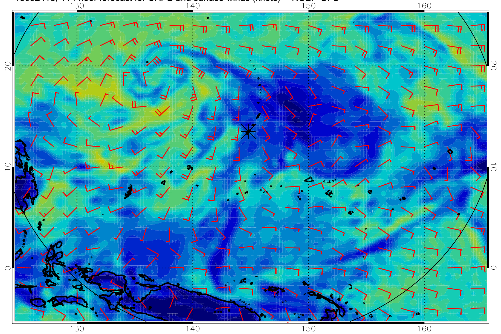
16092418, 114 hour forecast for CAPE and surface winds (knots) -- NCEP GFS
