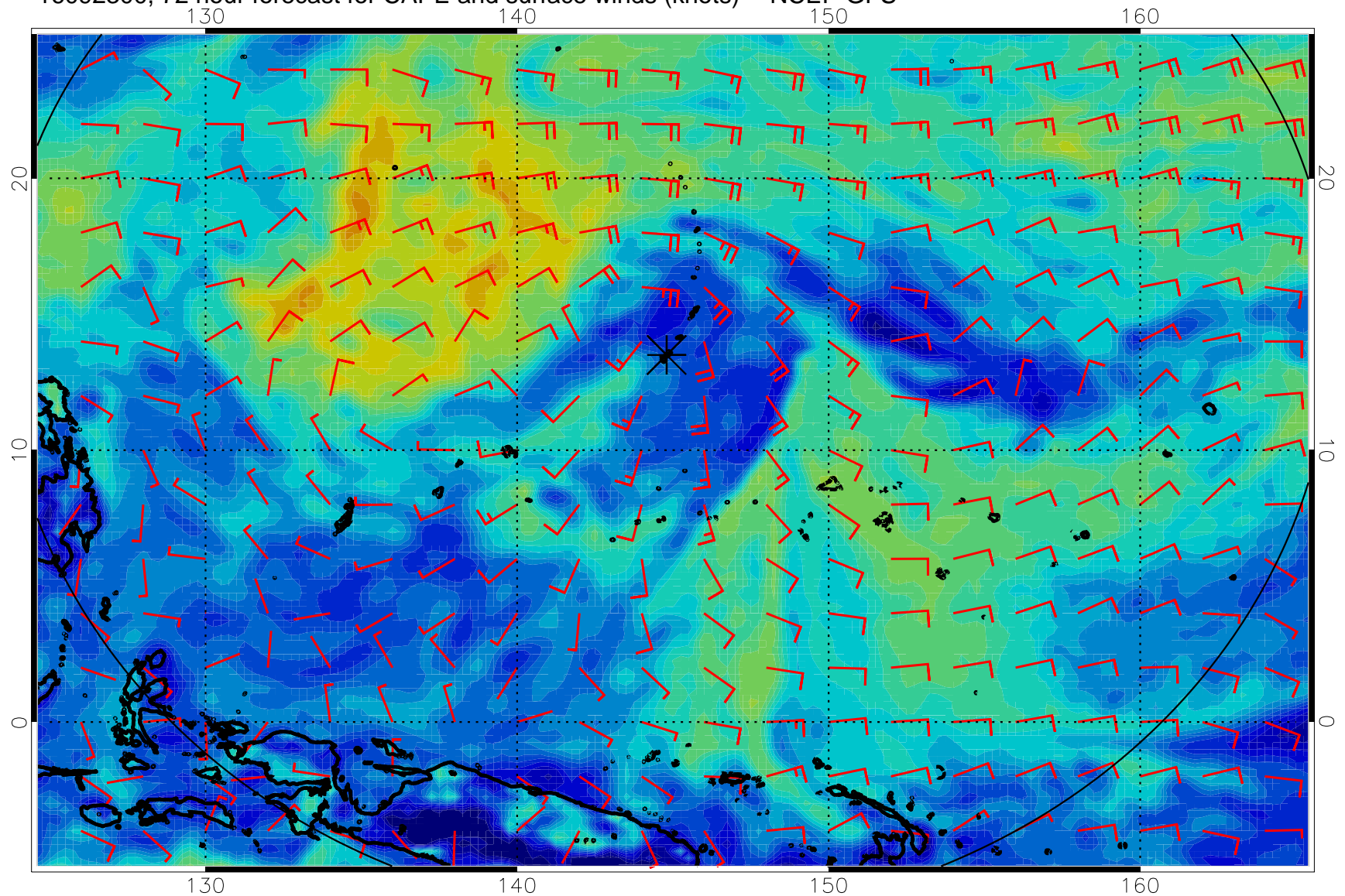
16092300, 72 hour forecast for CAPE and surface winds (knots) -- NCEP GFS
