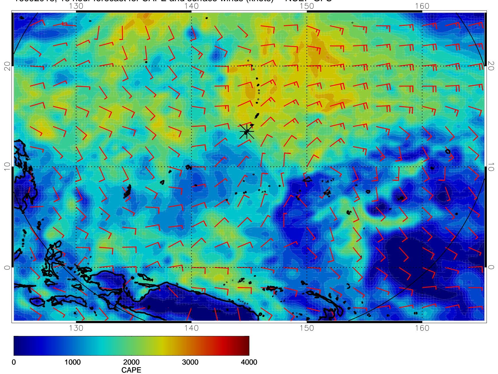
16092018, 18 hour forecast for CAPE and surface winds (knots) -- NCEP GFS
