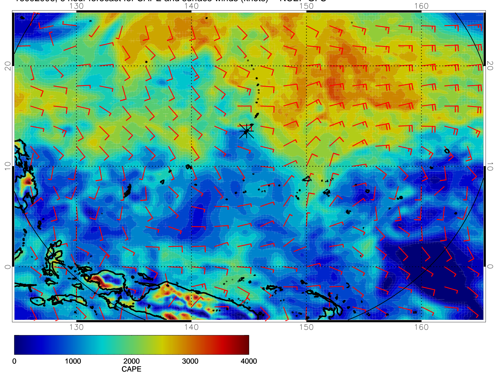
16092006, 6 hour forecast for CAPE and surface winds (knots) -- NCEP GFS
