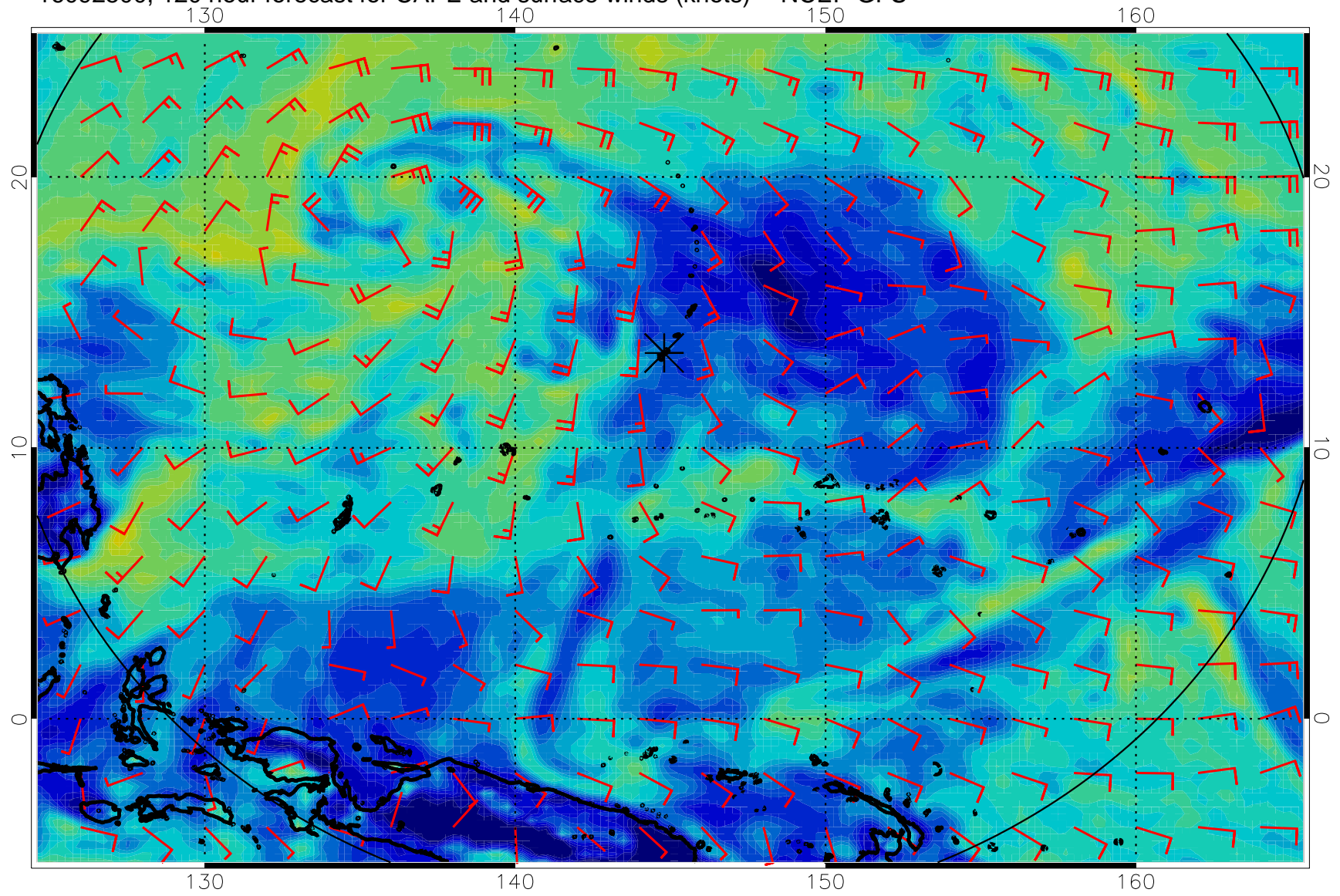
16092500, 120 hour forecast for CAPE and surface winds (knots) -- NCEP GFS
