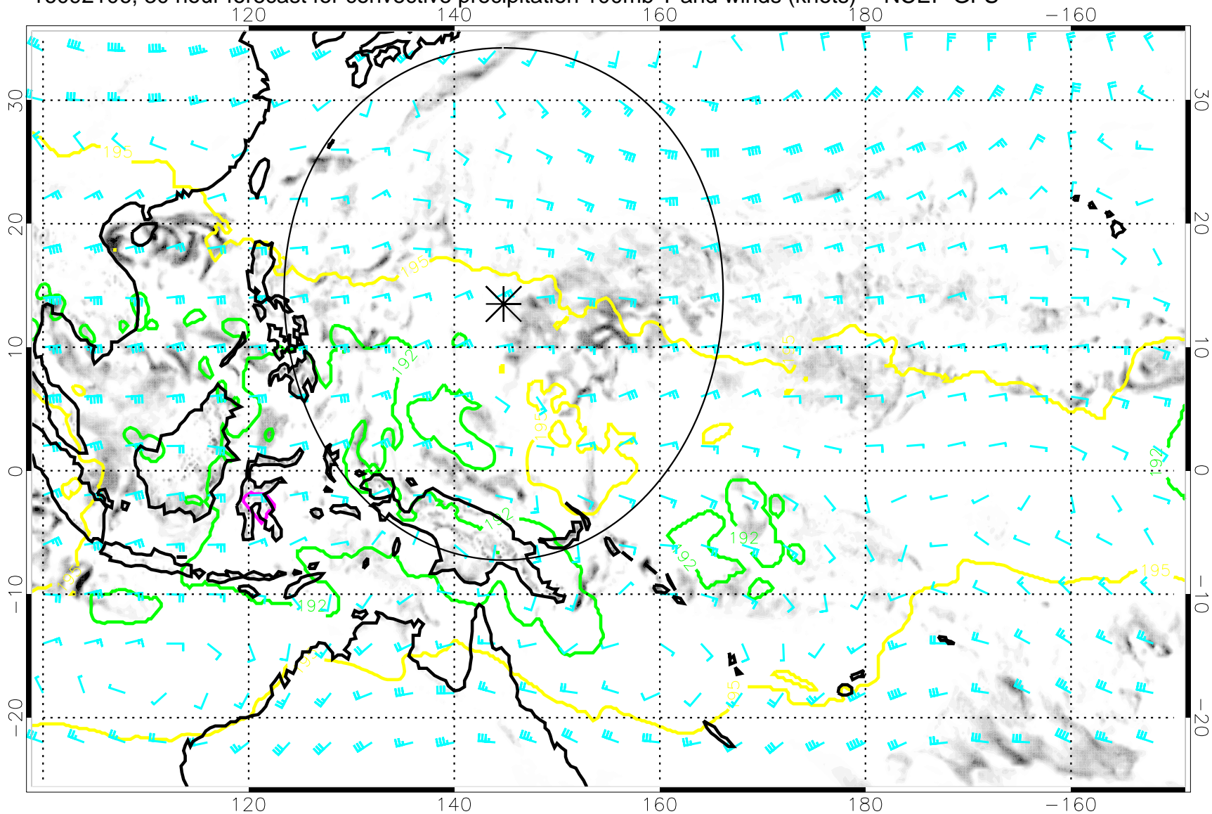
16092106, 30 hour forecast for convective precipitation 100mb T and winds (knots) -- NCEP GFS
