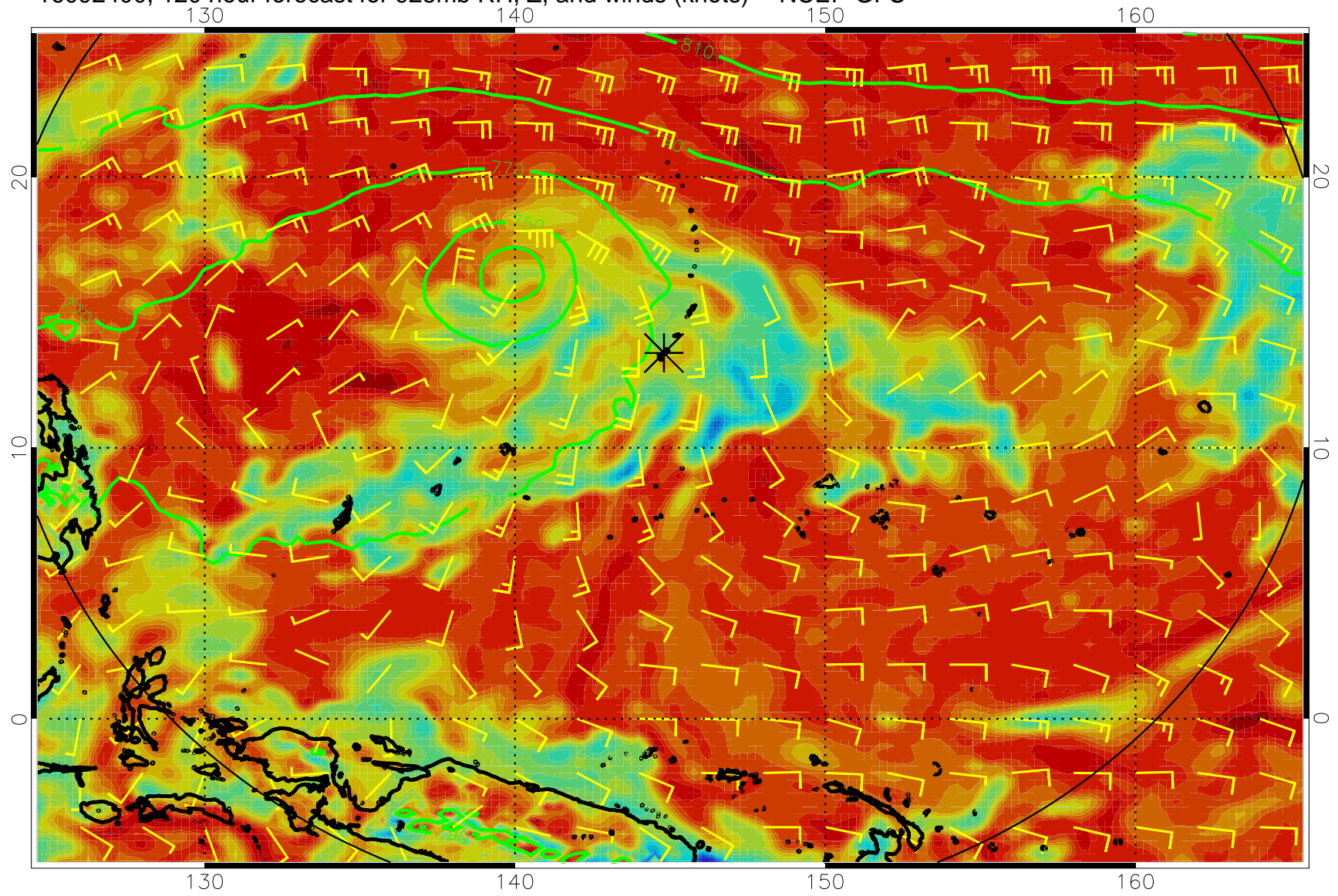
16092400, 120 hour forecast for 925mb RH, Z, and winds (knots) -- NCEP GFS
