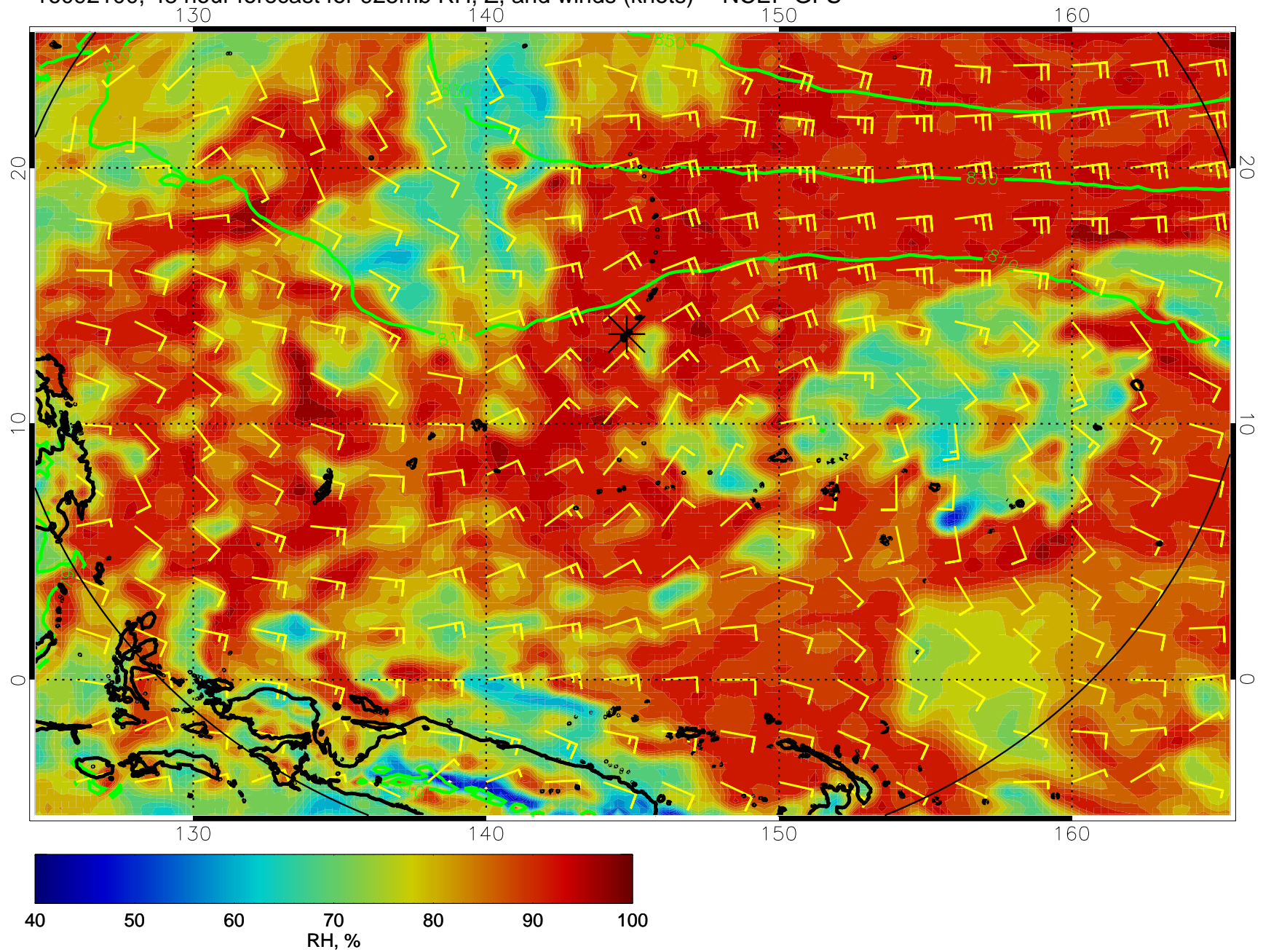
16092100, 48 hour forecast for 925mb RH, Z, and winds (knots) -- NCEP GFS
