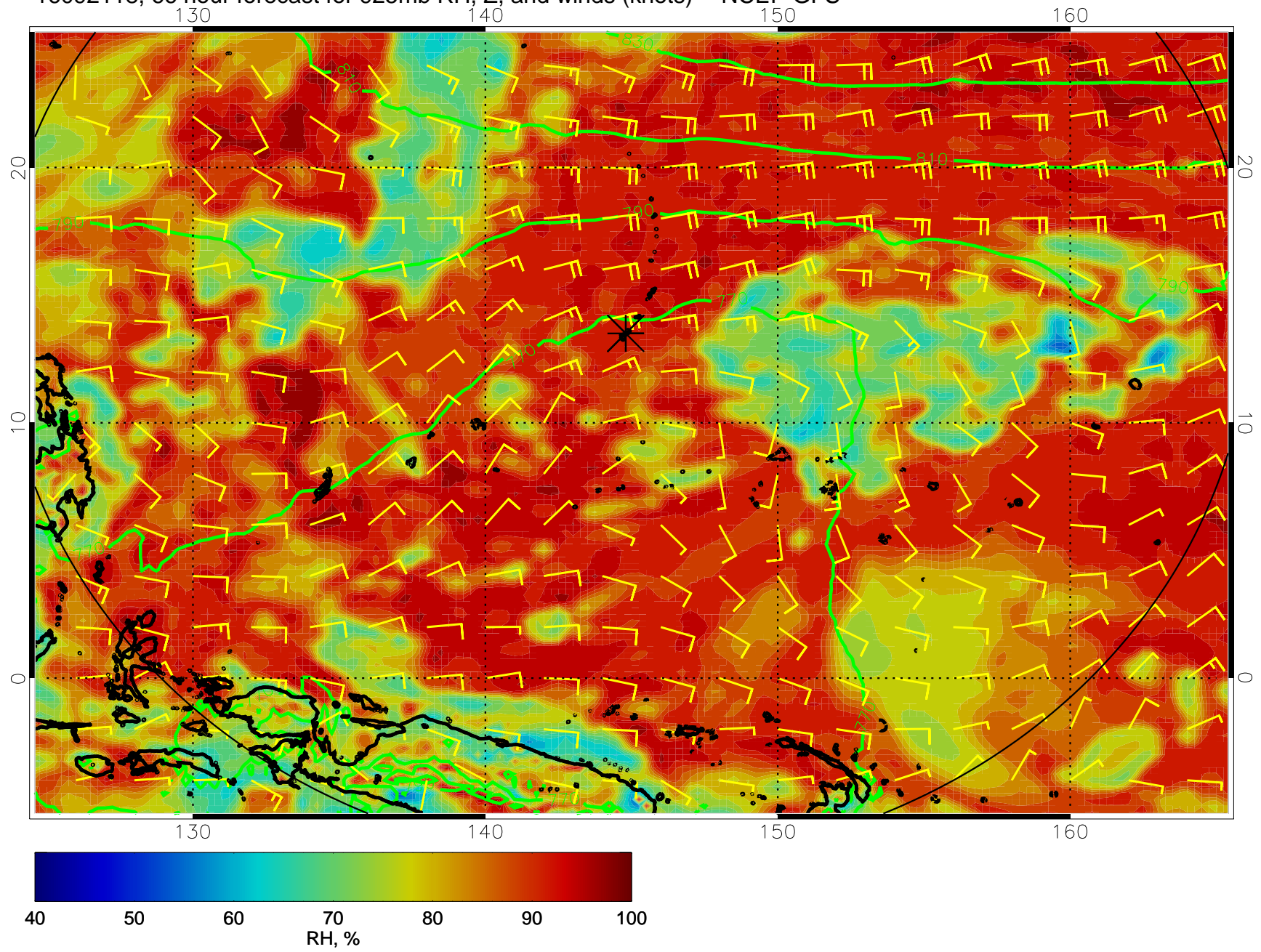
16092118, 66 hour forecast for 925mb RH, Z, and winds (knots) -- NCEP GFS
