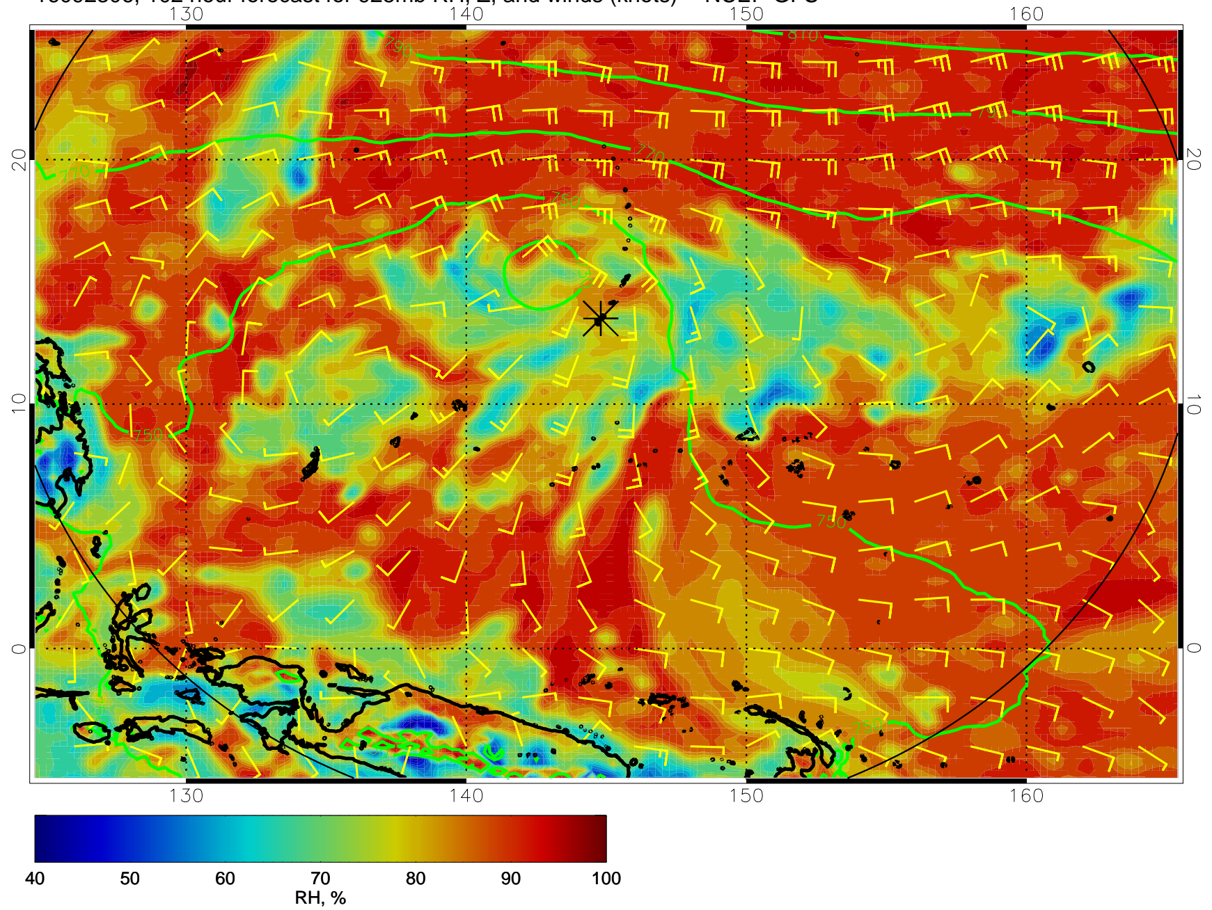
16092306, 102 hour forecast for 925mb RH, Z, and winds (knots) -- NCEP GFS
