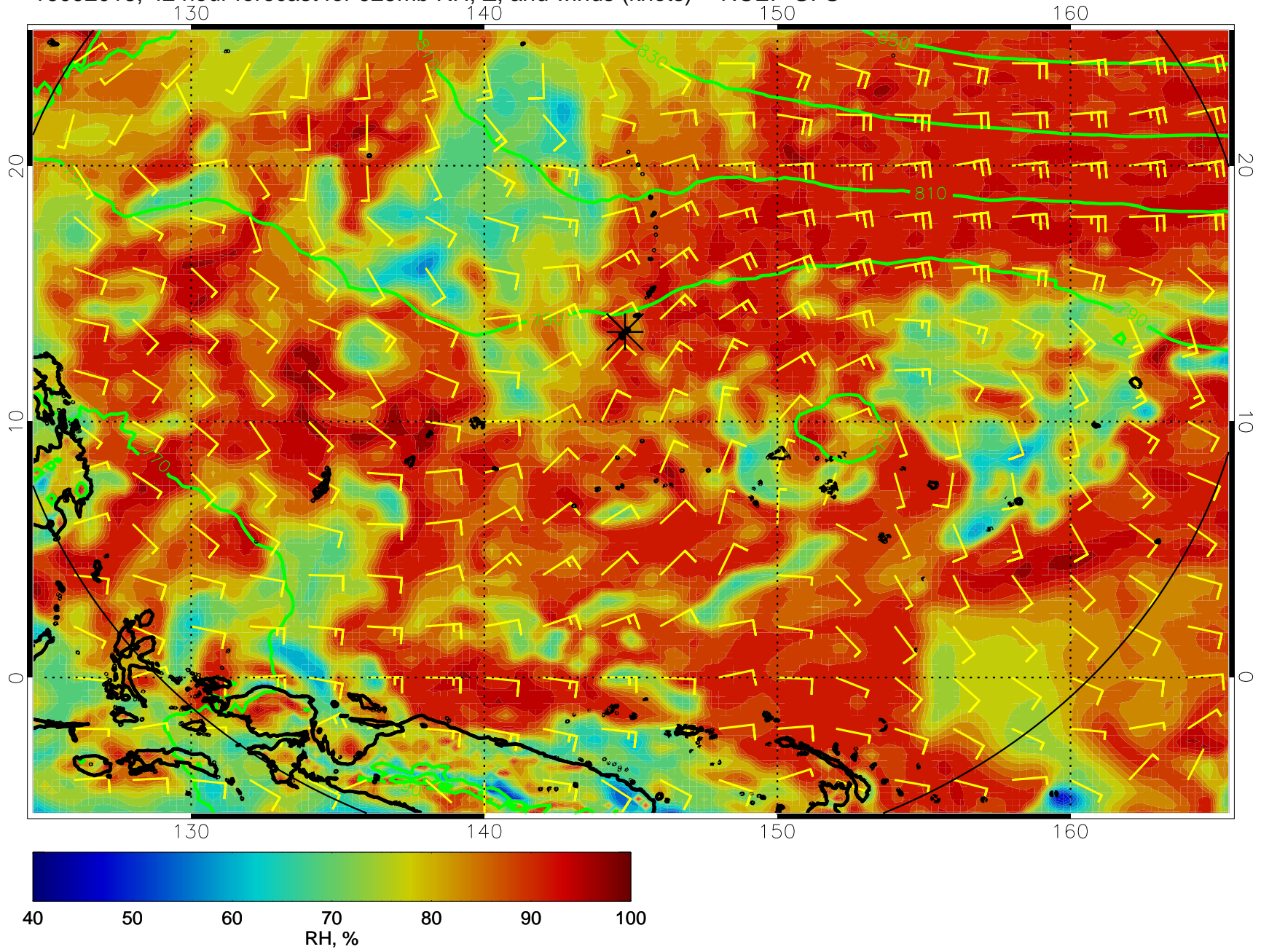
16092018, 42 hour forecast for 925mb RH, Z, and winds (knots) -- NCEP GFS
