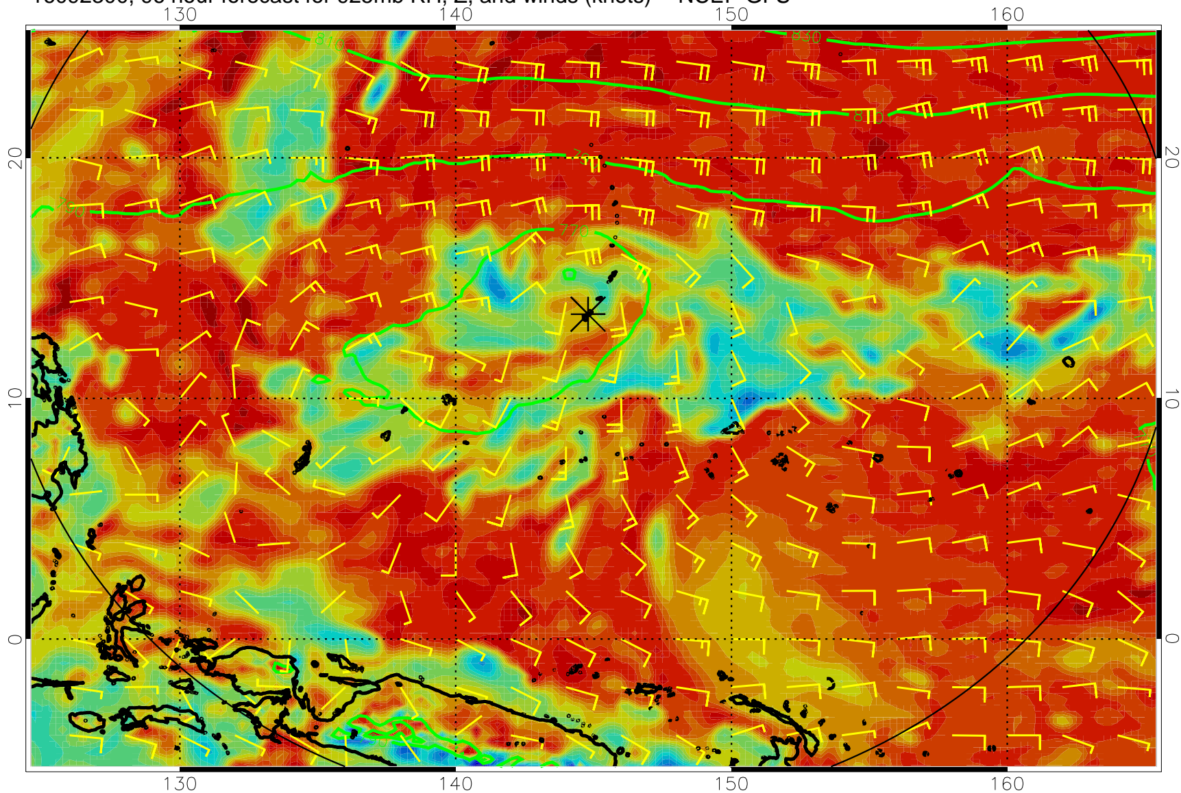
16092300, 96 hour forecast for 925mb RH, Z, and winds (knots) -- NCEP GFS
