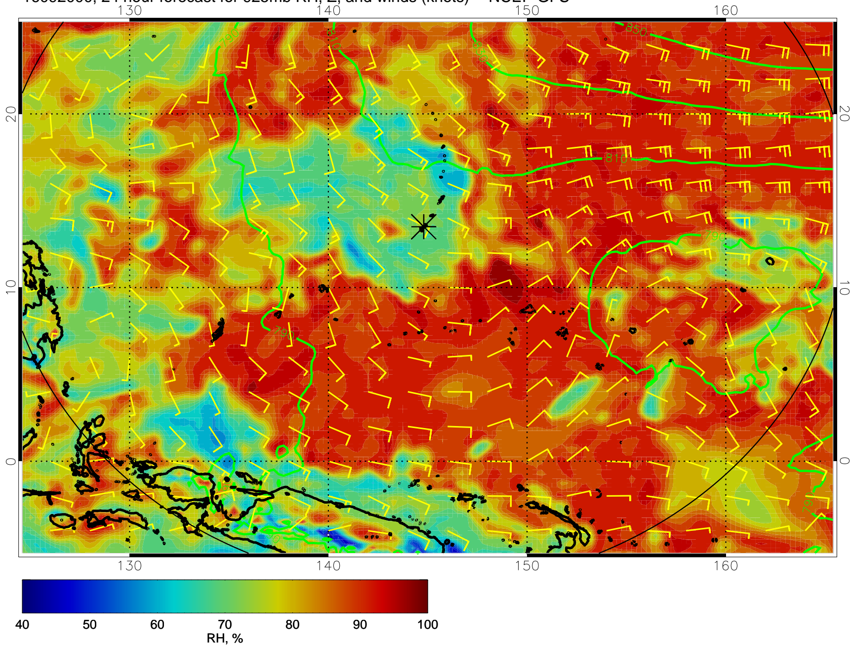
16092000, 24 hour forecast for 925mb RH, Z, and winds (knots) -- NCEP GFS
