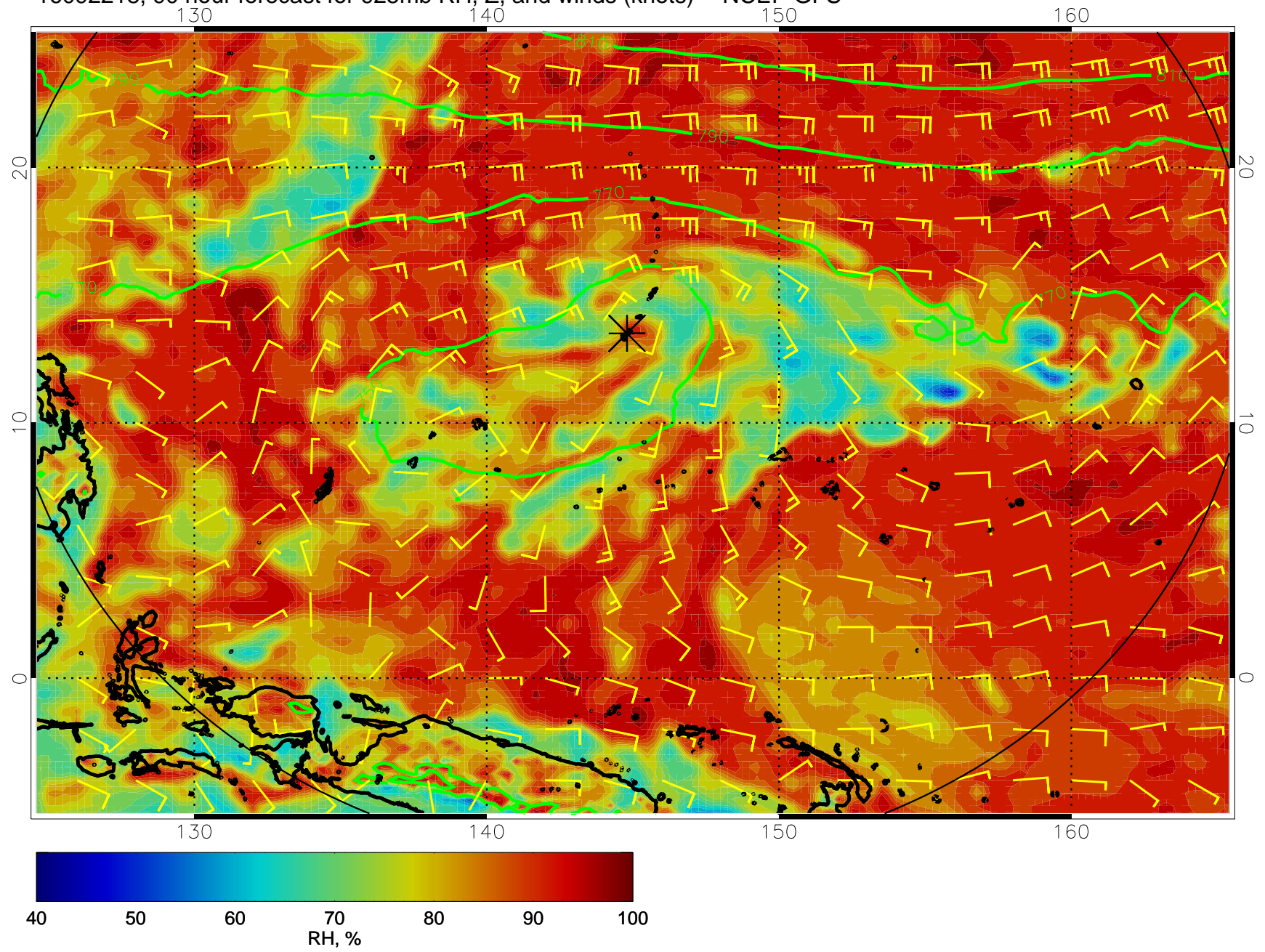
16092218, 90 hour forecast for 925mb RH, Z, and winds (knots) -- NCEP GFS
