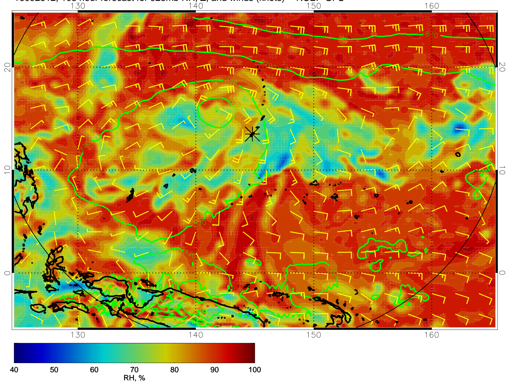
16092312, 108 hour forecast for 925mb RH, Z, and winds (knots) -- NCEP GFS
