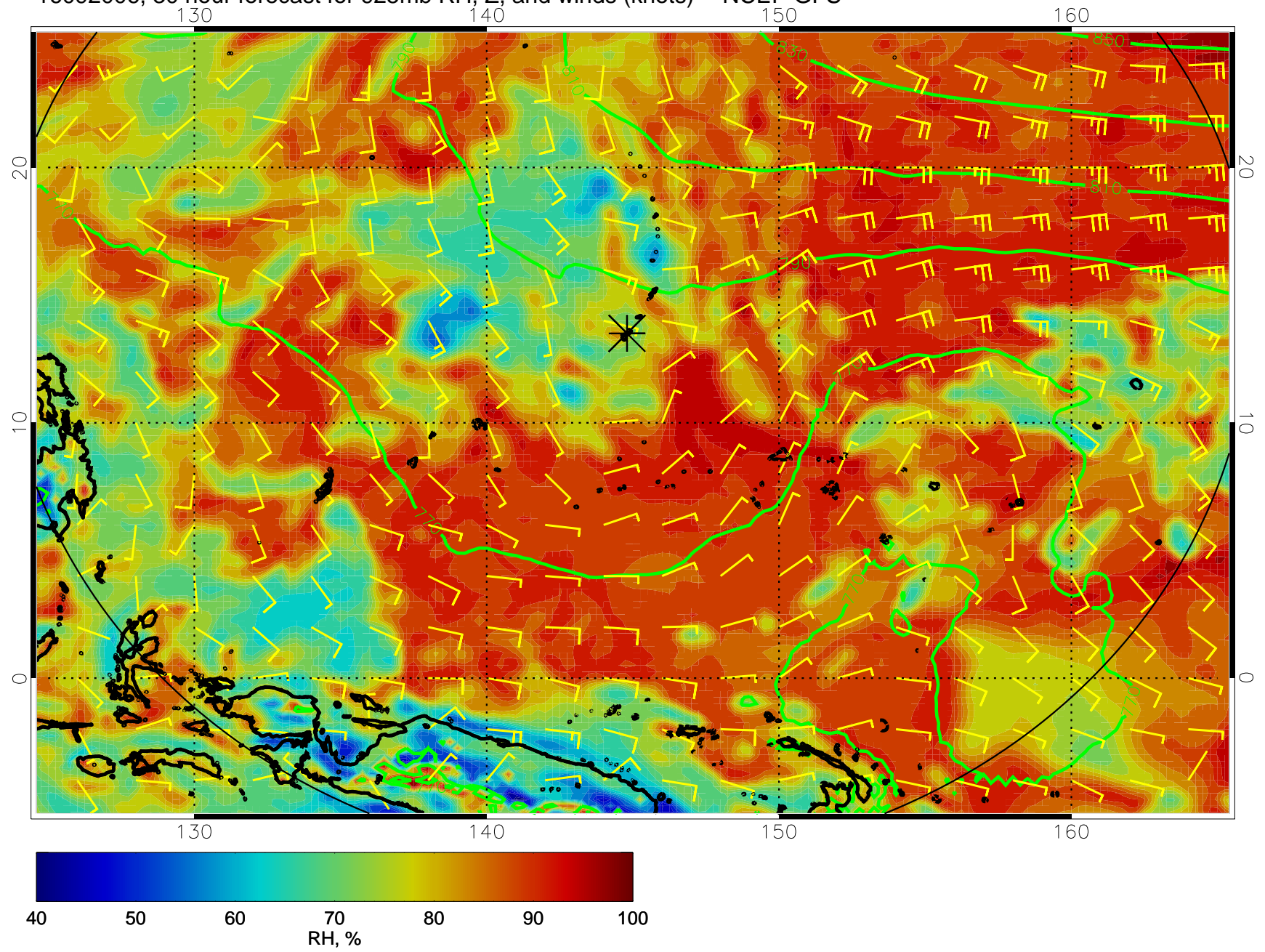
16092006, 30 hour forecast for 925mb RH, Z, and winds (knots) -- NCEP GFS
