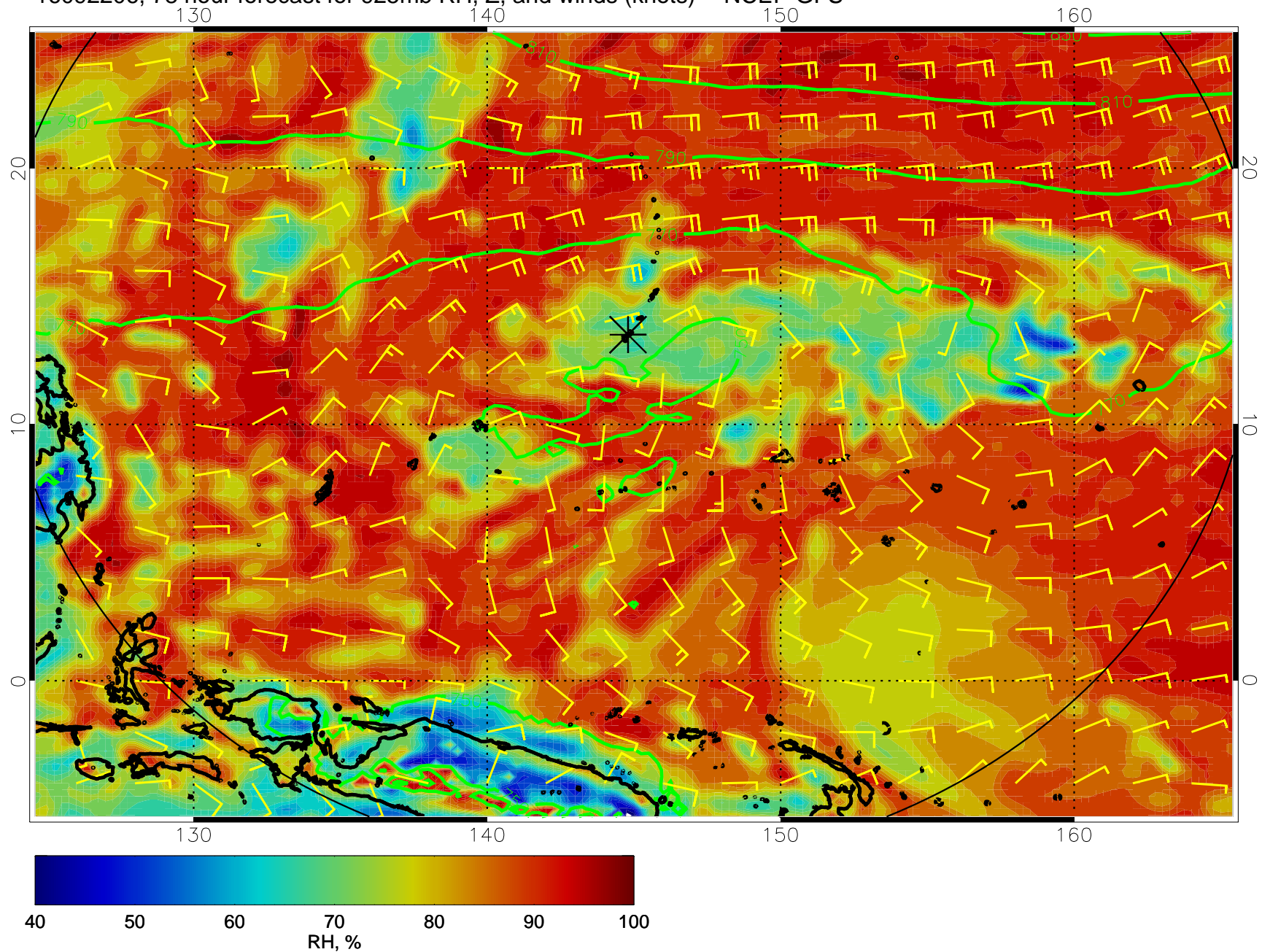
16092206, 78 hour forecast for 925mb RH, Z, and winds (knots) -- NCEP GFS
