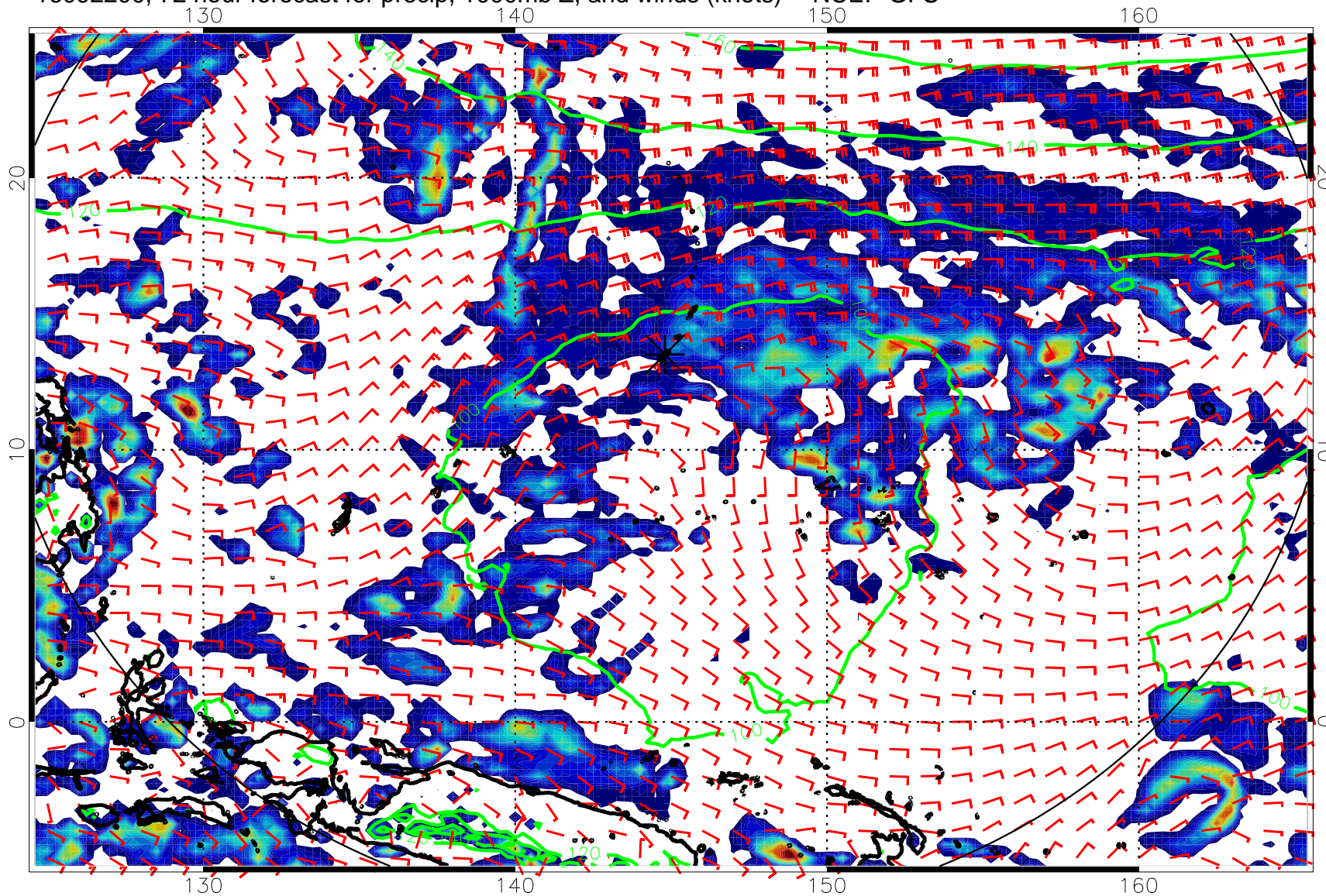
16092200, 72 hour forecast for precip, 1000mb Z, and winds (knots) -- NCEP GFS
