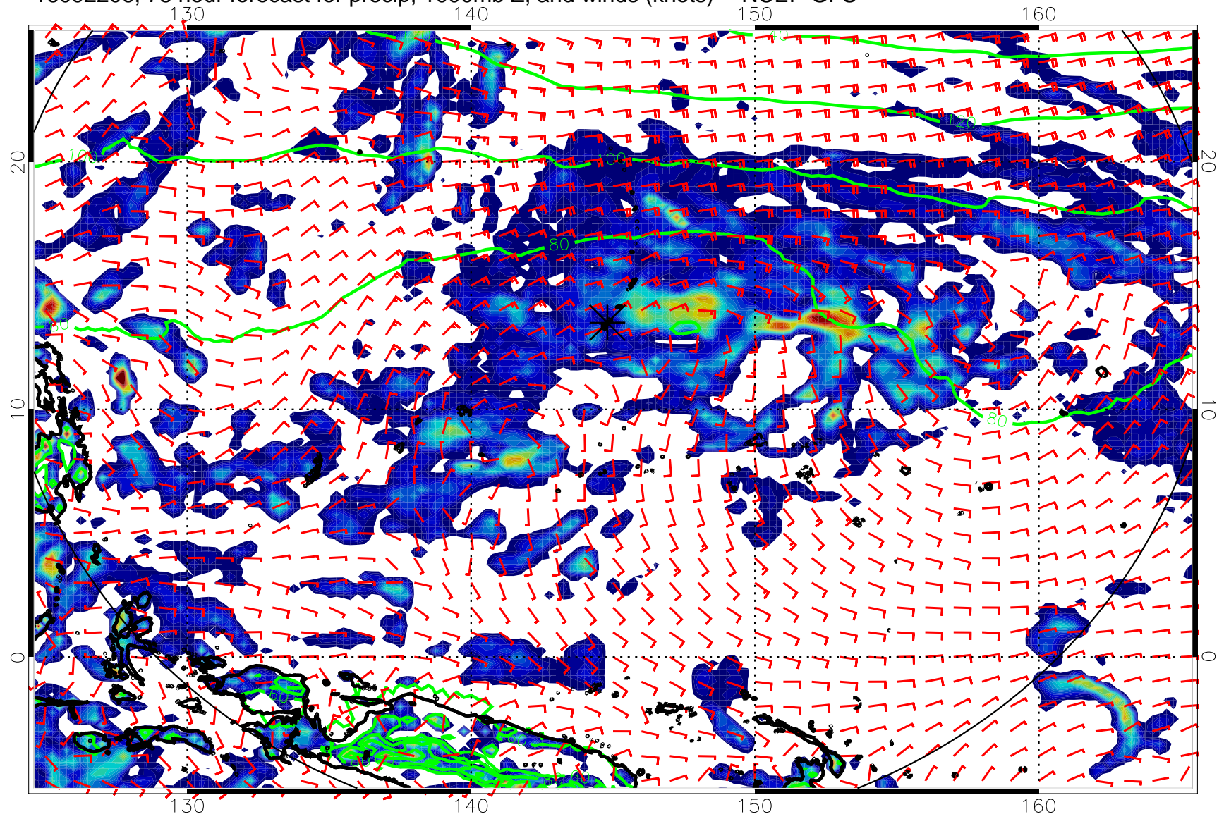
16092206, 78 hour forecast for precip, 1000mb Z, and winds (knots) -- NCEP GFS
