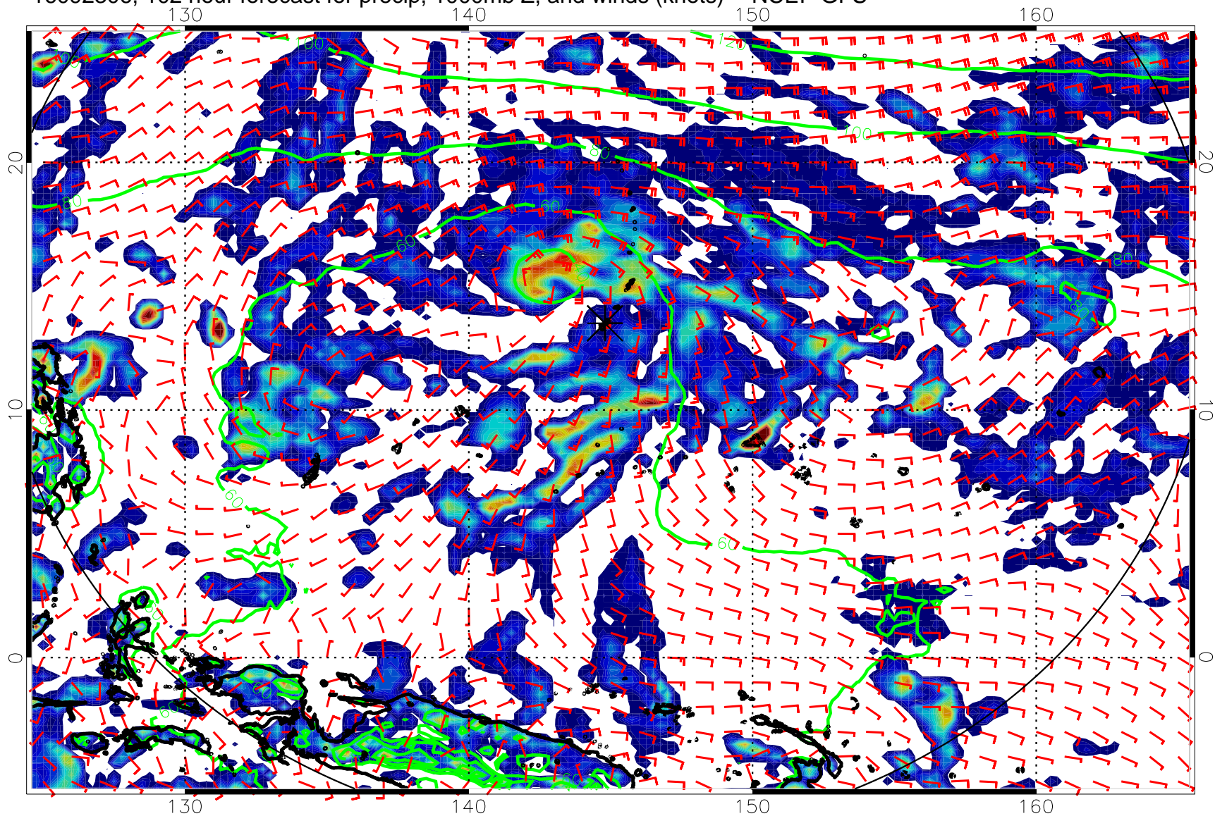
16092306, 102 hour forecast for precip, 1000mb Z, and winds (knots) -- NCEP GFS
