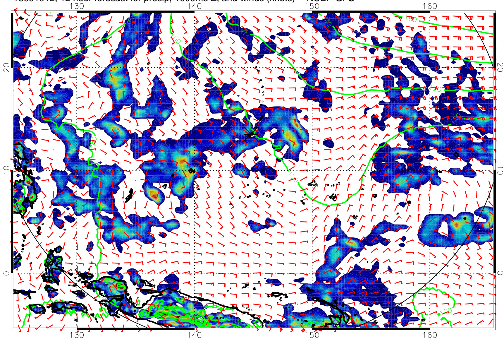
16091912, 12 hour forecast for precip, 1000mb Z, and winds (knots) -- NCEP GFS
