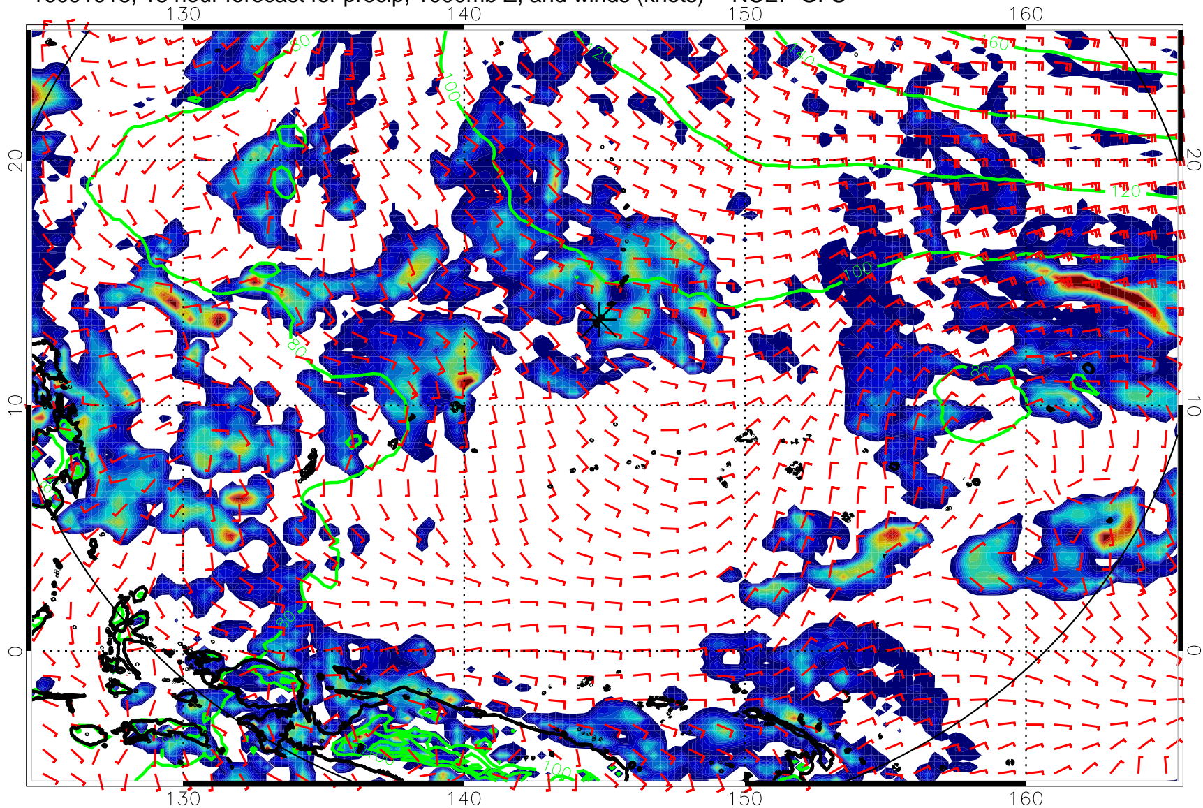
16091918, 18 hour forecast for precip, 1000mb Z, and winds (knots) -- NCEP GFS
