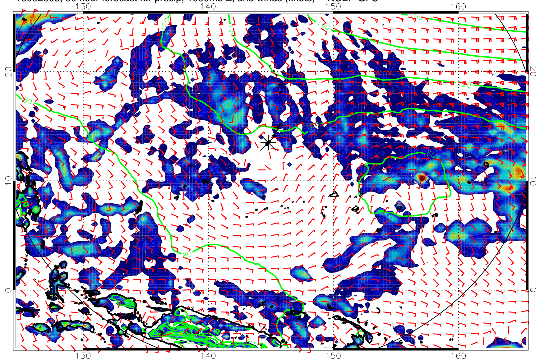
16092006, 30 hour forecast for precip, 1000mb Z, and winds (knots) -- NCEP GFS
