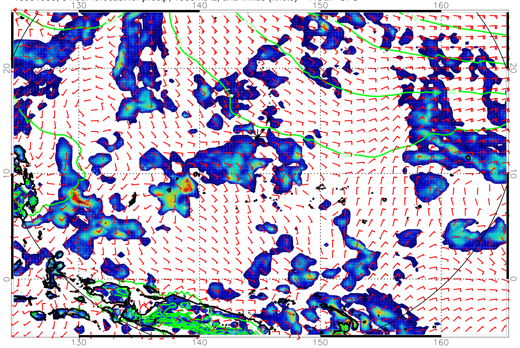
16091906, 6 hour forecast for precip, 1000mb Z, and winds (knots) -- NCEP GFS
