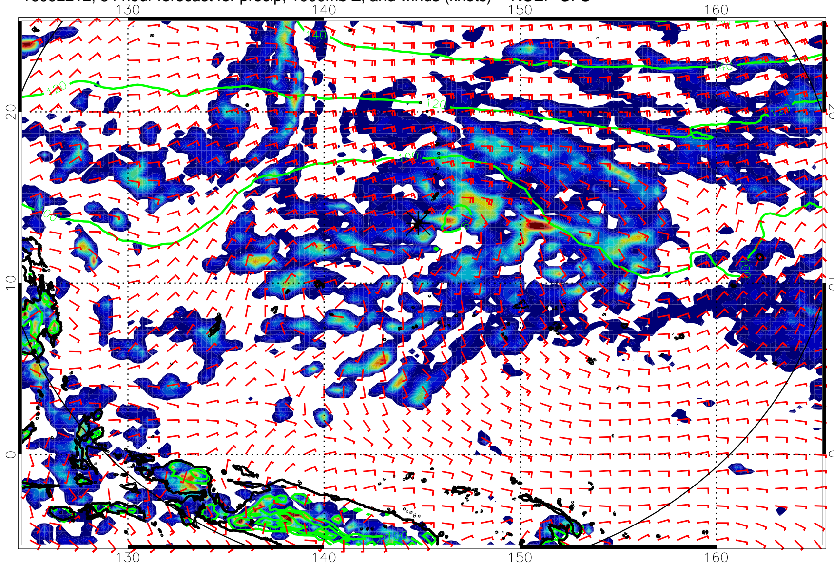
16092212, 84 hour forecast for precip, 1000mb Z, and winds (knots) -- NCEP GFS
