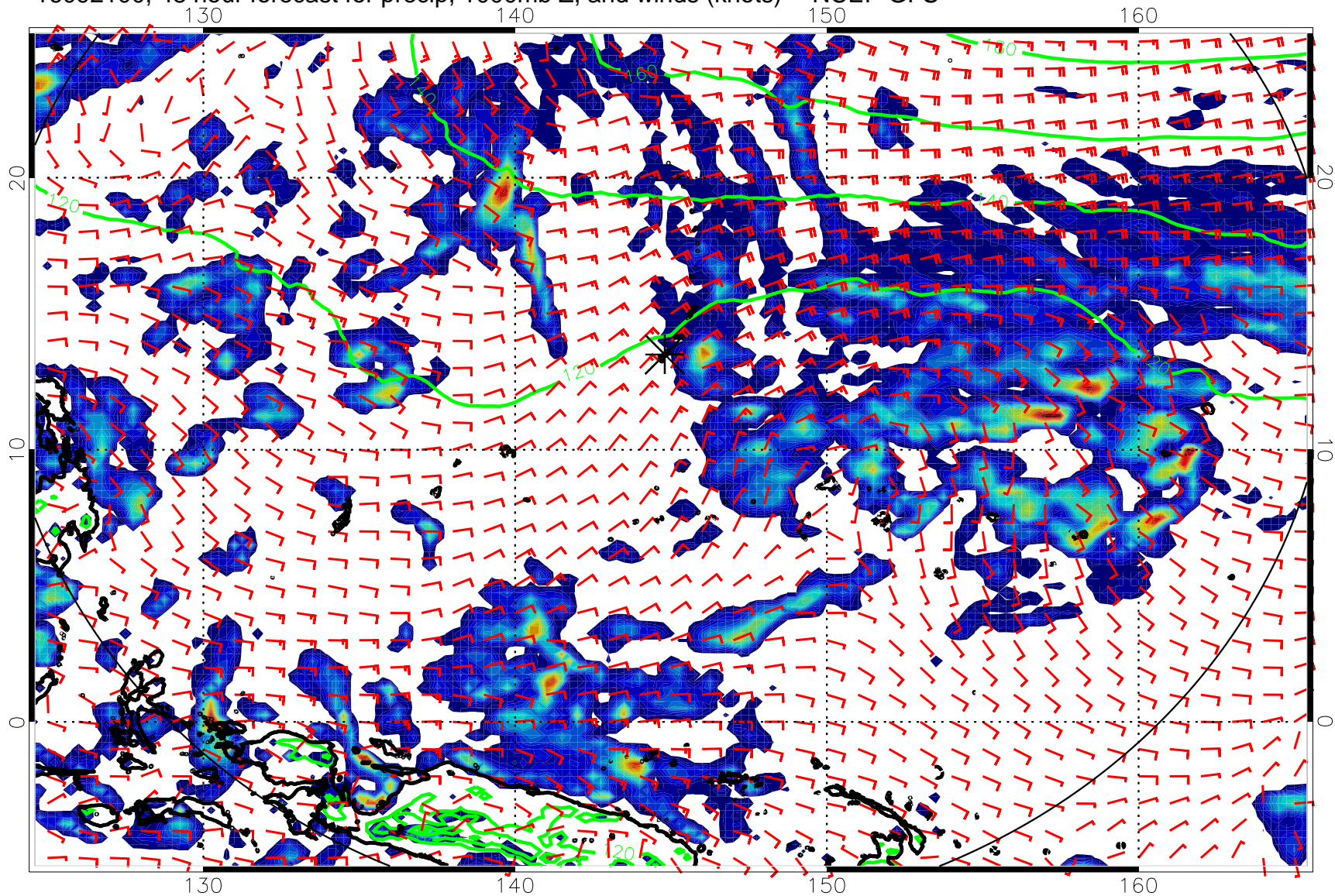
16092100, 48 hour forecast for precip, 1000mb Z, and winds (knots) -- NCEP GFS
