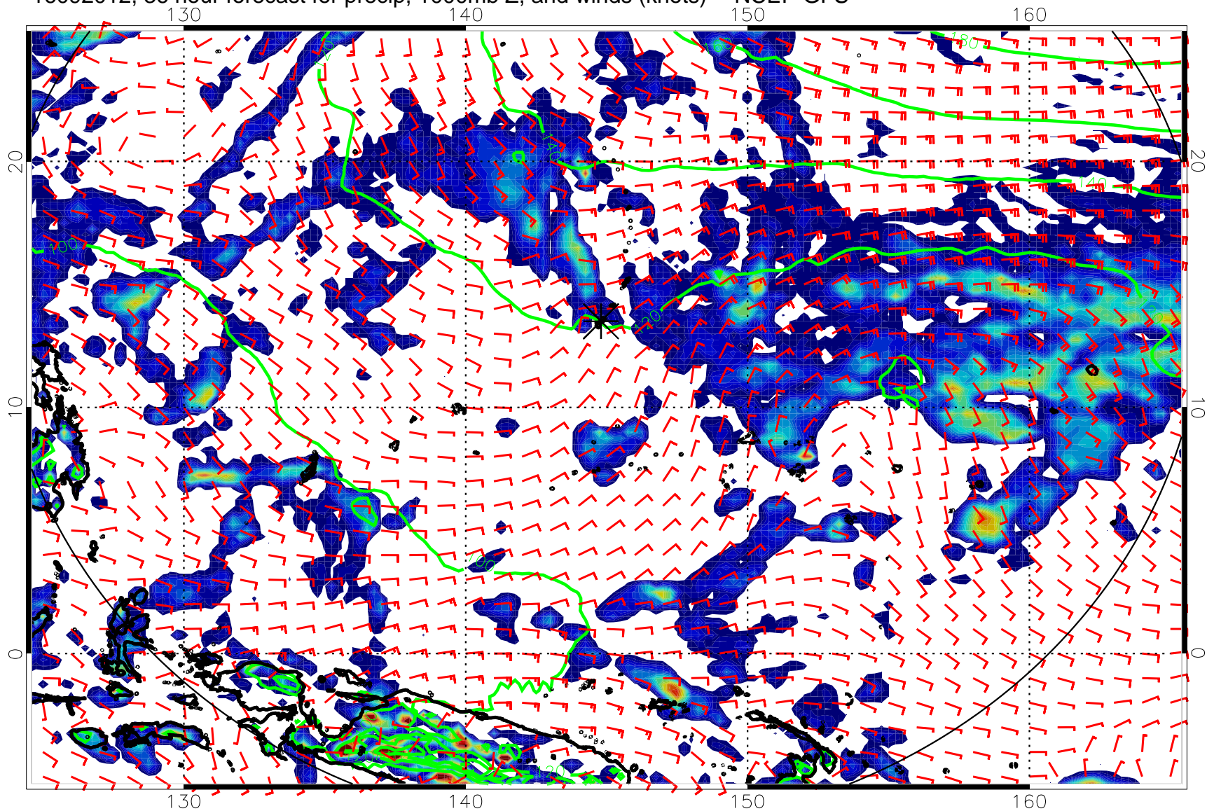
16092012, 36 hour forecast for precip, 1000mb Z, and winds (knots) -- NCEP GFS
