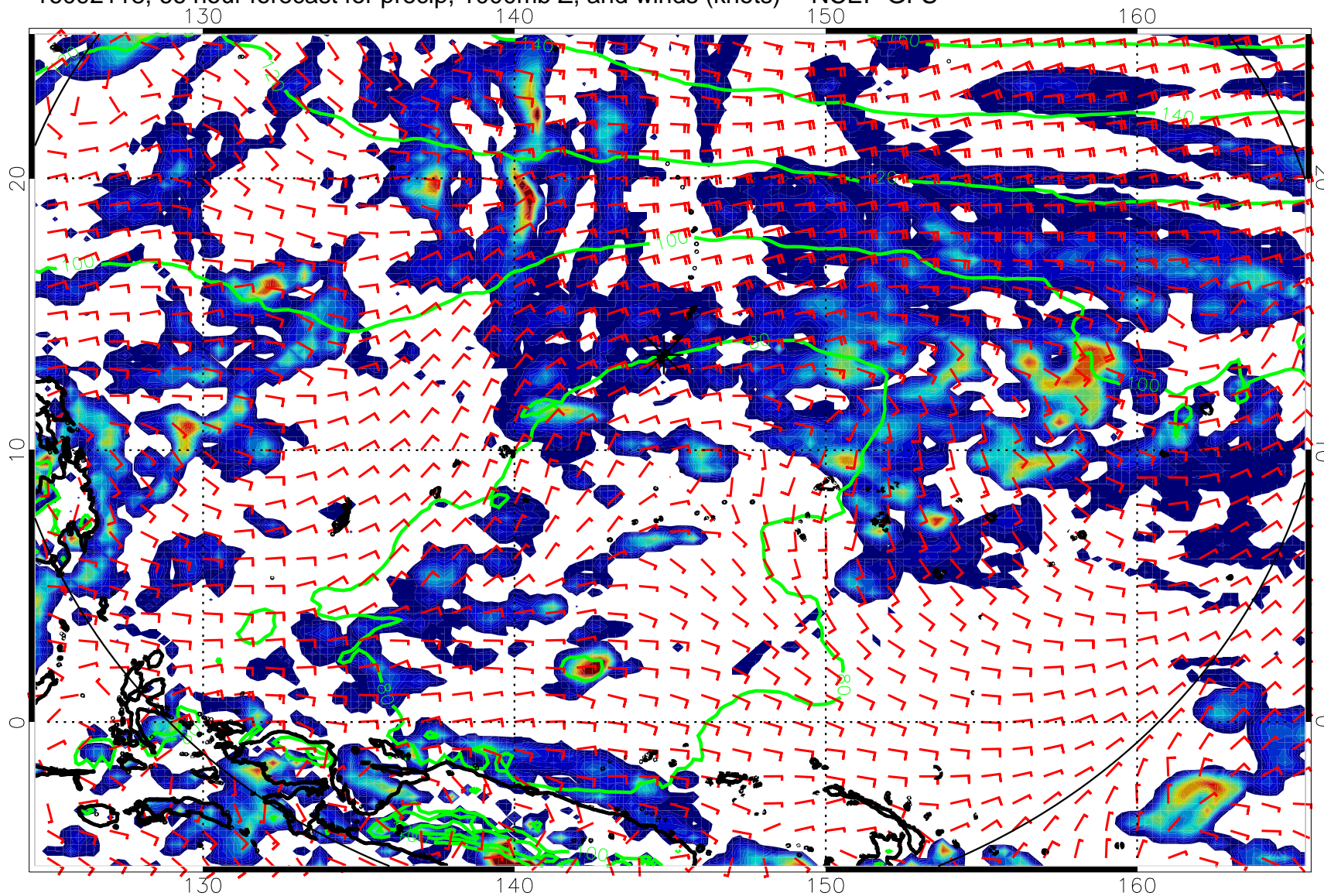
16092118, 66 hour forecast for precip, 1000mb Z, and winds (knots) -- NCEP GFS
