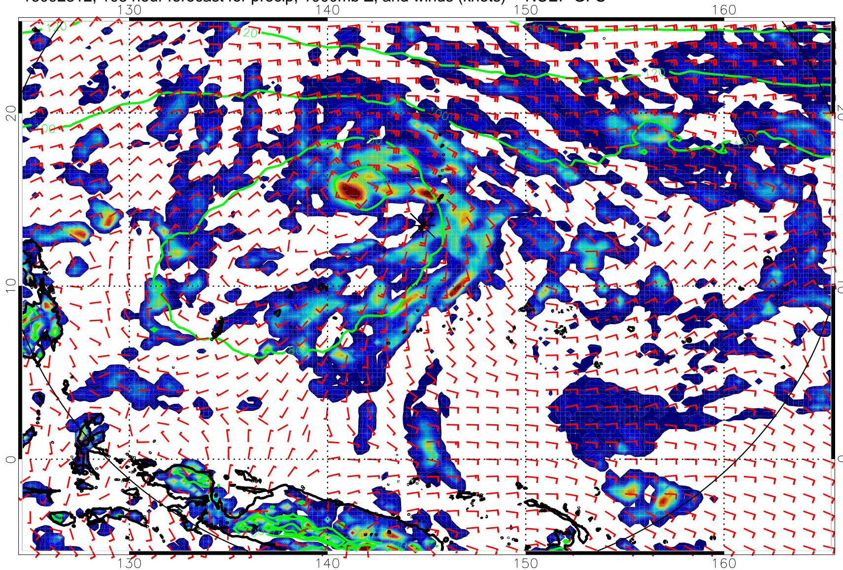
16092312, 108 hour forecast for precip, 1000mb Z, and winds (knots) -- NCEP GFS
