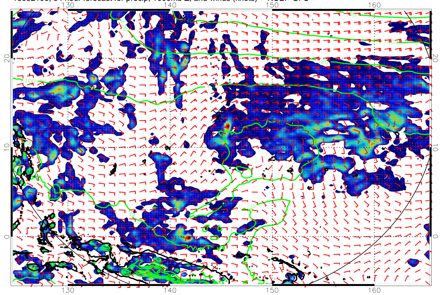
16092106, 54 hour forecast for precip, 1000mb Z, and winds (knots) -- NCEP GFS
