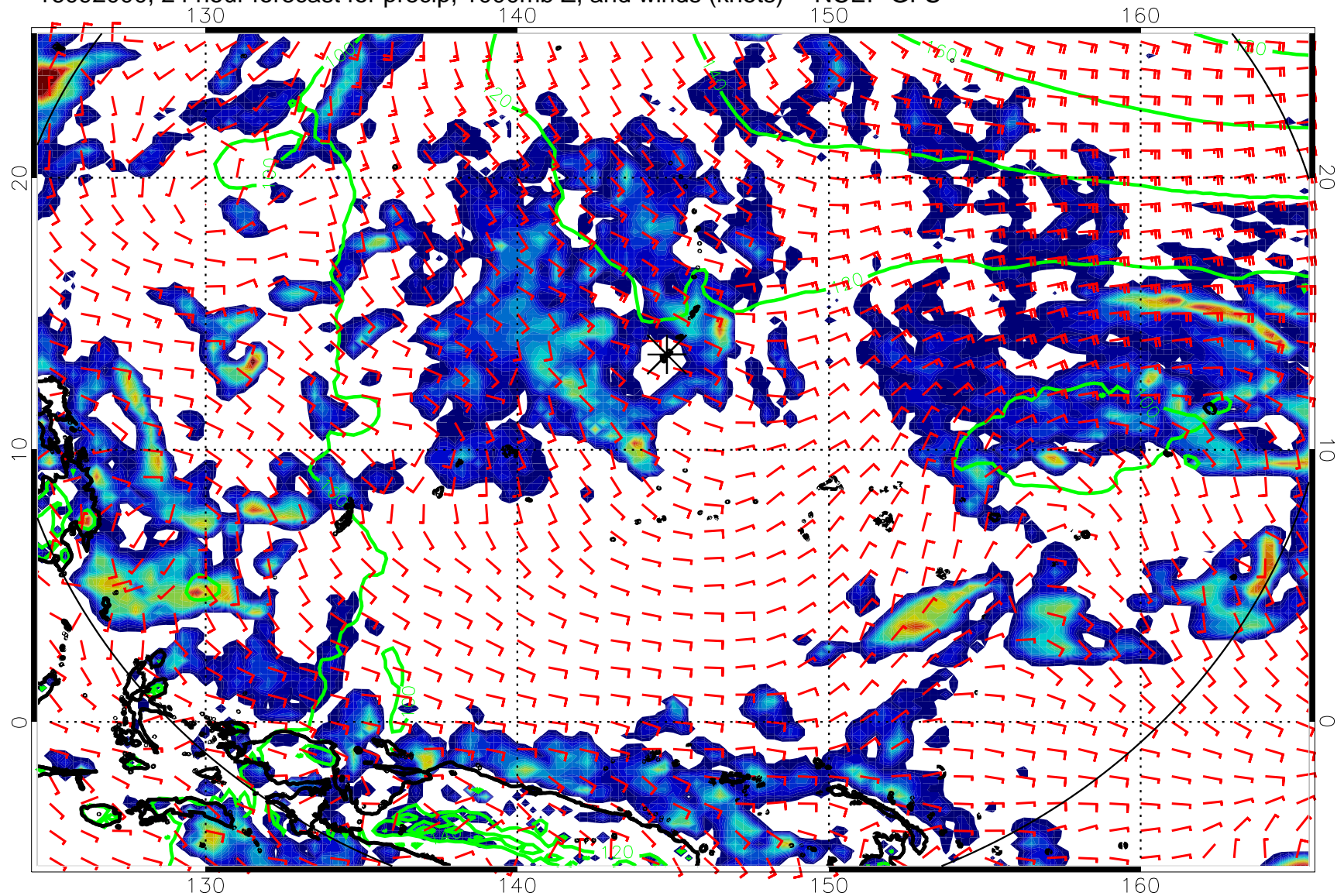
16092000, 24 hour forecast for precip, 1000mb Z, and winds (knots) -- NCEP GFS
