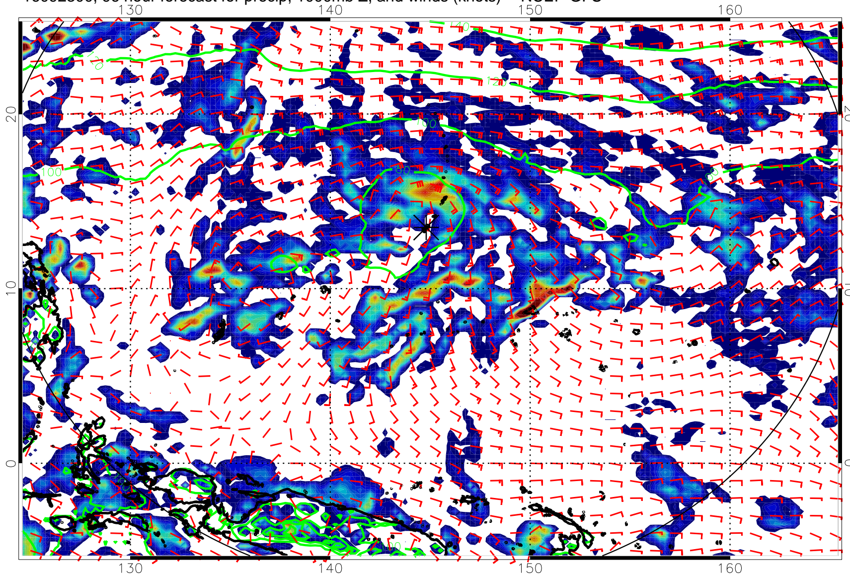
16092300, 96 hour forecast for precip, 1000mb Z, and winds (knots) -- NCEP GFS
