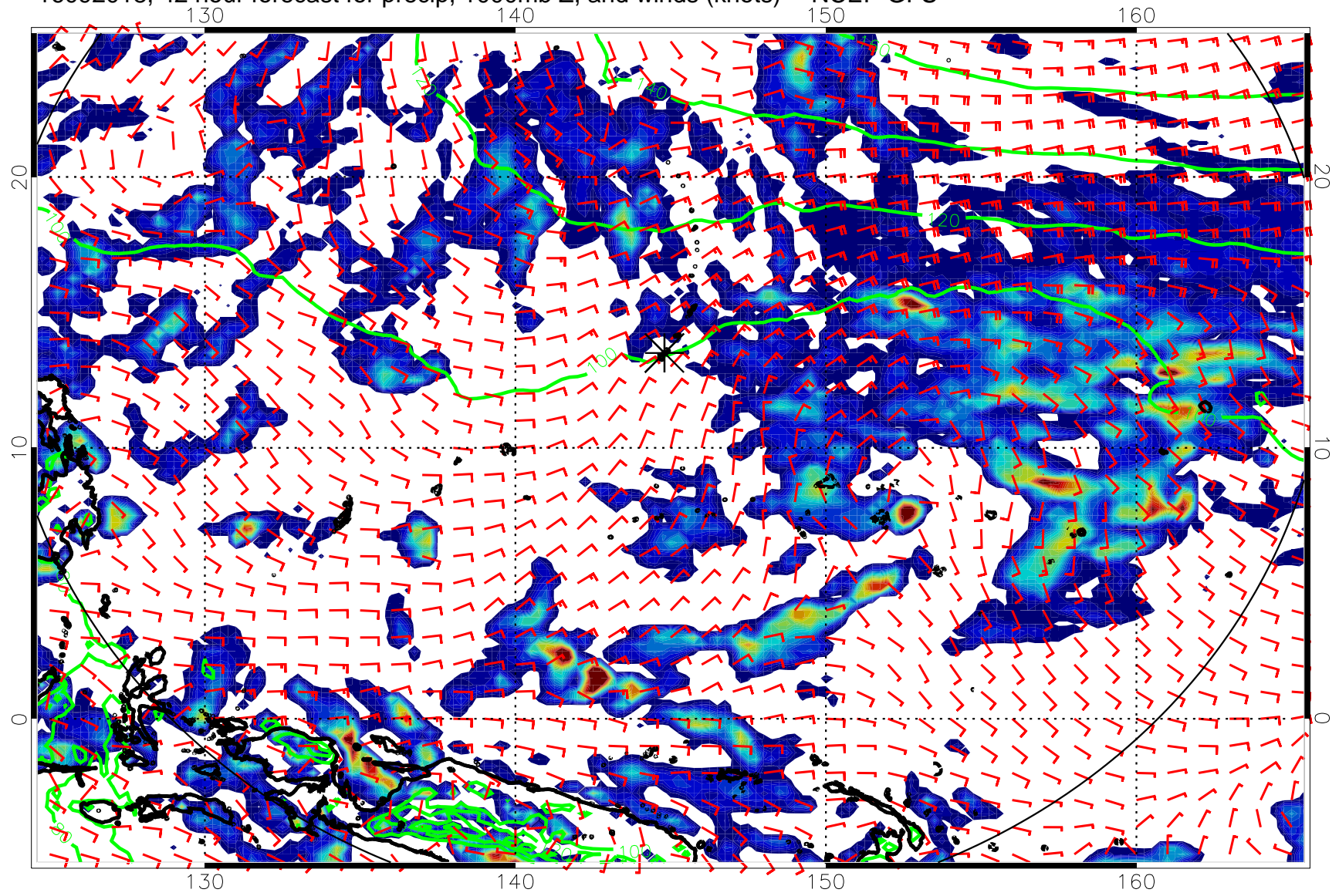
16092018, 42 hour forecast for precip, 1000mb Z, and winds (knots) -- NCEP GFS
