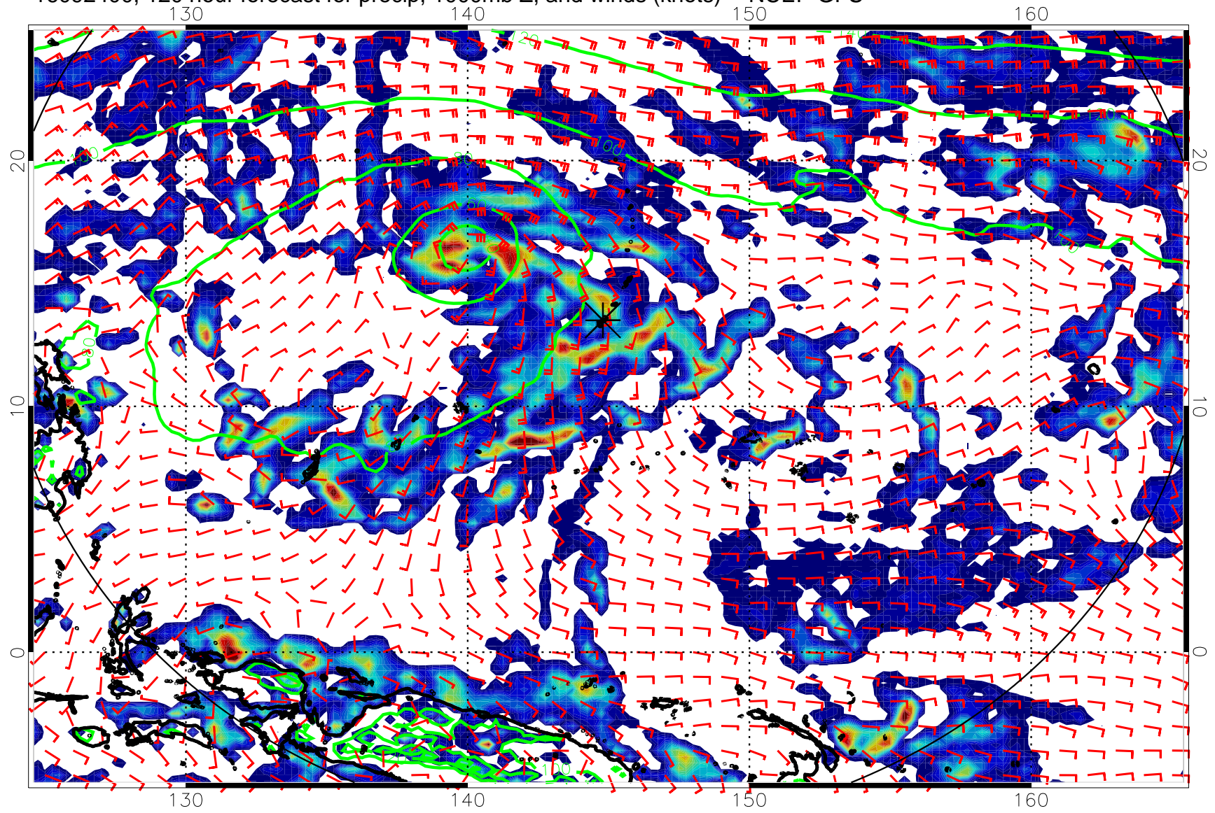
16092400, 120 hour forecast for precip, 1000mb Z, and winds (knots) -- NCEP GFS
