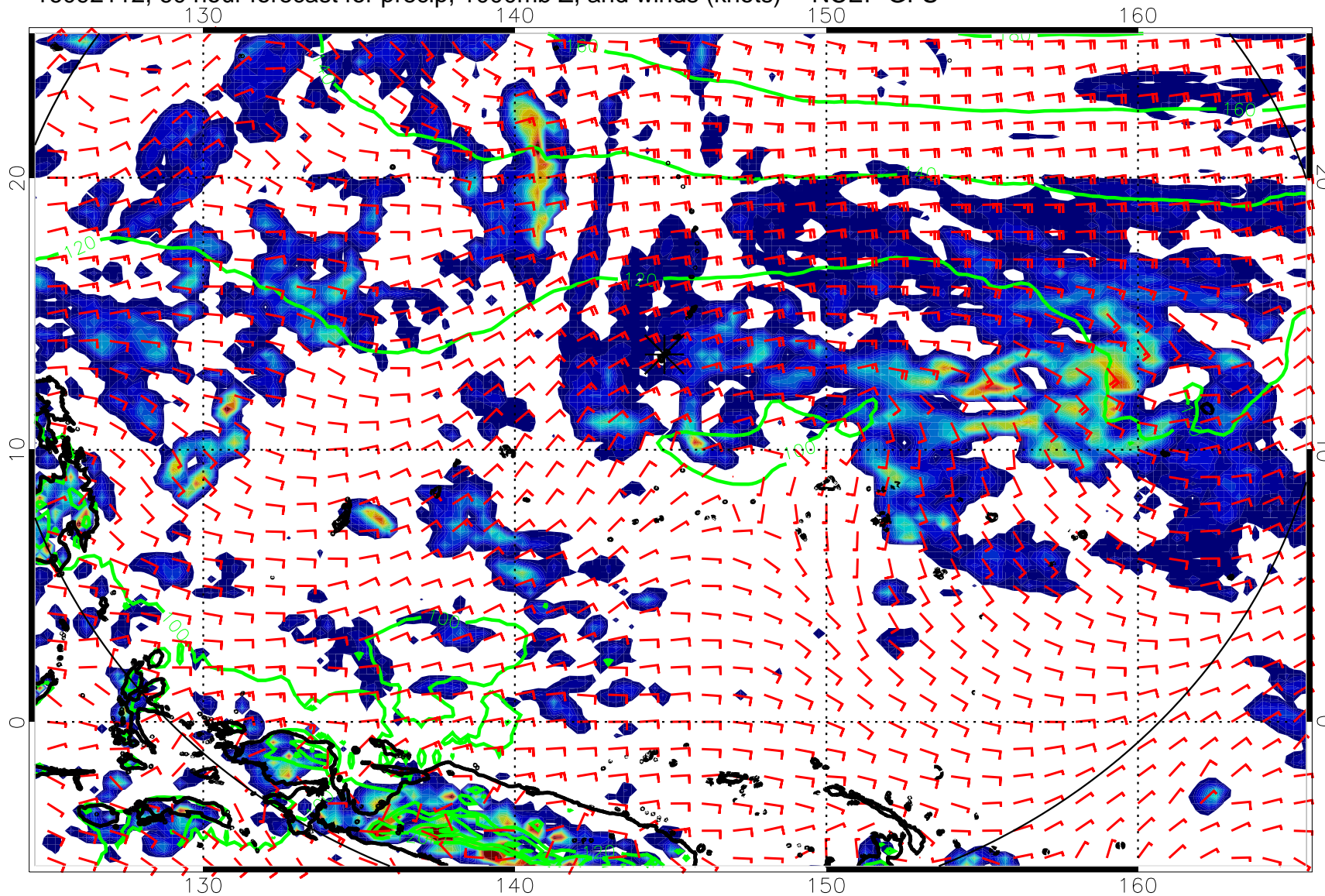
16092112, 60 hour forecast for precip, 1000mb Z, and winds (knots) -- NCEP GFS
