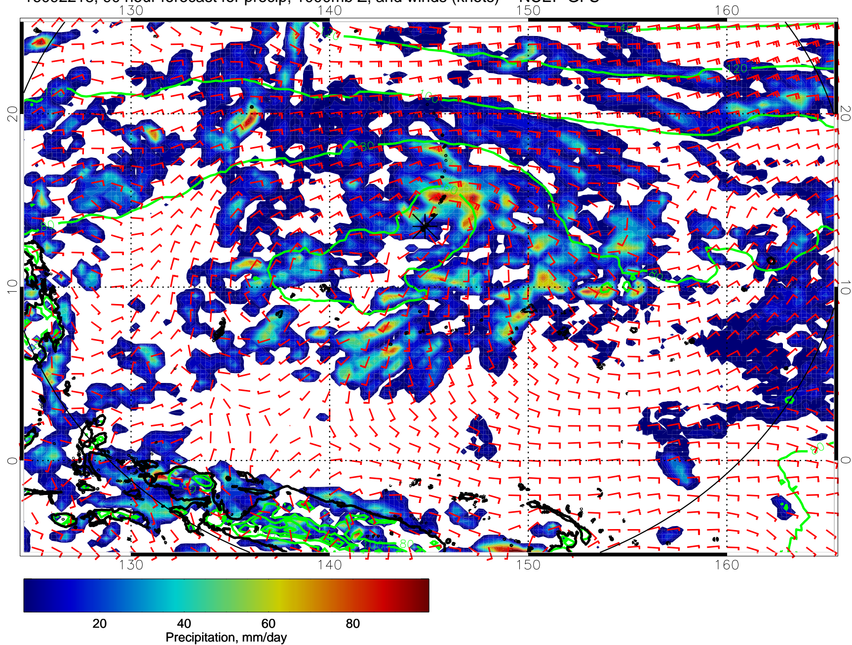
16092218, 90 hour forecast for precip, 1000mb Z, and winds (knots) -- NCEP GFS
