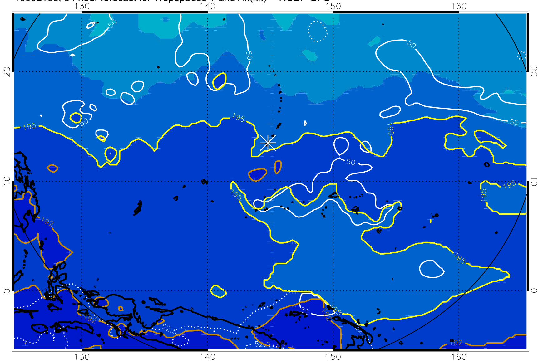
16092106, 54 hour forecast for Tropopause T and Alt(kft) -- NCEP GFS
