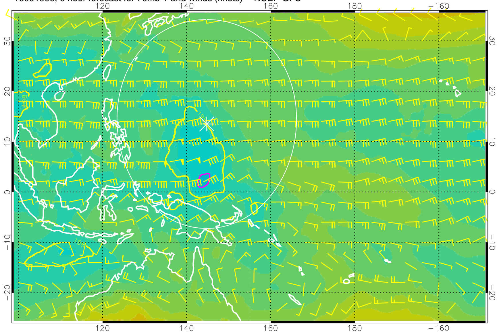
16091906, 6 hour forecast for 70mb T and winds (knots) -- NCEP GFS
