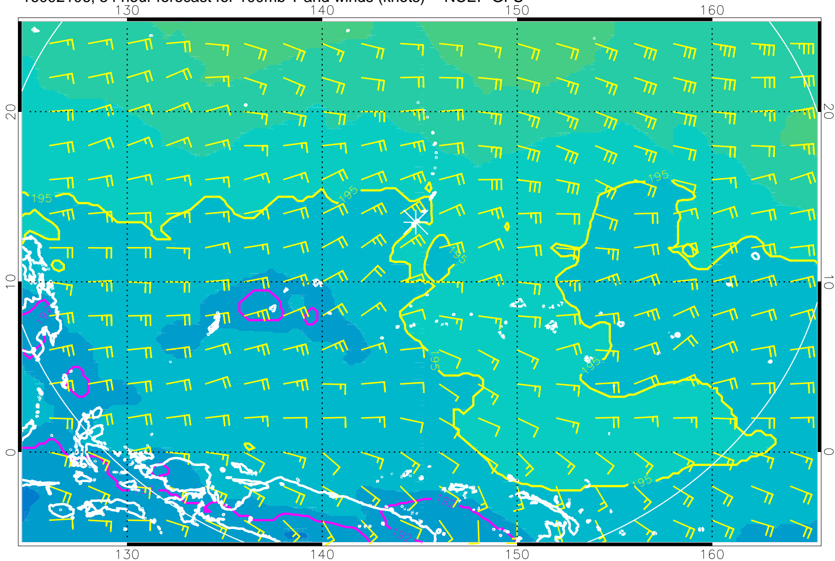
16092106, 54 hour forecast for 100mb T and winds (knots) -- NCEP GFS
