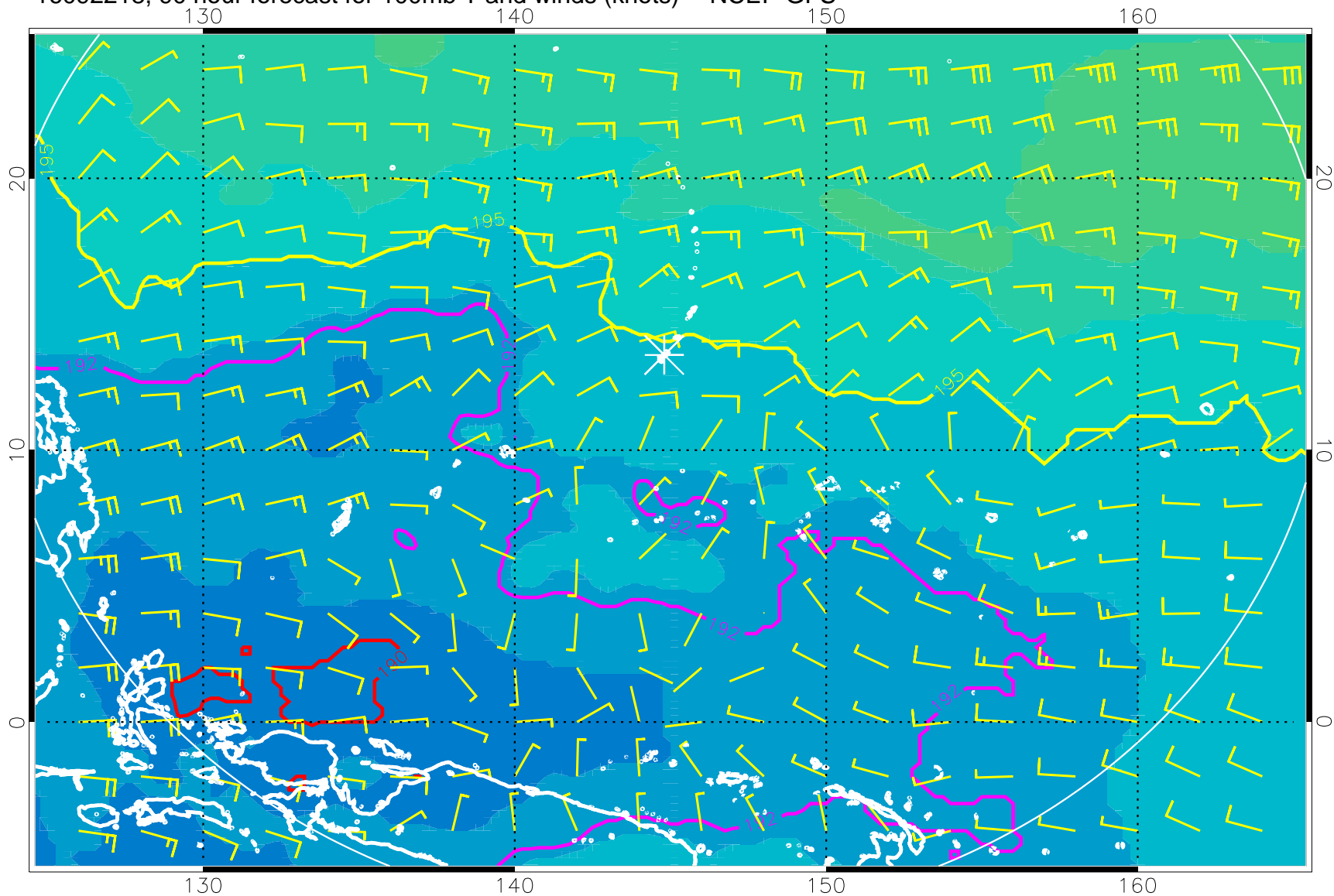
16092218, 90 hour forecast for 100mb T and winds (knots) -- NCEP GFS
