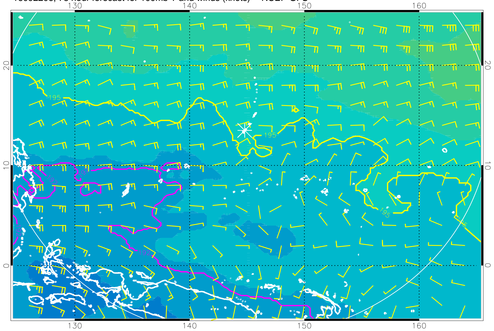
16092206, 78 hour forecast for 100mb T and winds (knots) -- NCEP GFS
