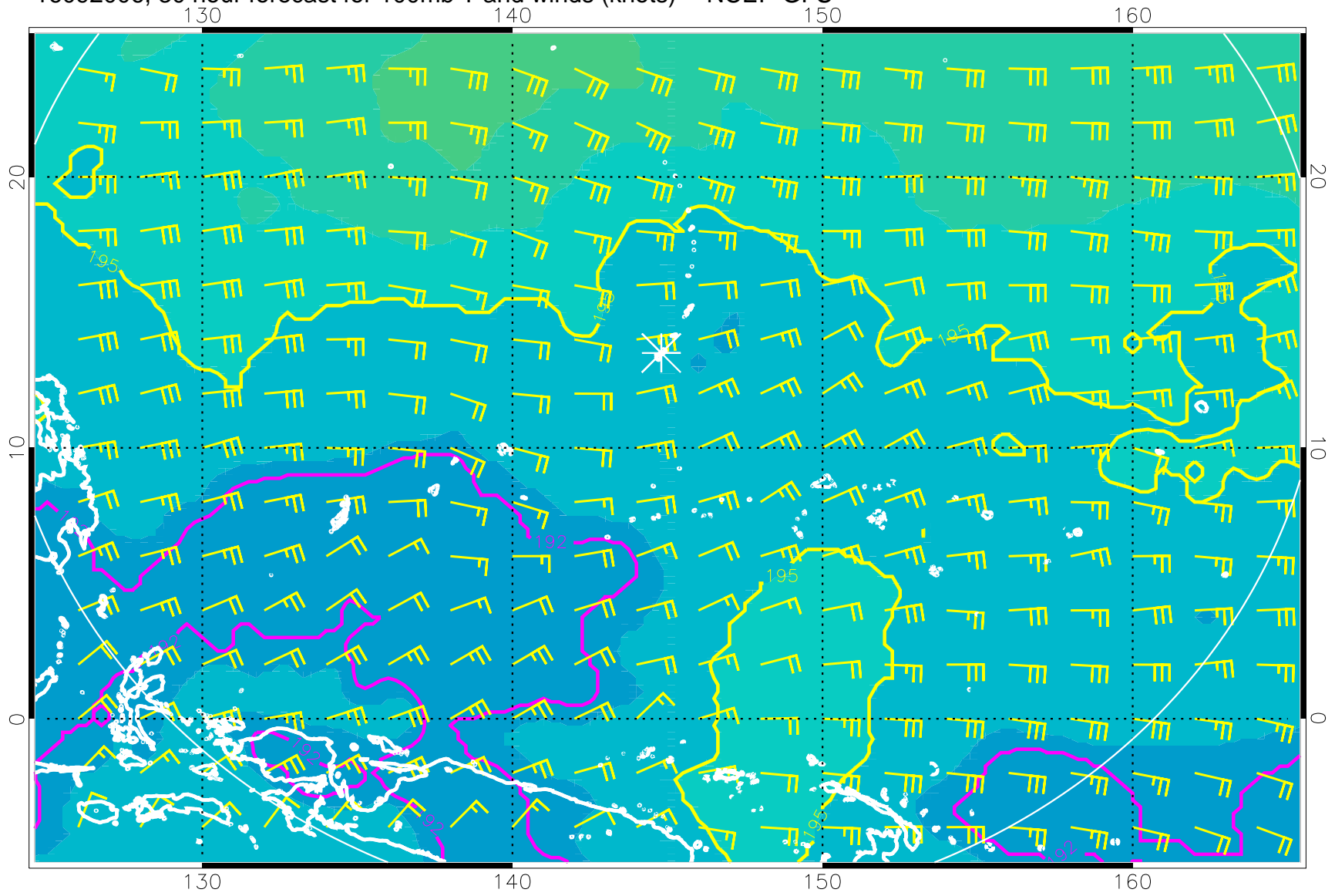
16092006, 30 hour forecast for 100mb T and winds (knots) -- NCEP GFS
