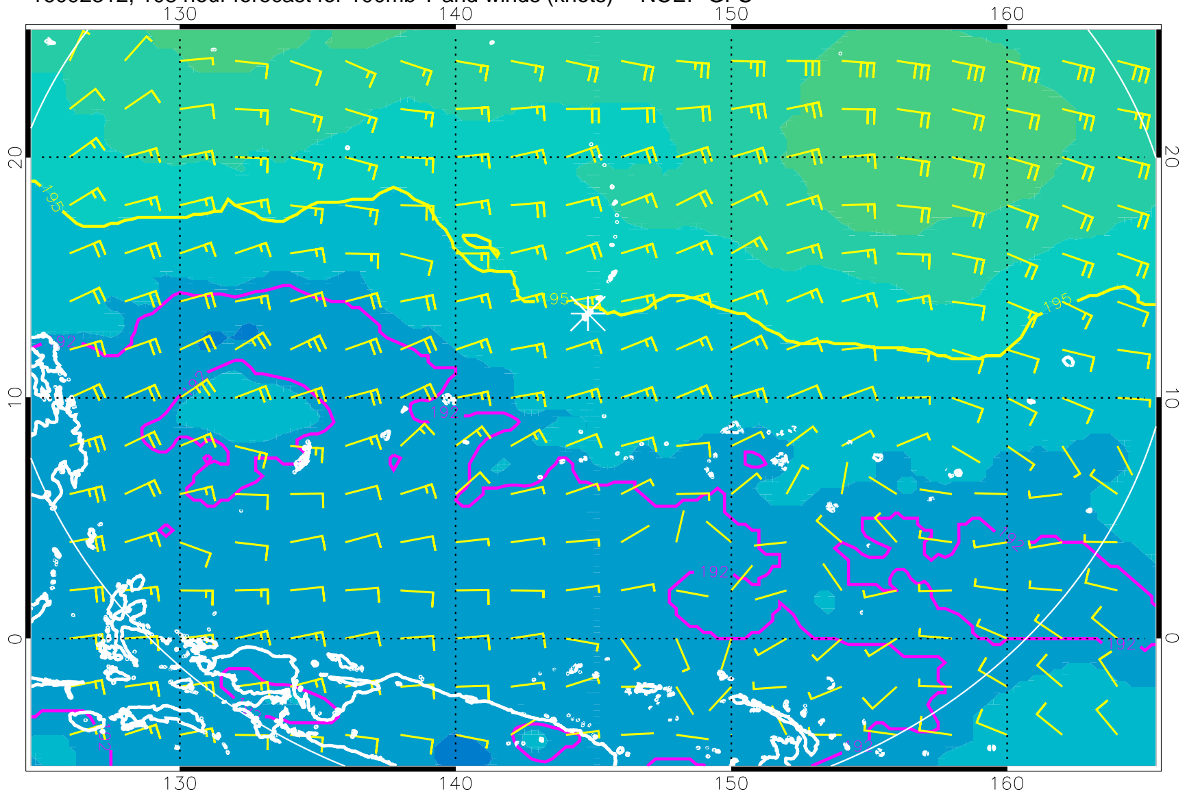
16092312, 108 hour forecast for 100mb T and winds (knots) -- NCEP GFS
