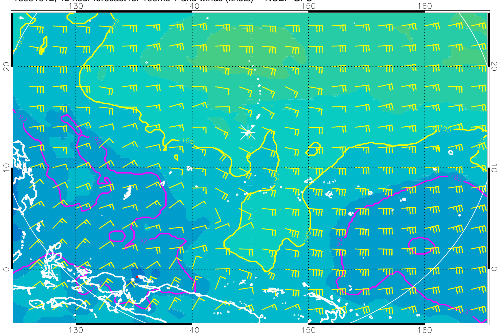
16091912, 12 hour forecast for 100mb T and winds (knots) -- NCEP GFS
