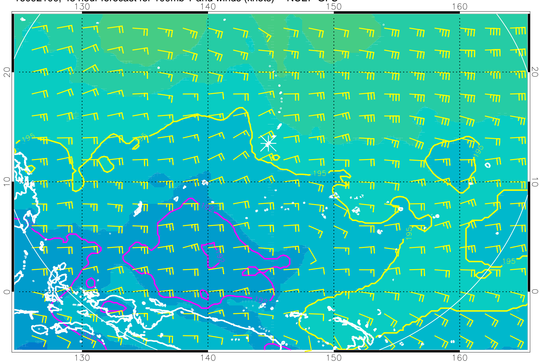
16092100, 48 hour forecast for 100mb T and winds (knots) -- NCEP GFS
