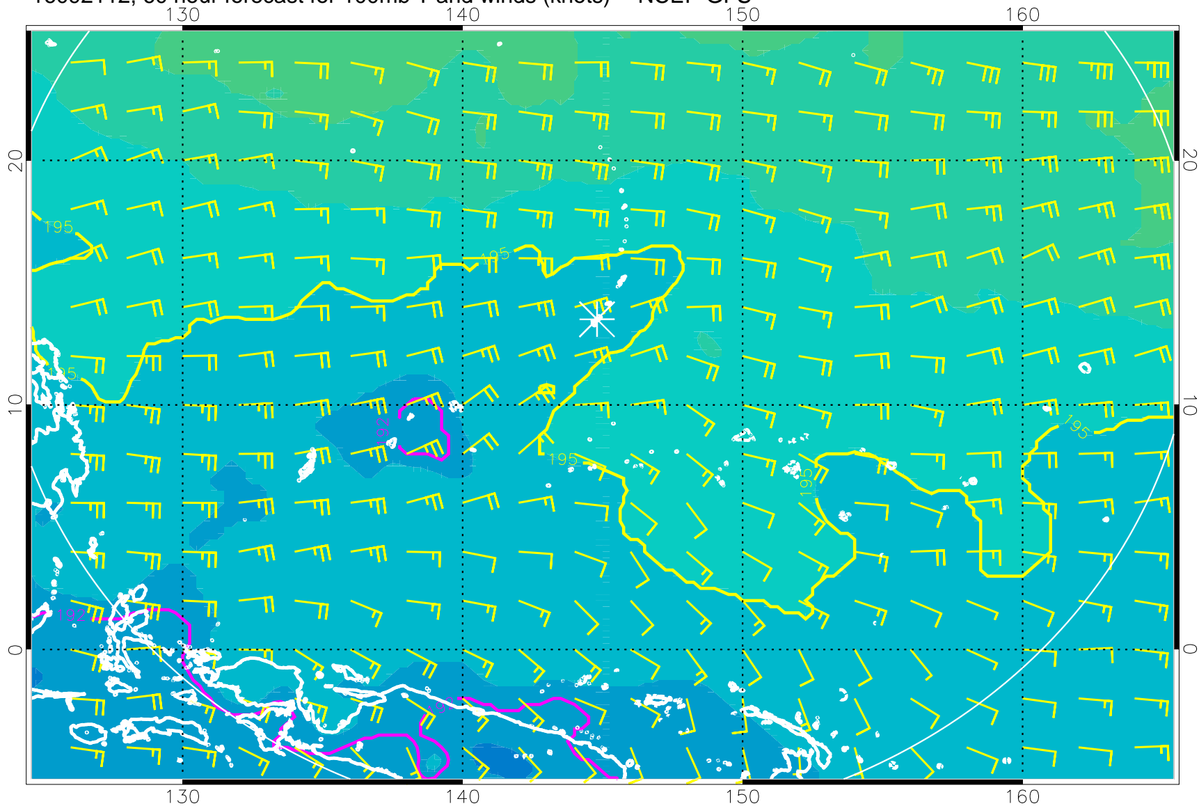
16092112, 60 hour forecast for 100mb T and winds (knots) -- NCEP GFS
