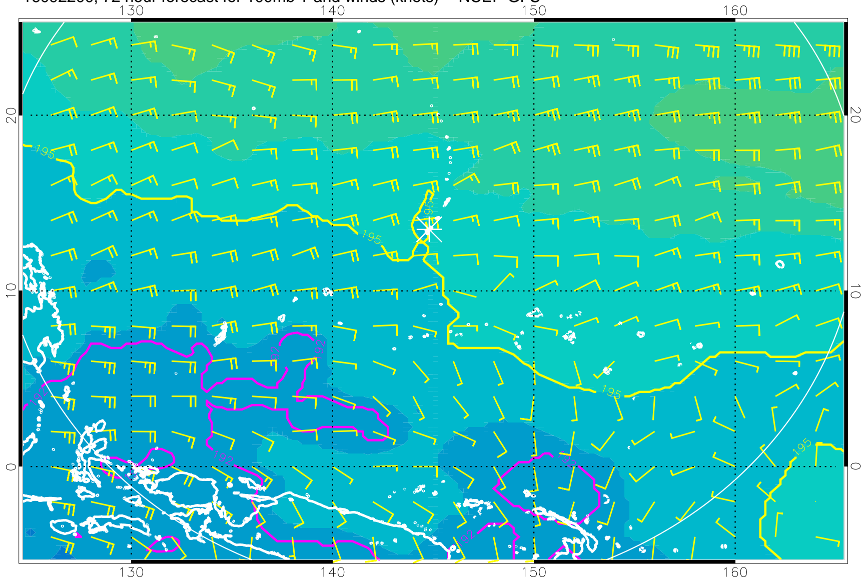
16092200, 72 hour forecast for 100mb T and winds (knots) -- NCEP GFS
