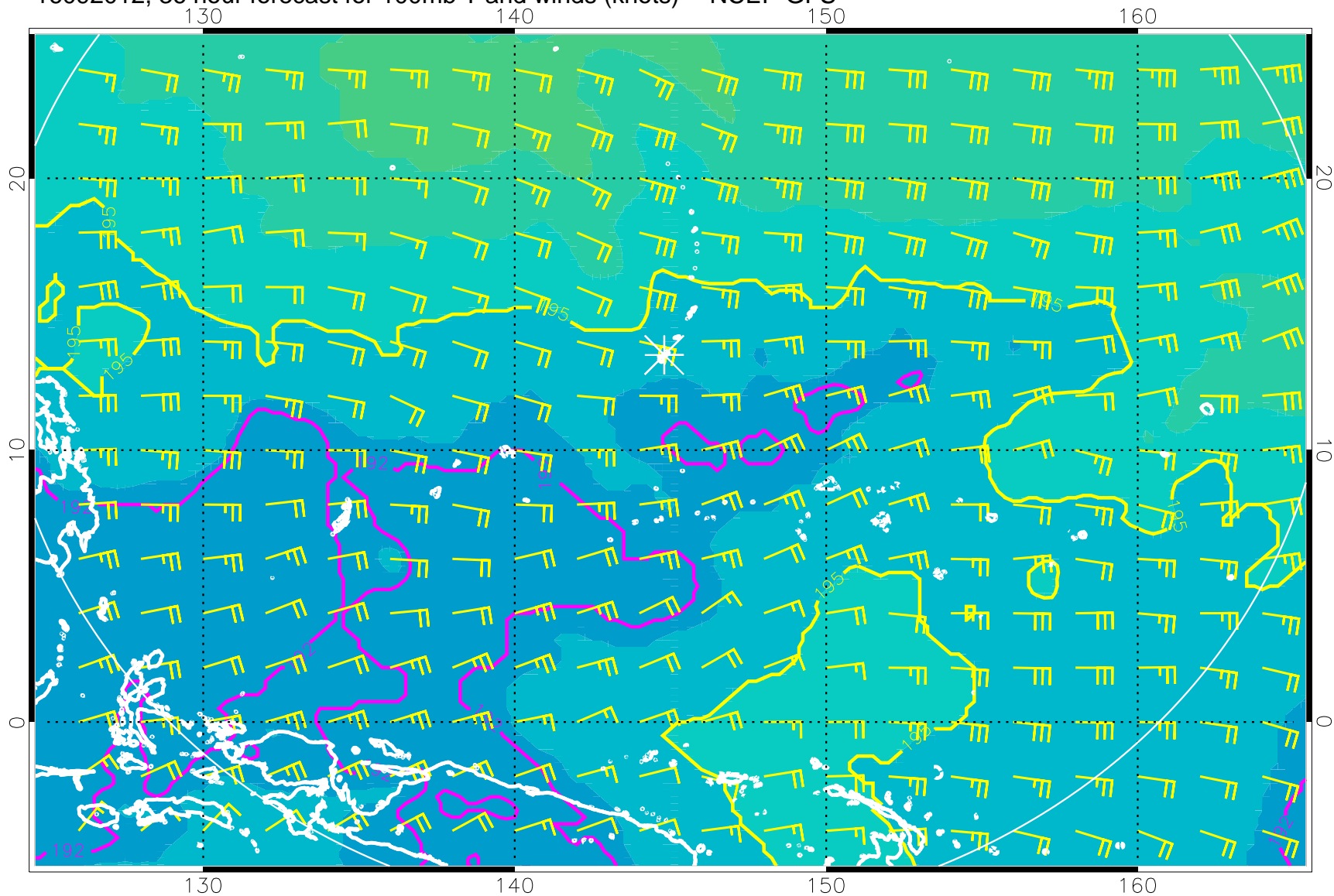
16092012, 36 hour forecast for 100mb T and winds (knots) -- NCEP GFS
