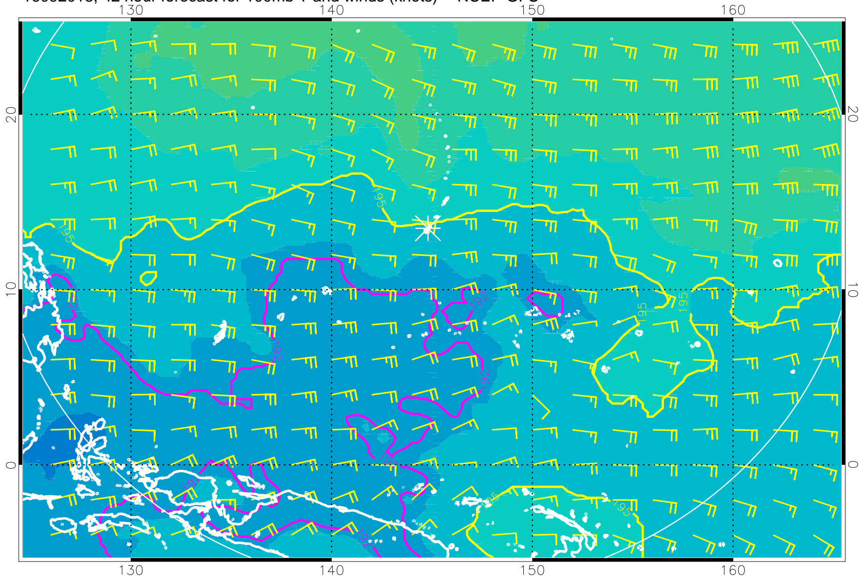
16092018, 42 hour forecast for 100mb T and winds (knots) -- NCEP GFS
