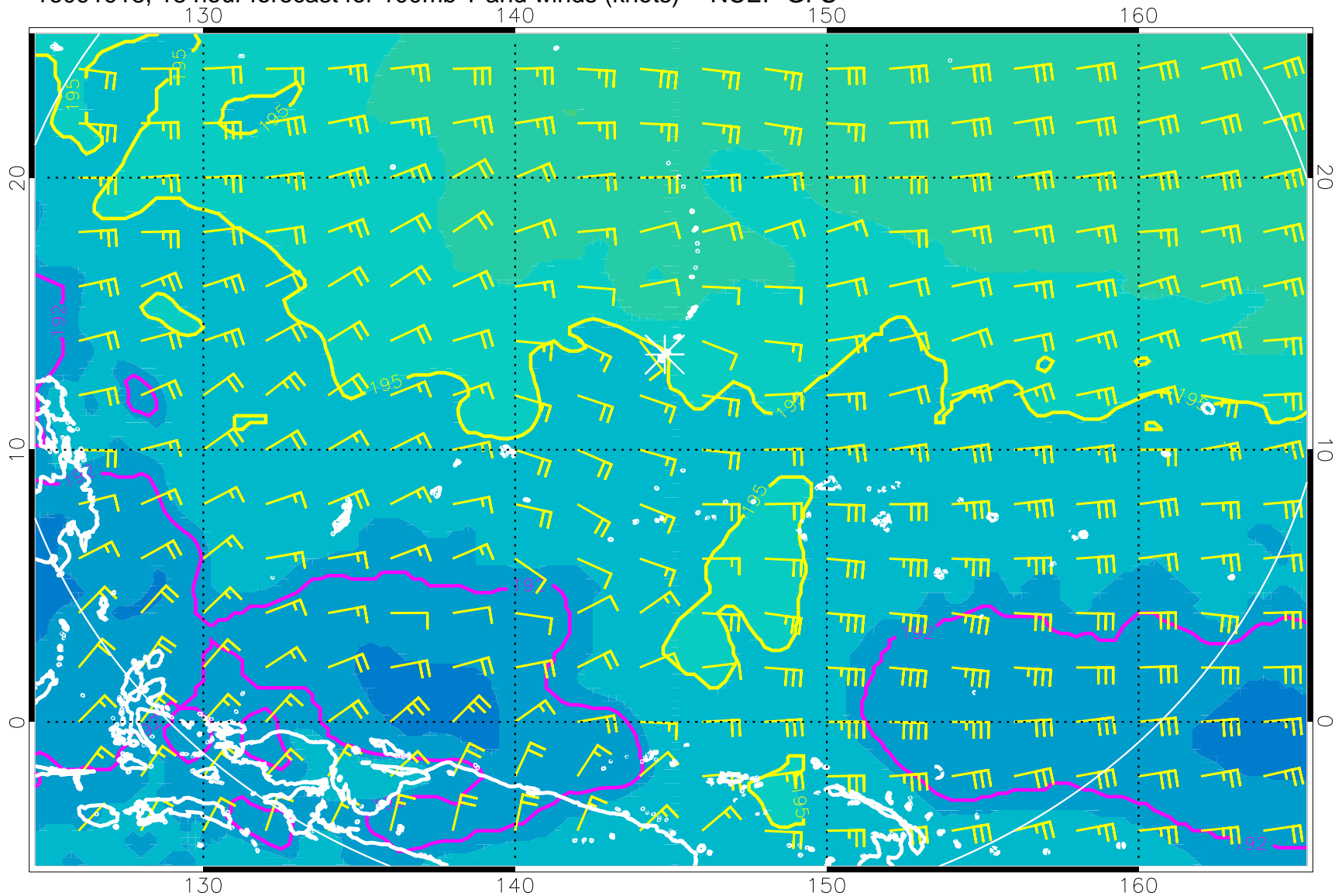
16091918, 18 hour forecast for 100mb T and winds (knots) -- NCEP GFS
