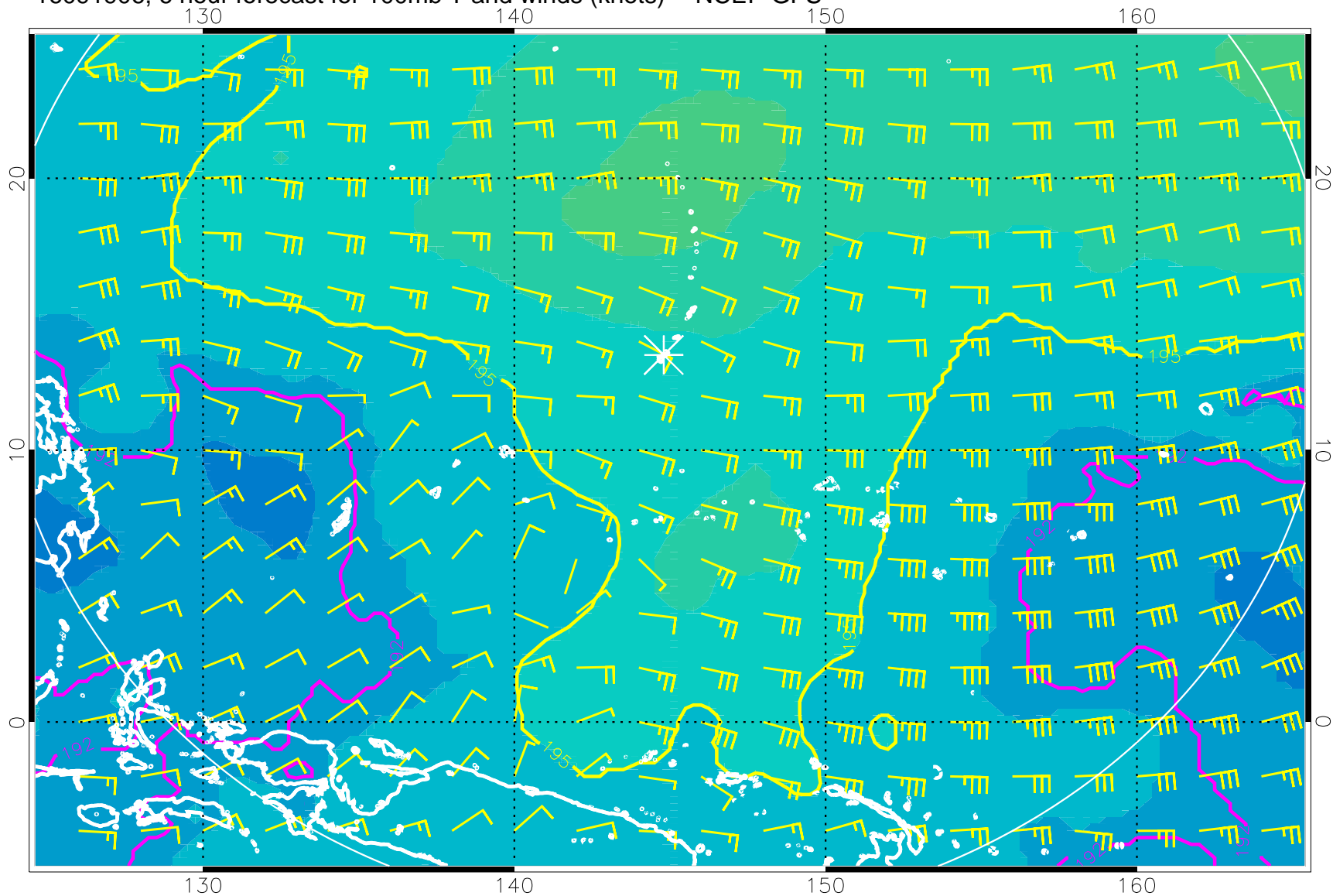
16091906, 6 hour forecast for 100mb T and winds (knots) -- NCEP GFS
