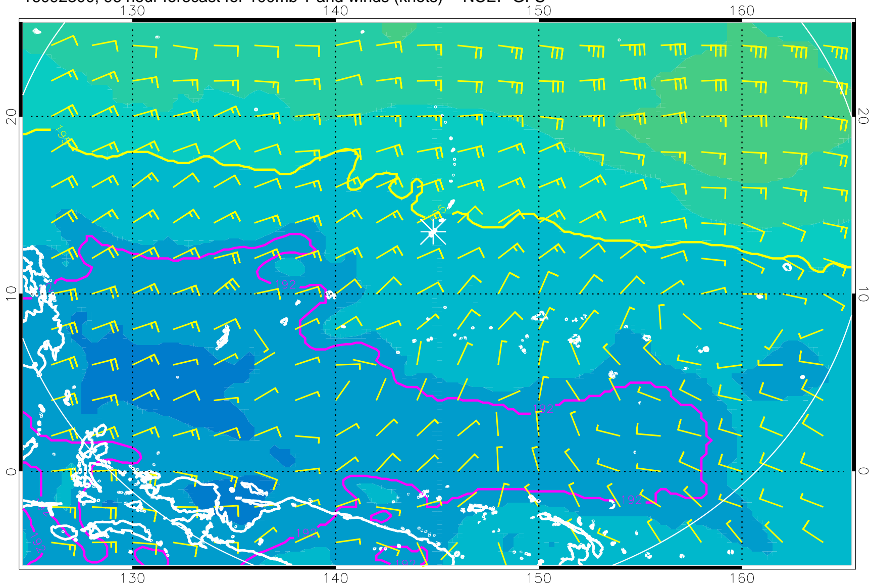
16092300, 96 hour forecast for 100mb T and winds (knots) -- NCEP GFS
