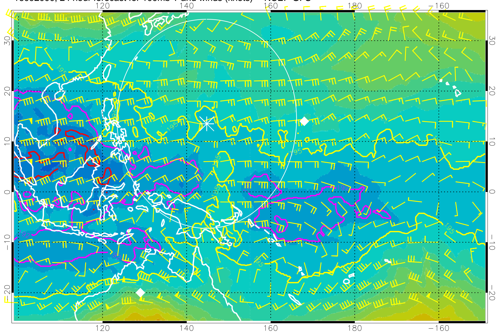
16092000, 24 hour forecast for 100mb T and winds (knots) -- NCEP GFS
