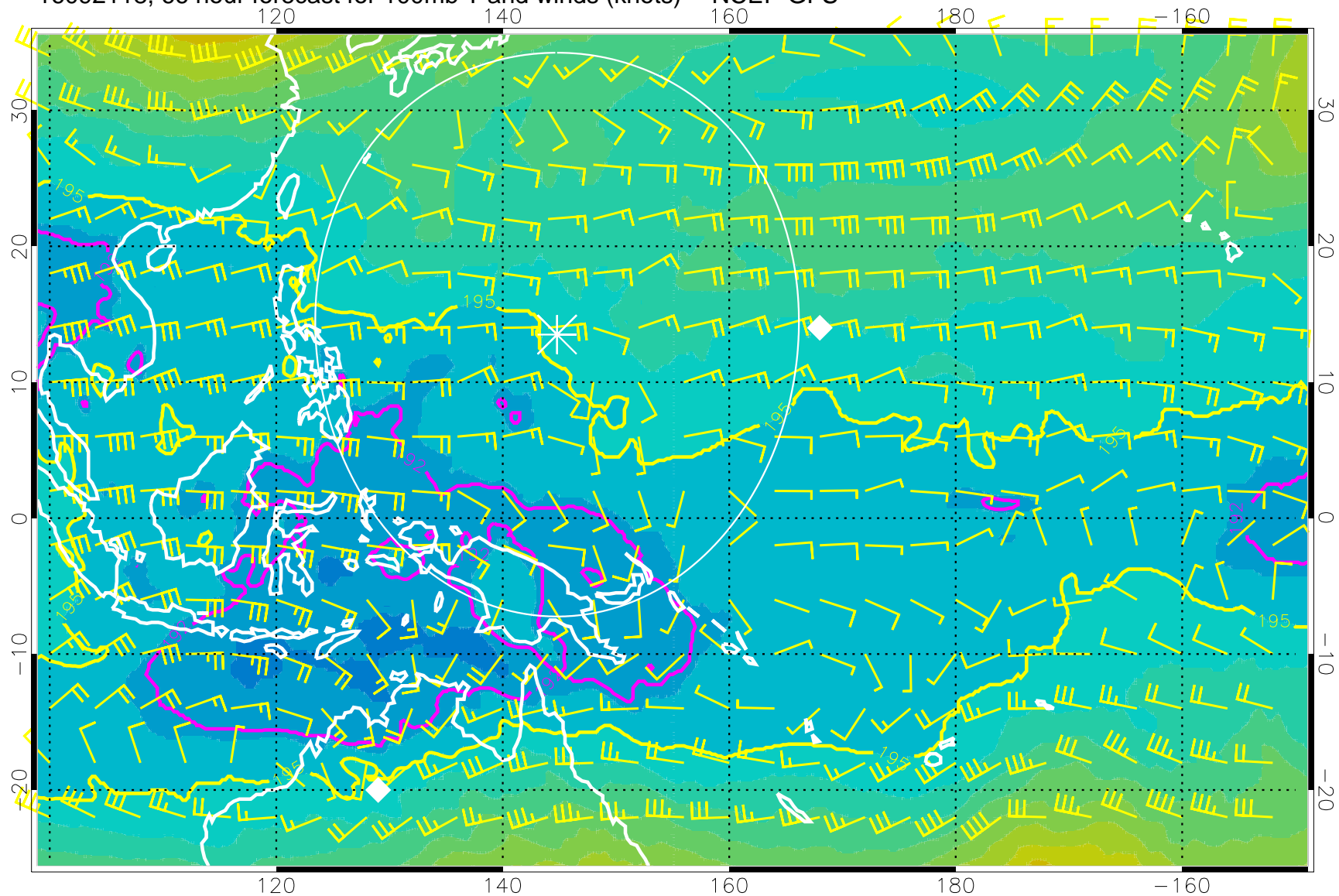
16092118, 66 hour forecast for 100mb T and winds (knots) -- NCEP GFS
