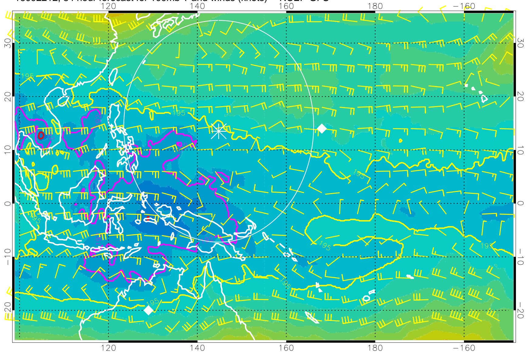
16092212, 84 hour forecast for 100mb T and winds (knots) -- NCEP GFS
