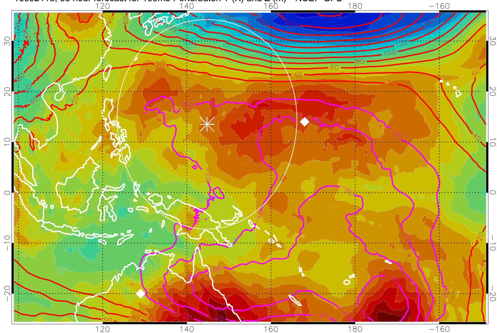
16092118, 66 hour forecast for 100mb Perturbaton T (K) and Z (m)-- NCEP GFS
