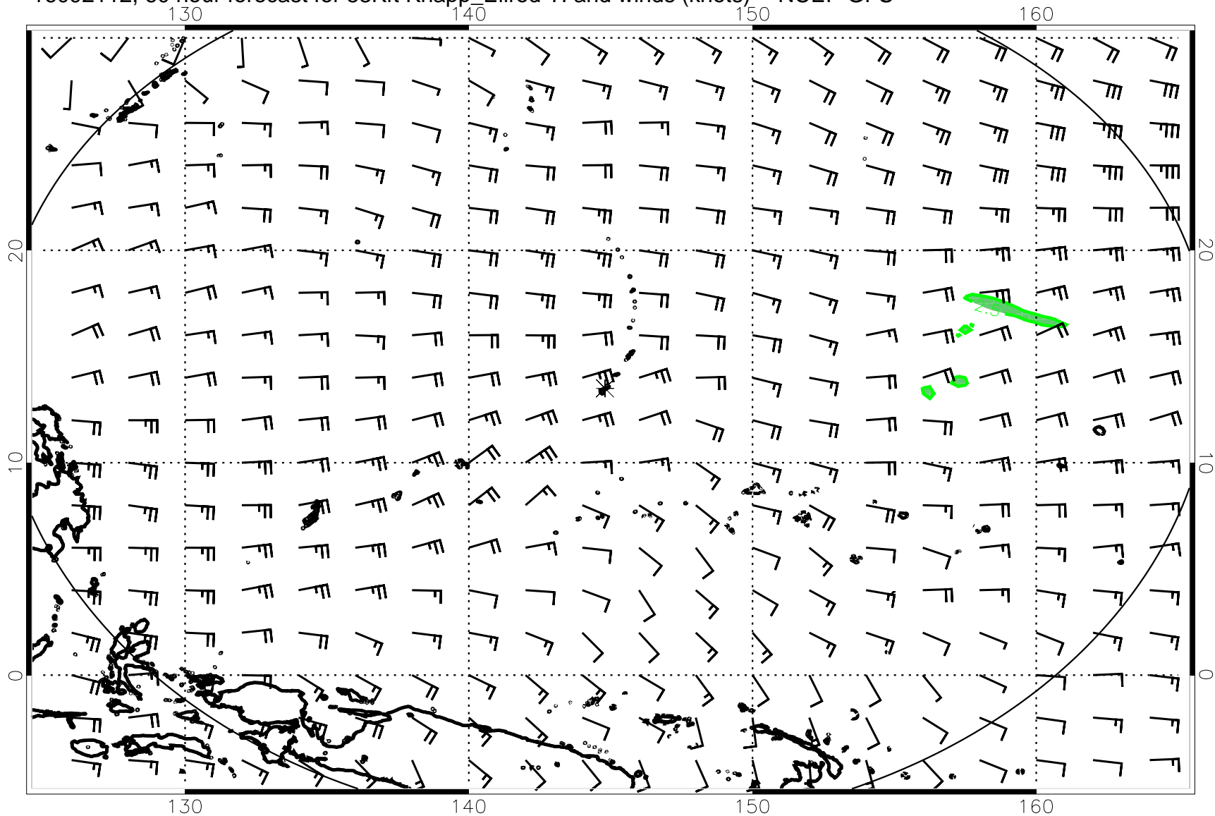
16092112, 60 hour forecast for 53Kft Knapp_Ellrod TI and winds (knots) -- NCEP GFS
