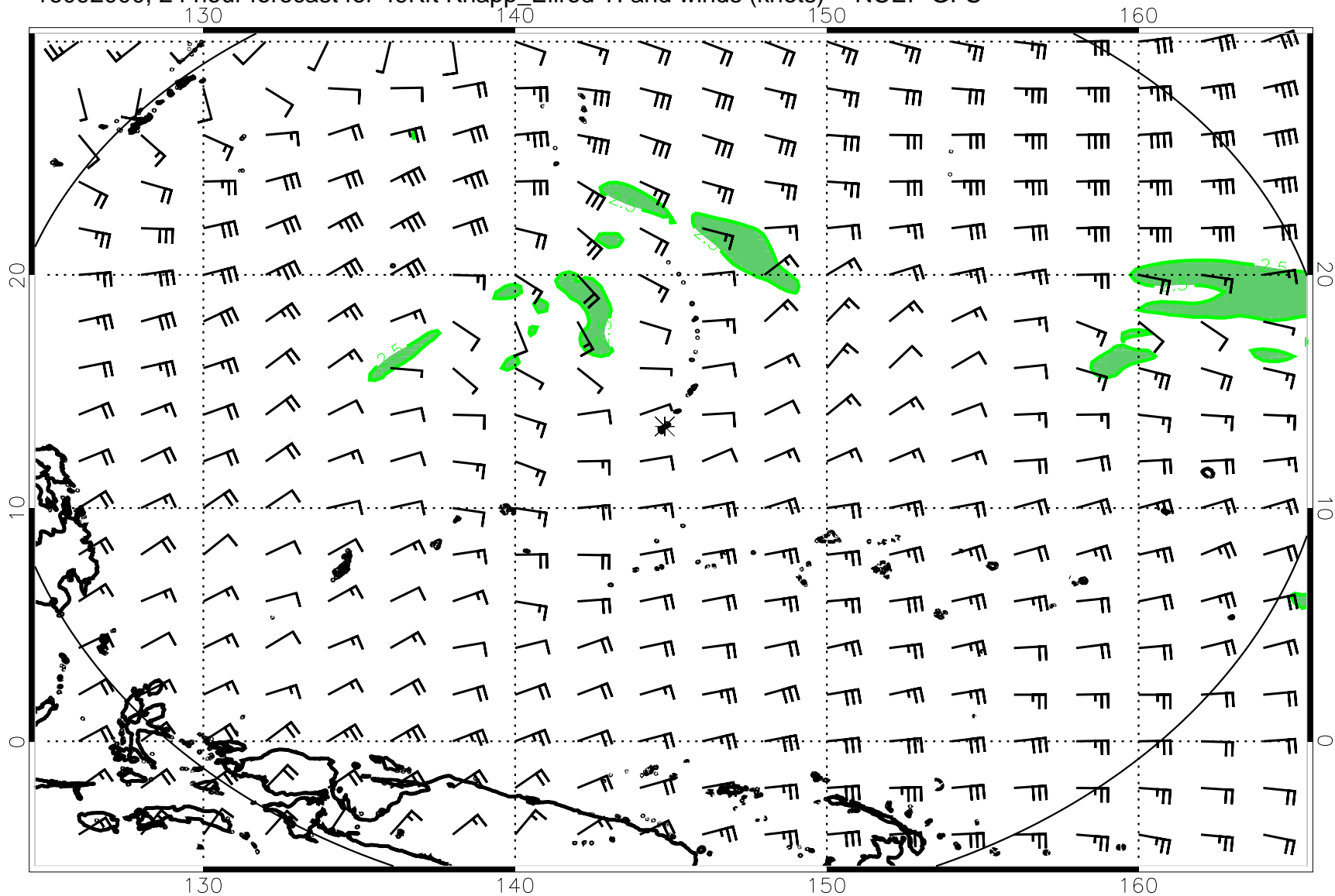
16092000, 24 hour forecast for 49Kft Knapp_Ellrod TI and winds (knots) -- NCEP GFS
