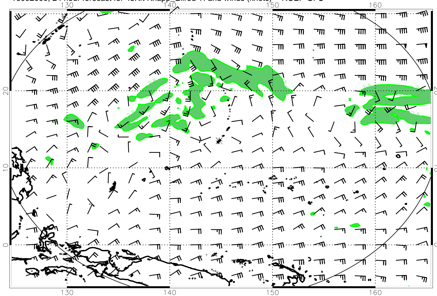
16092000, 24 hour forecast for 45Kft Knapp_Ellrod TI and winds (knots) -- NCEP GFS
