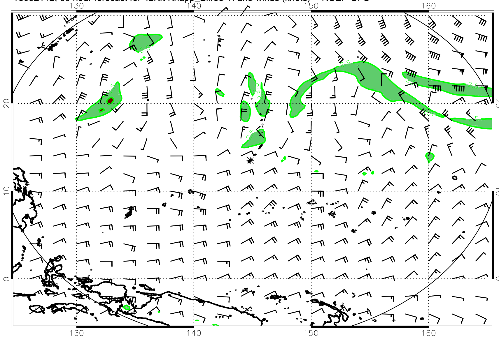
16092112, 60 hour forecast for 42Kft Knapp_Ellrod TI and winds (knots) -- NCEP GFS
