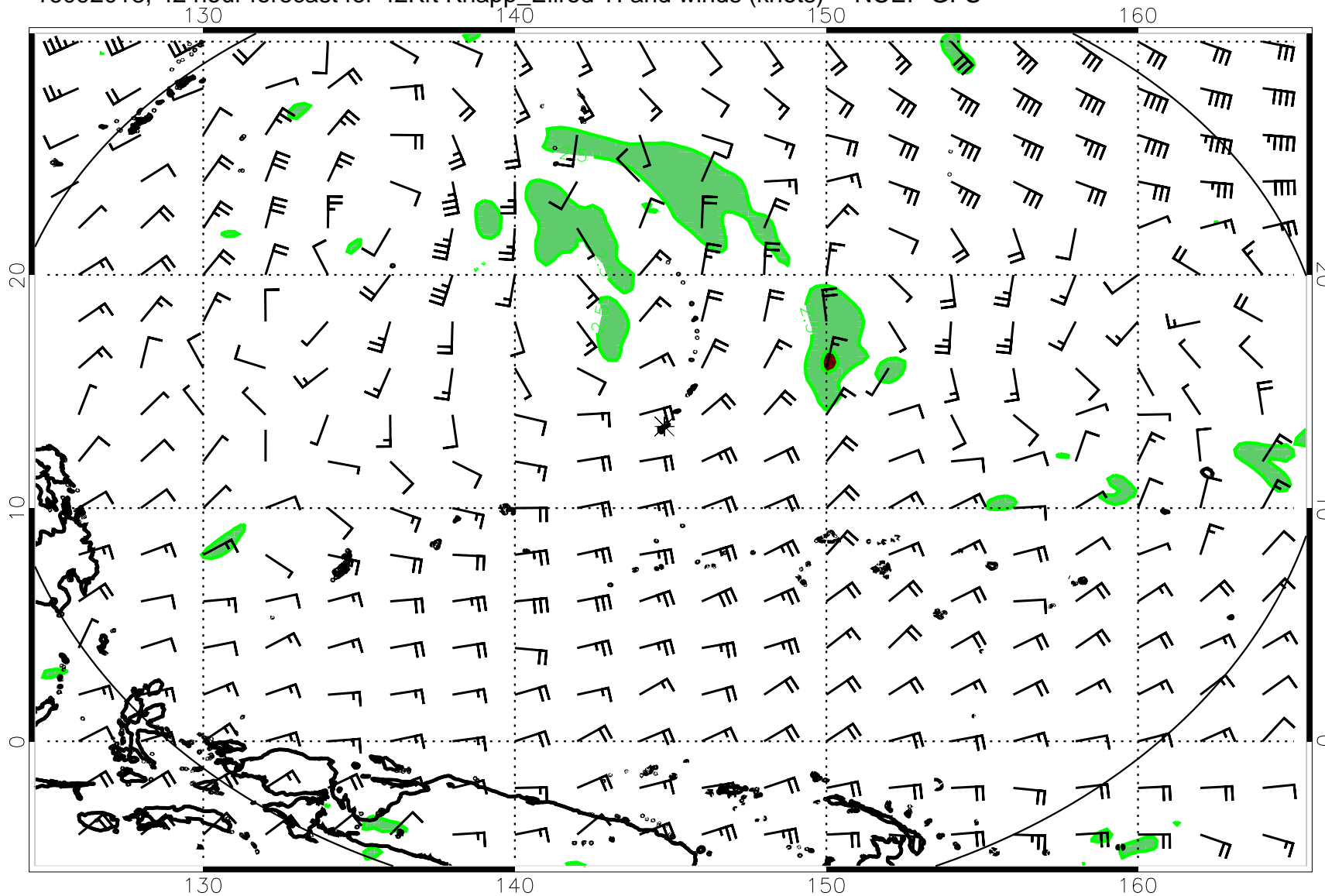
16092018, 42 hour forecast for 42Kft Knapp_Ellrod TI and winds (knots) -- NCEP GFS
