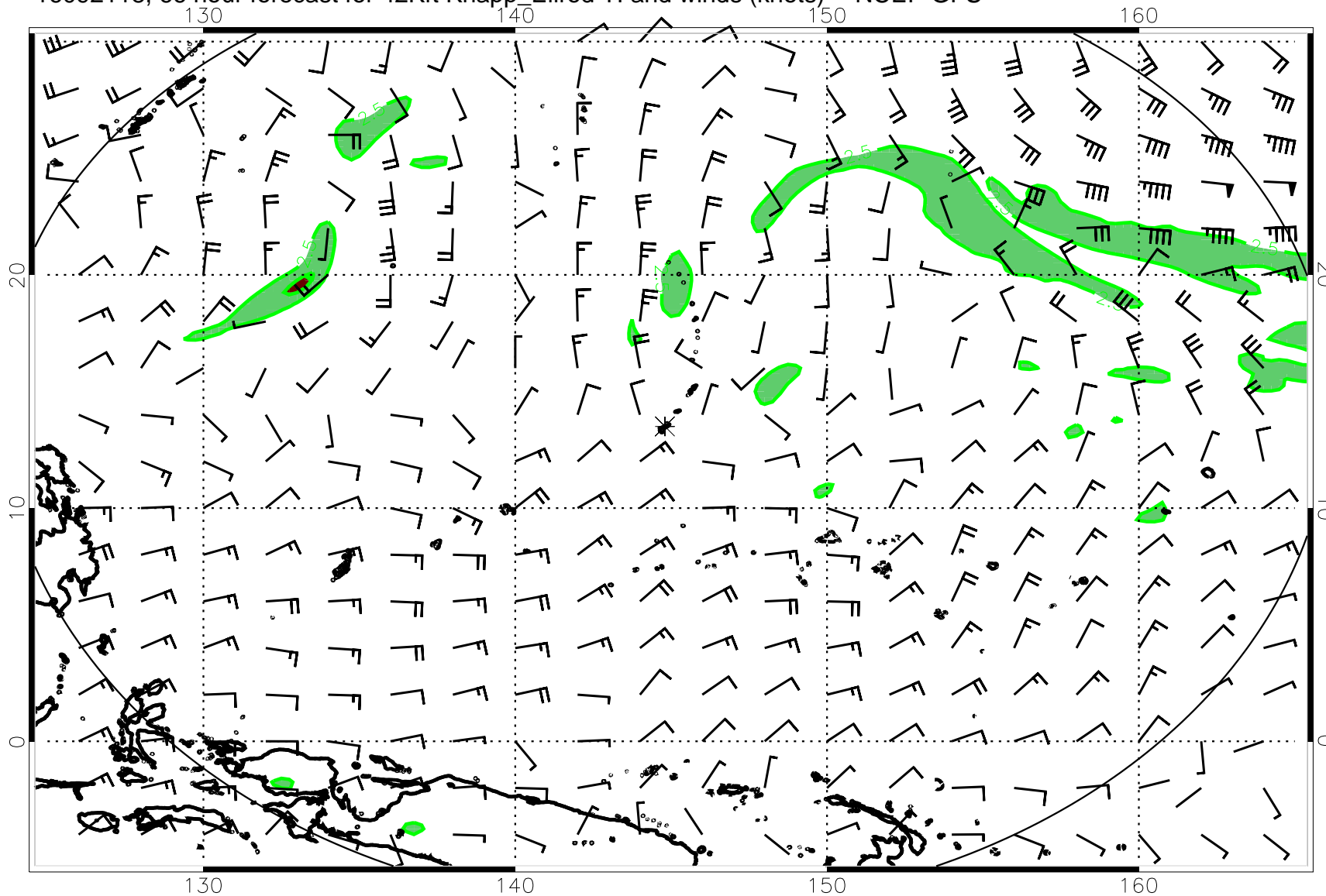
16092118, 66 hour forecast for 42Kft Knapp_Ellrod TI and winds (knots) -- NCEP GFS
