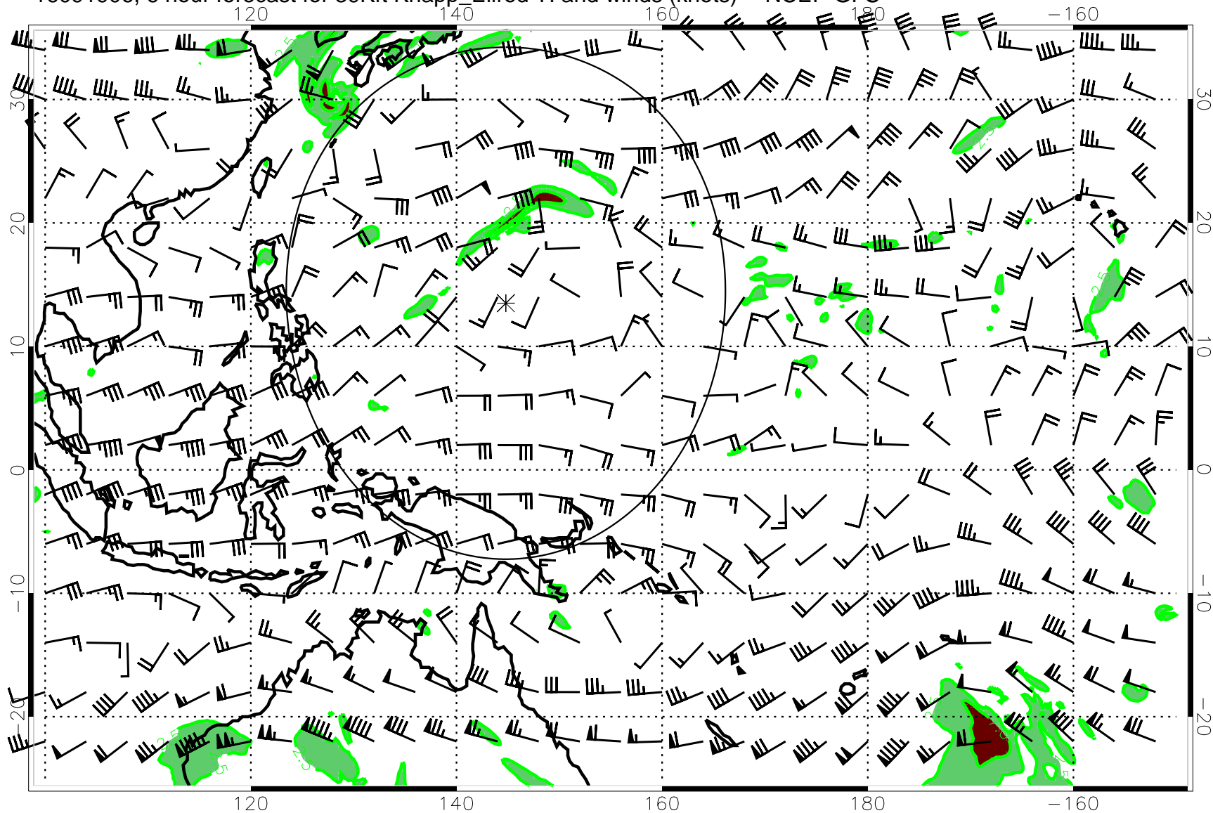
16091906, 6 hour forecast for 39Kft Knapp_Ellrod TI and winds (knots) -- NCEP GFS
