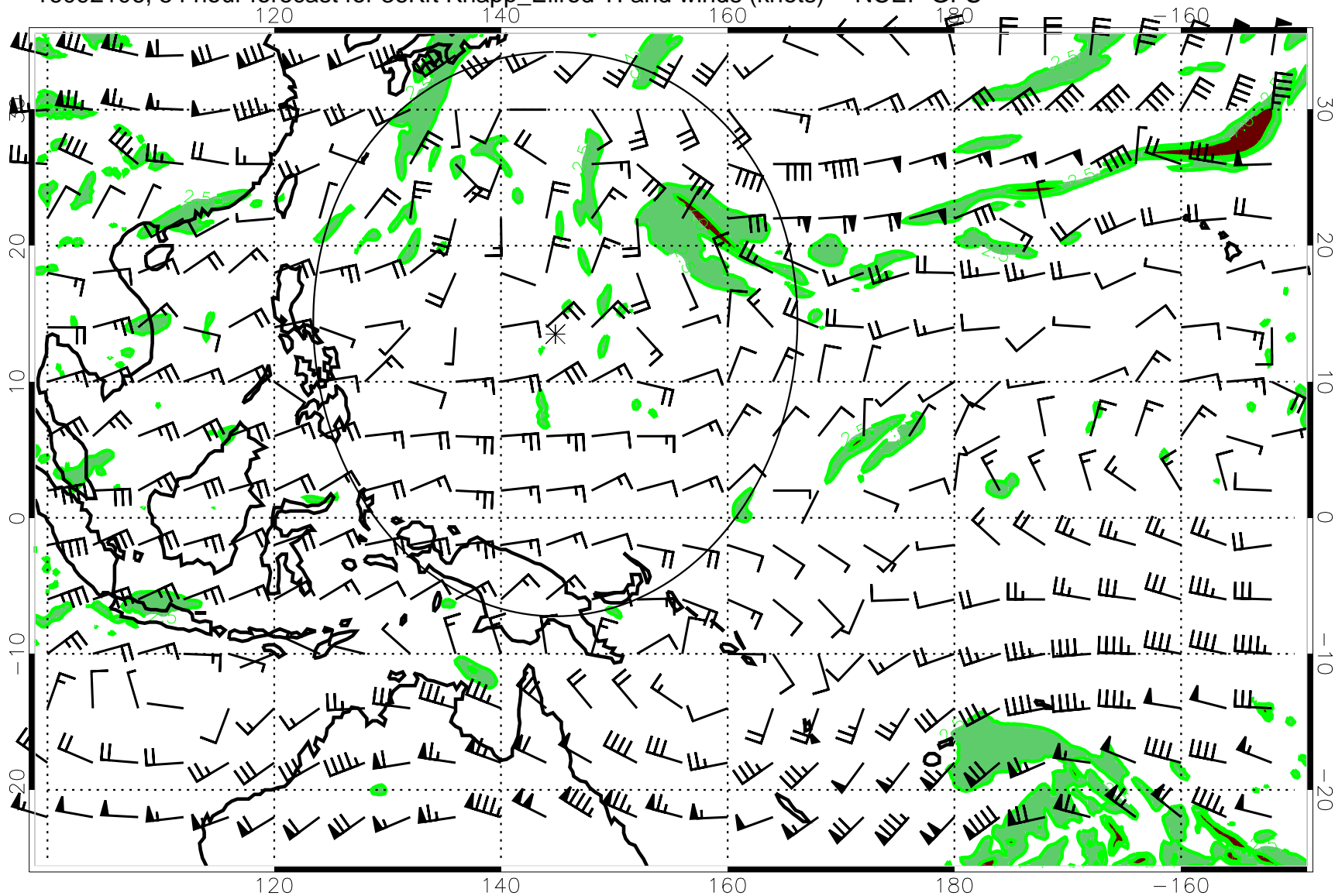
16092106, 54 hour forecast for 36Kft Knapp_Ellrod TI and winds (knots) -- NCEP GFS
