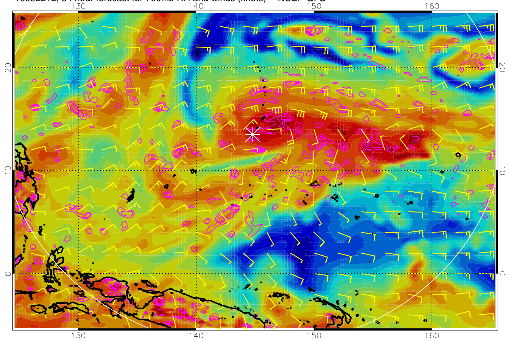
16092212, 84 hour forecast for 700mb RH and winds (knots) -- NCEP GFS
