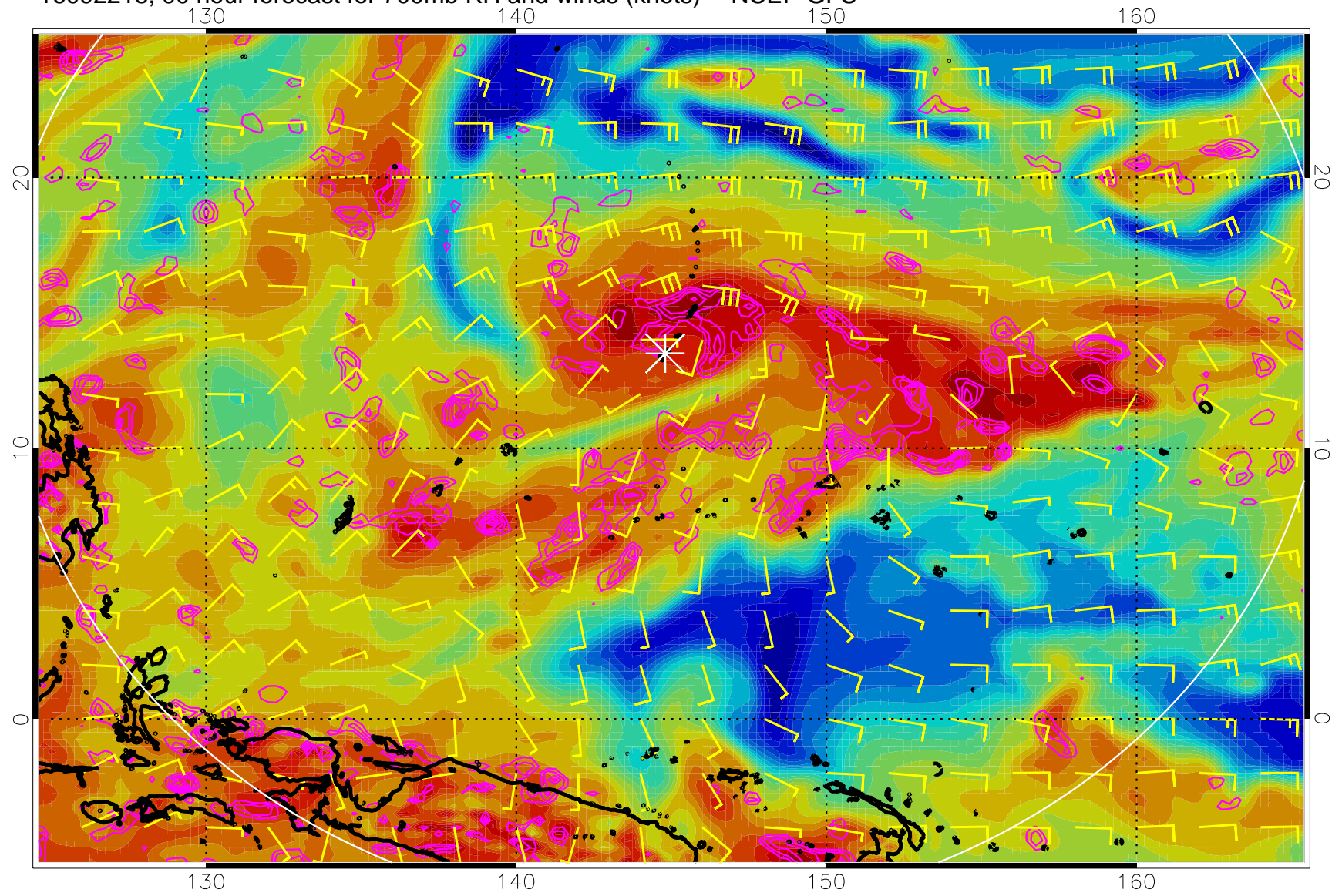
16092218, 90 hour forecast for 700mb RH and winds (knots) -- NCEP GFS
