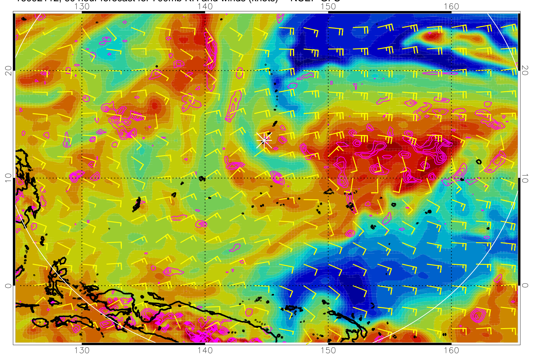
16092112, 60 hour forecast for 700mb RH and winds (knots) -- NCEP GFS
