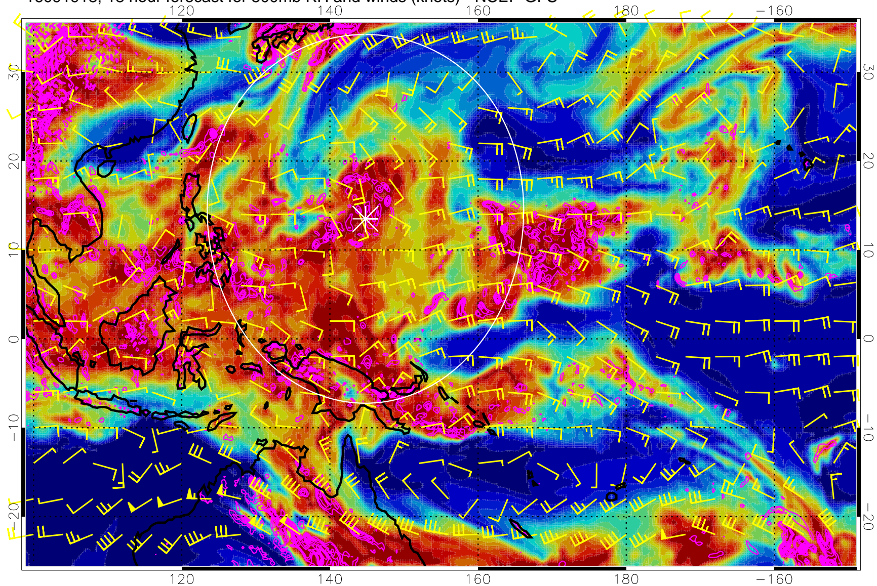
16091918, 18 hour forecast for 500mb RH and winds (knots) - NCEP GFS
