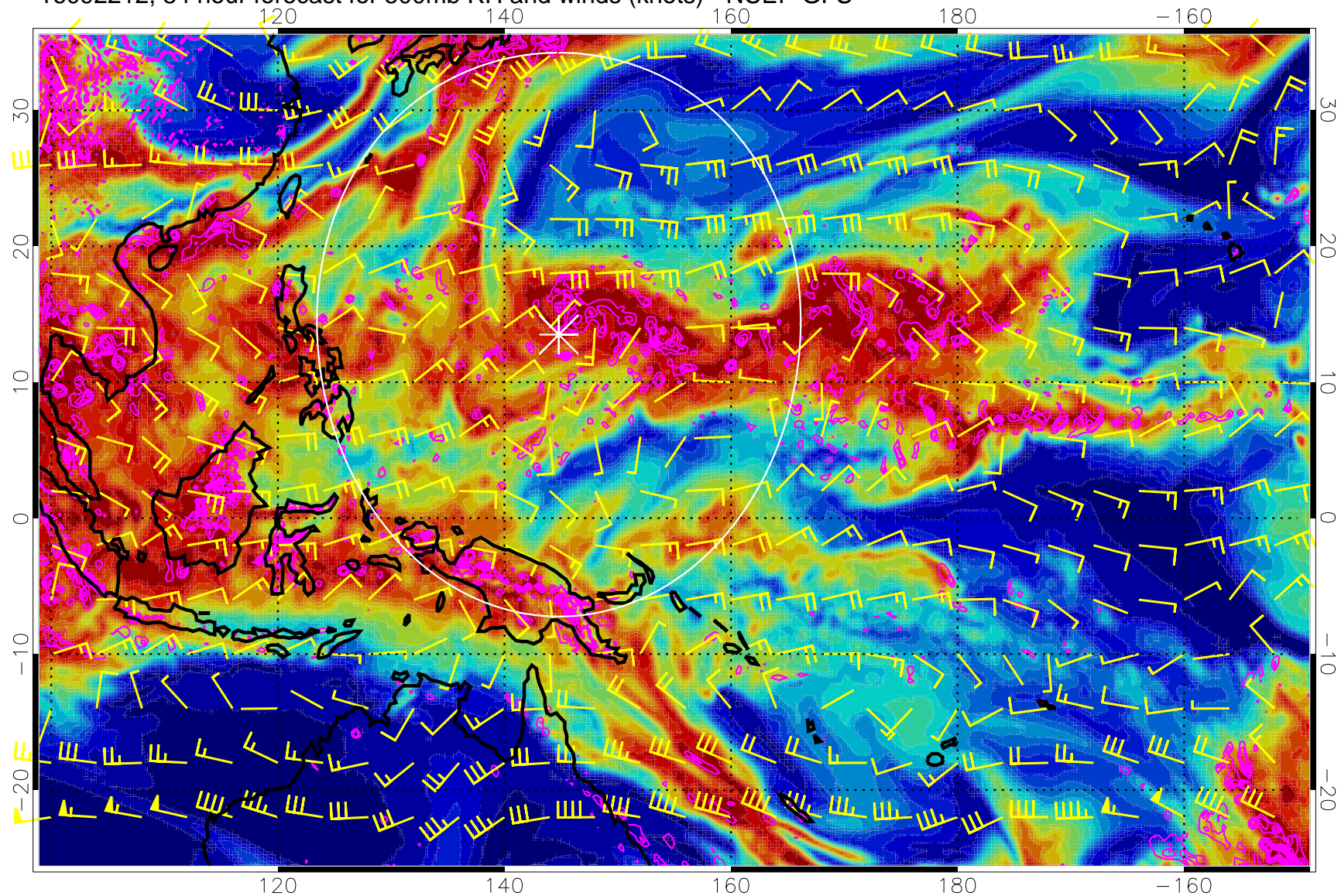
16092212, 84 hour forecast for 500mb RH and winds (knots) - NCEP GFS
