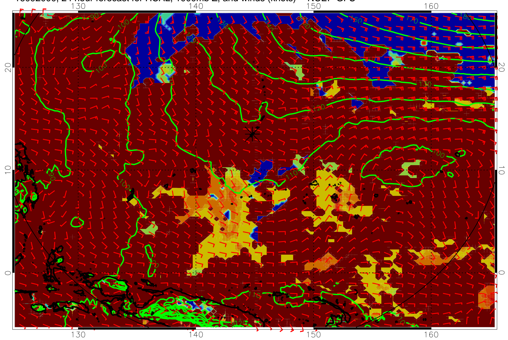
16092000, 24 hour forecast for HCAL, 1000mb Z, and winds (knots) -- NCEP GFS
