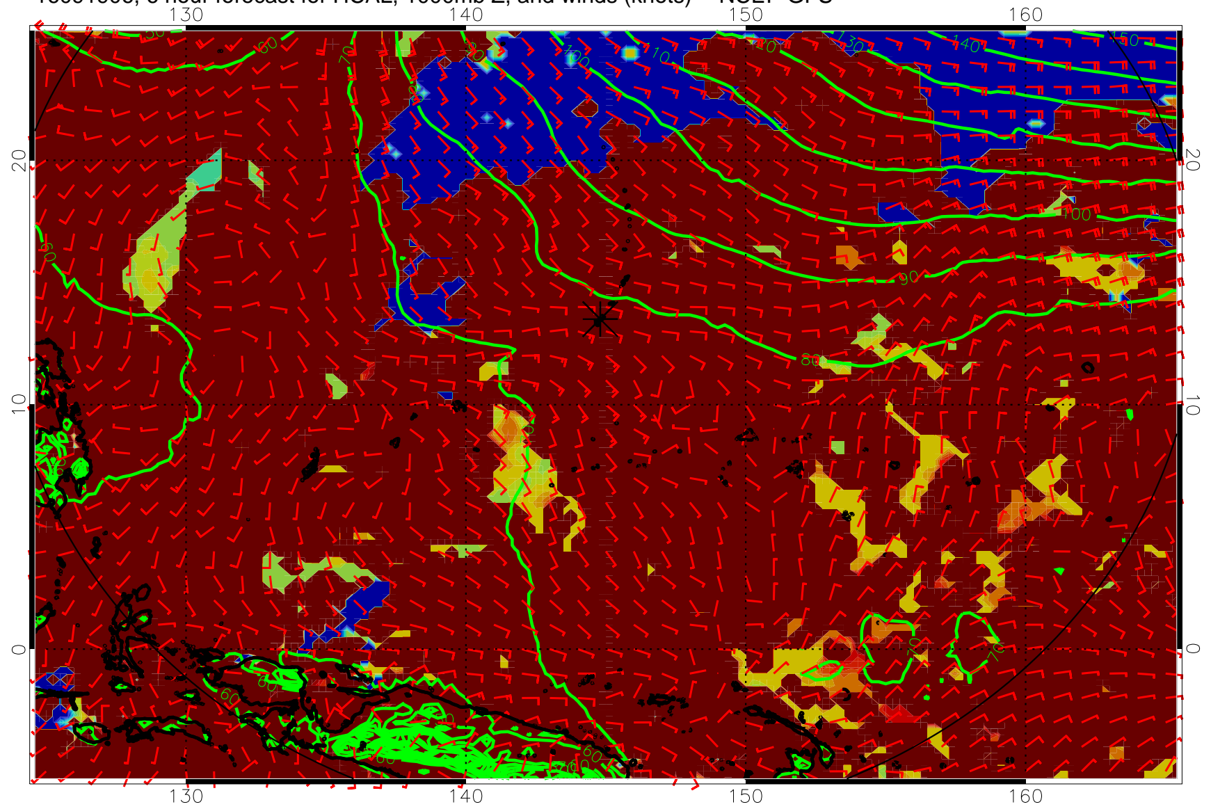
16091906, 6 hour forecast for HCAL, 1000mb Z, and winds (knots) -- NCEP GFS
