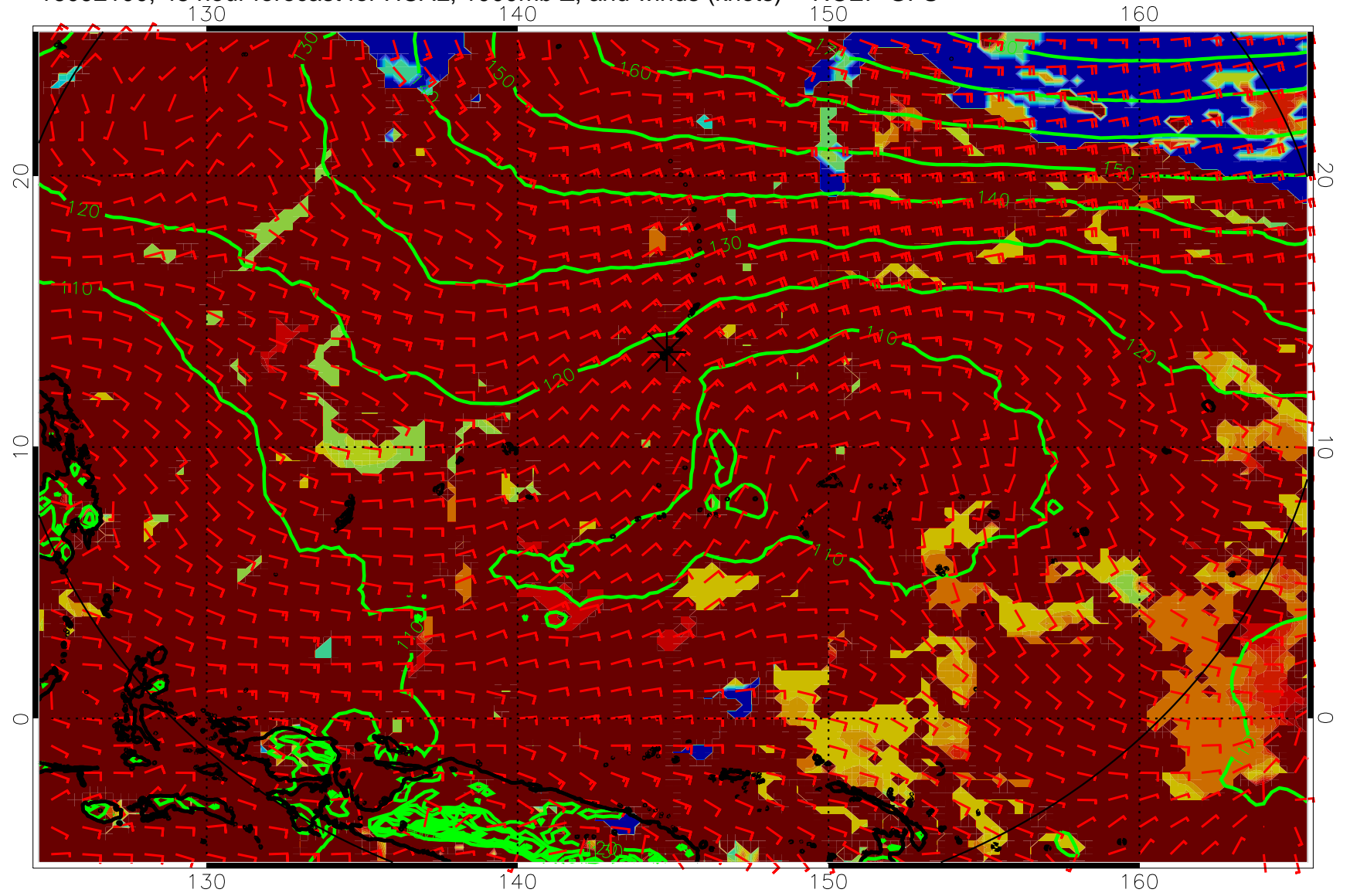
16092100, 48 hour forecast for HCAL, 1000mb Z, and winds (knots) -- NCEP GFS
