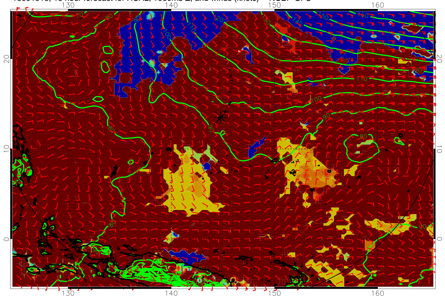
16091918, 18 hour forecast for HCAL, 1000mb Z, and winds (knots) -- NCEP GFS
