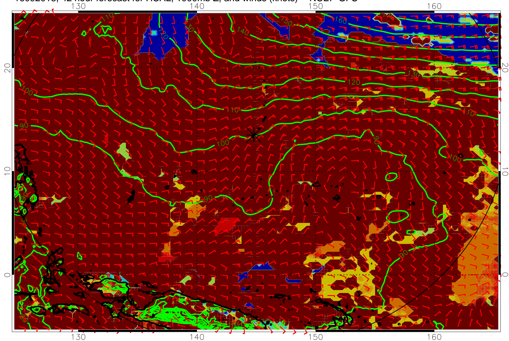
16092018, 42 hour forecast for HCAL, 1000mb Z, and winds (knots) -- NCEP GFS
