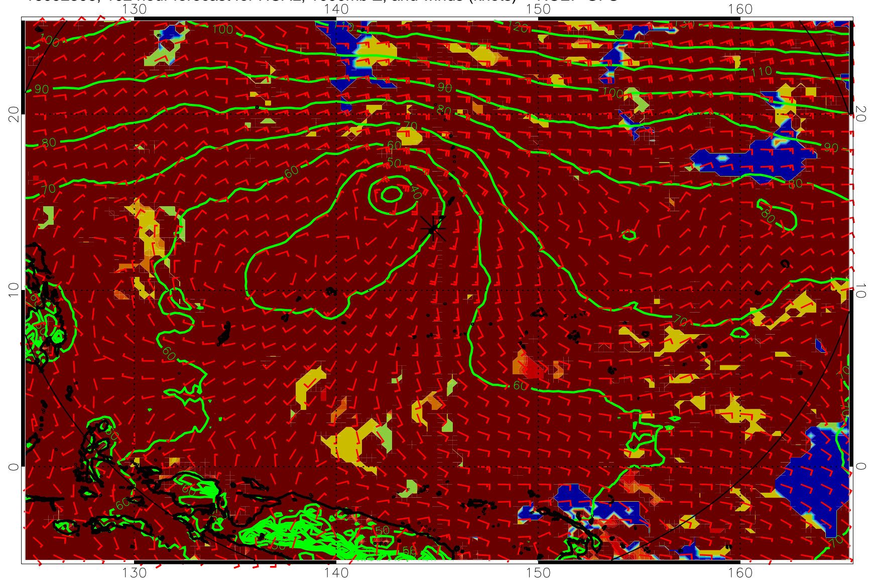
16092306, 102 hour forecast for HCAL, 1000mb Z, and winds (knots) -- NCEP GFS
