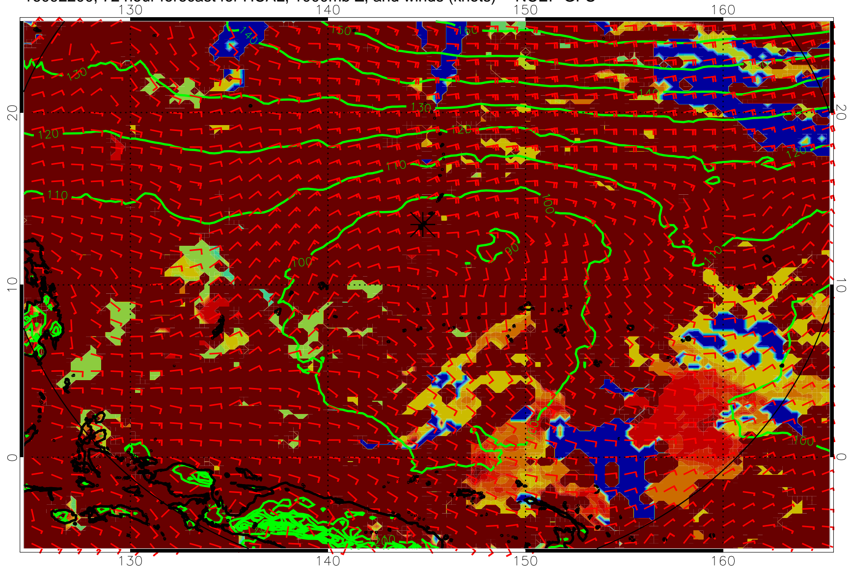
16092200, 72 hour forecast for HCAL, 1000mb Z, and winds (knots) -- NCEP GFS
