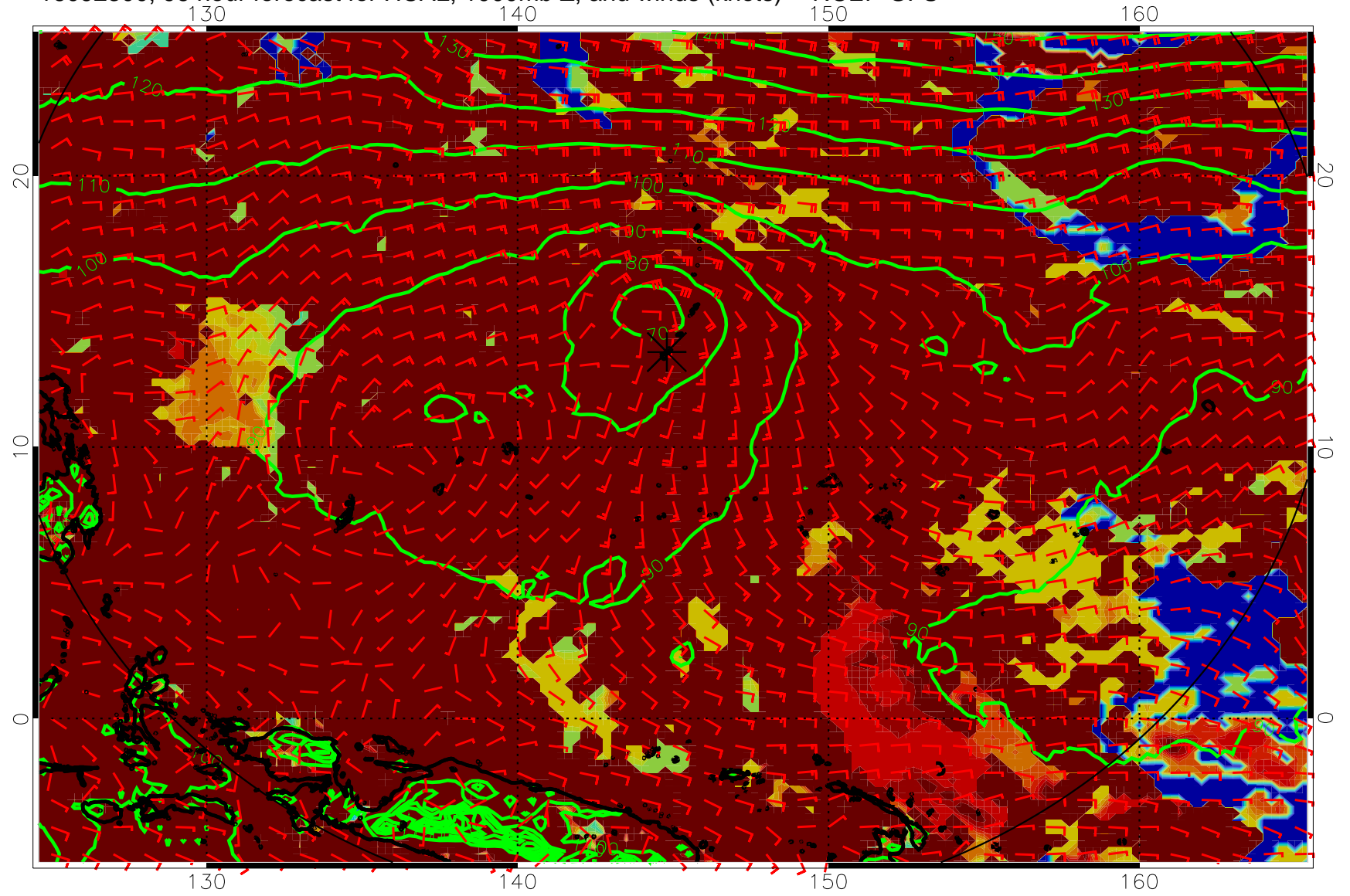
16092300, 96 hour forecast for HCAL, 1000mb Z, and winds (knots) -- NCEP GFS
