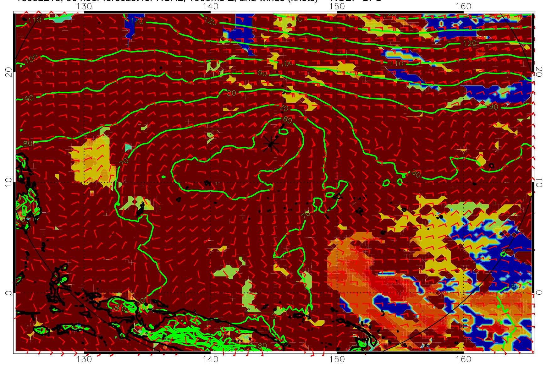
16092218, 90 hour forecast for HCAL, 1000mb Z, and winds (knots) -- NCEP GFS
