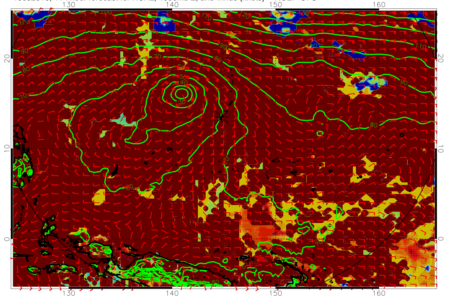
16092318, 114 hour forecast for HCAL, 1000mb Z, and winds (knots) -- NCEP GFS
