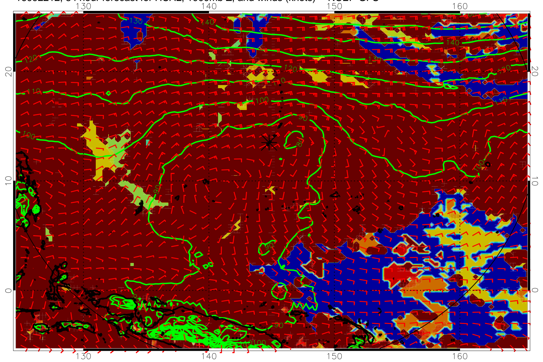
16092212, 84 hour forecast for HCAL, 1000mb Z, and winds (knots) -- NCEP GFS
