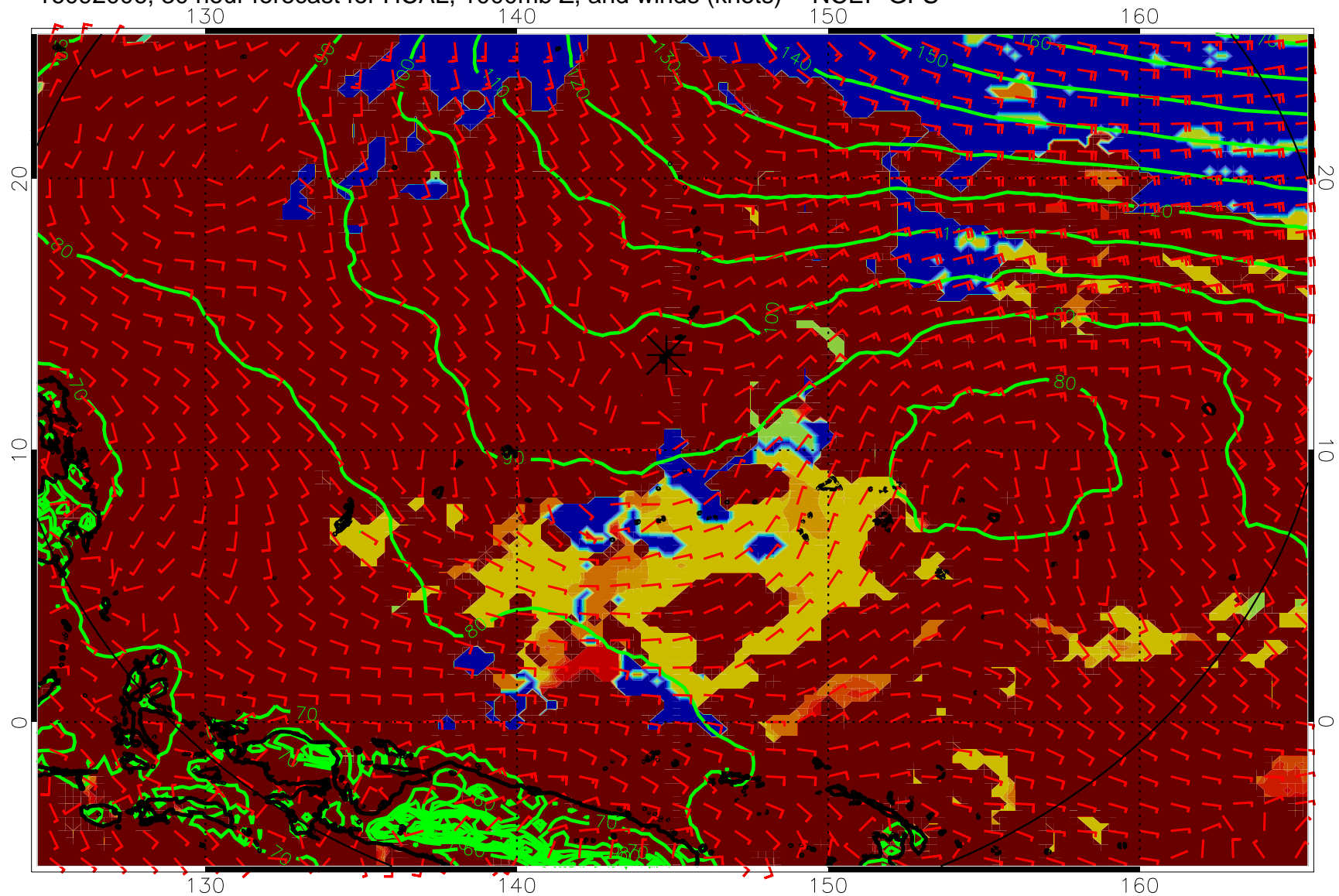
16092006, 30 hour forecast for HCAL, 1000mb Z, and winds (knots) -- NCEP GFS
