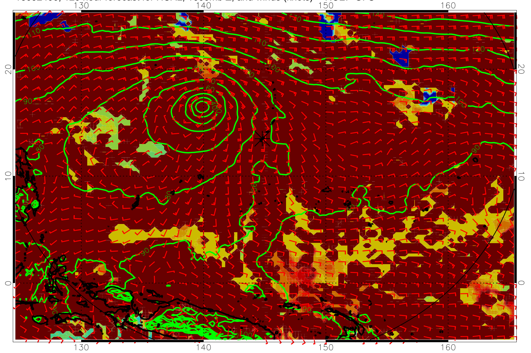
16092400, 120 hour forecast for HCAL, 1000mb Z, and winds (knots) -- NCEP GFS
