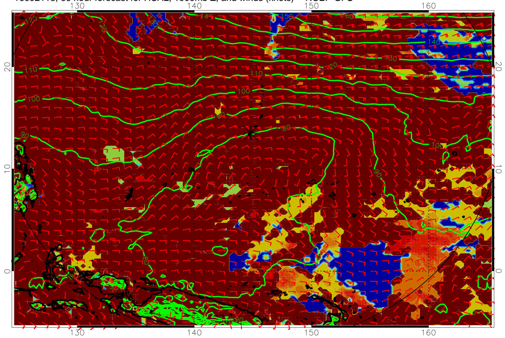
16092118, 66 hour forecast for HCAL, 1000mb Z, and winds (knots) -- NCEP GFS
