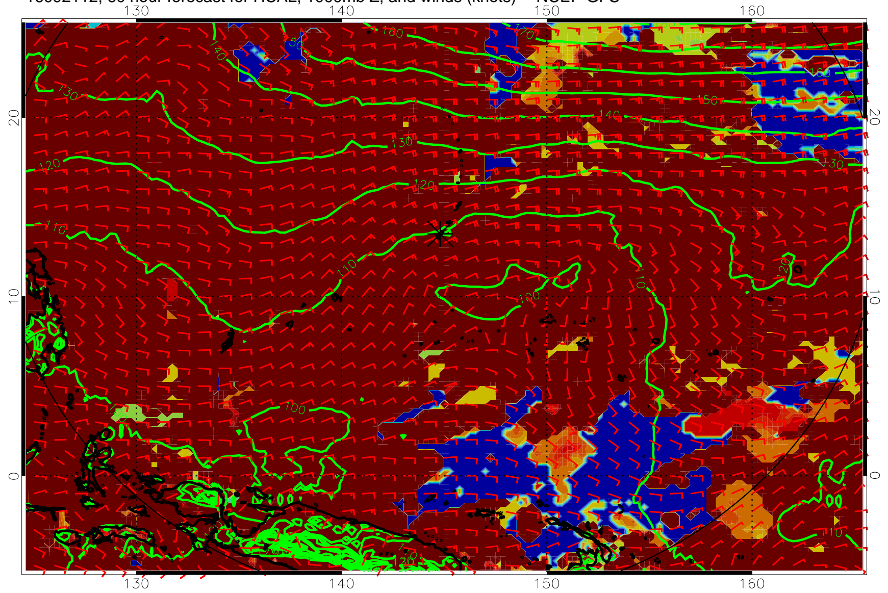
16092112, 60 hour forecast for HCAL, 1000mb Z, and winds (knots) -- NCEP GFS
