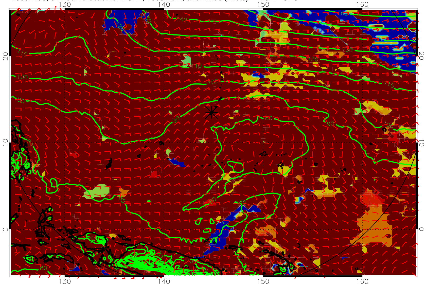
16092106, 54 hour forecast for HCAL, 1000mb Z, and winds (knots) -- NCEP GFS
