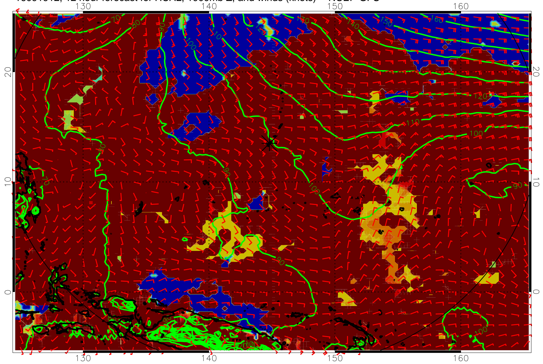
16091912, 12 hour forecast for HCAL, 1000mb Z, and winds (knots) -- NCEP GFS
