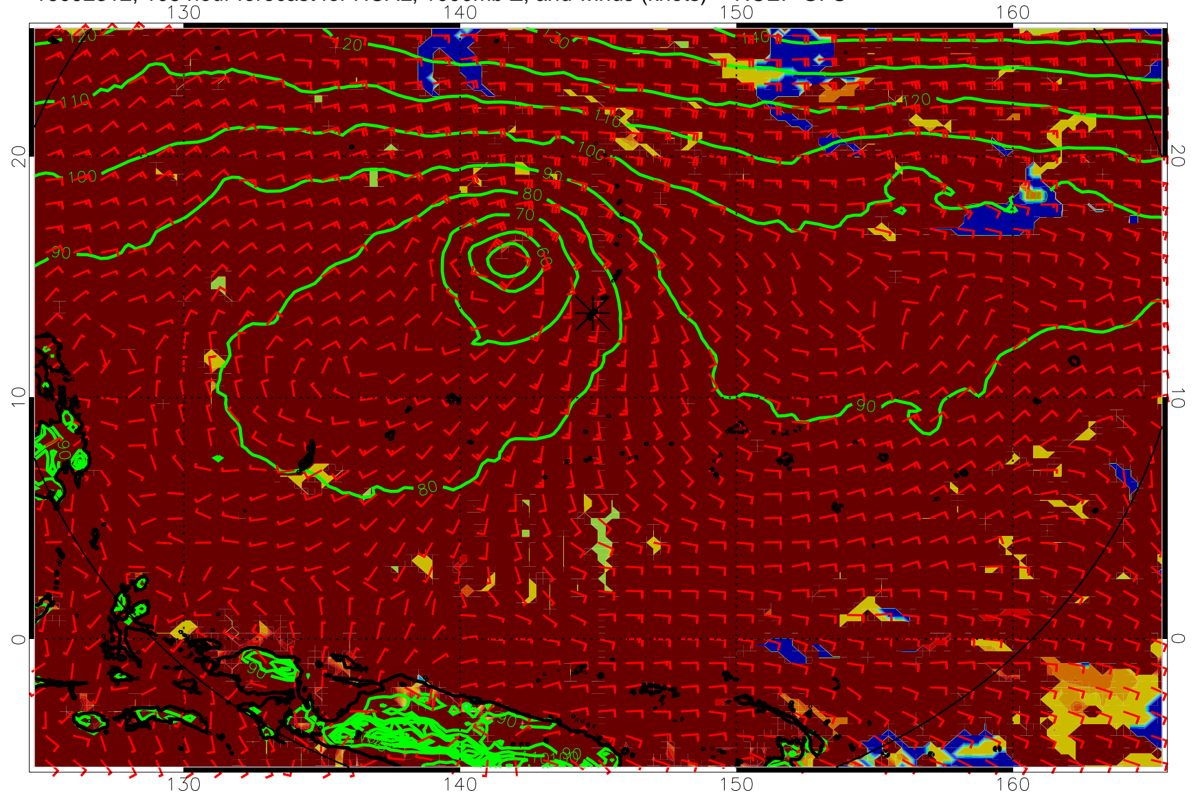
16092312, 108 hour forecast for HCAL, 1000mb Z, and winds (knots) -- NCEP GFS
