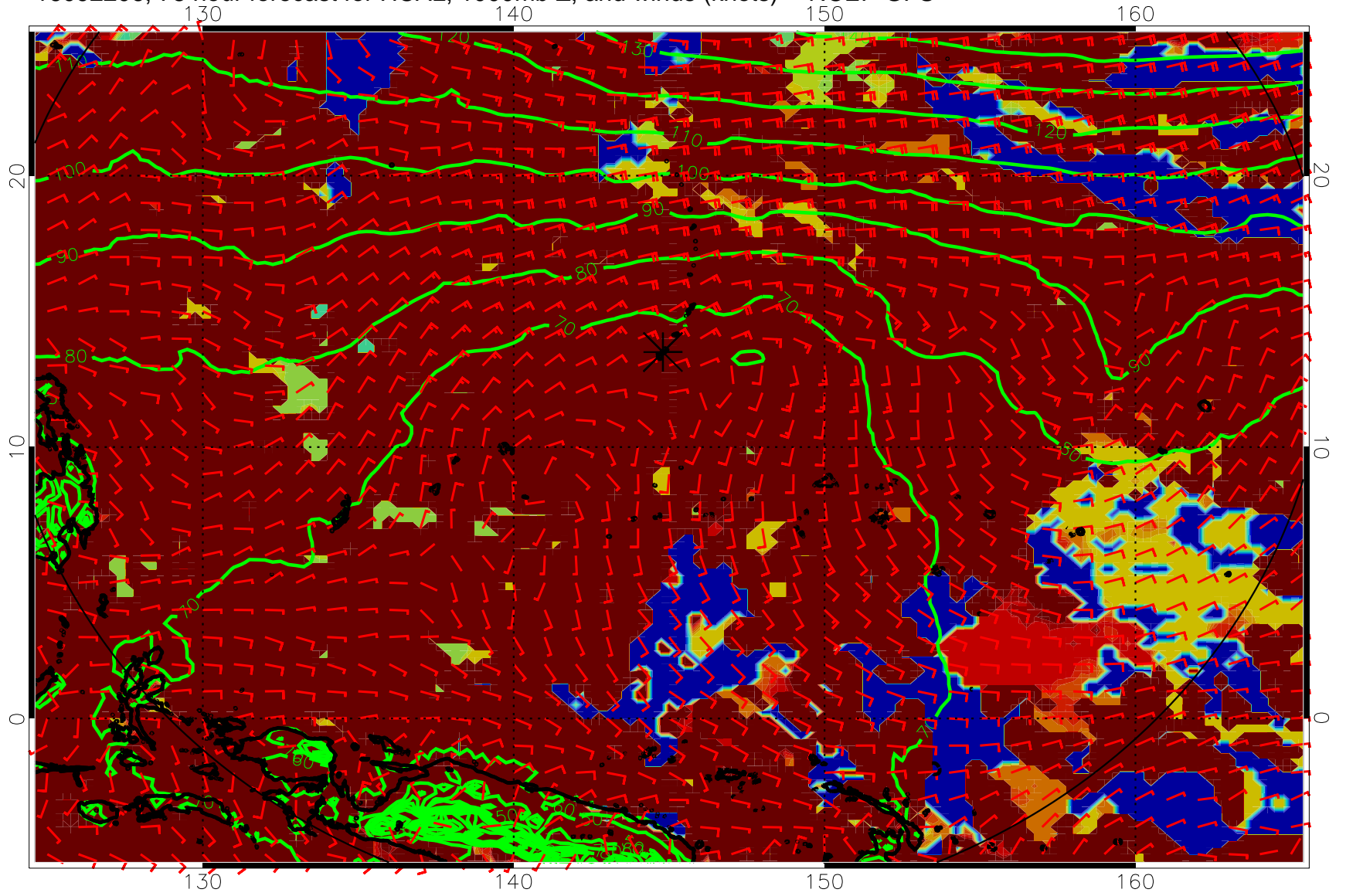
16092206, 78 hour forecast for HCAL, 1000mb Z, and winds (knots) -- NCEP GFS
