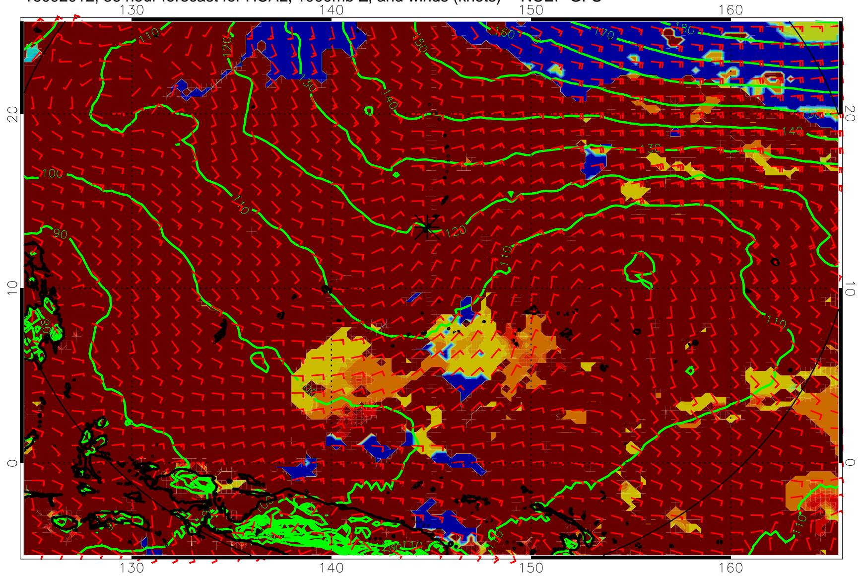
16092012, 36 hour forecast for HCAL, 1000mb Z, and winds (knots) -- NCEP GFS
