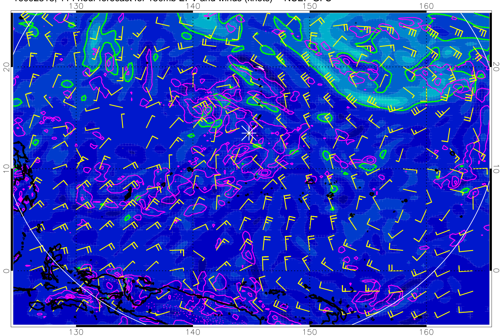
16092318, 114 hour forecast for 150mb EPV and winds (knots) -- NCEP GFS
