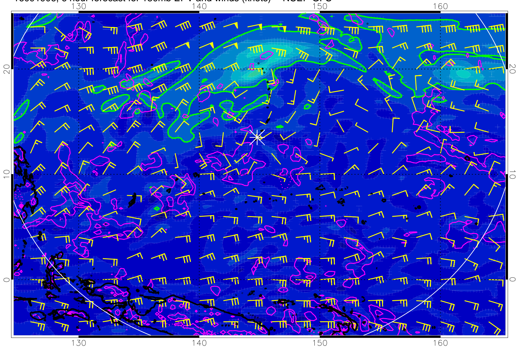
16091906, 6 hour forecast for 150mb EPV and winds (knots) -- NCEP GFS
