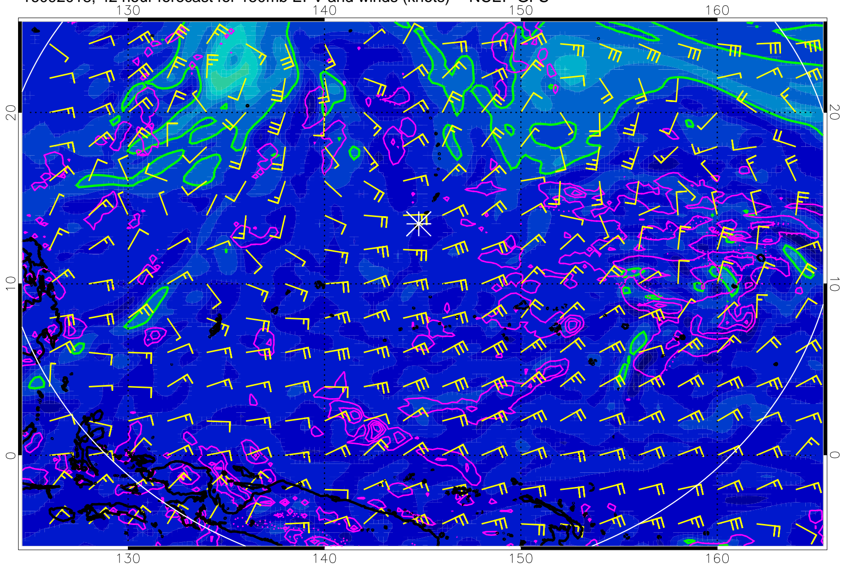
16092018, 42 hour forecast for 150mb EPV and winds (knots) -- NCEP GFS
