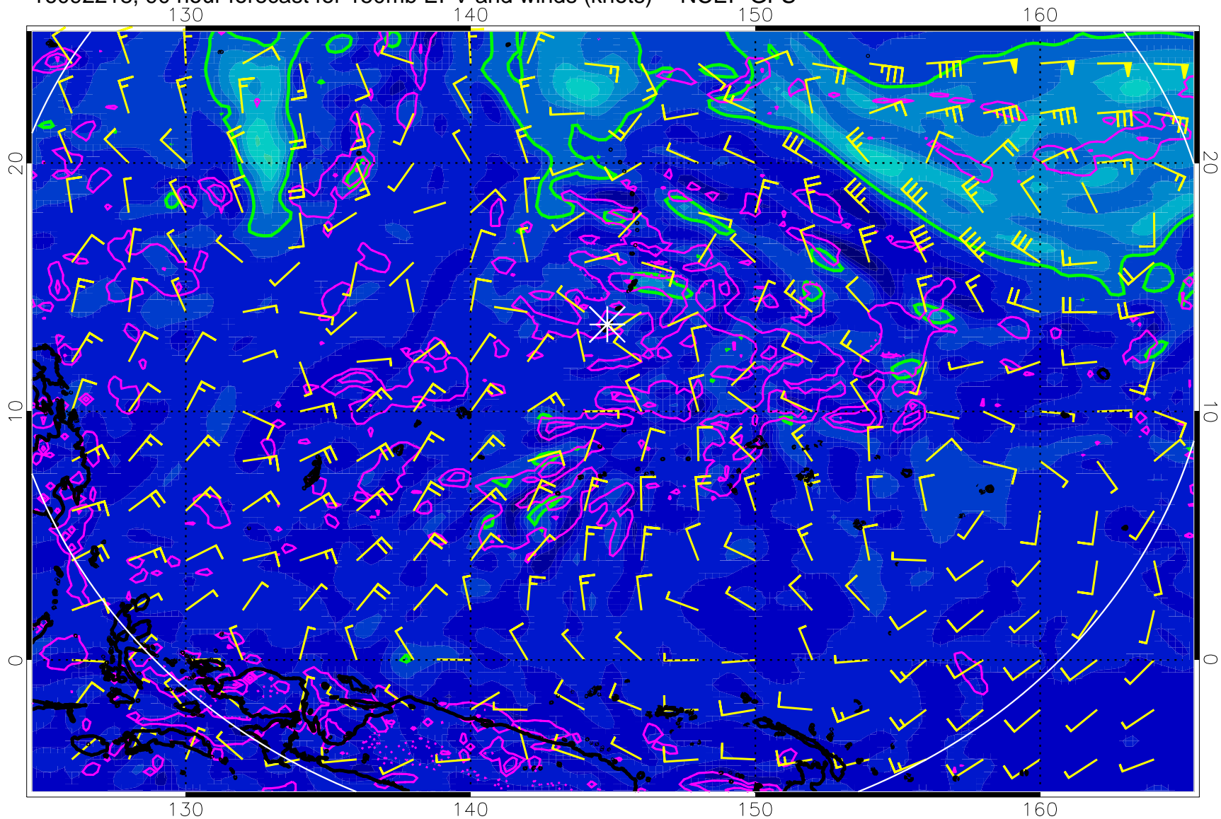
16092218, 90 hour forecast for 150mb EPV and winds (knots) -- NCEP GFS
