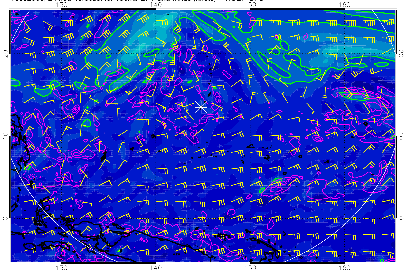
16092000, 24 hour forecast for 150mb EPV and winds (knots) -- NCEP GFS
