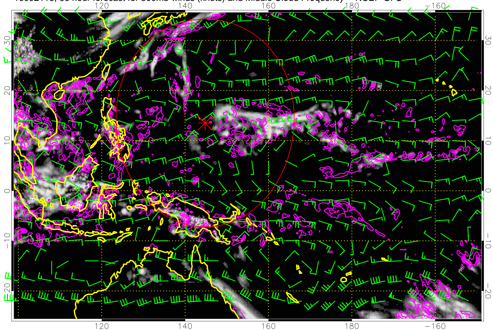
16092118, 66 hour forecast for 500mb winds (knots) and Middle Cloud Frequency -- NCEP GFS
