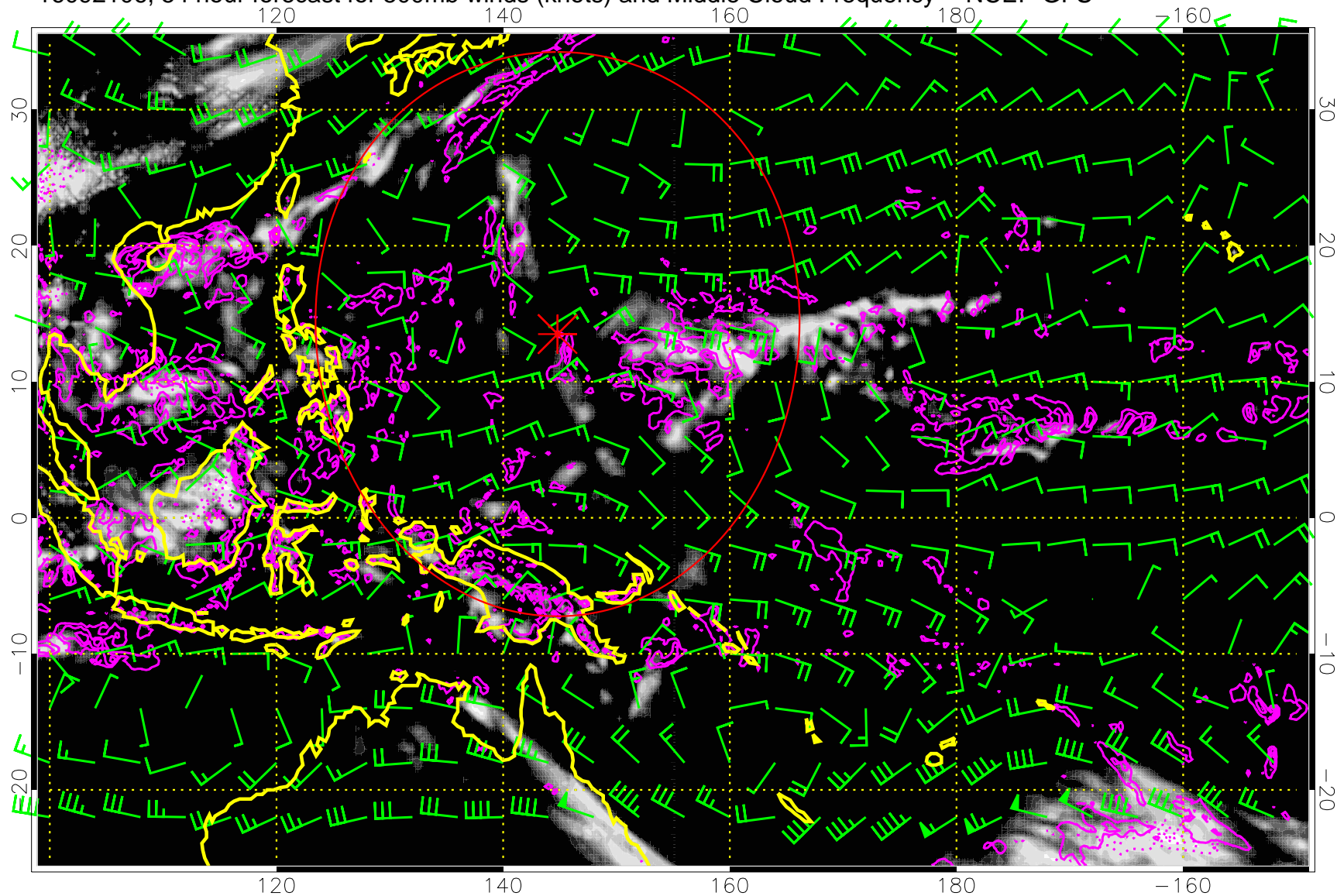
16092106, 54 hour forecast for 500mb winds (knots) and Middle Cloud Frequency -- NCEP GFS
