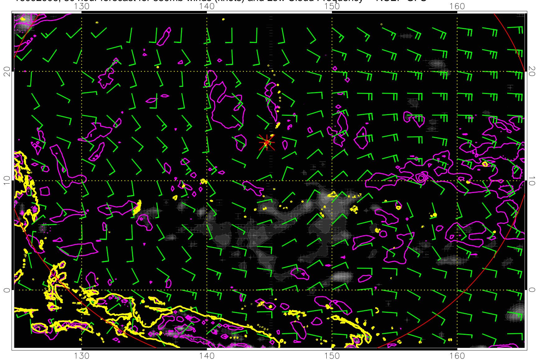
16092006, 30 hour forecast for 850mb winds (knots) and Low Cloud Frequency -- NCEP GFS
