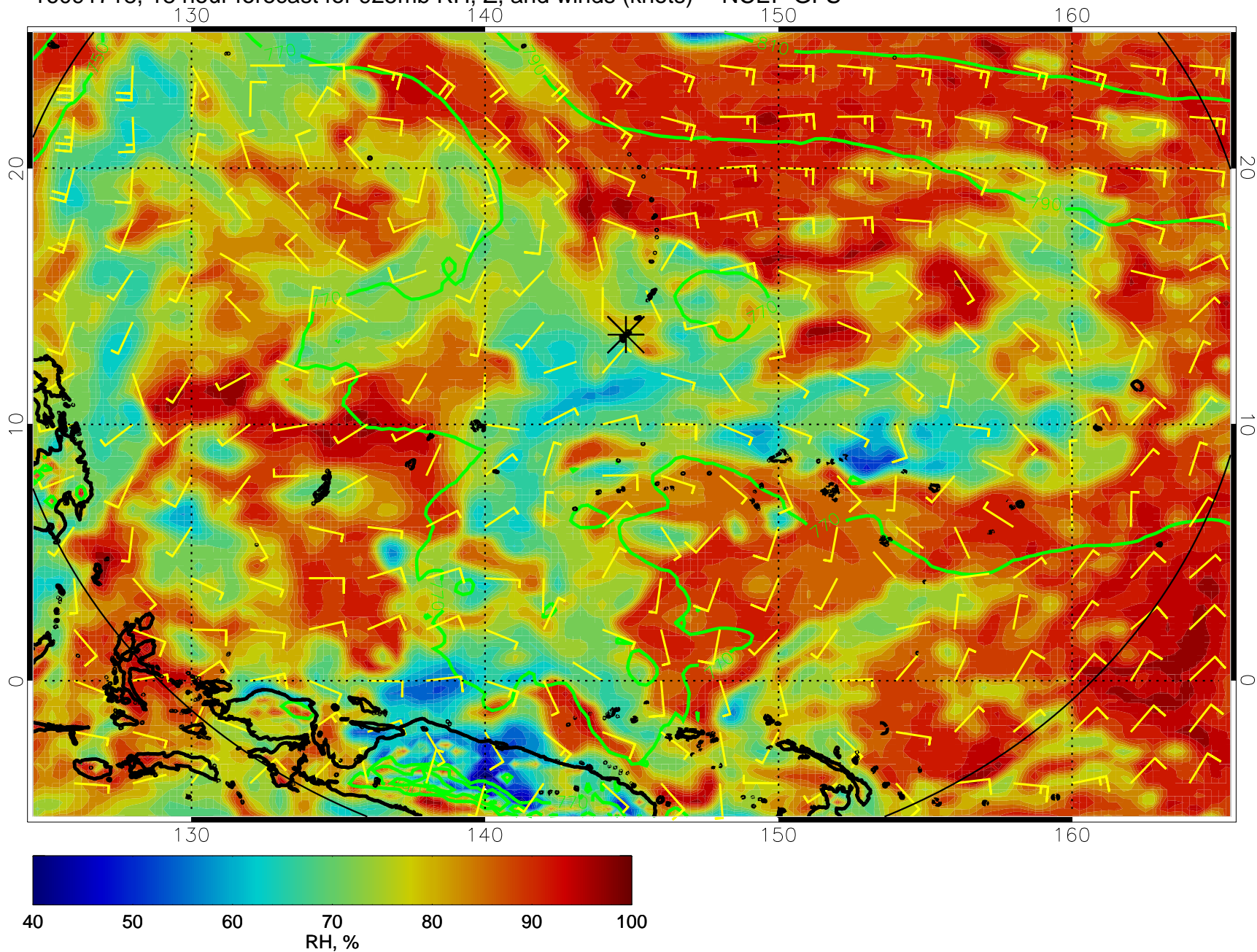
16091718, 18 hour forecast for 925mb RH, Z, and winds (knots) -- NCEP GFS
