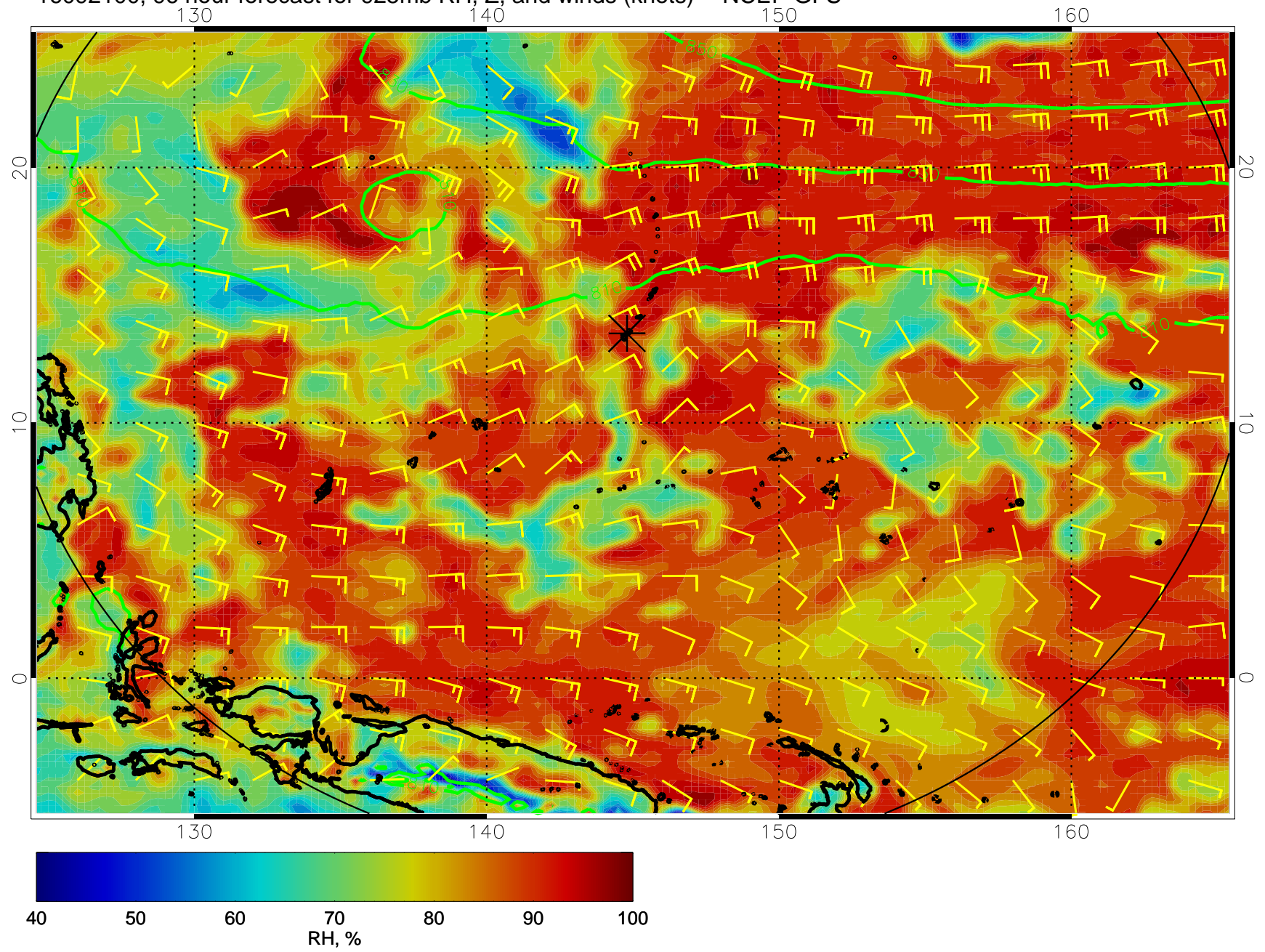
16092100, 96 hour forecast for 925mb RH, Z, and winds (knots) -- NCEP GFS
