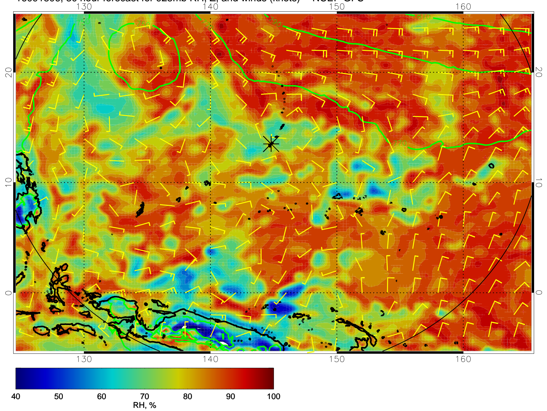
16091806, 30 hour forecast for 925mb RH, Z, and winds (knots) -- NCEP GFS
