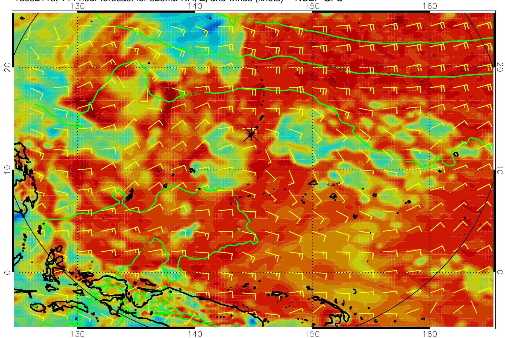
16092118, 114 hour forecast for 925mb RH, Z, and winds (knots) -- NCEP GFS
