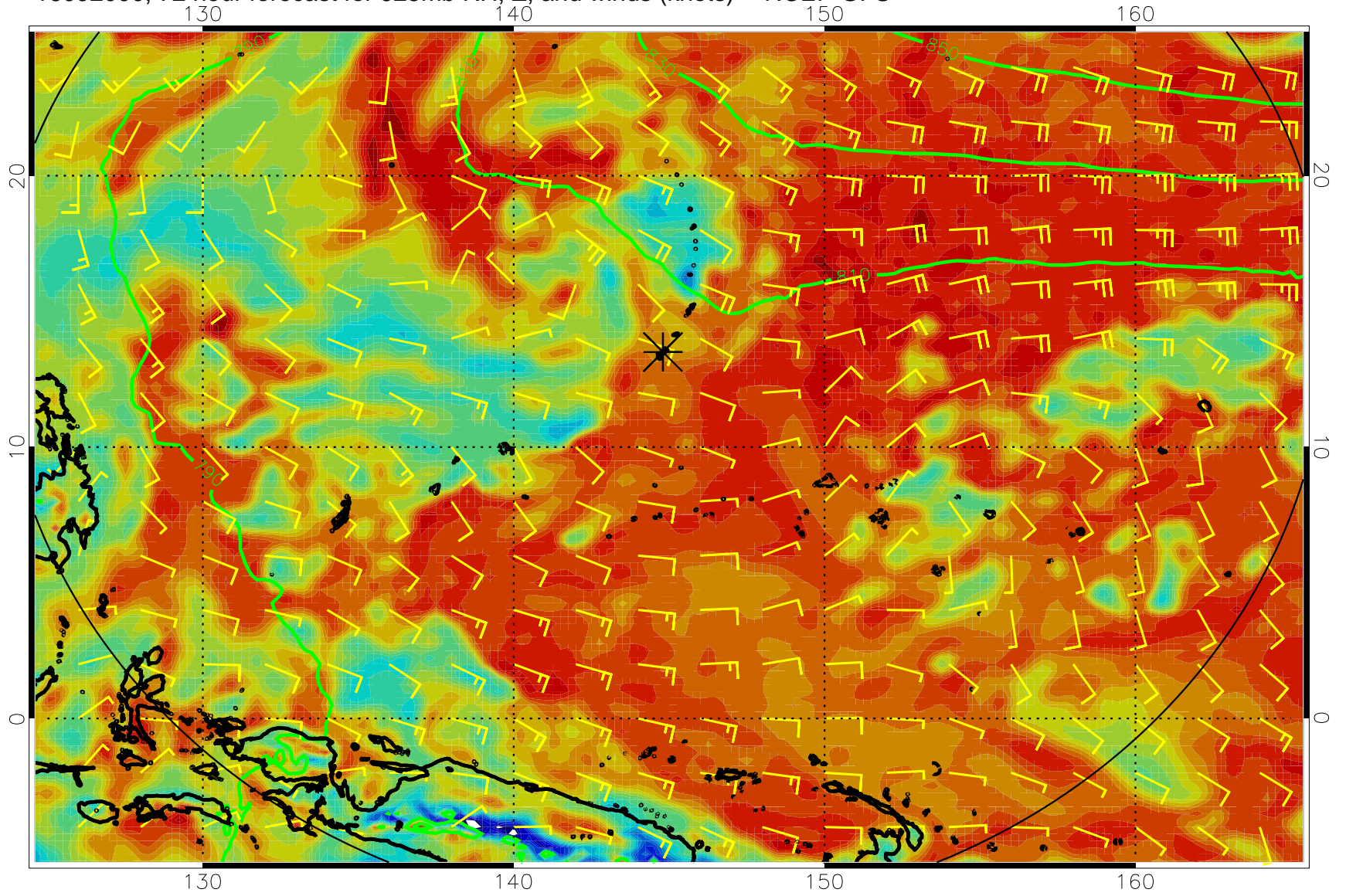
16092000, 72 hour forecast for 925mb RH, Z, and winds (knots) -- NCEP GFS
