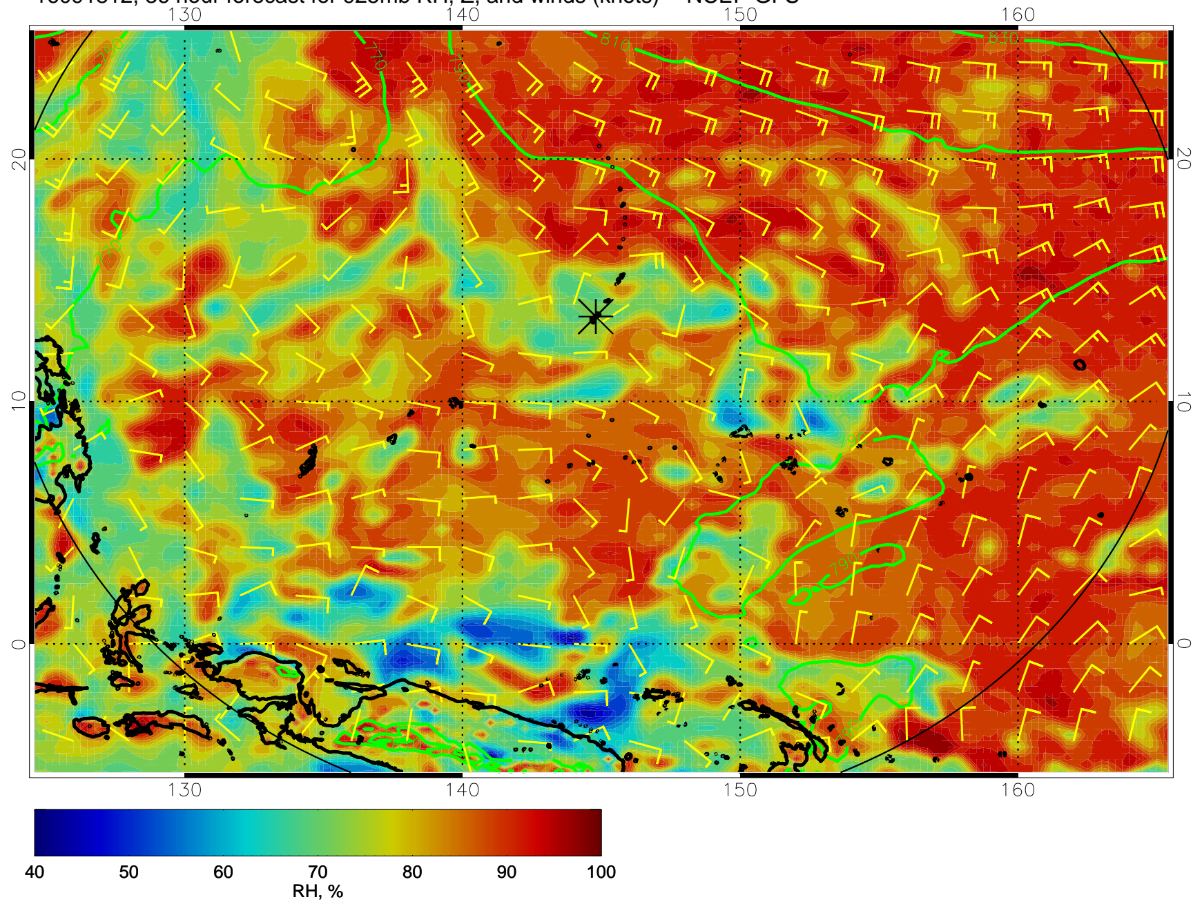
16091812, 36 hour forecast for 925mb RH, Z, and winds (knots) -- NCEP GFS
