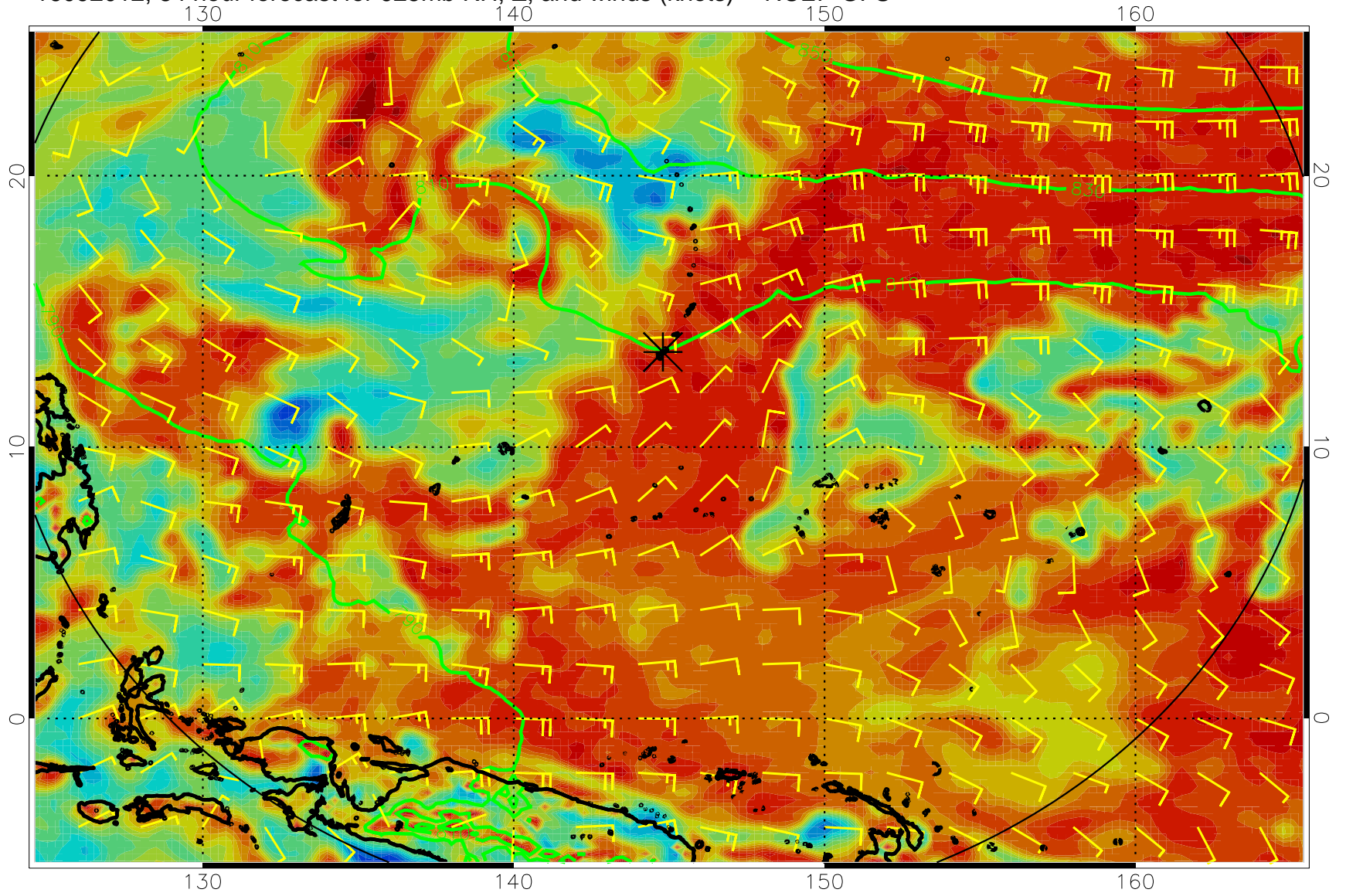
16092012, 84 hour forecast for 925mb RH, Z, and winds (knots) -- NCEP GFS
