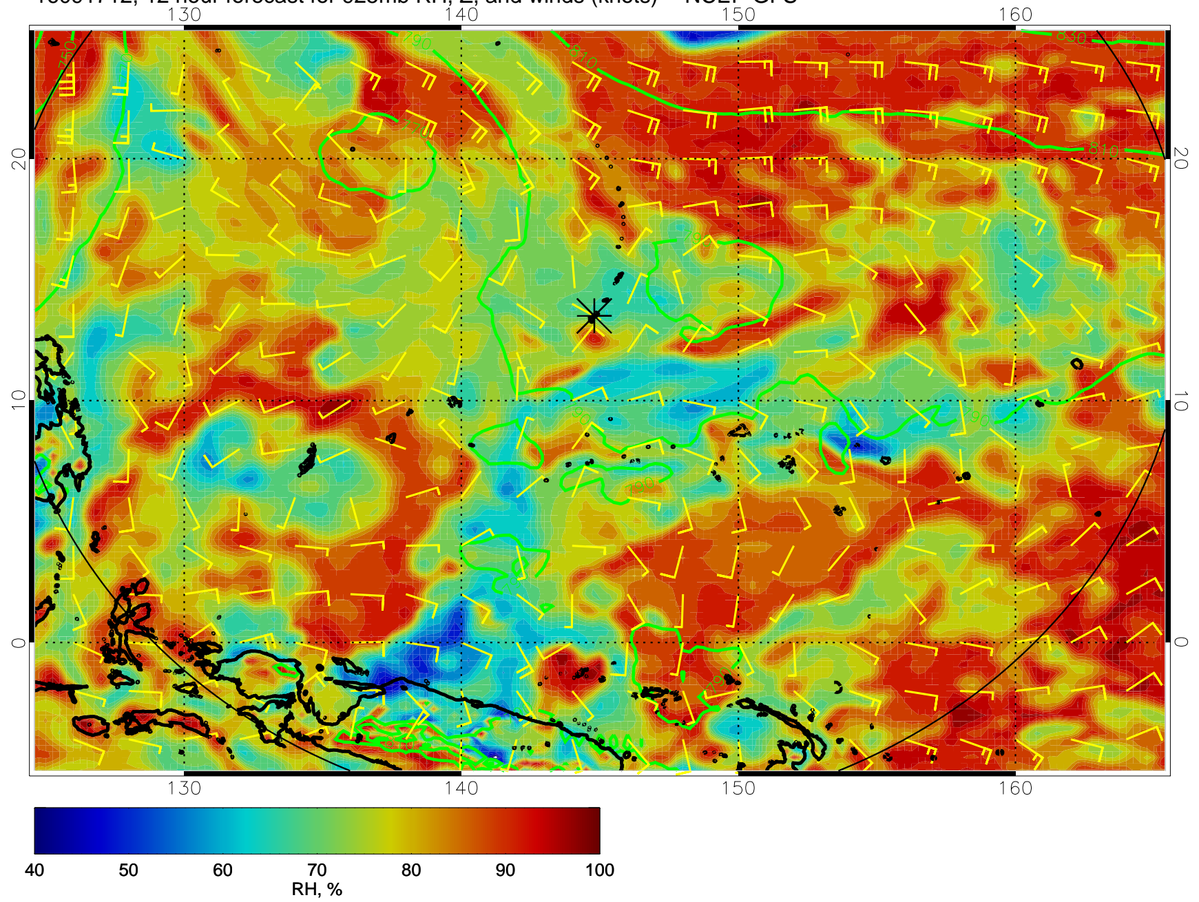
16091712, 12 hour forecast for 925mb RH, Z, and winds (knots) -- NCEP GFS
