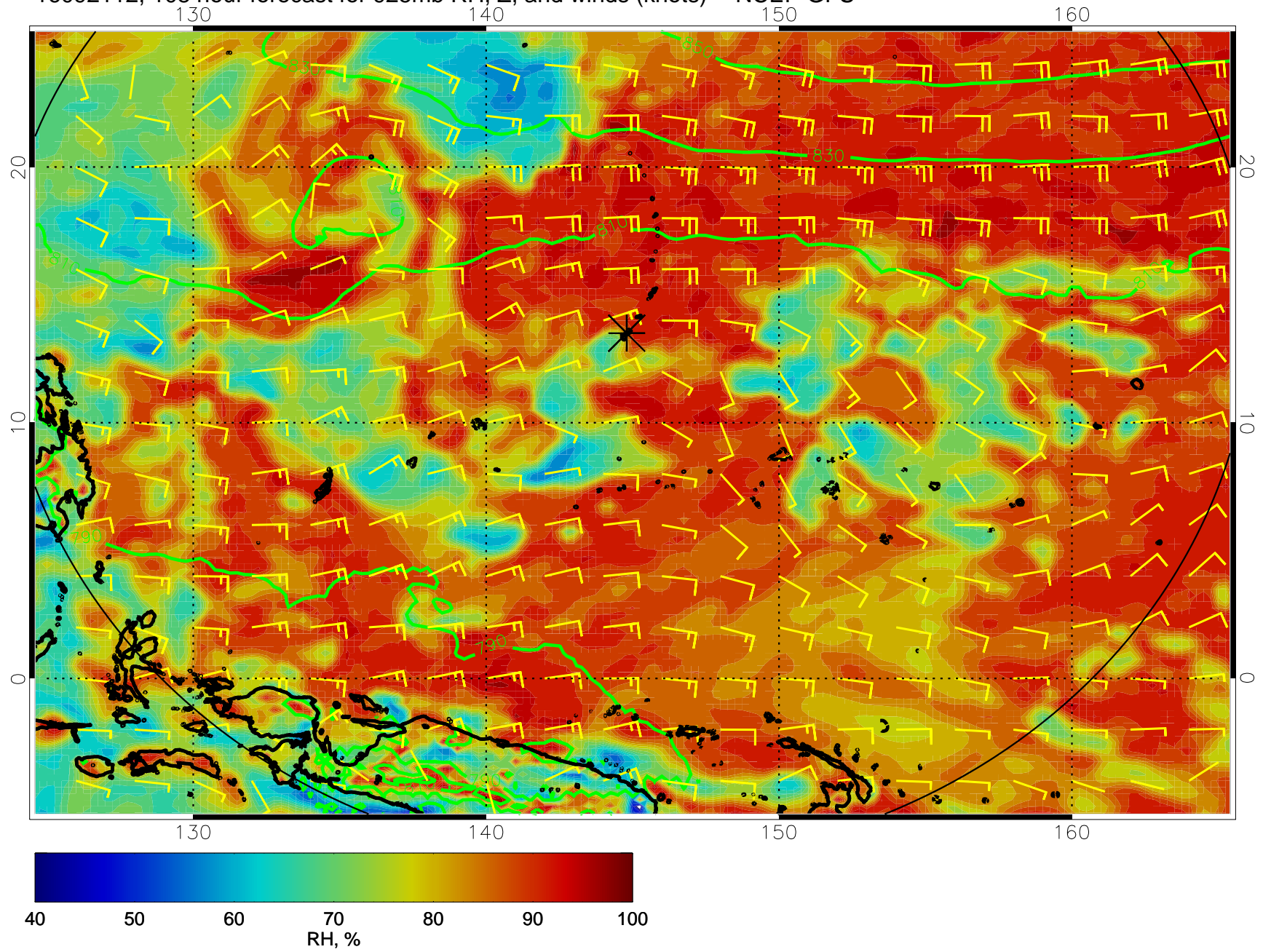
16092112, 108 hour forecast for 925mb RH, Z, and winds (knots) -- NCEP GFS
