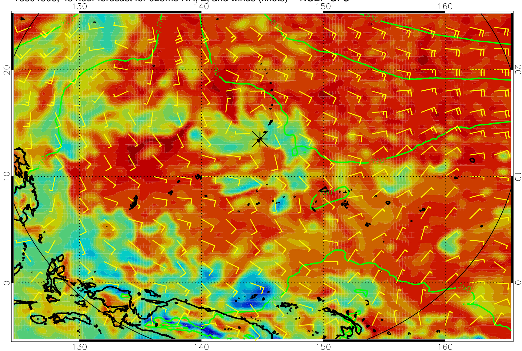
16091900, 48 hour forecast for 925mb RH, Z, and winds (knots) -- NCEP GFS
