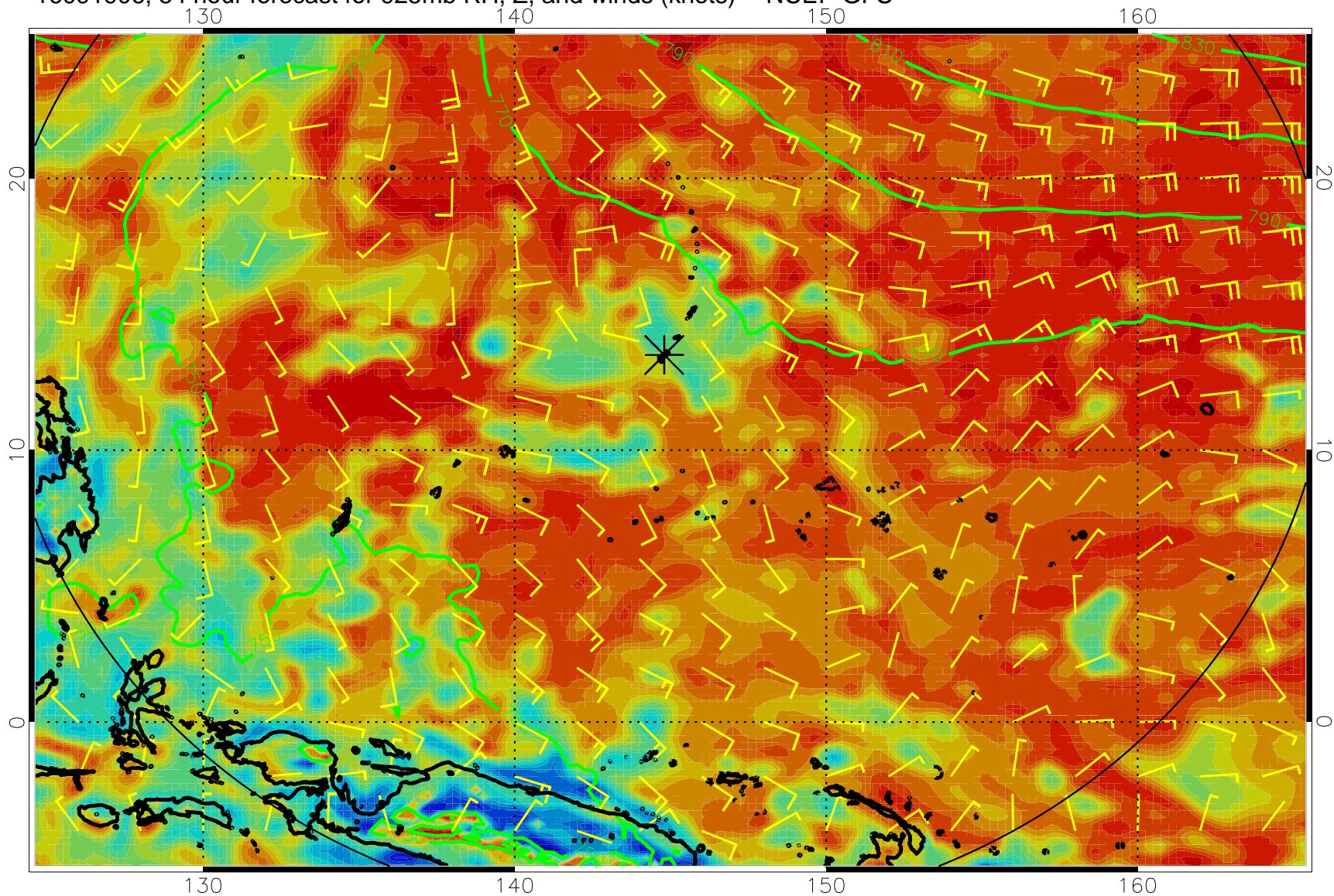
16091906, 54 hour forecast for 925mb RH, Z, and winds (knots) -- NCEP GFS
