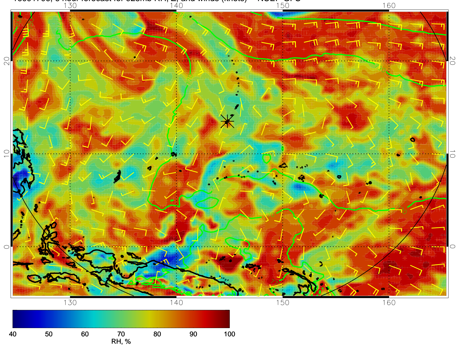
16091706, 6 hour forecast for 925mb RH, Z, and winds (knots) -- NCEP GFS
