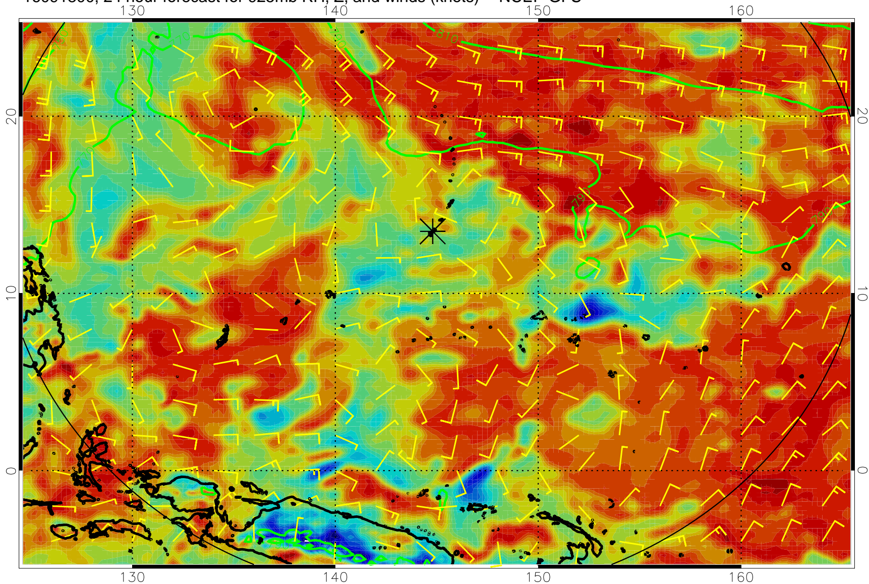
16091800, 24 hour forecast for 925mb RH, Z, and winds (knots) -- NCEP GFS
