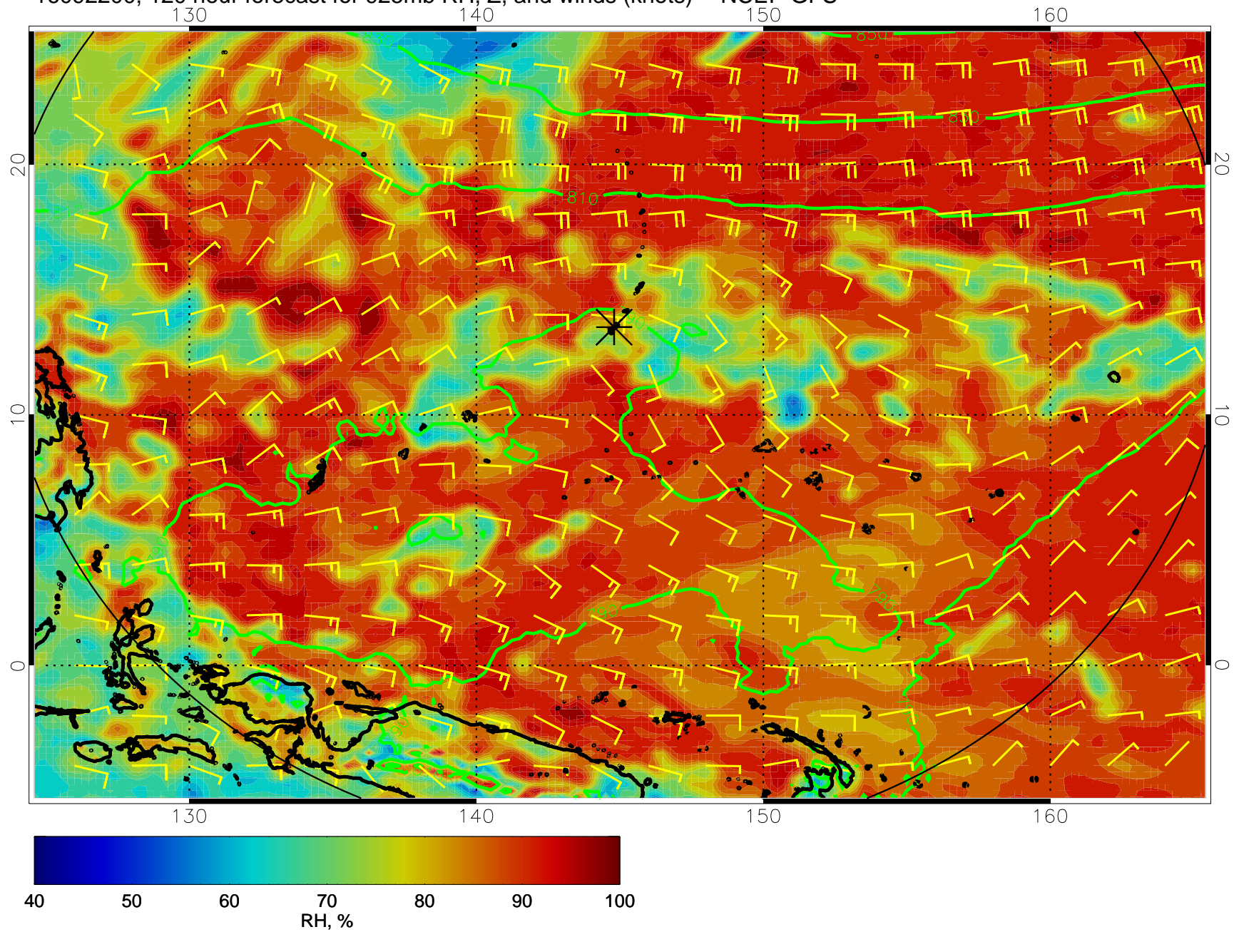
16092200, 120 hour forecast for 925mb RH, Z, and winds (knots) -- NCEP GFS
