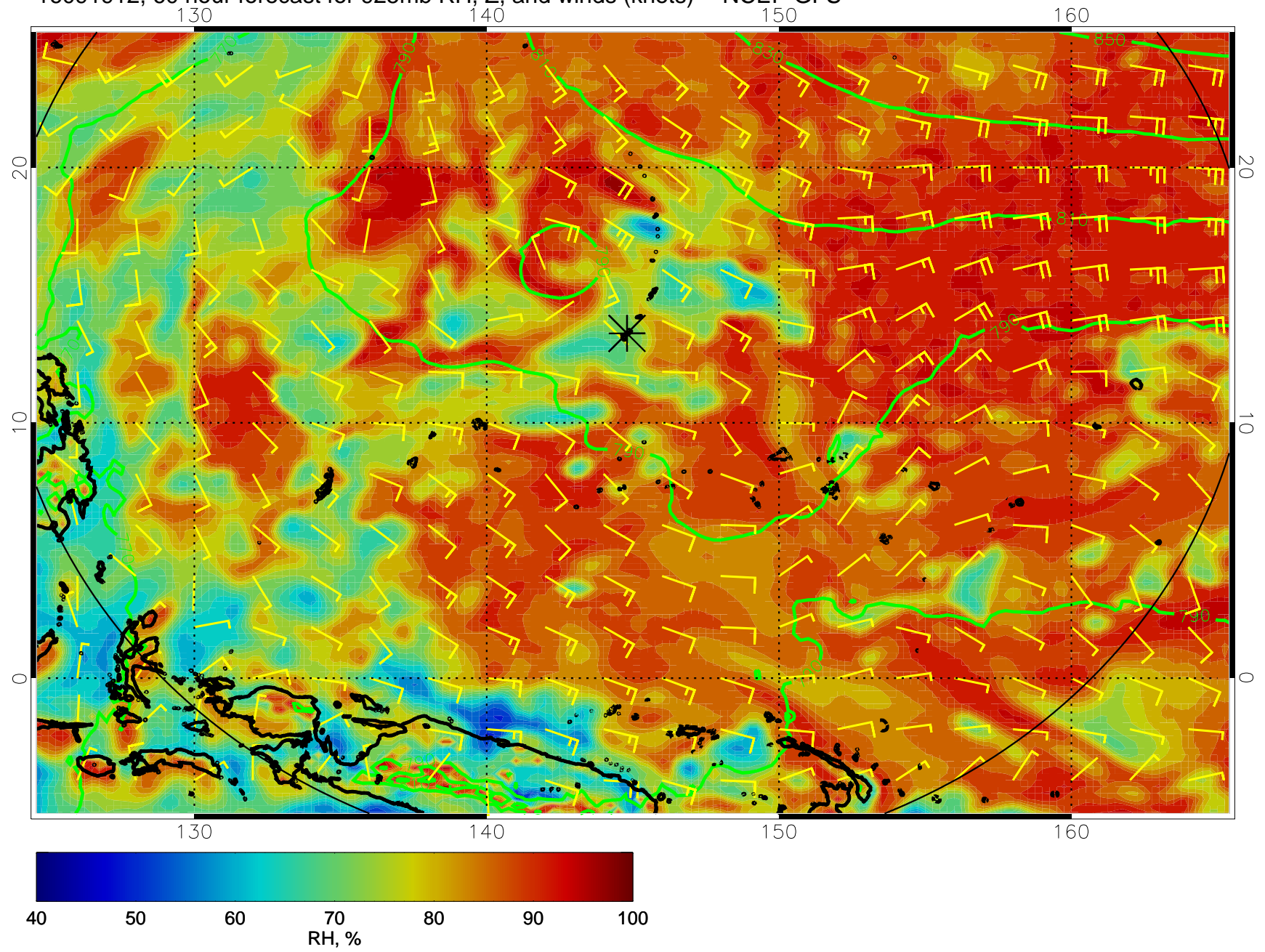
16091912, 60 hour forecast for 925mb RH, Z, and winds (knots) -- NCEP GFS
