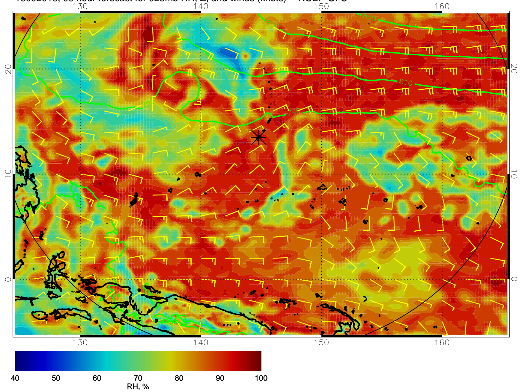
16092018, 90 hour forecast for 925mb RH, Z, and winds (knots) -- NCEP GFS
