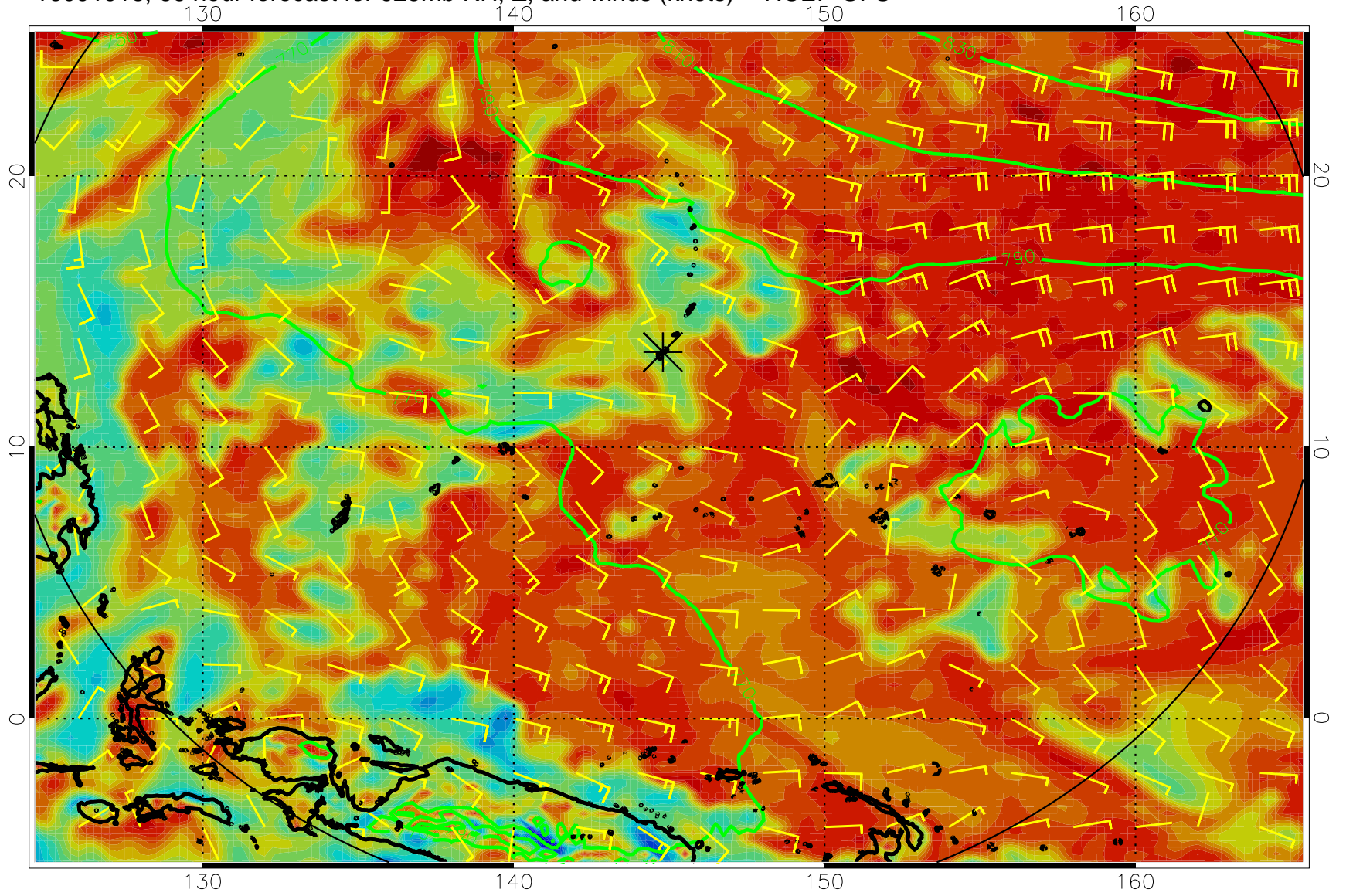
16091918, 66 hour forecast for 925mb RH, Z, and winds (knots) -- NCEP GFS
