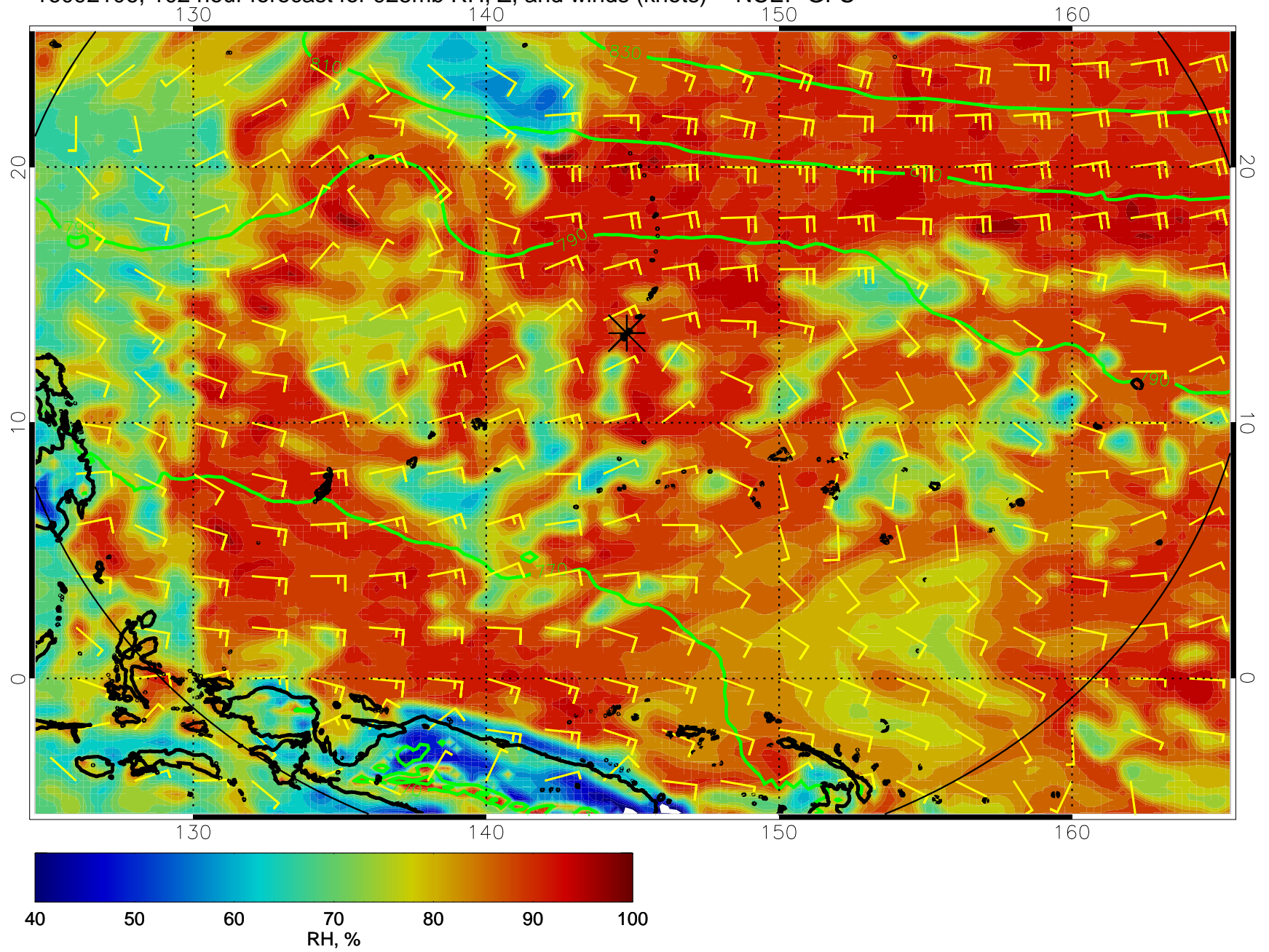
16092106, 102 hour forecast for 925mb RH, Z, and winds (knots) -- NCEP GFS
