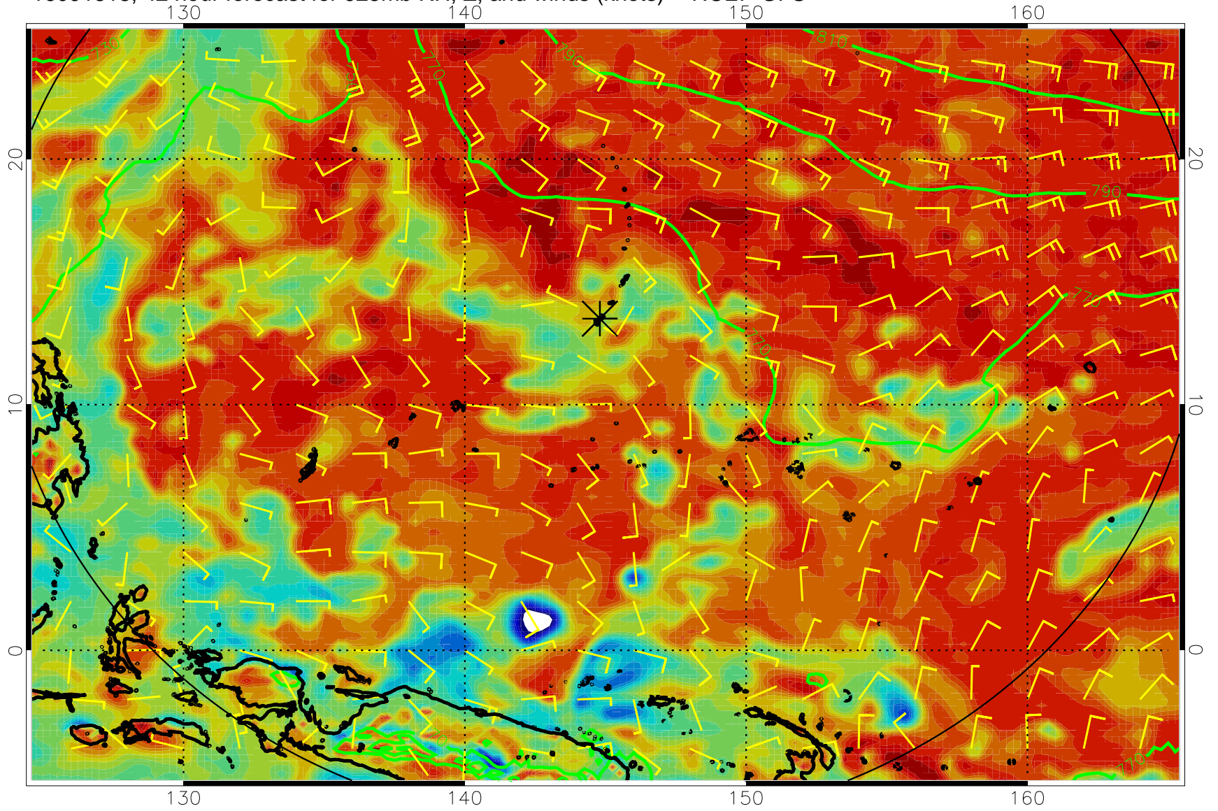
16091818, 42 hour forecast for 925mb RH, Z, and winds (knots) -- NCEP GFS
