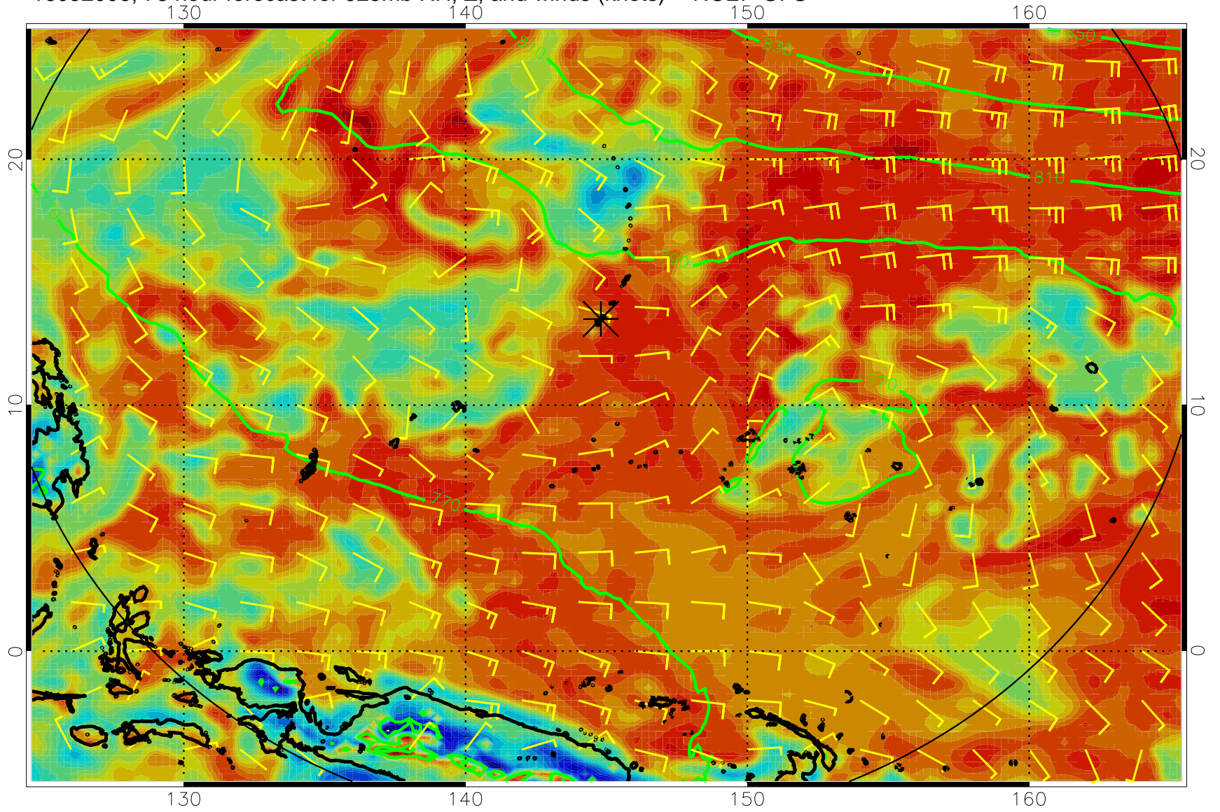
16092006, 78 hour forecast for 925mb RH, Z, and winds (knots) -- NCEP GFS
