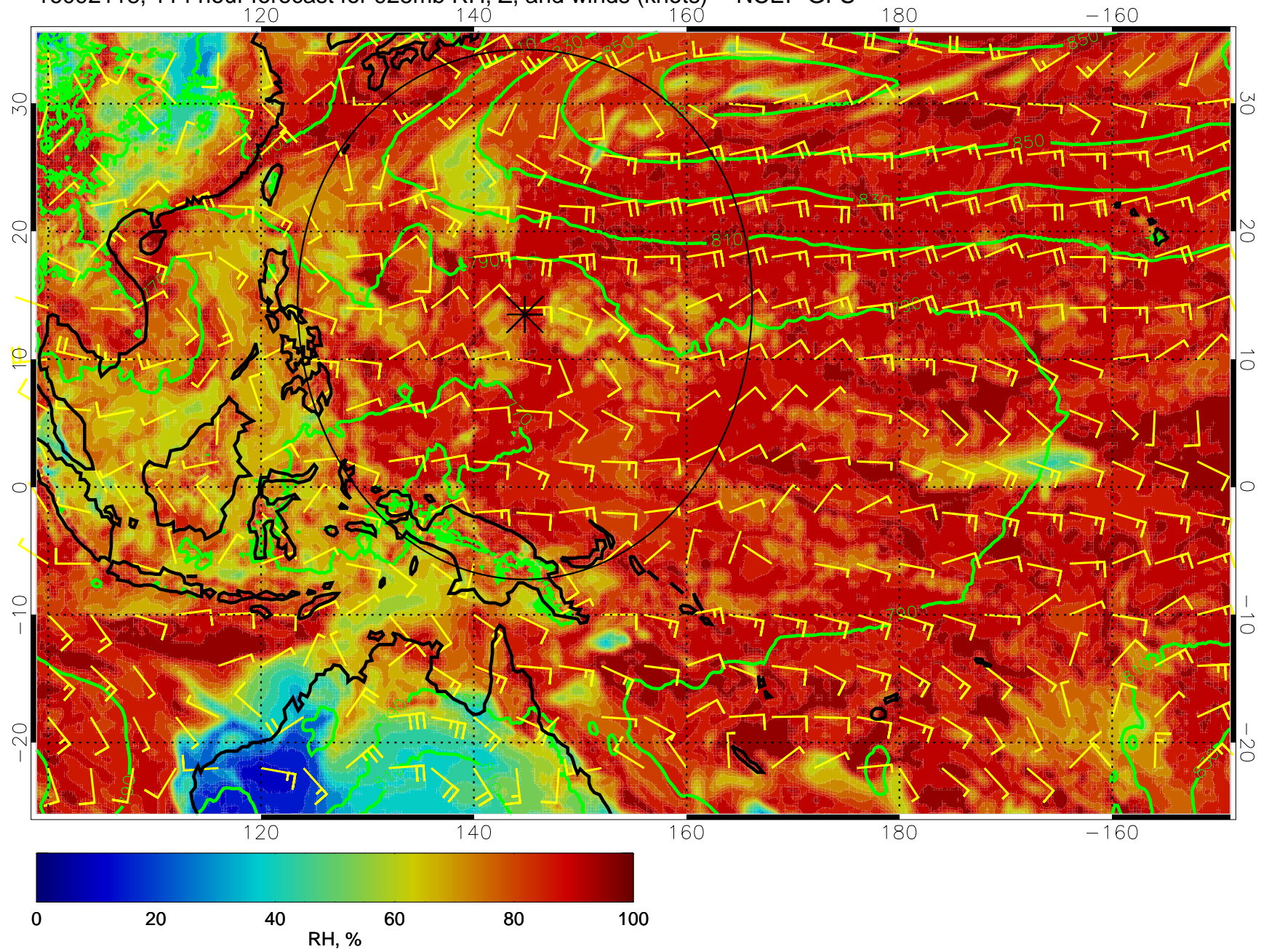
16092118, 114 hour forecast for 925mb RH, Z, and winds (knots) -- NCEP GFS
