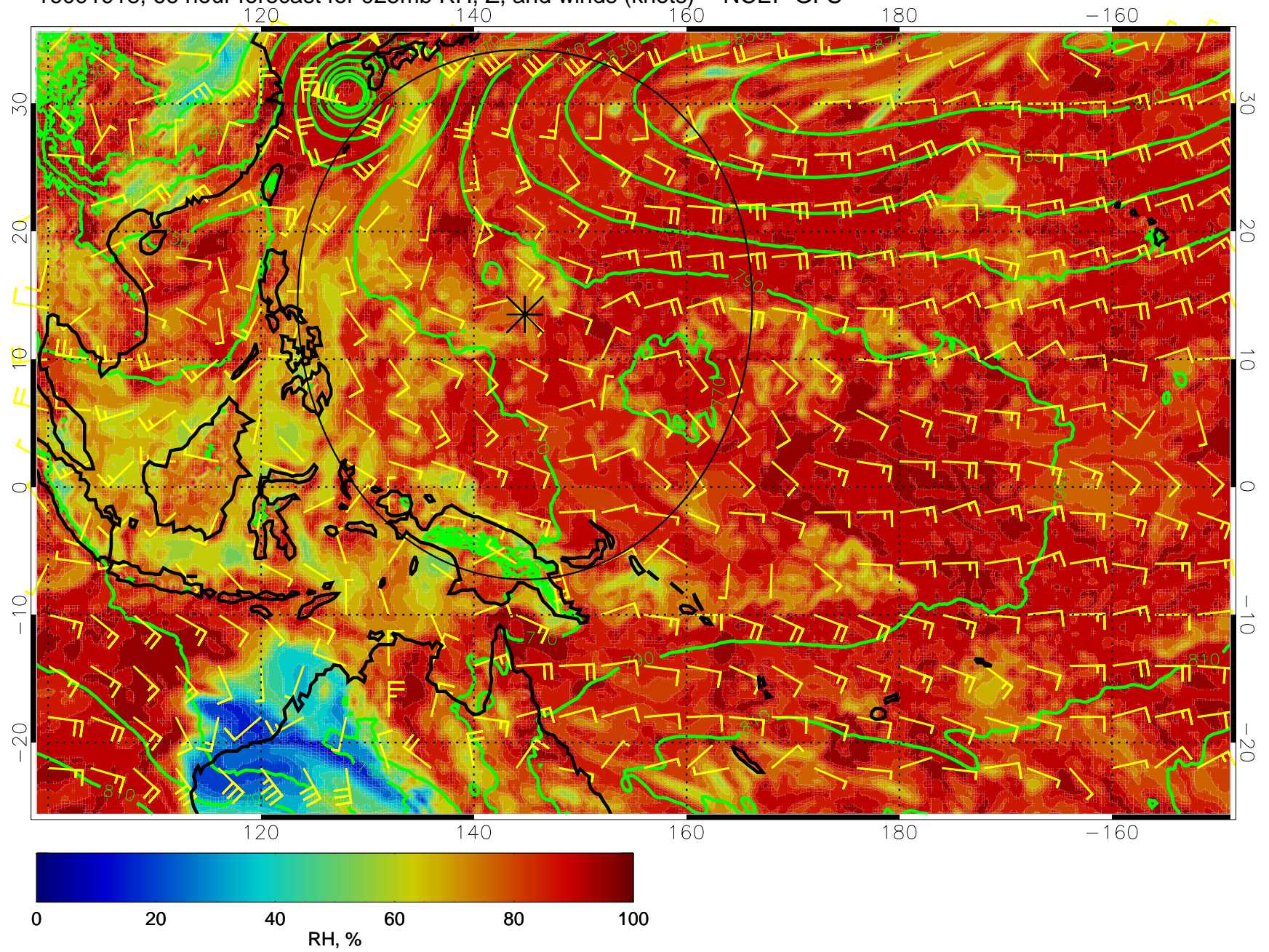
16091918, 66 hour forecast for 925mb RH, Z, and winds (knots) -- NCEP GFS
