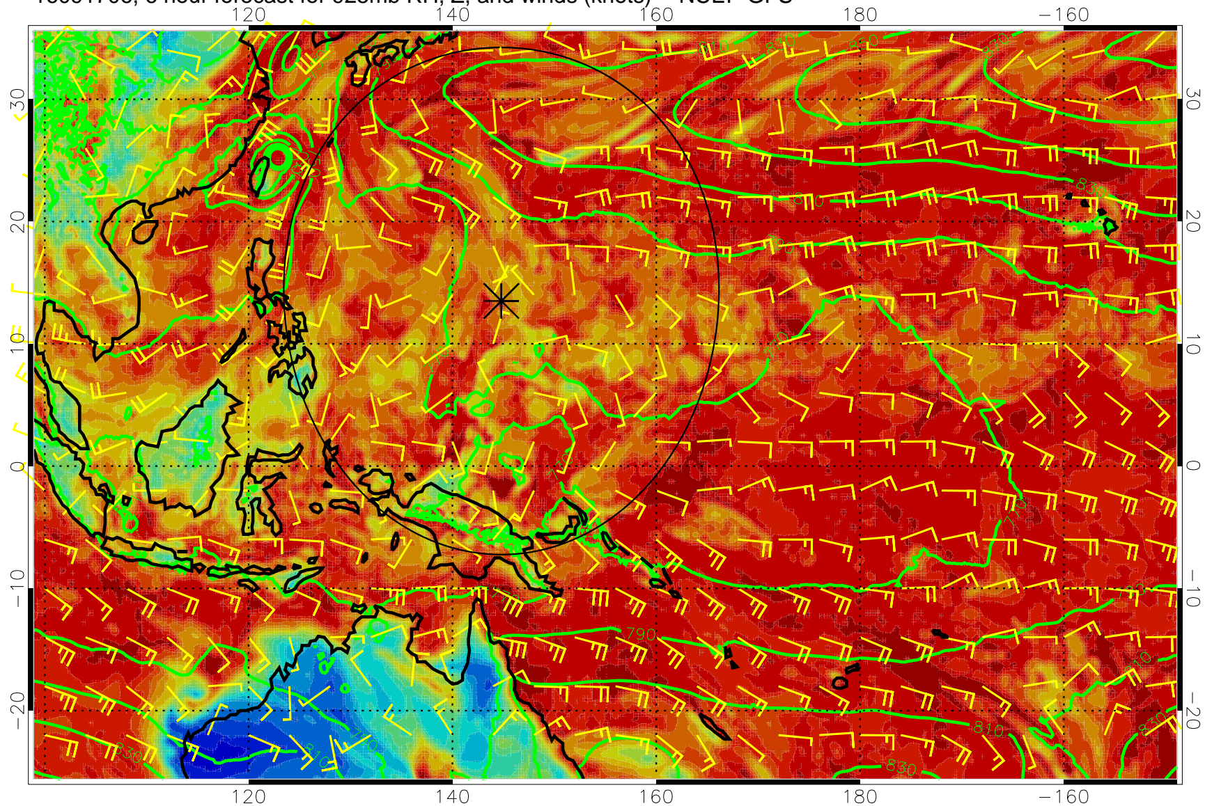
16091706, 6 hour forecast for 925mb RH, Z, and winds (knots) -- NCEP GFS
