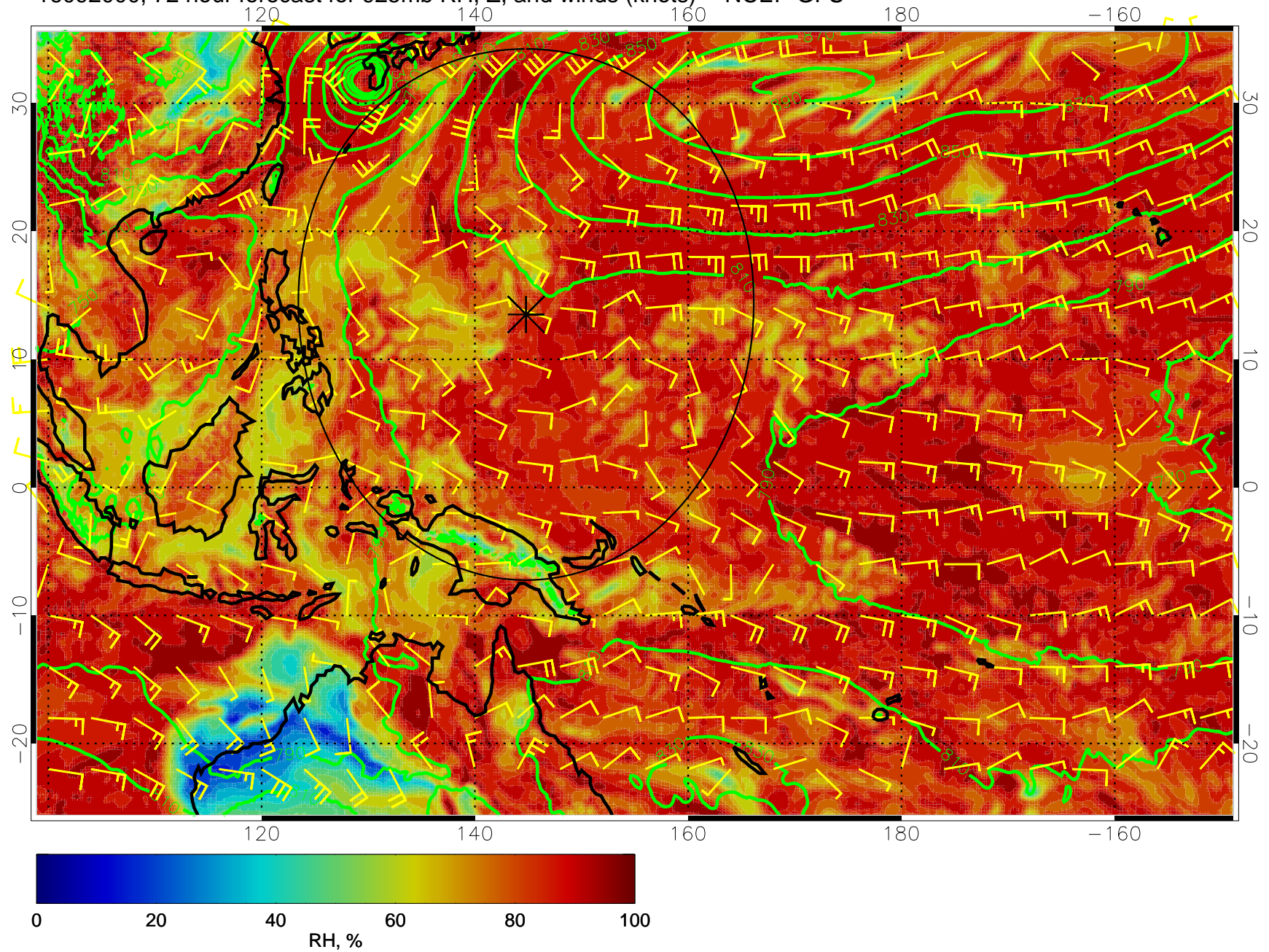
16092000, 72 hour forecast for 925mb RH, Z, and winds (knots) -- NCEP GFS
