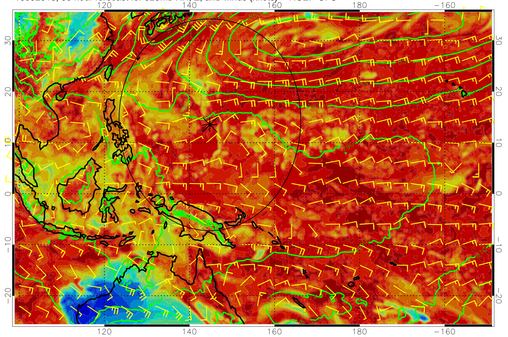
16092018, 90 hour forecast for 925mb RH, Z, and winds (knots) -- NCEP GFS
