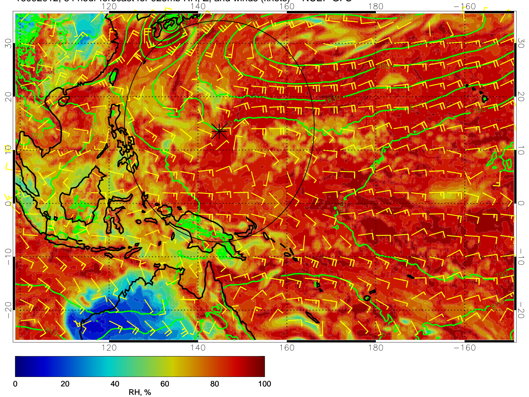
16092012, 84 hour forecast for 925mb RH, Z, and winds (knots) -- NCEP GFS
