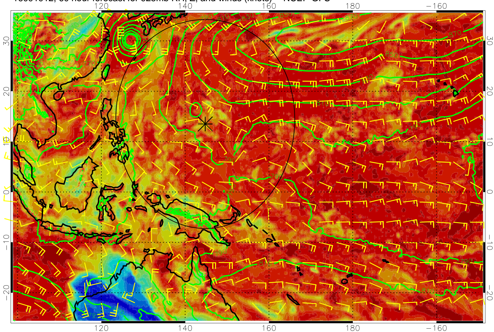
16091912, 60 hour forecast for 925mb RH, Z, and winds (knots) -- NCEP GFS
