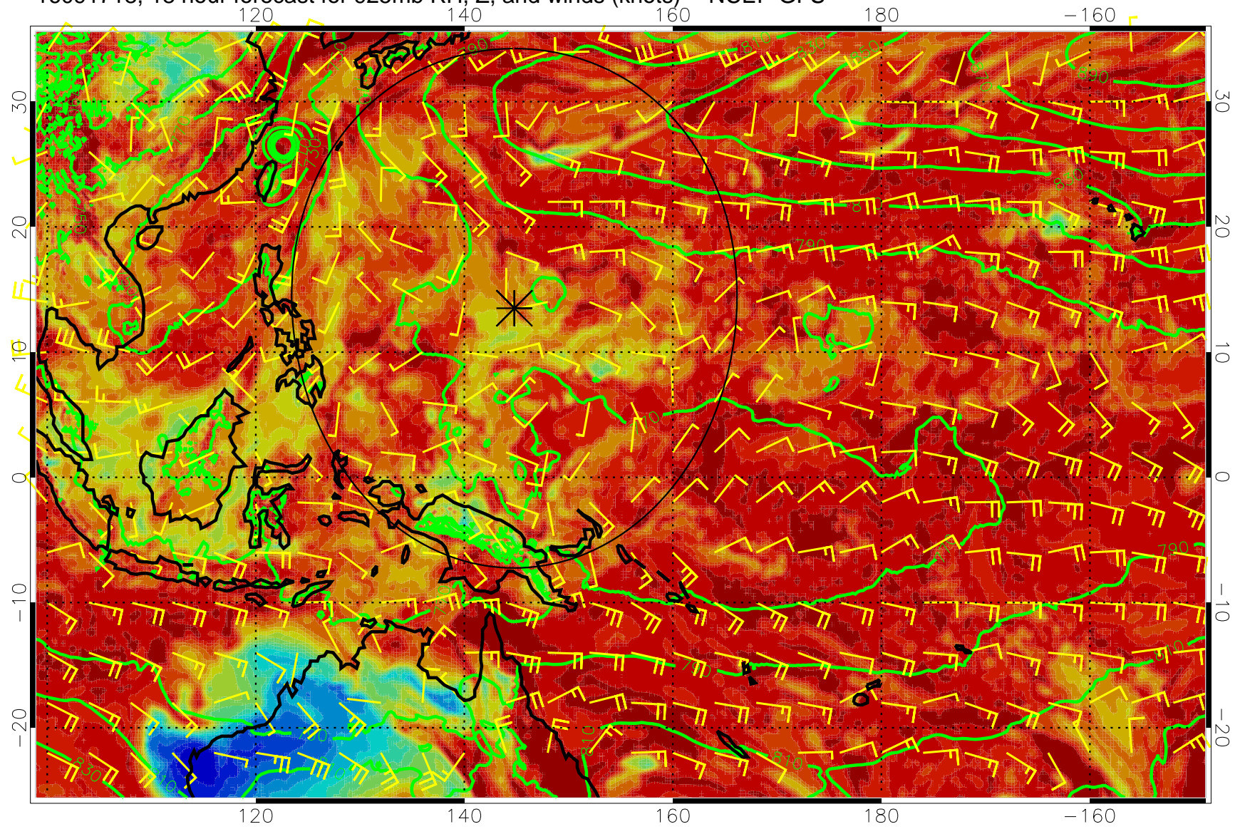
16091718, 18 hour forecast for 925mb RH, Z, and winds (knots) -- NCEP GFS
