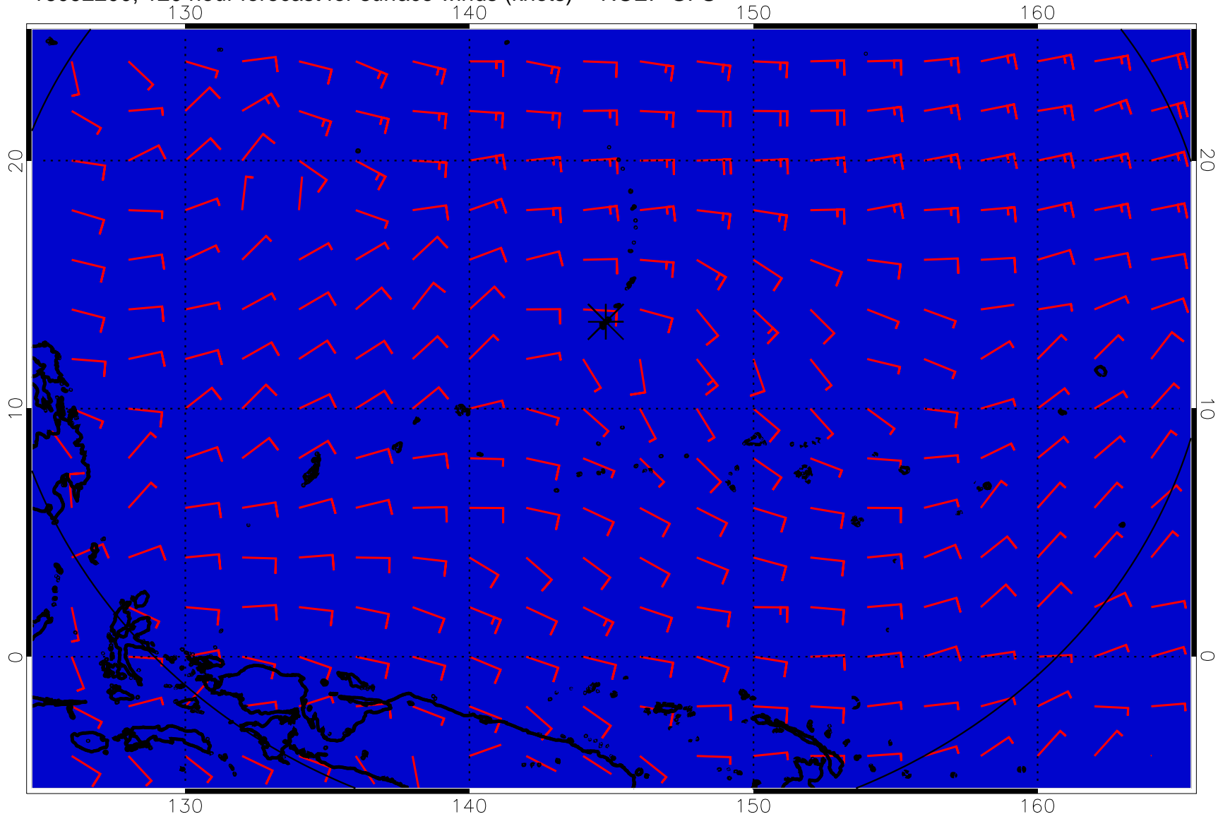
16092200, 120 hour forecast for surface winds (knots) -- NCEP GFS
