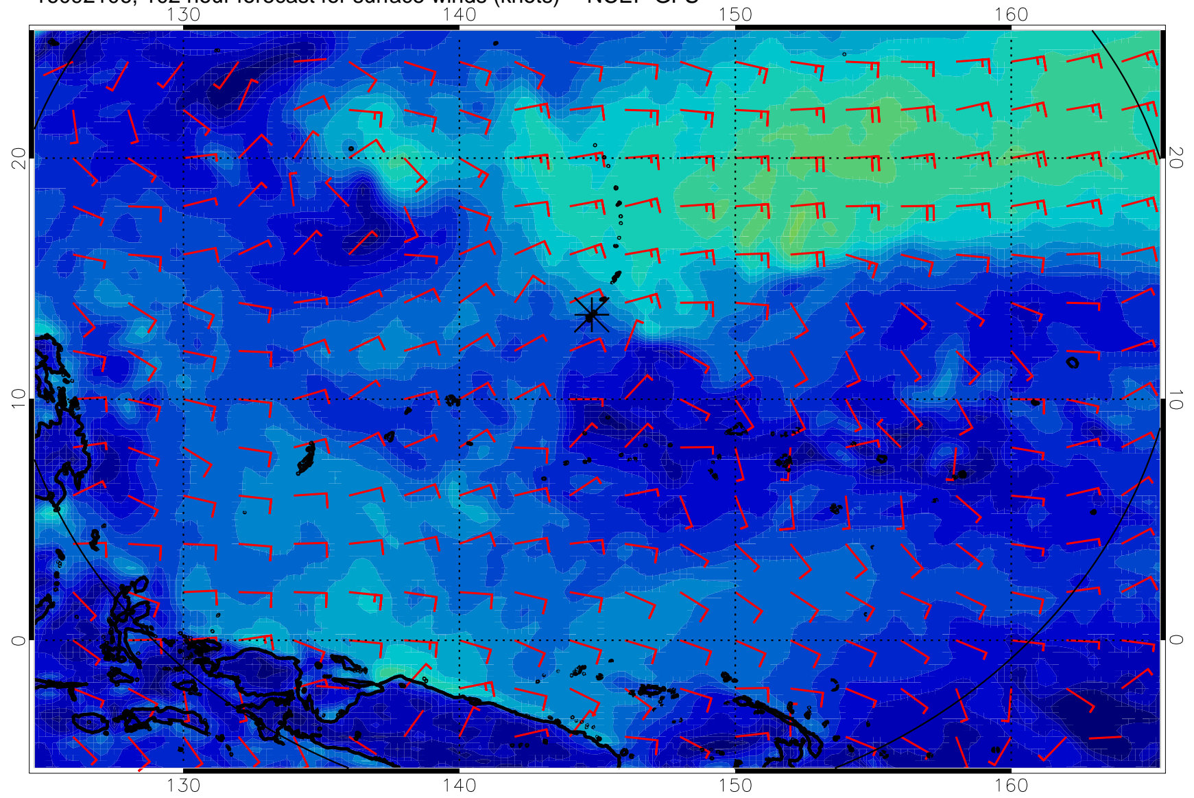
16092106, 102 hour forecast for surface winds (knots) -- NCEP GFS
