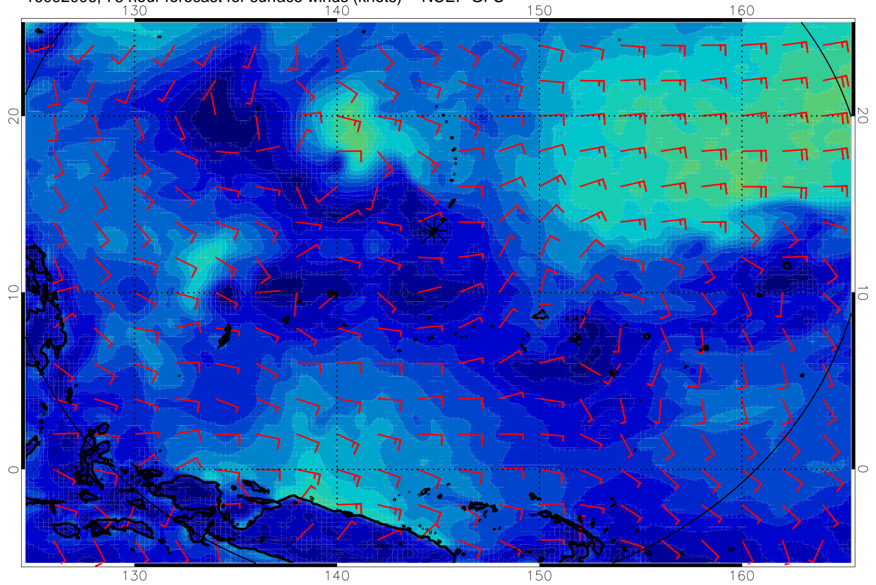
16092006, 78 hour forecast for surface winds (knots) -- NCEP GFS
