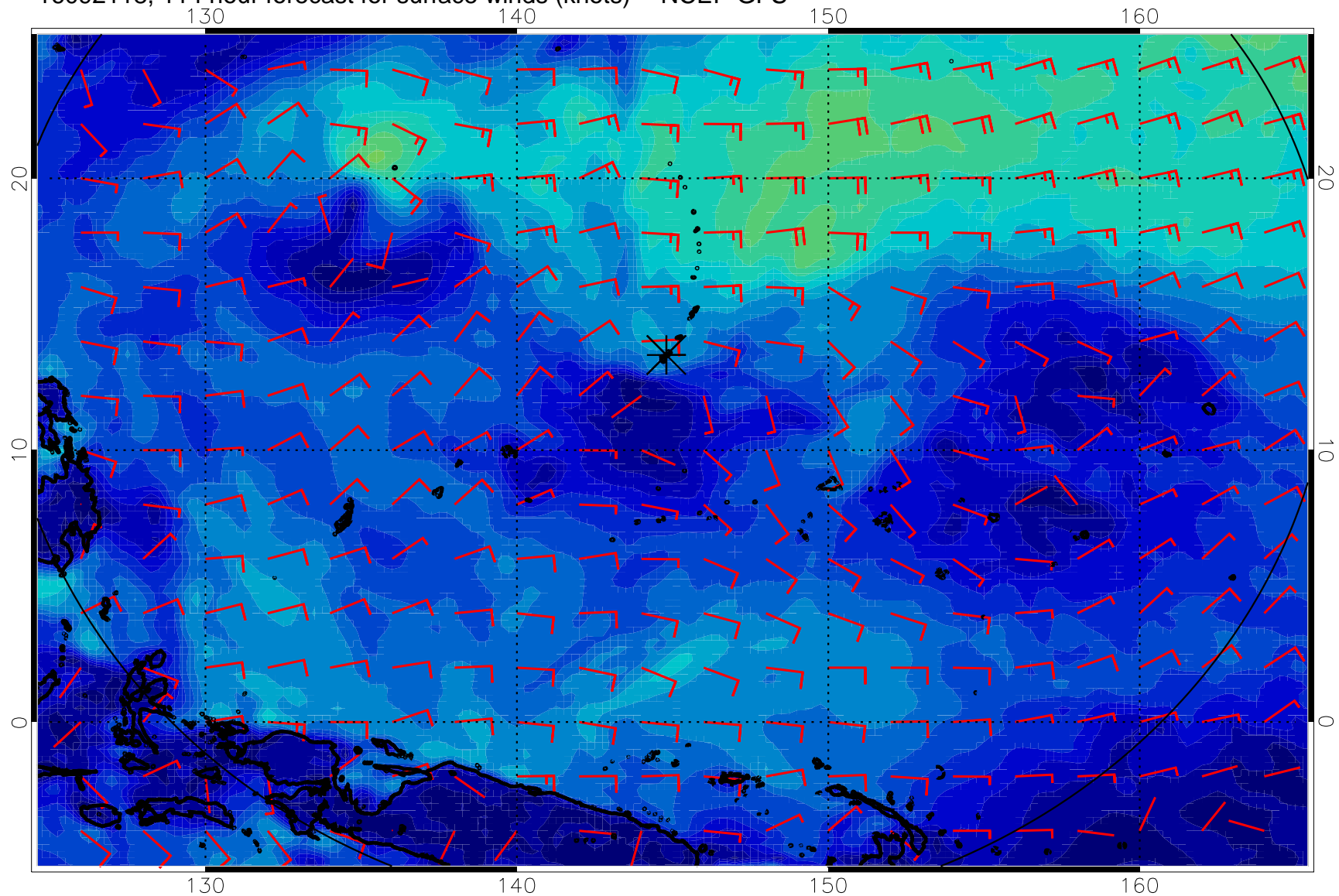
16092118, 114 hour forecast for surface winds (knots) -- NCEP GFS
