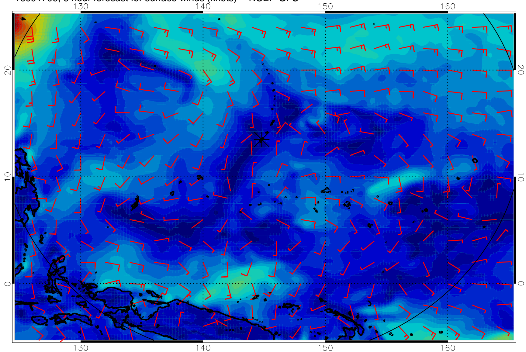
16091706, 6 hour forecast for surface winds (knots) -- NCEP GFS
