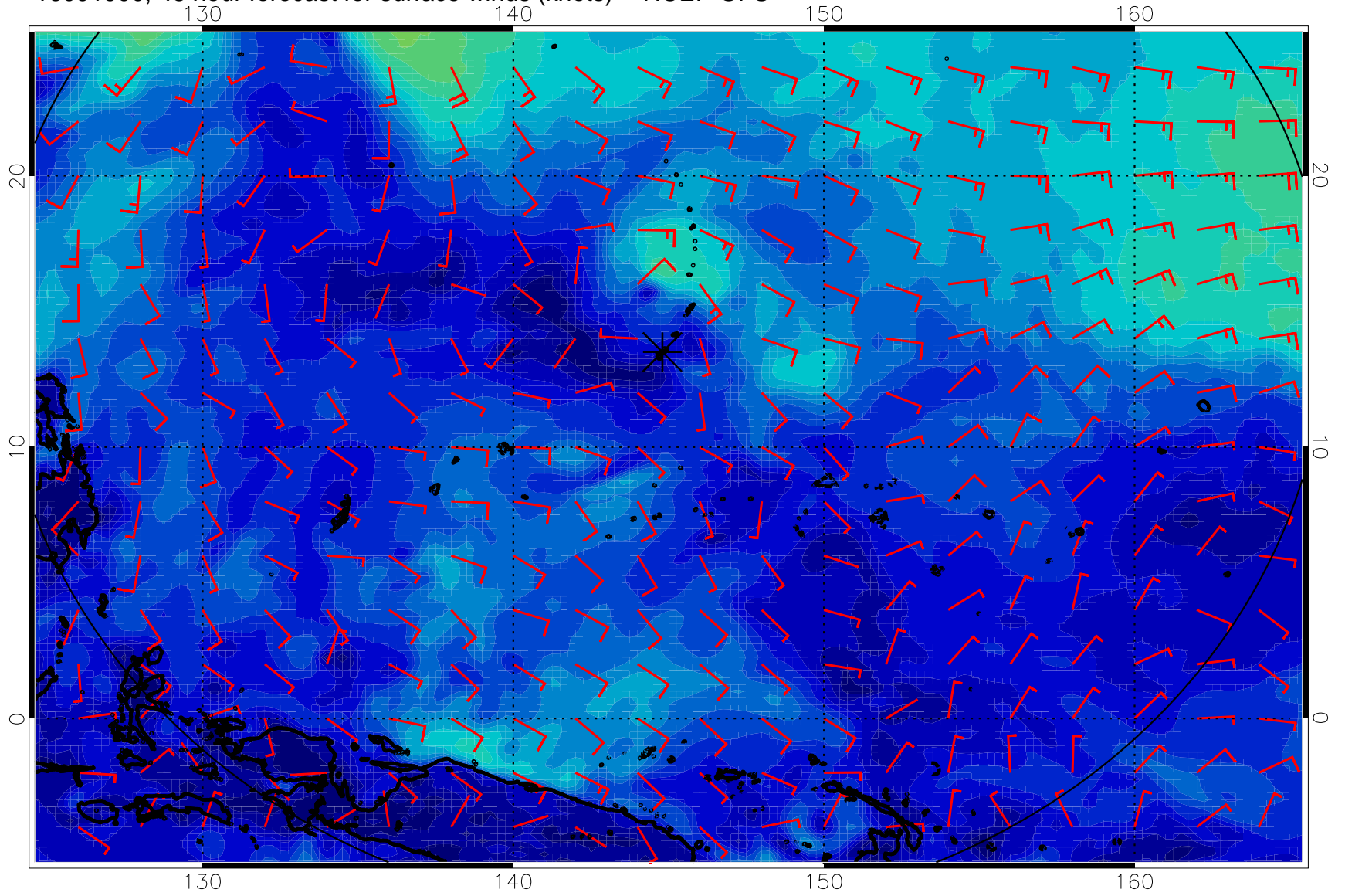
16091900, 48 hour forecast for surface winds (knots) -- NCEP GFS
