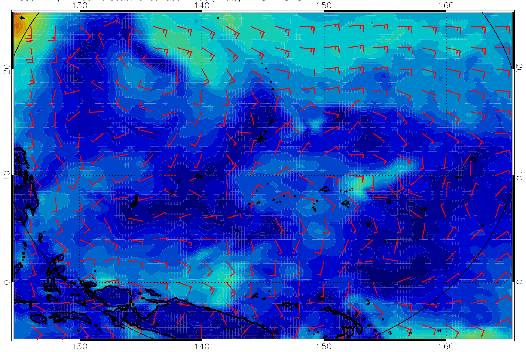
16091712, 12 hour forecast for surface winds (knots) -- NCEP GFS
