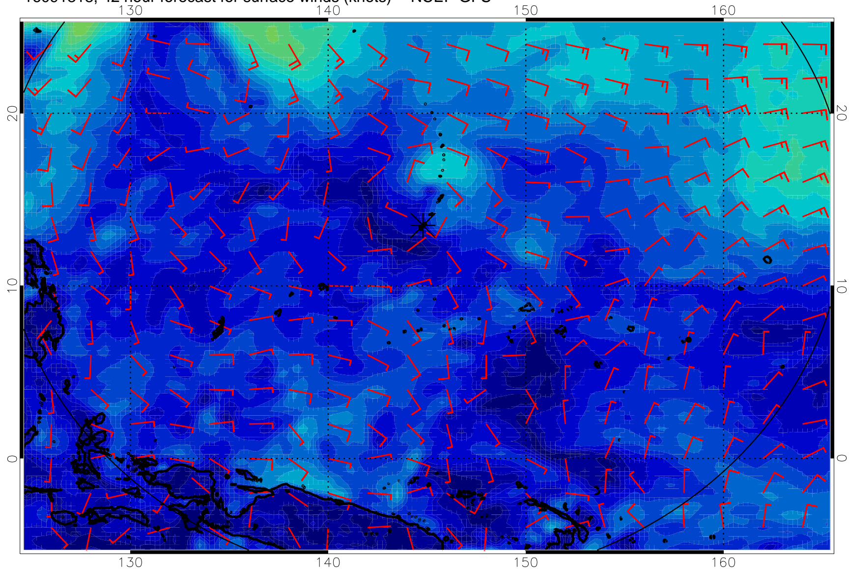
16091818, 42 hour forecast for surface winds (knots) -- NCEP GFS
