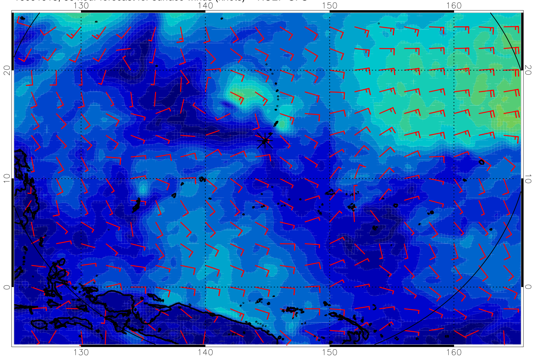
16091918, 66 hour forecast for surface winds (knots) -- NCEP GFS
