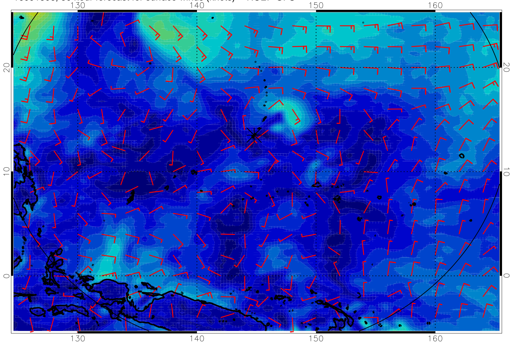
16091806, 30 hour forecast for surface winds (knots) -- NCEP GFS
