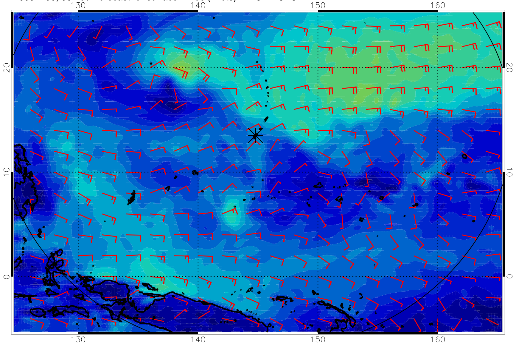
16092100, 96 hour forecast for surface winds (knots) -- NCEP GFS
