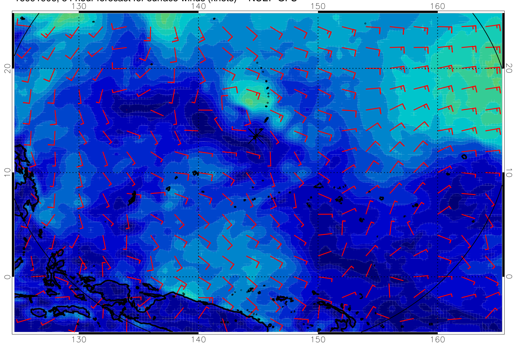
16091906, 54 hour forecast for surface winds (knots) -- NCEP GFS
