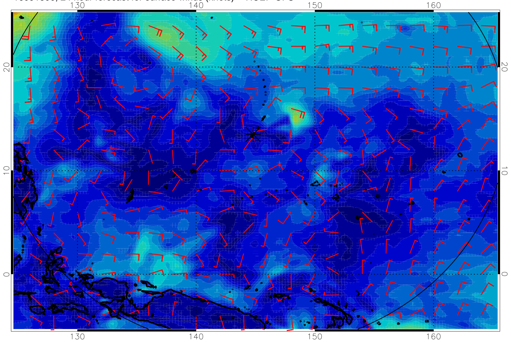
16091800, 24 hour forecast for surface winds (knots) -- NCEP GFS
