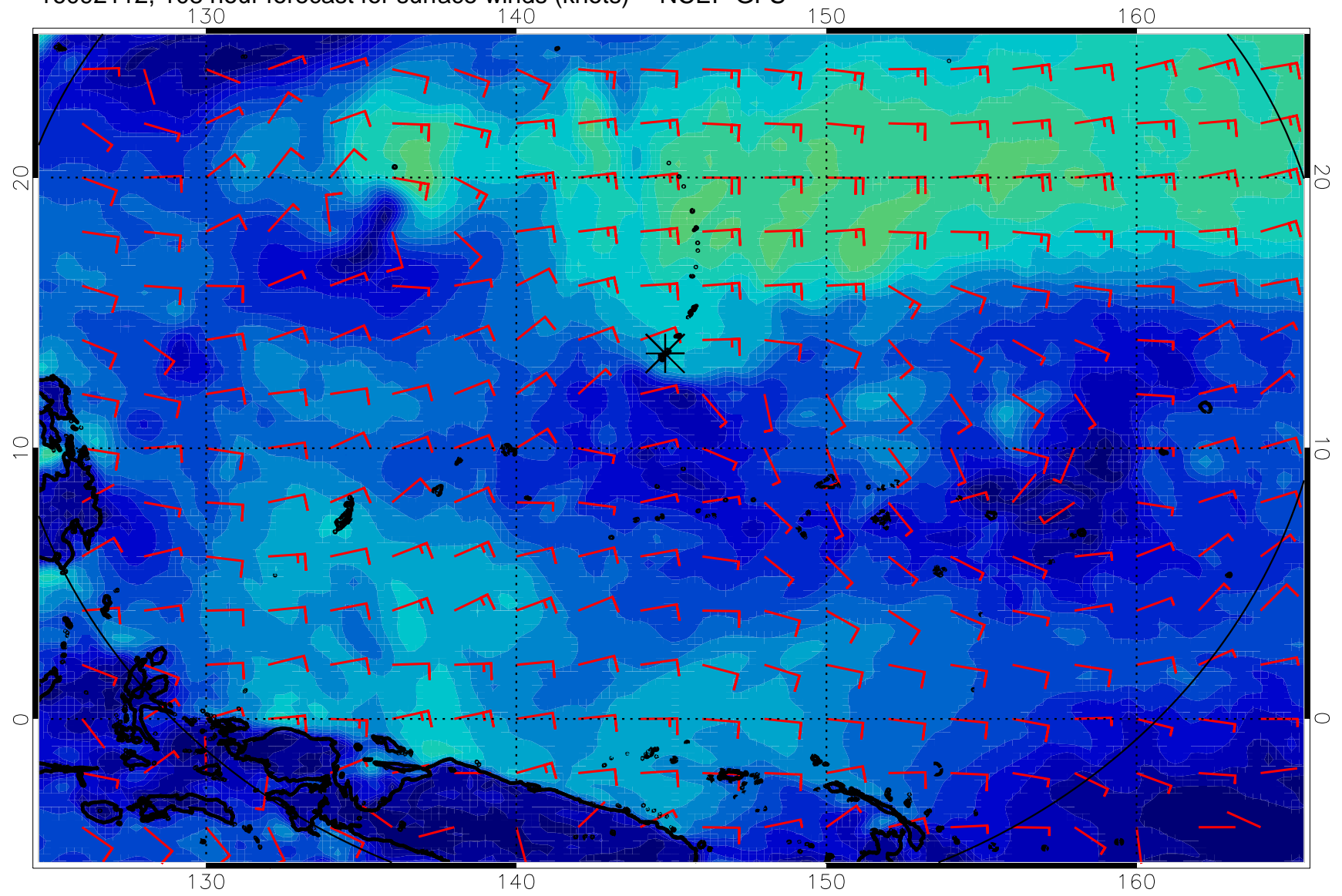
16092112, 108 hour forecast for surface winds (knots) -- NCEP GFS
