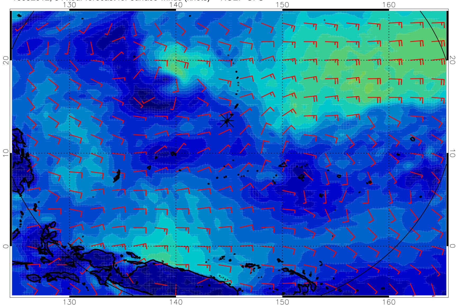
16092012, 84 hour forecast for surface winds (knots) -- NCEP GFS
