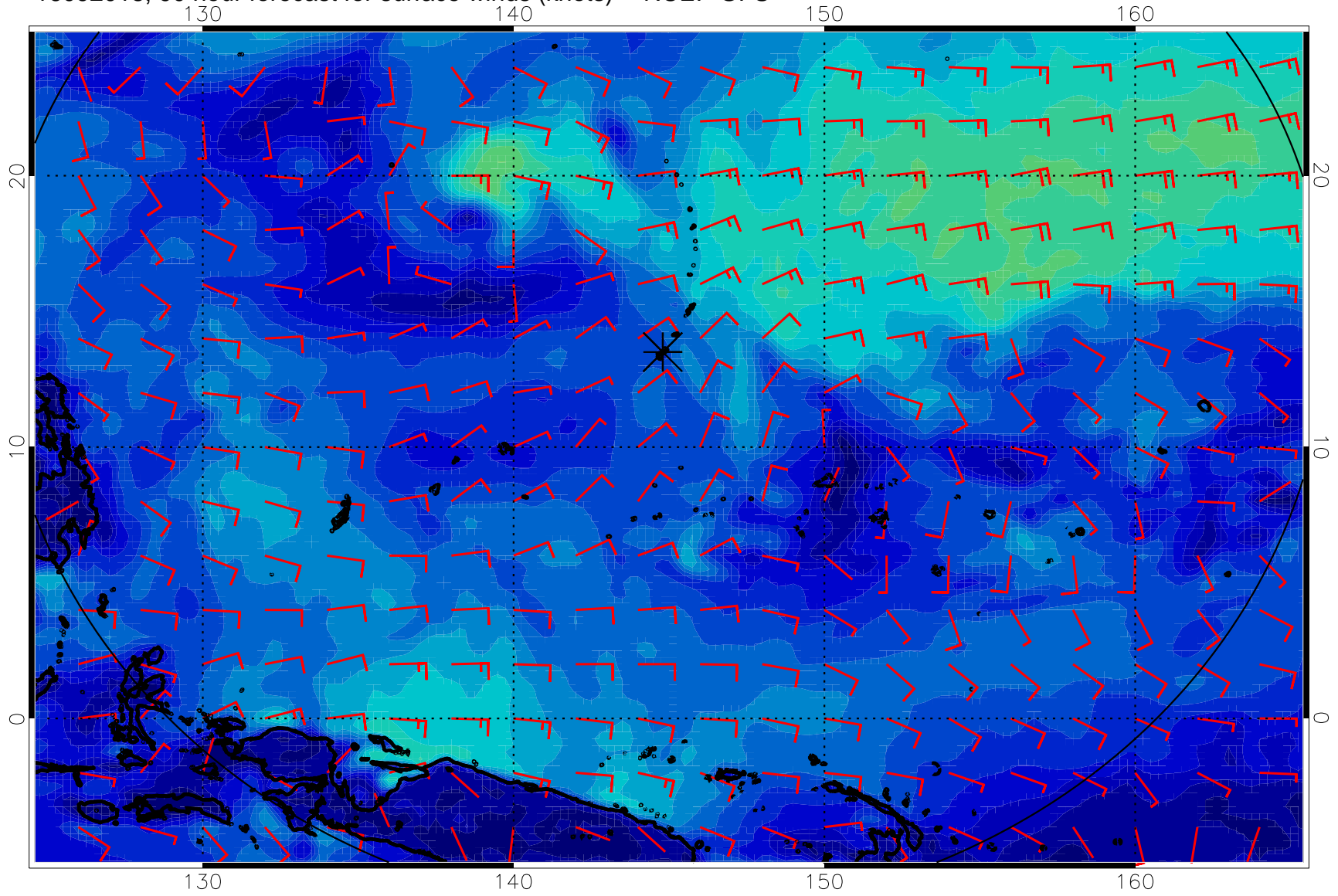
16092018, 90 hour forecast for surface winds (knots) -- NCEP GFS
