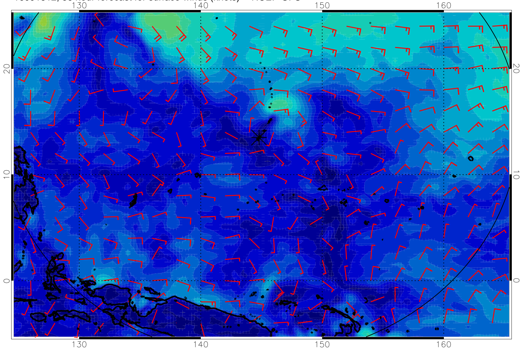
16091812, 36 hour forecast for surface winds (knots) -- NCEP GFS
