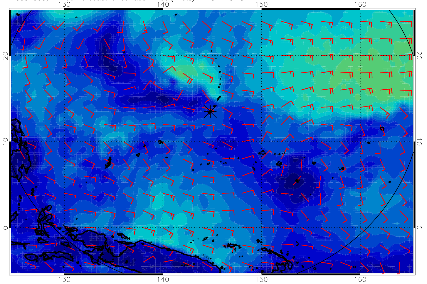
16092000, 72 hour forecast for surface winds (knots) -- NCEP GFS
