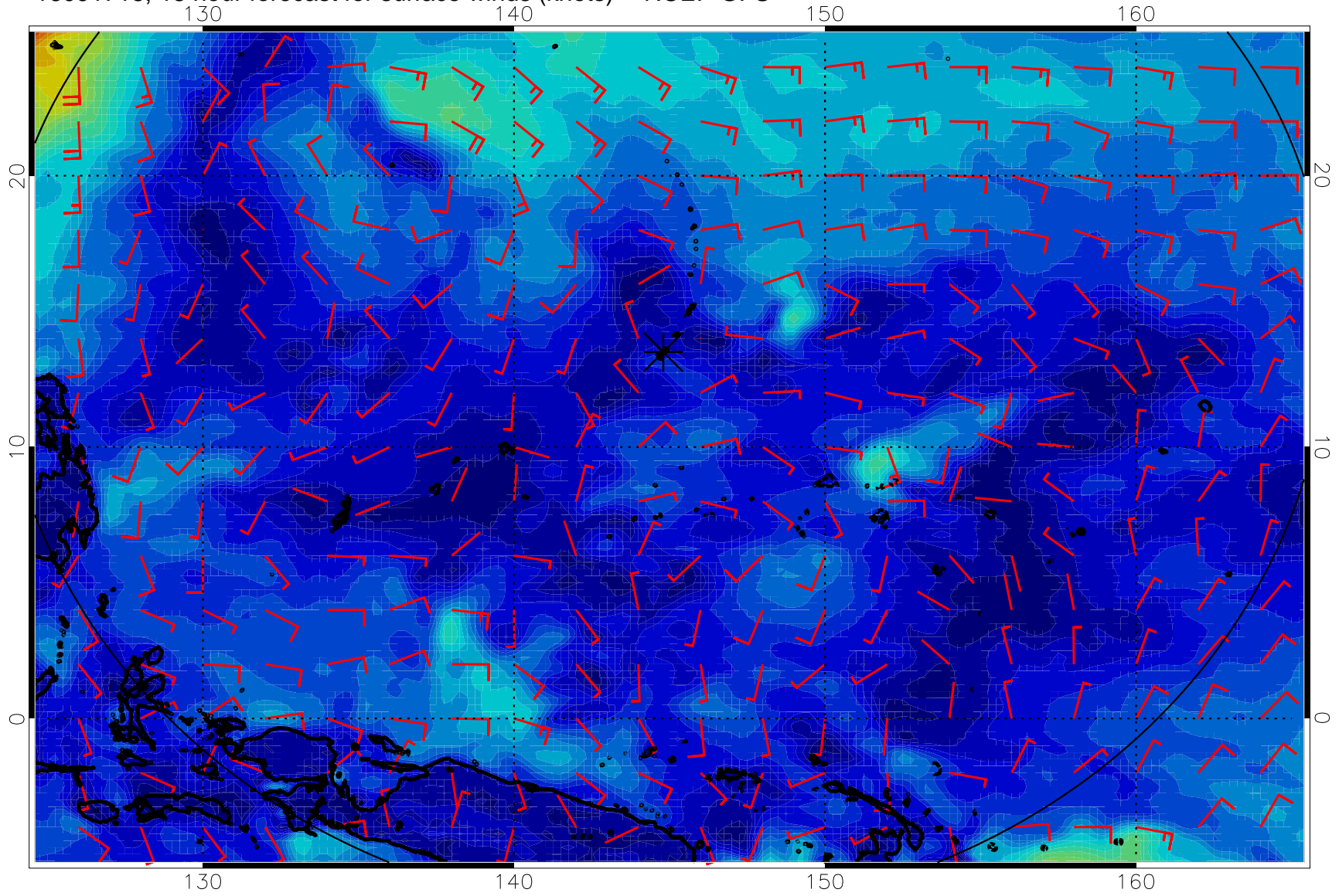
16091718, 18 hour forecast for surface winds (knots) -- NCEP GFS
