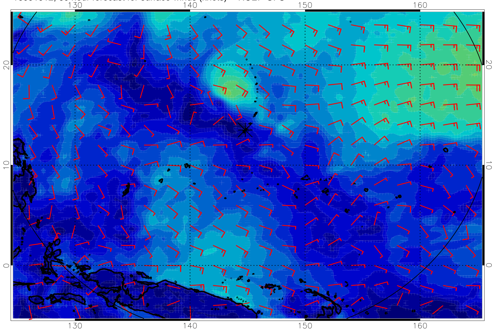
16091912, 60 hour forecast for surface winds (knots) -- NCEP GFS
