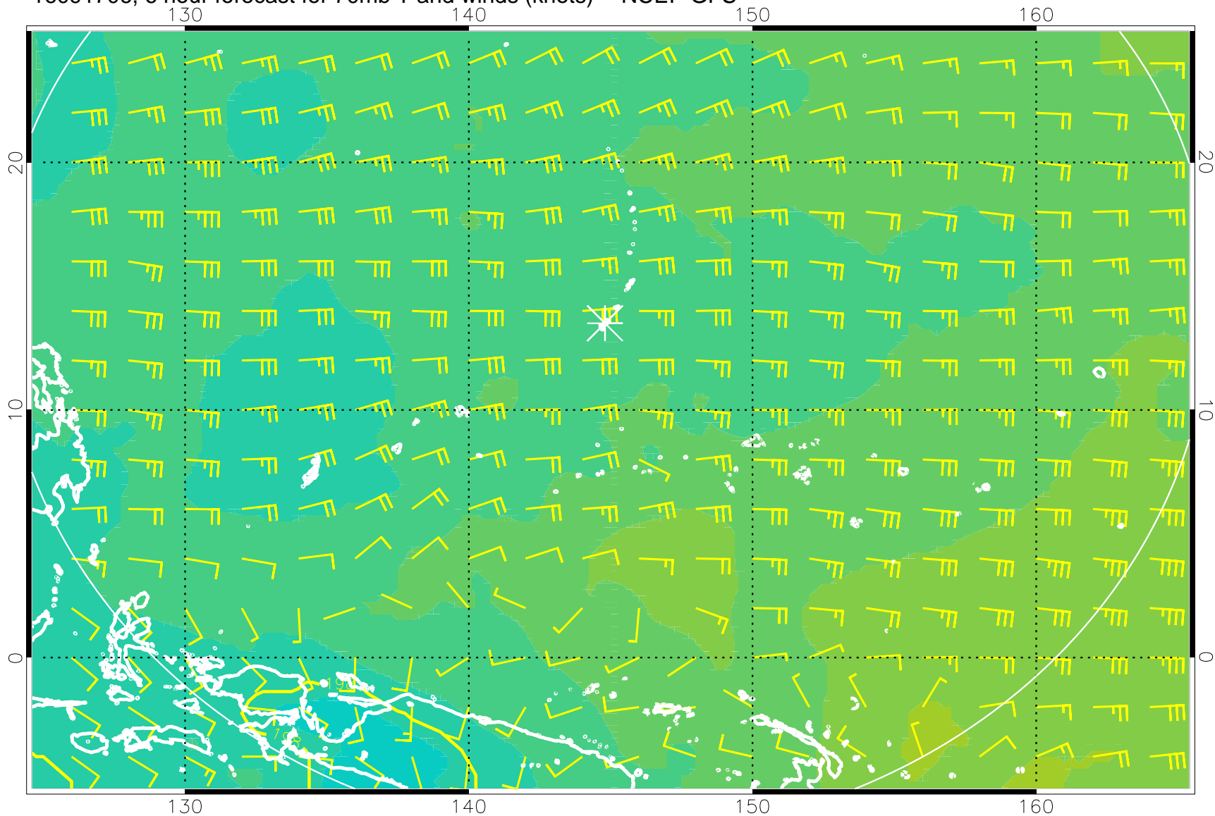
16091706, 6 hour forecast for 70mb T and winds (knots) -- NCEP GFS
