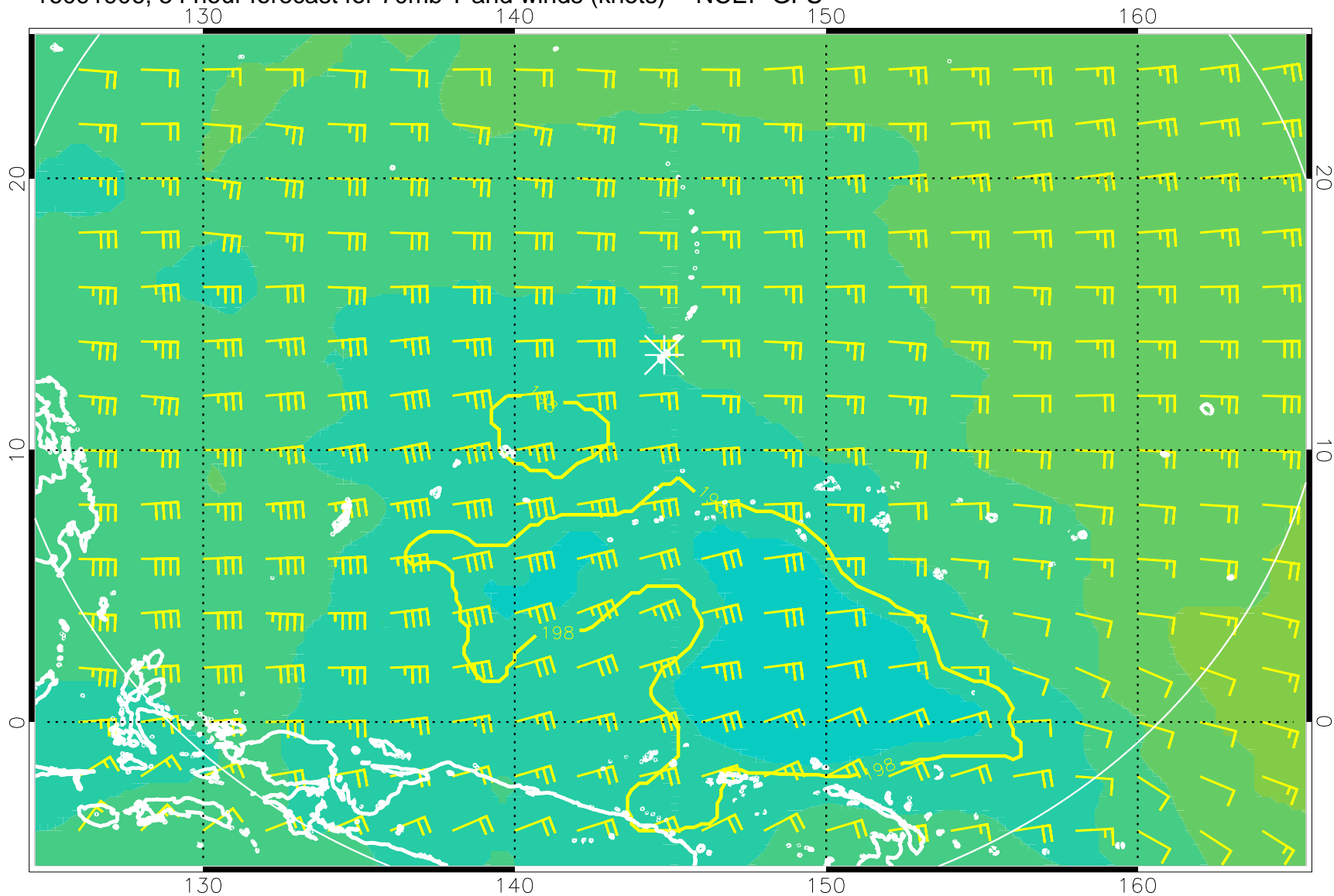
16091906, 54 hour forecast for 70mb T and winds (knots) -- NCEP GFS
