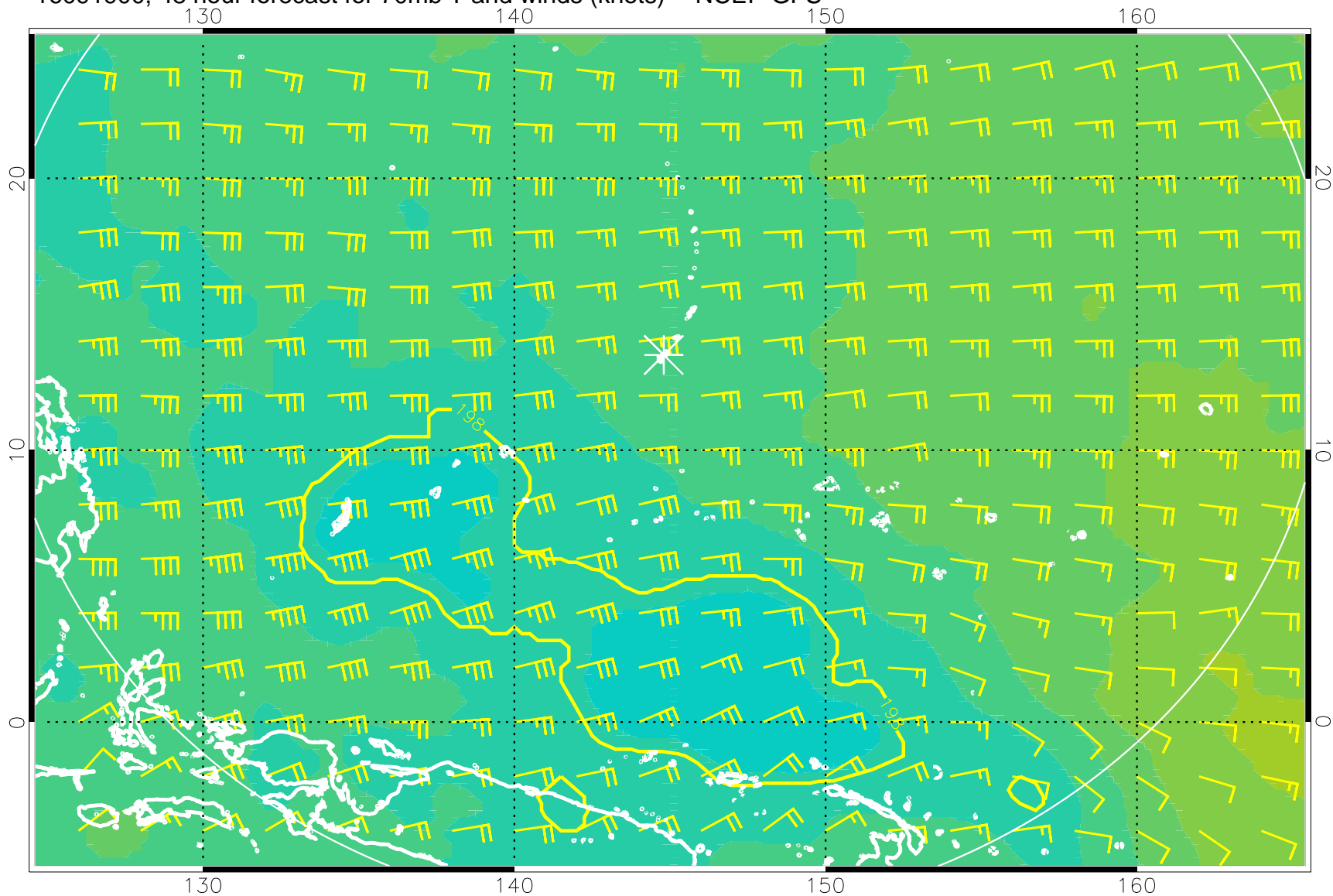
16091900, 48 hour forecast for 70mb T and winds (knots) -- NCEP GFS
