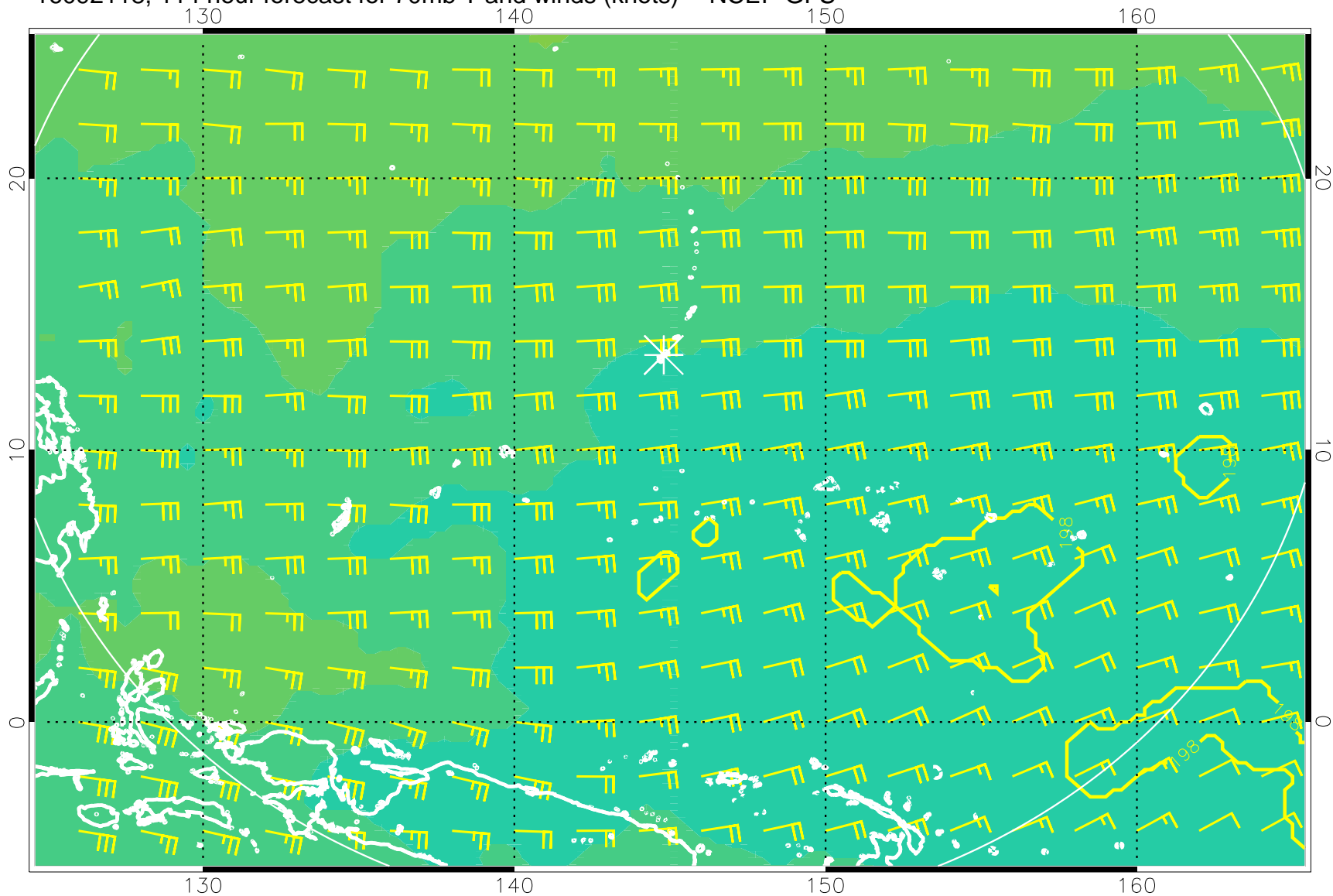
16092118, 114 hour forecast for 70mb T and winds (knots) -- NCEP GFS
