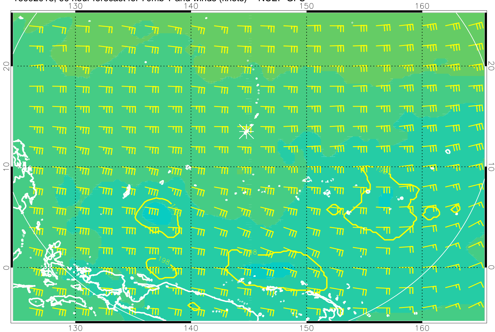
16092018, 90 hour forecast for 70mb T and winds (knots) -- NCEP GFS
