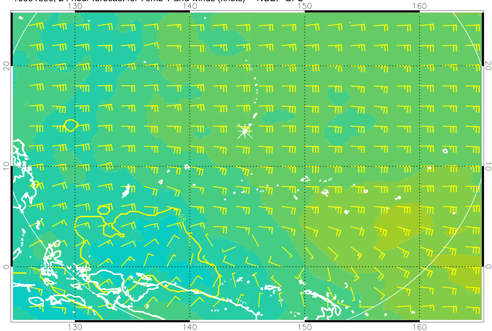
16091800, 24 hour forecast for 70mb T and winds (knots) -- NCEP GFS
