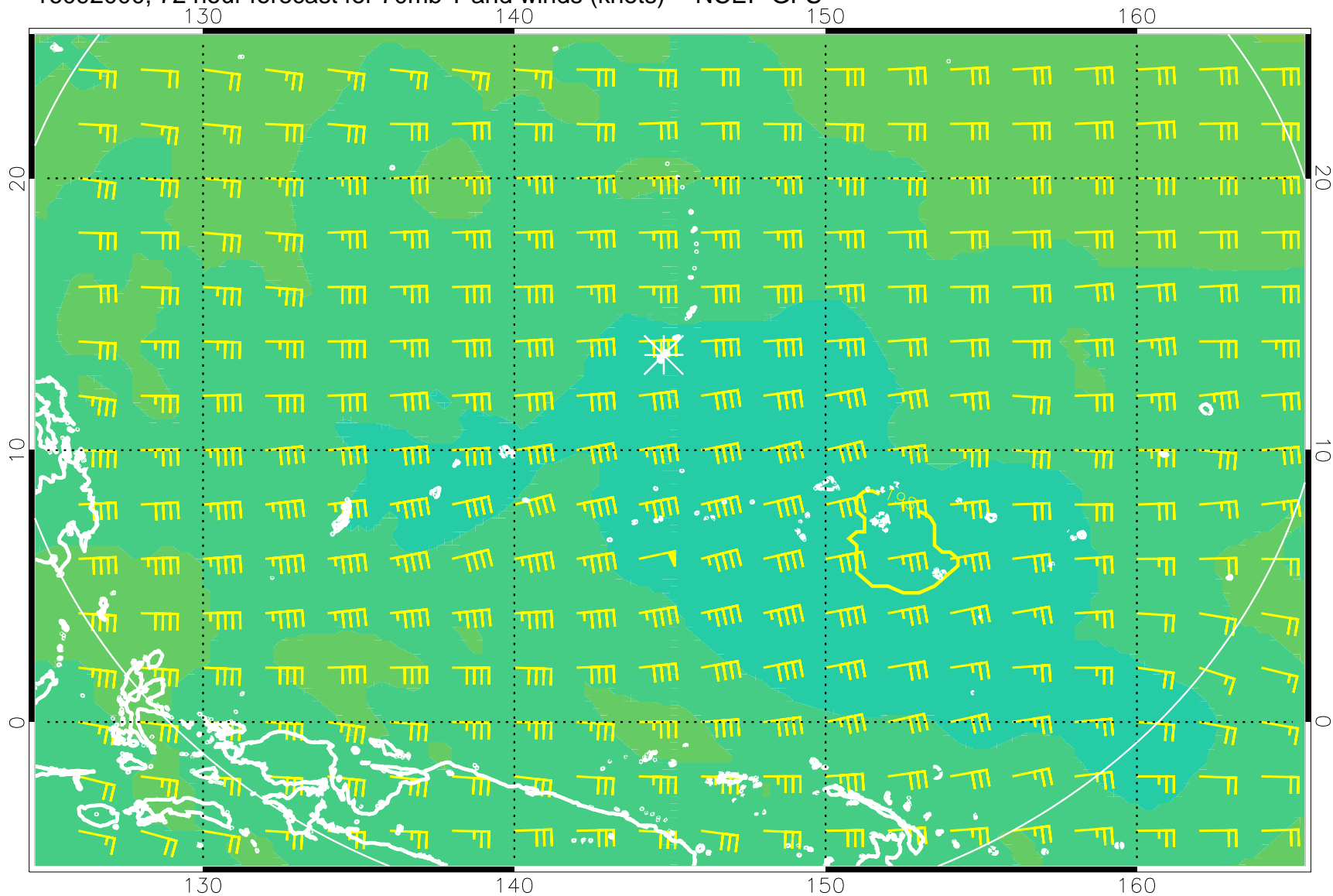
16092000, 72 hour forecast for 70mb T and winds (knots) -- NCEP GFS
