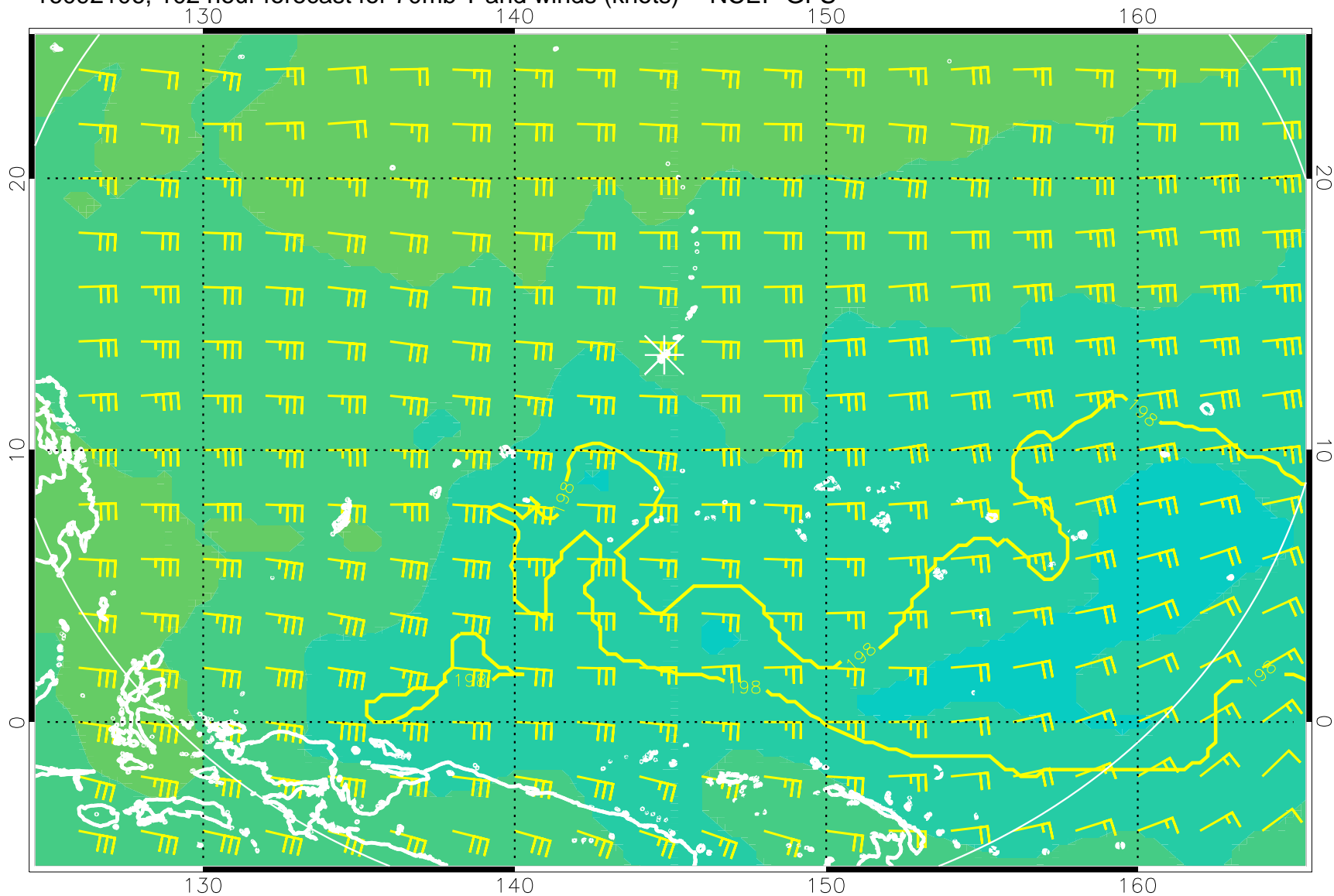
16092106, 102 hour forecast for 70mb T and winds (knots) -- NCEP GFS
