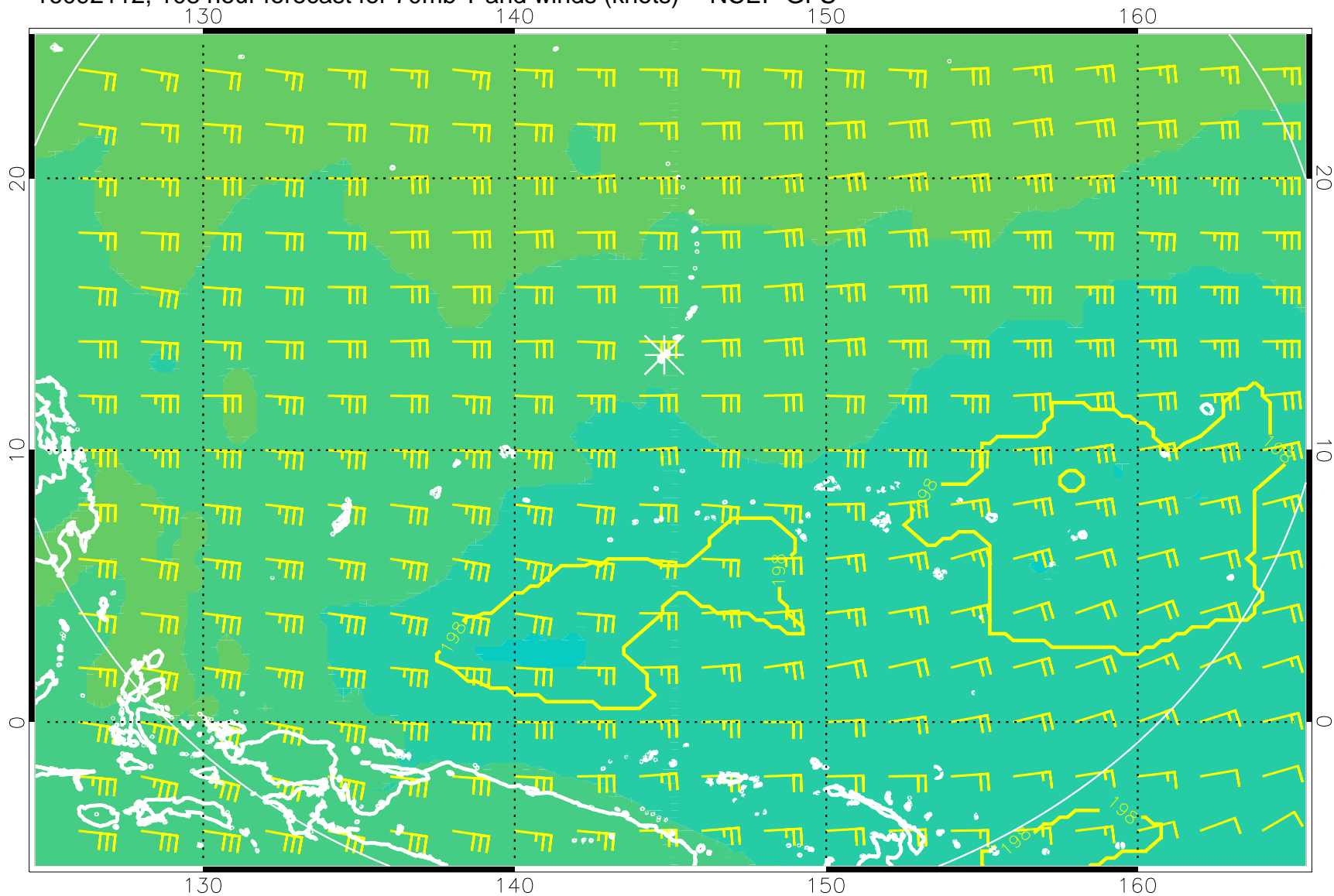
16092112, 108 hour forecast for 70mb T and winds (knots) -- NCEP GFS
