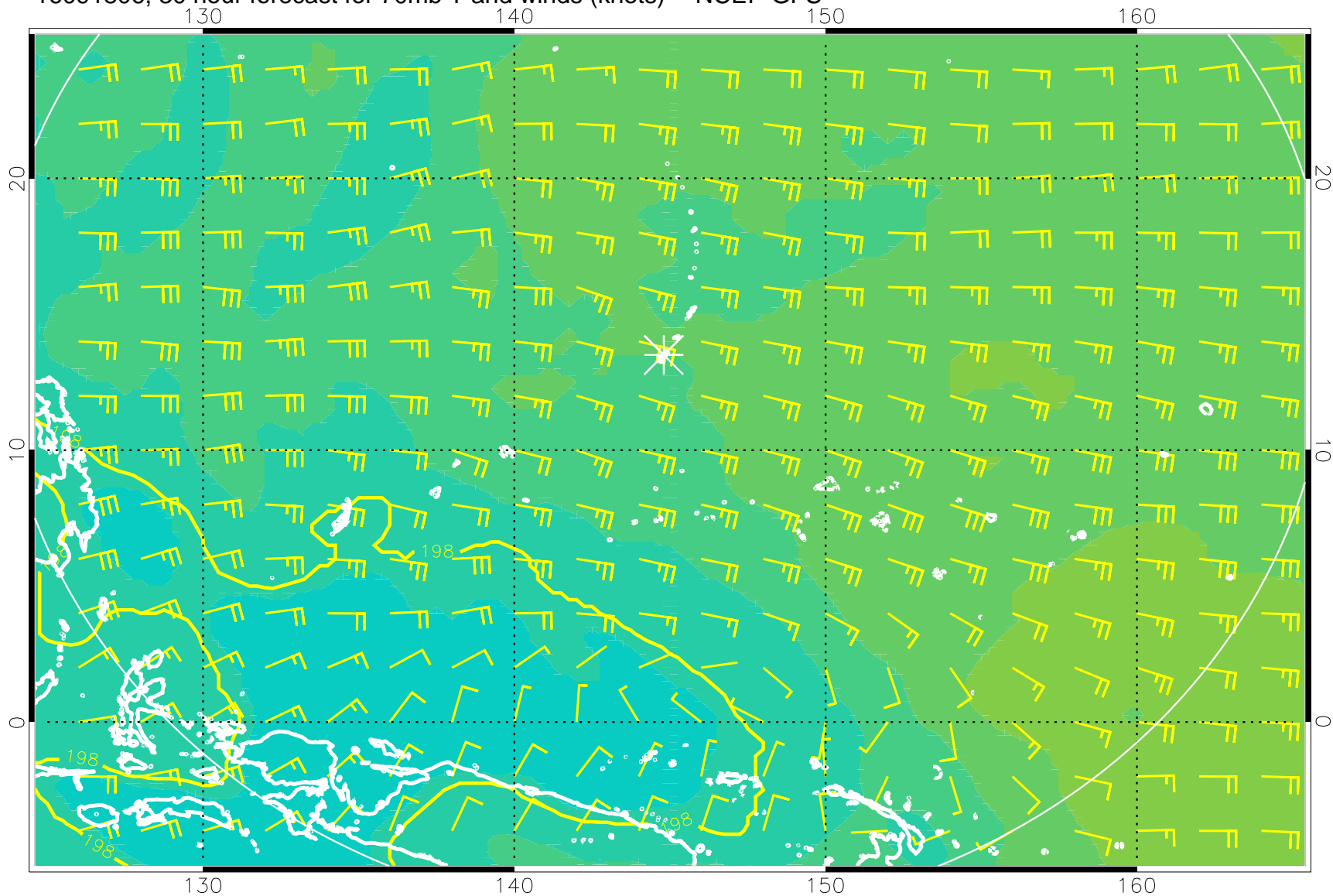
16091806, 30 hour forecast for 70mb T and winds (knots) -- NCEP GFS
