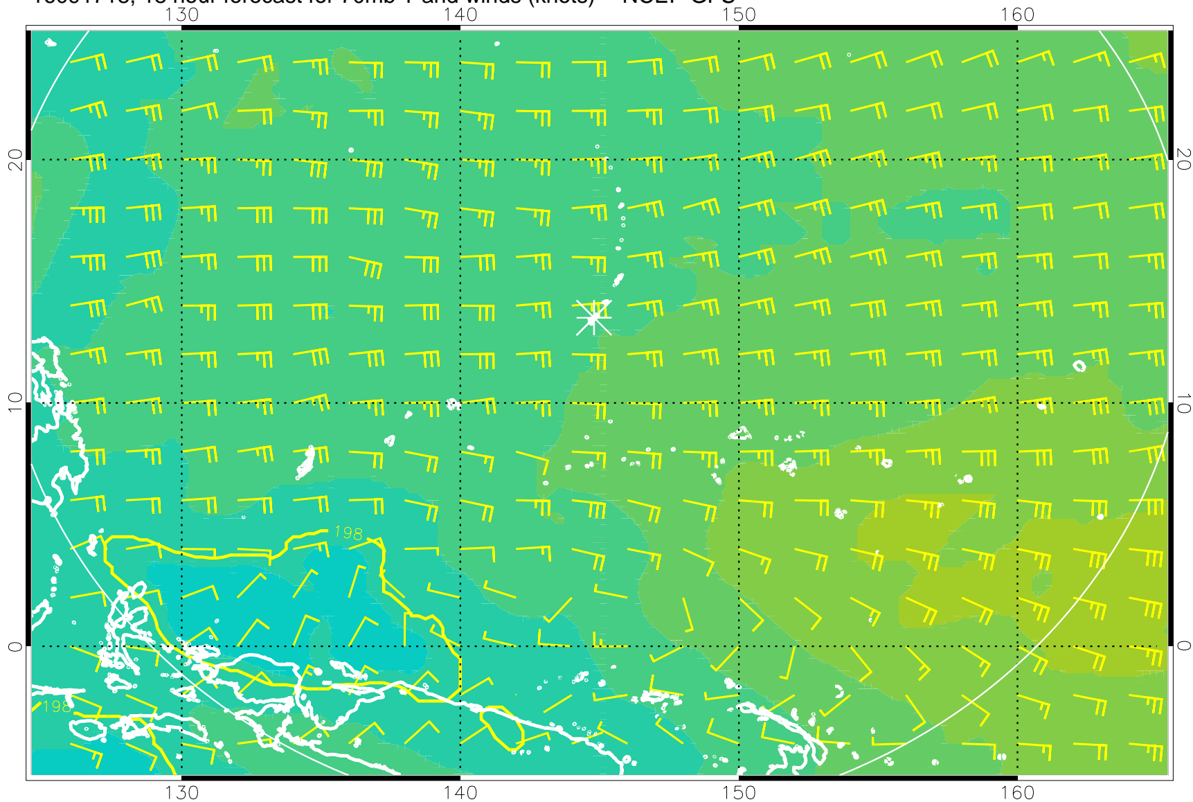
16091718, 18 hour forecast for 70mb T and winds (knots) -- NCEP GFS
