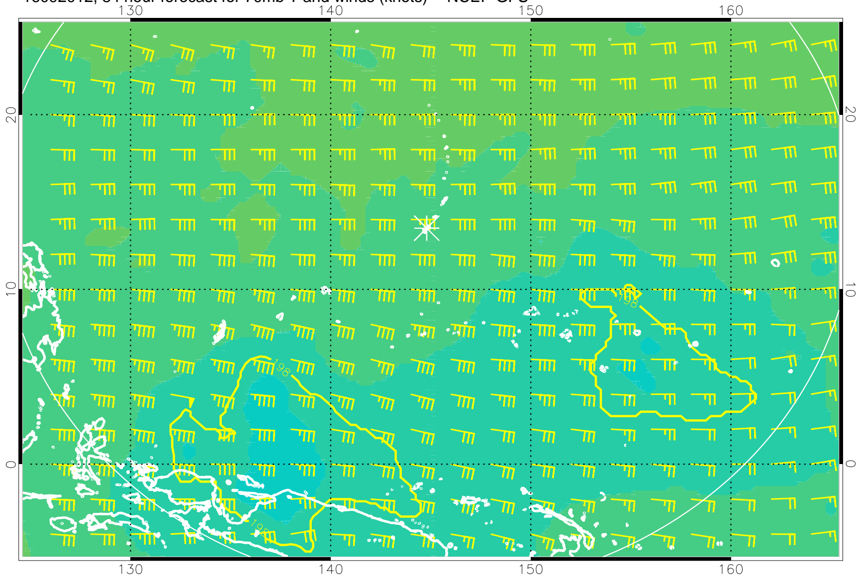
16092012, 84 hour forecast for 70mb T and winds (knots) -- NCEP GFS
