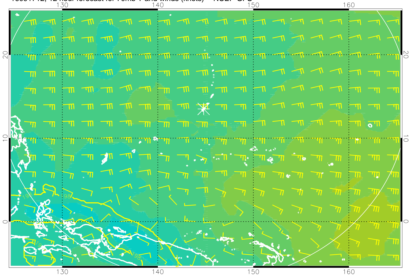
16091712, 12 hour forecast for 70mb T and winds (knots) -- NCEP GFS
