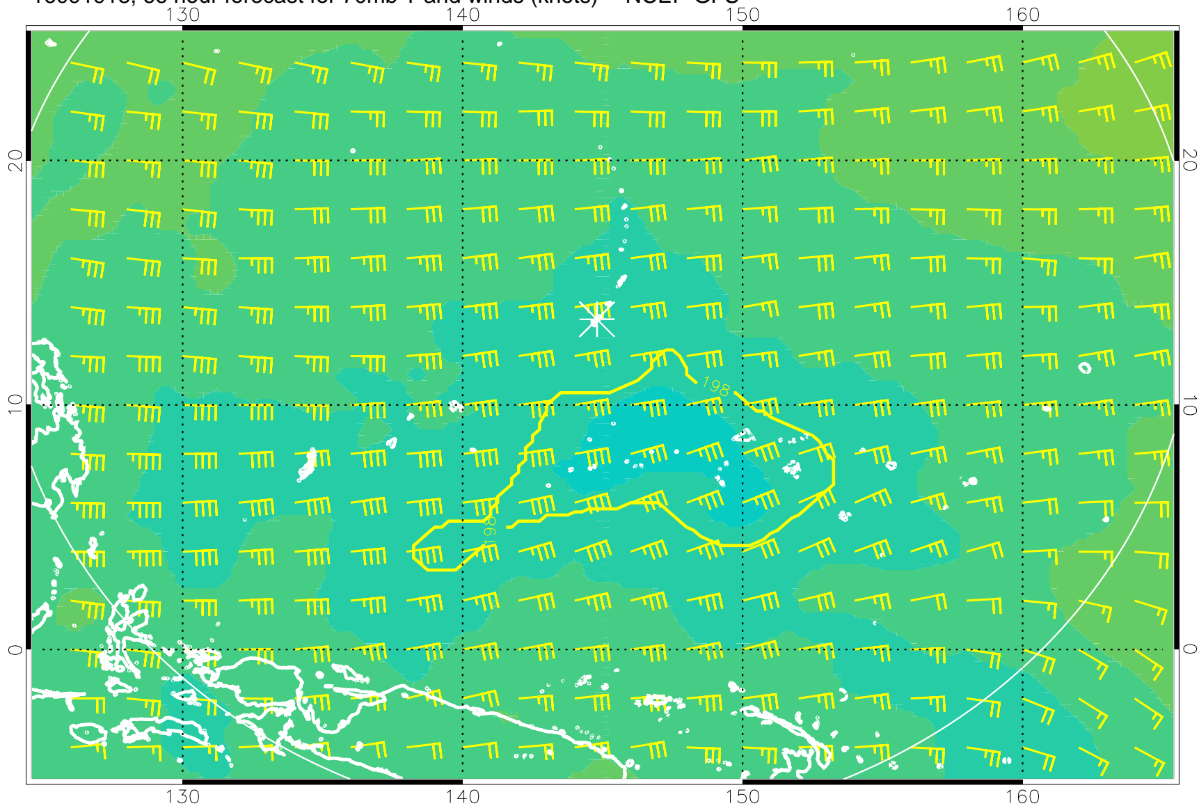
16091918, 66 hour forecast for 70mb T and winds (knots) -- NCEP GFS
