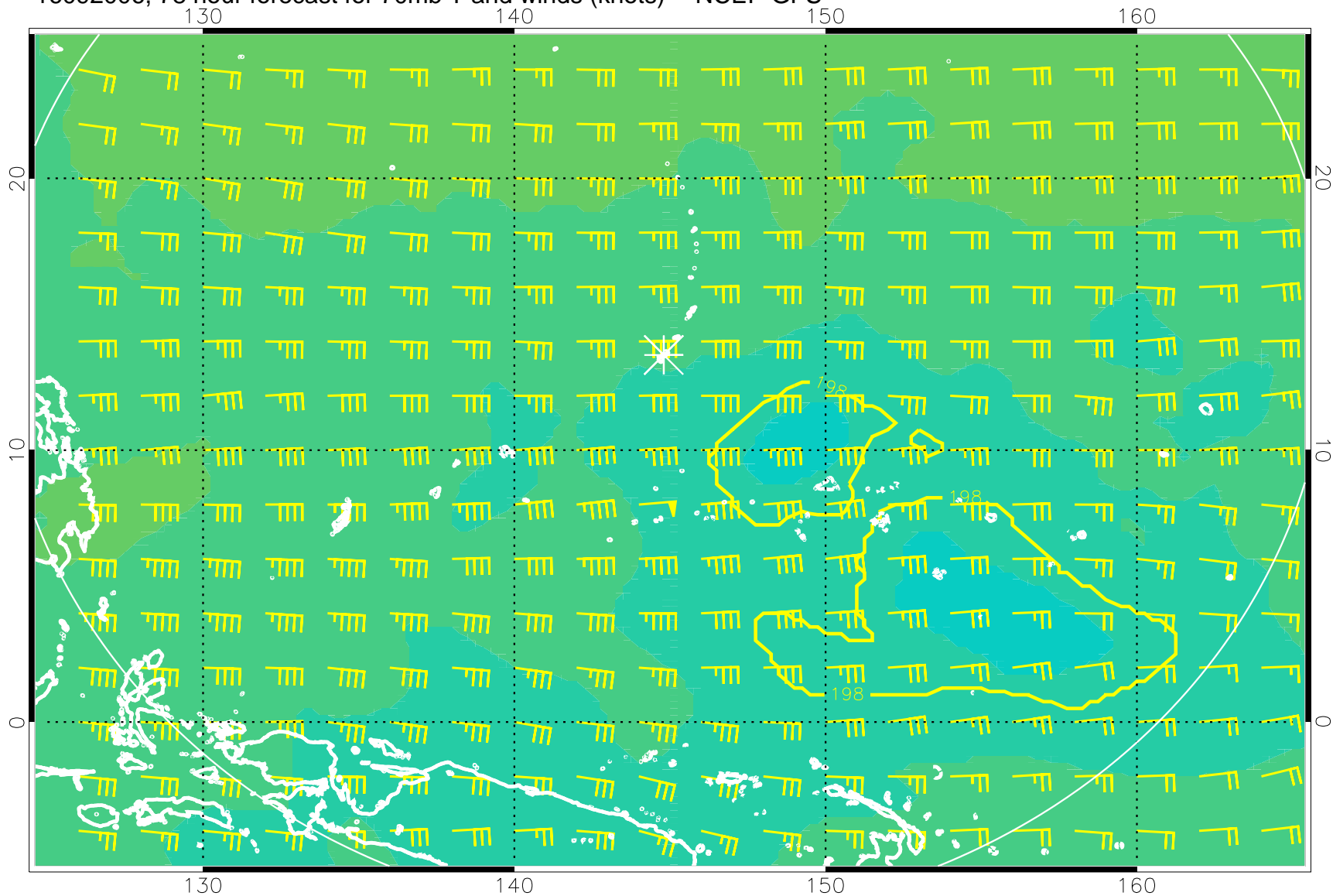
16092006, 78 hour forecast for 70mb T and winds (knots) -- NCEP GFS
