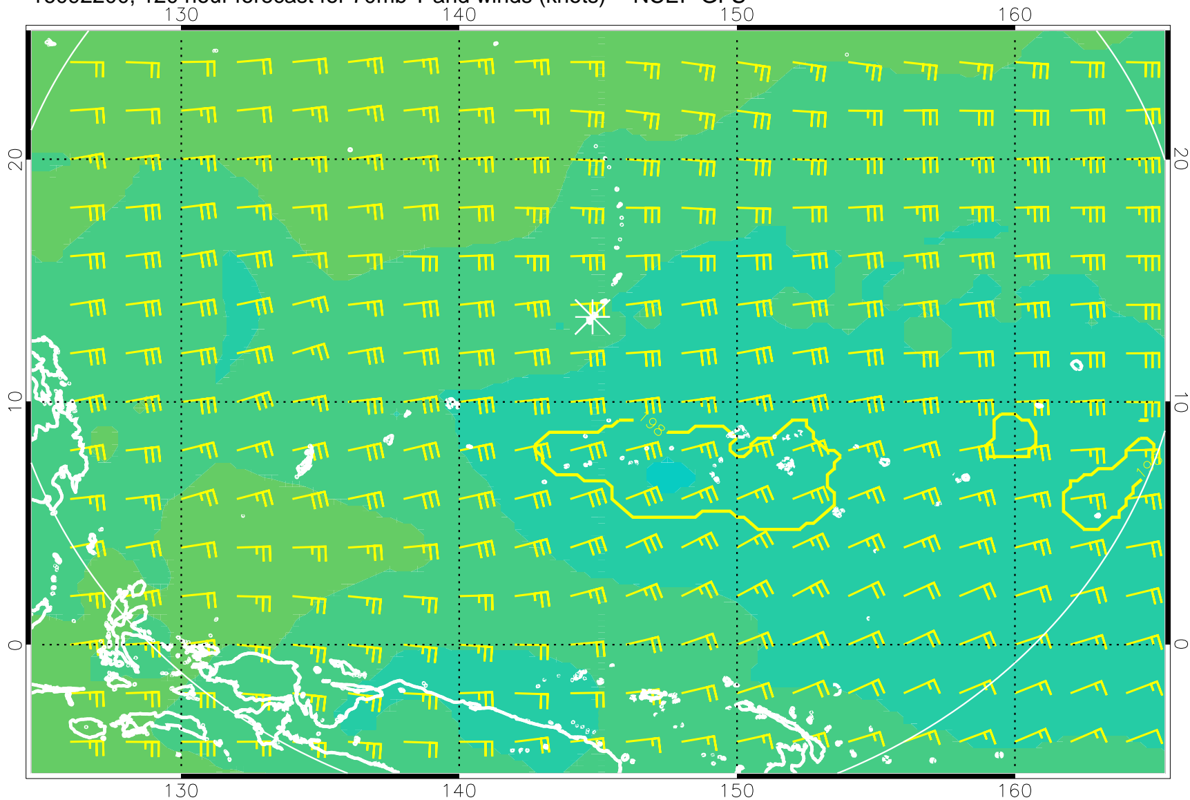
16092200, 120 hour forecast for 70mb T and winds (knots) -- NCEP GFS
