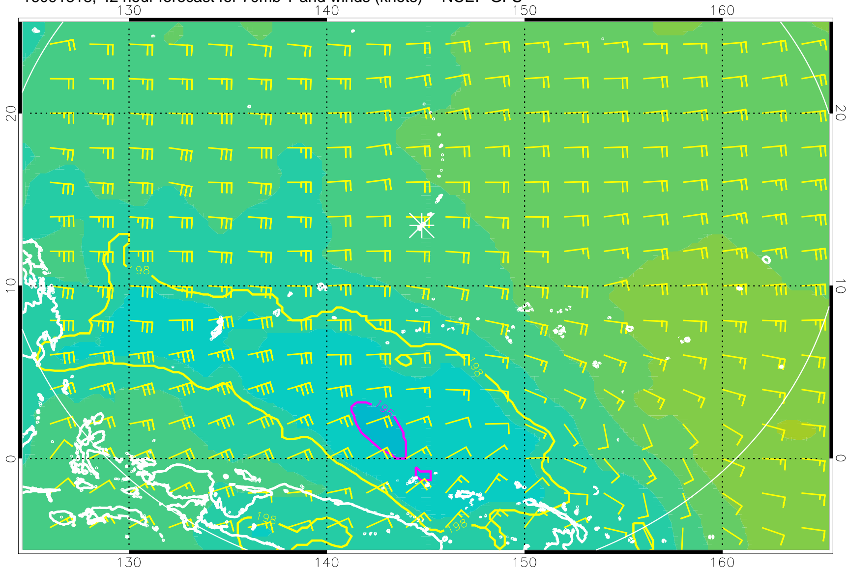
16091818, 42 hour forecast for 70mb T and winds (knots) -- NCEP GFS
