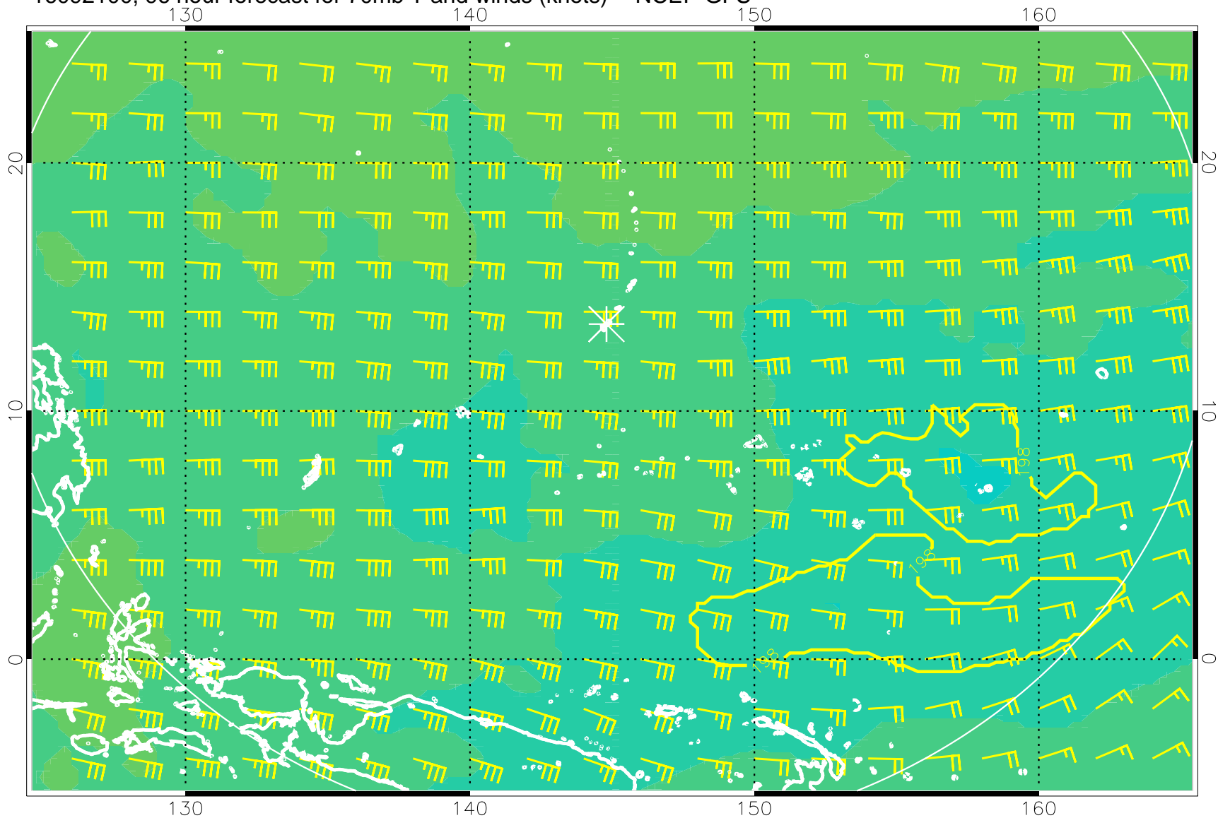
16092100, 96 hour forecast for 70mb T and winds (knots) -- NCEP GFS
