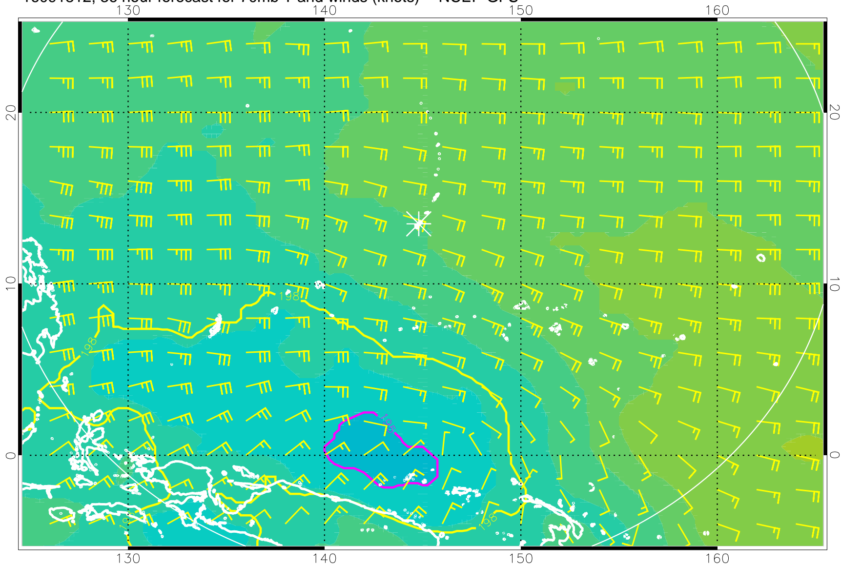
16091812, 36 hour forecast for 70mb T and winds (knots) -- NCEP GFS
