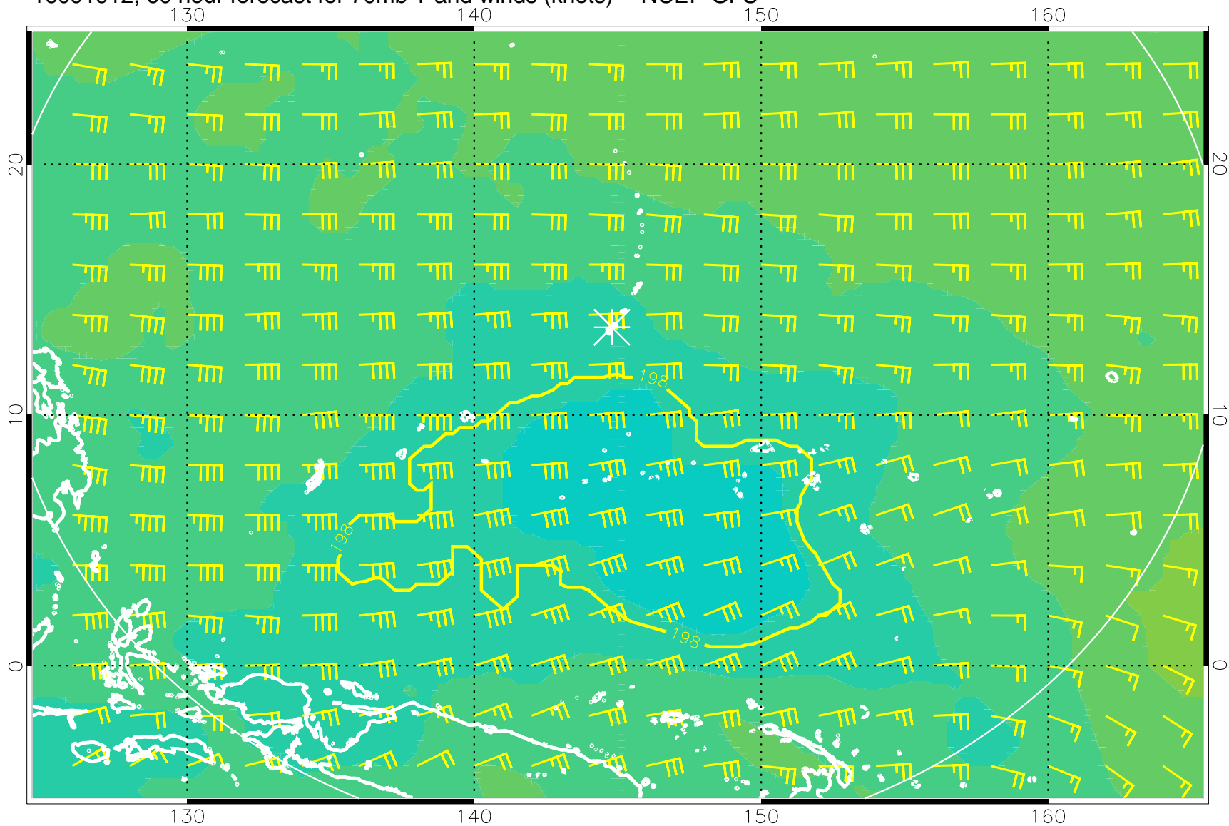
16091912, 60 hour forecast for 70mb T and winds (knots) -- NCEP GFS
