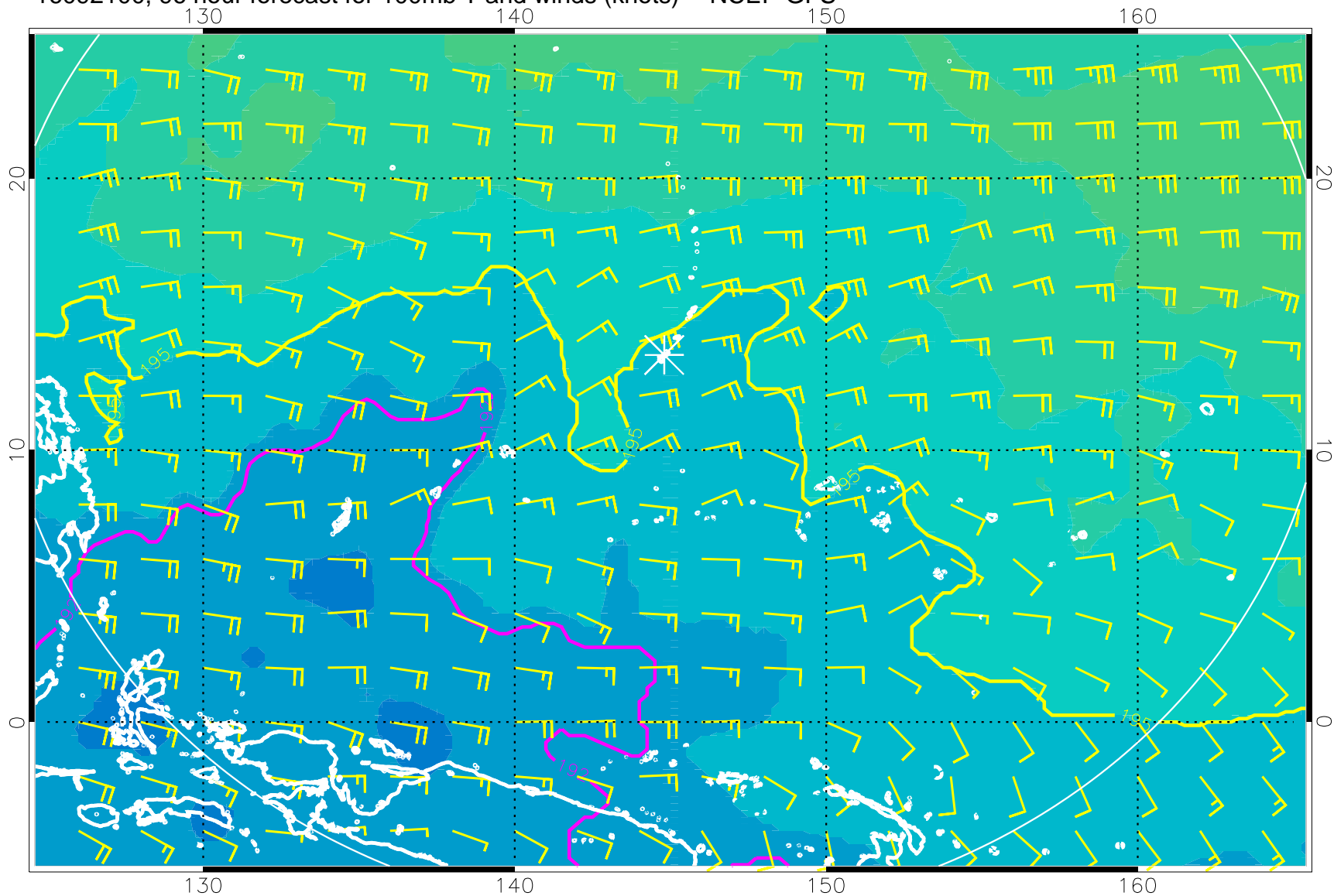
16092100, 96 hour forecast for 100mb T and winds (knots) -- NCEP GFS
