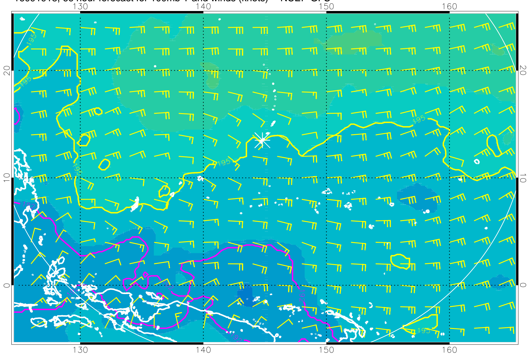
16091918, 66 hour forecast for 100mb T and winds (knots) -- NCEP GFS
