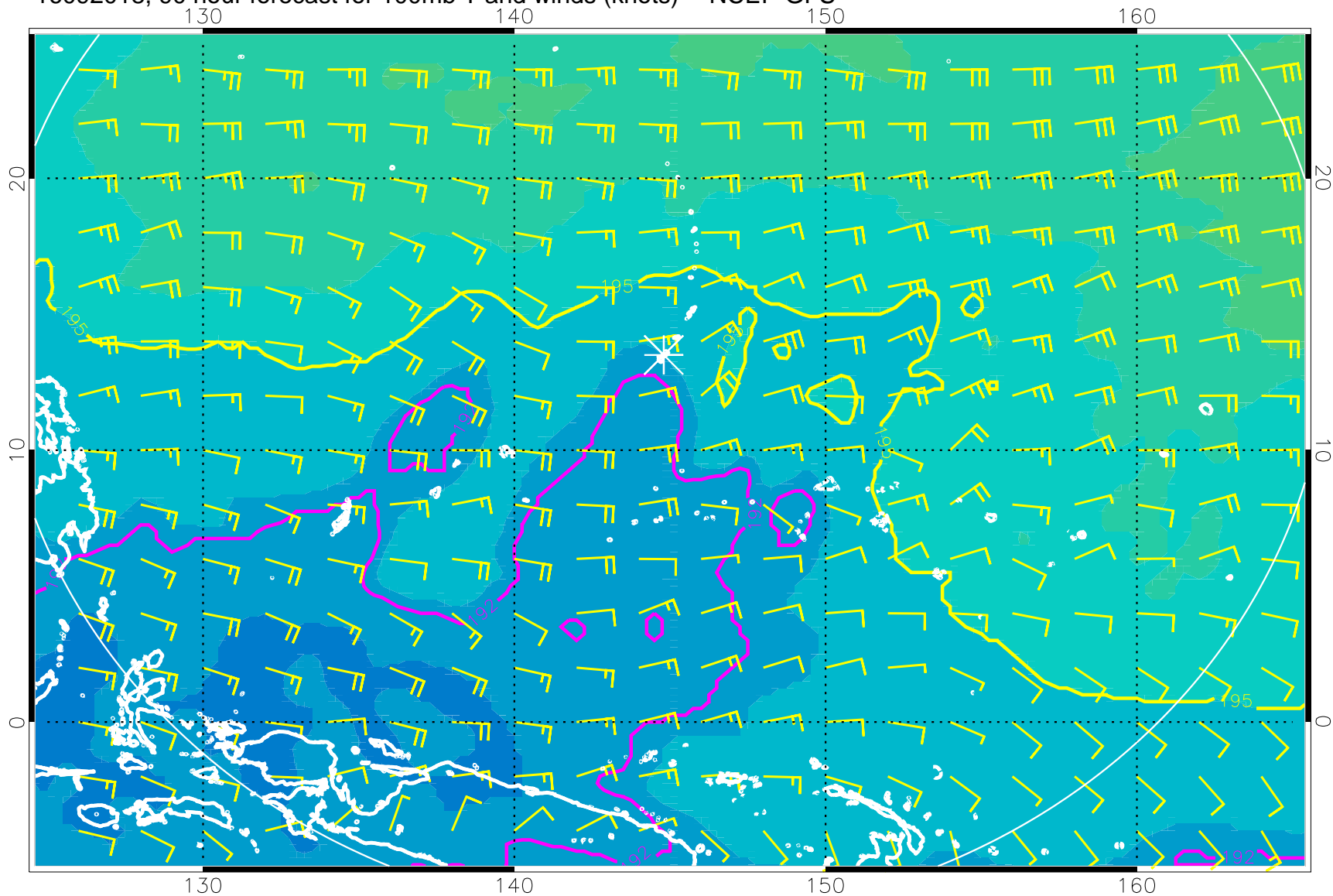
16092018, 90 hour forecast for 100mb T and winds (knots) -- NCEP GFS
