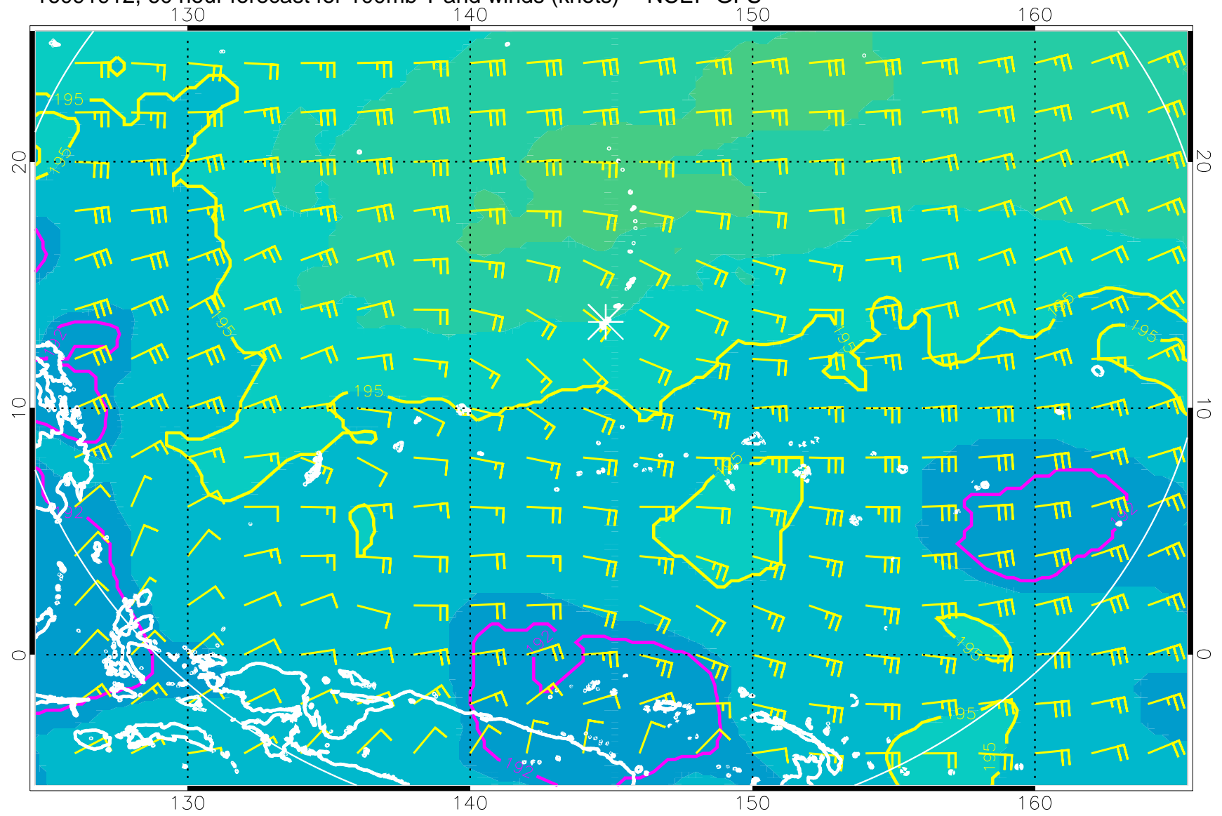
16091912, 60 hour forecast for 100mb T and winds (knots) -- NCEP GFS
