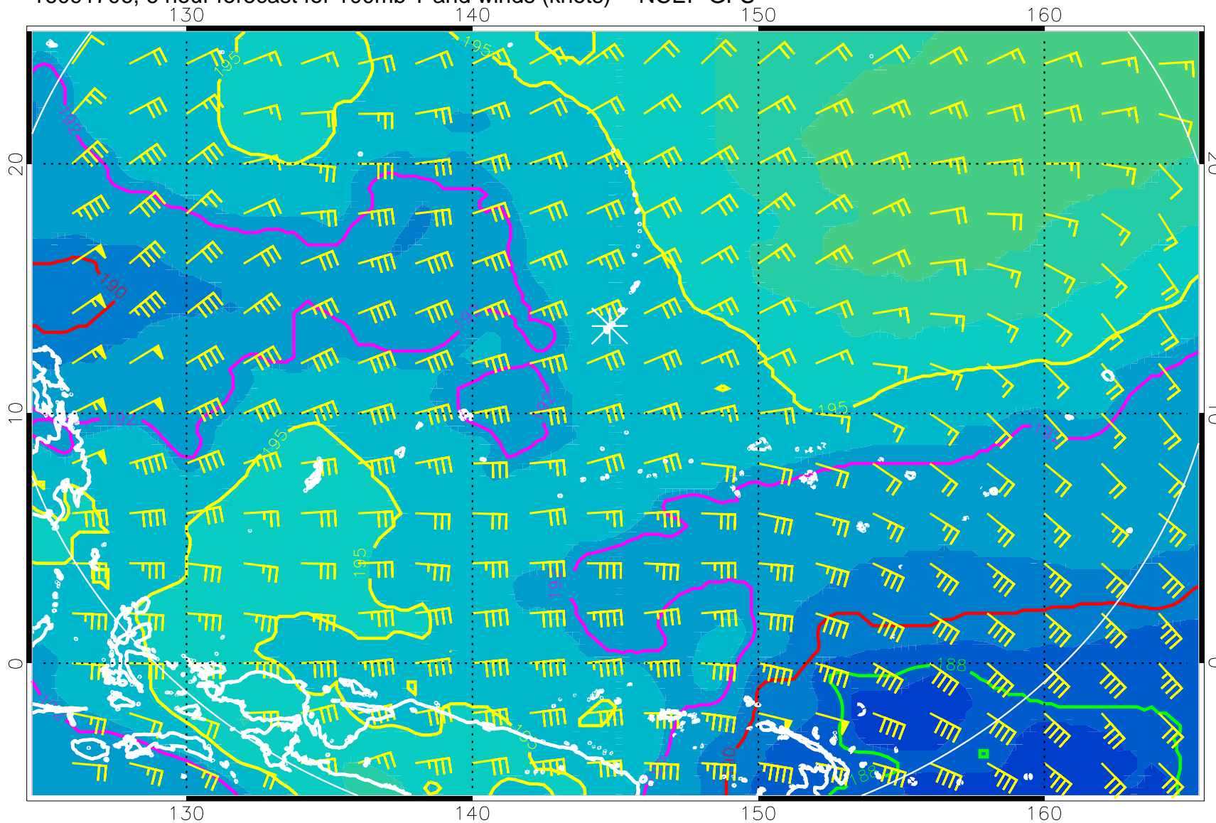
16091706, 6 hour forecast for 100mb T and winds (knots) -- NCEP GFS
