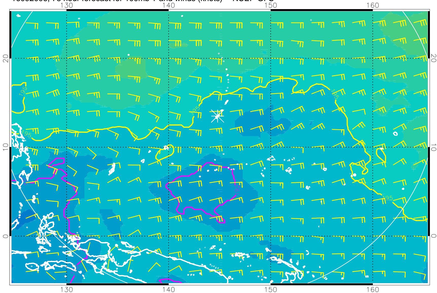
16092006, 78 hour forecast for 100mb T and winds (knots) -- NCEP GFS
