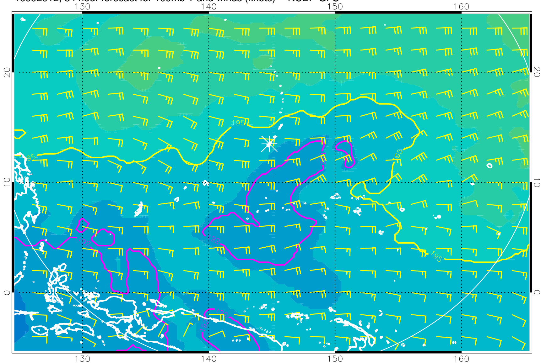
16092012, 84 hour forecast for 100mb T and winds (knots) -- NCEP GFS
