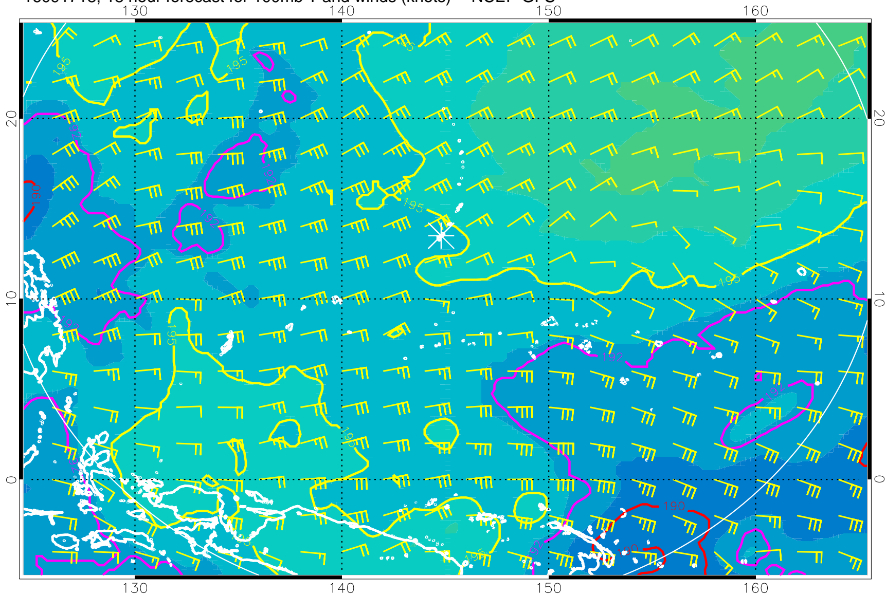
16091718, 18 hour forecast for 100mb T and winds (knots) -- NCEP GFS
