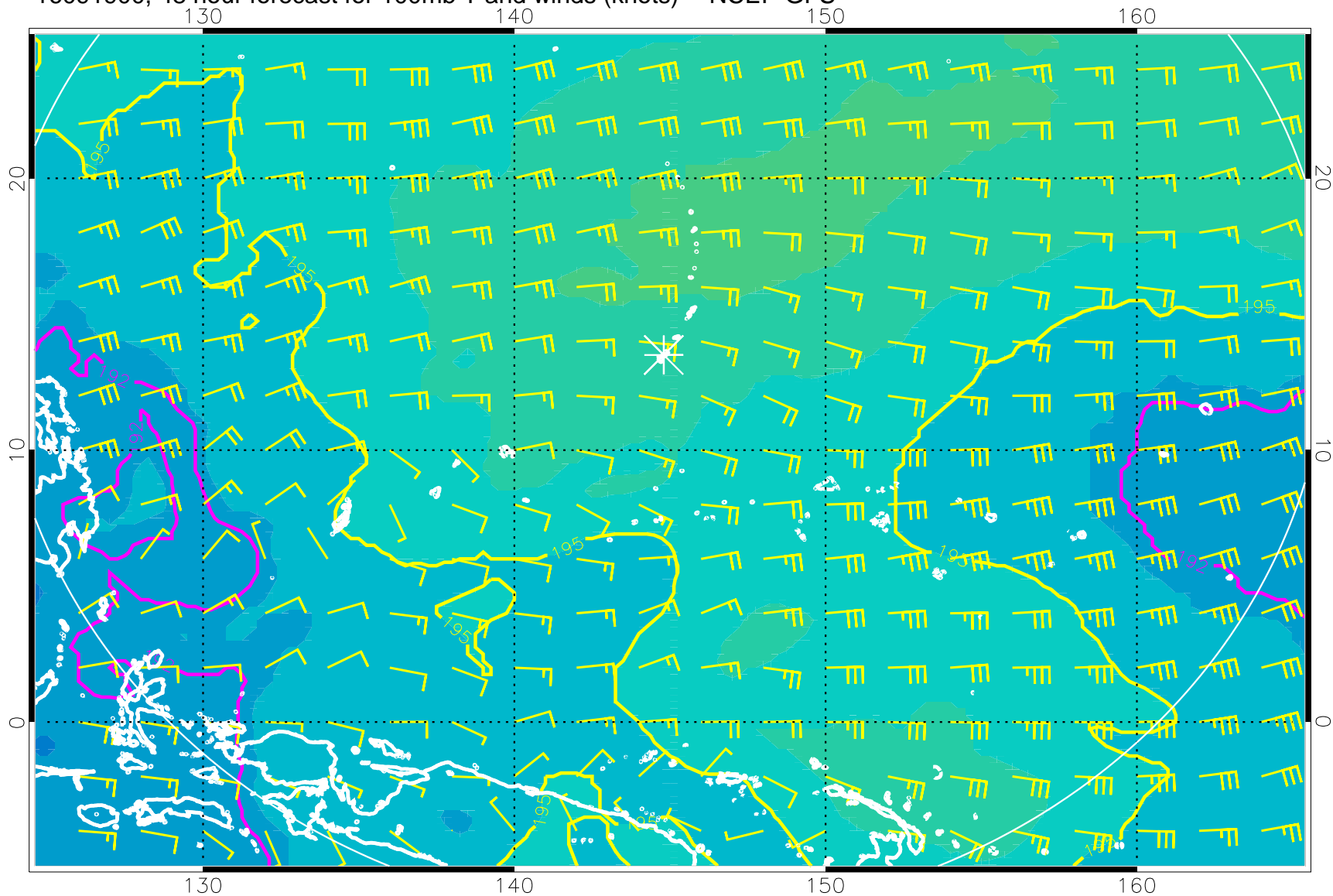
16091900, 48 hour forecast for 100mb T and winds (knots) -- NCEP GFS
