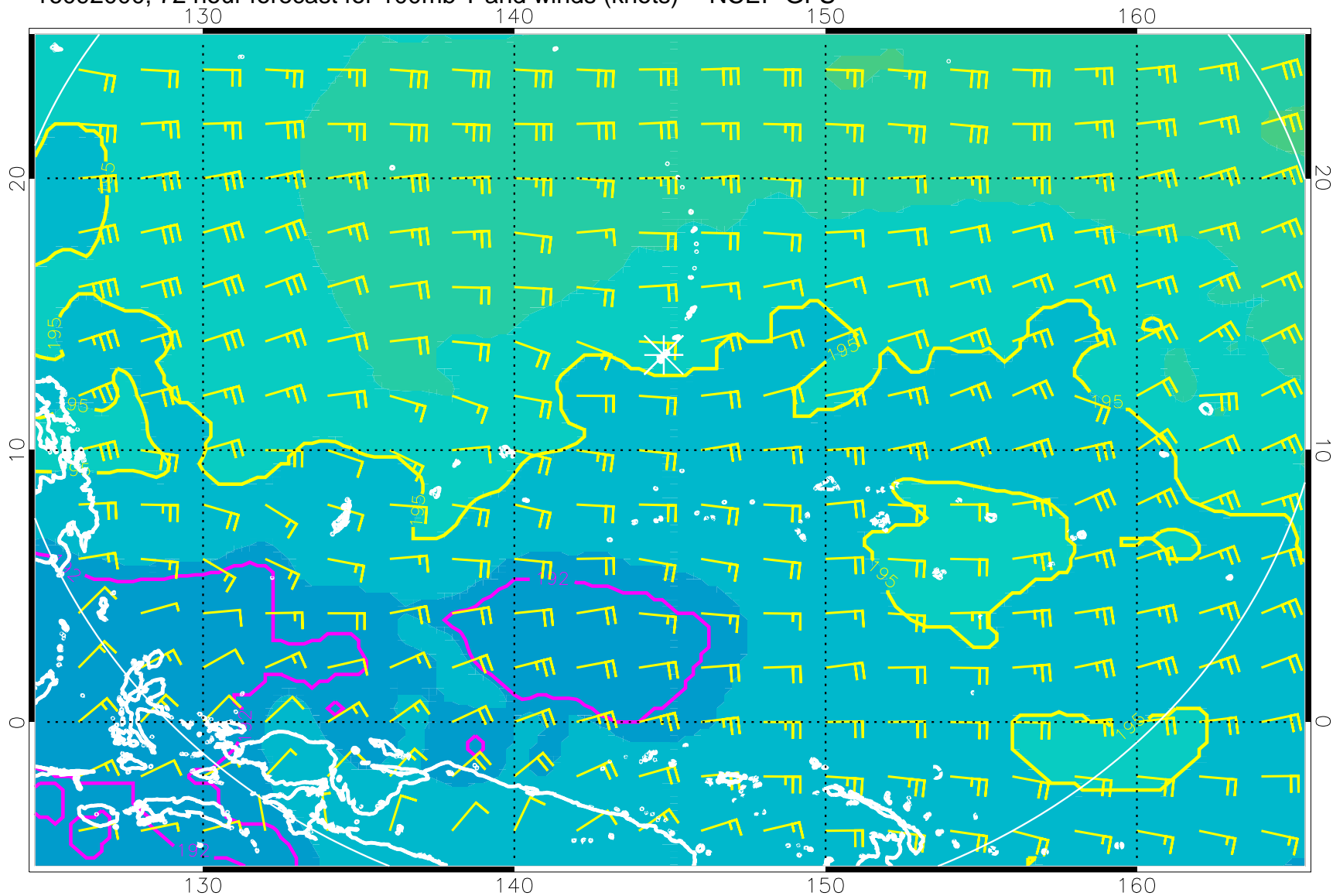
16092000, 72 hour forecast for 100mb T and winds (knots) -- NCEP GFS
