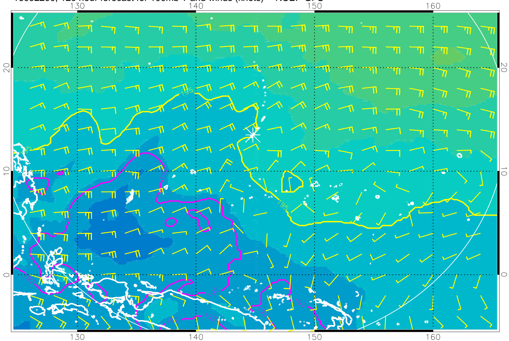
16092200, 120 hour forecast for 100mb T and winds (knots) -- NCEP GFS
