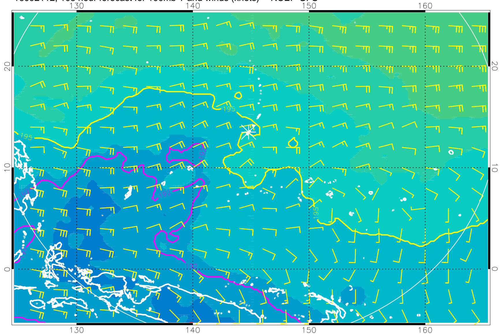
16092112, 108 hour forecast for 100mb T and winds (knots) -- NCEP GFS
