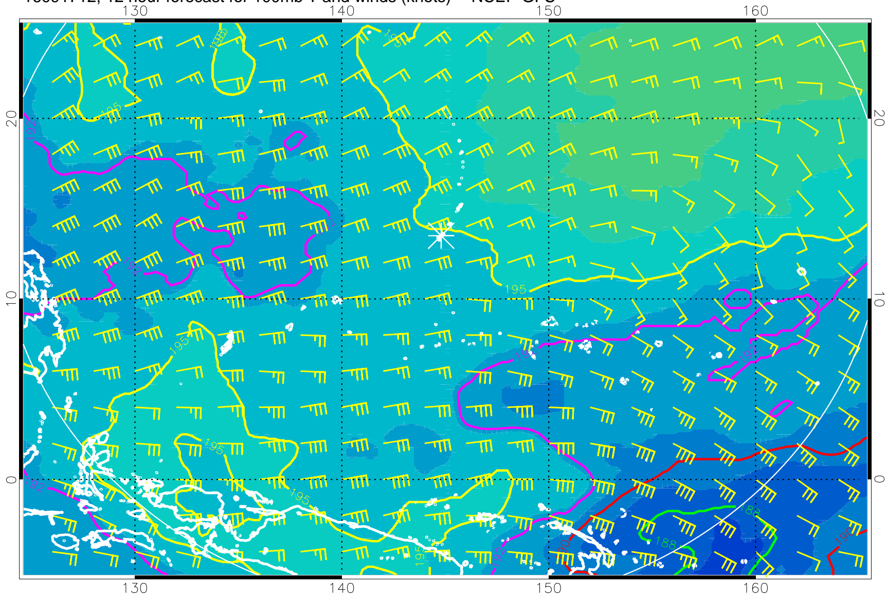
16091712, 12 hour forecast for 100mb T and winds (knots) -- NCEP GFS
