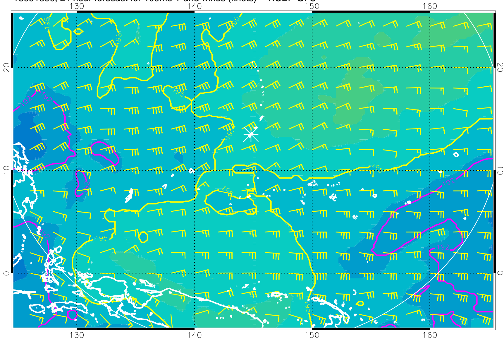
16091800, 24 hour forecast for 100mb T and winds (knots) -- NCEP GFS
