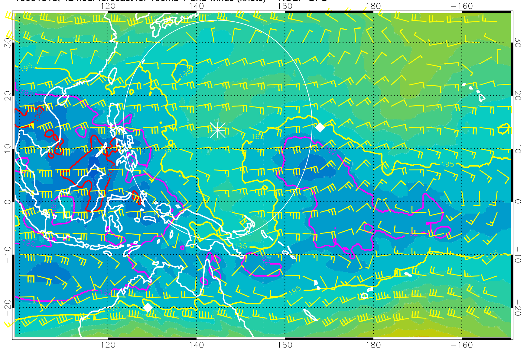
16091818, 42 hour forecast for 100mb T and winds (knots) -- NCEP GFS
