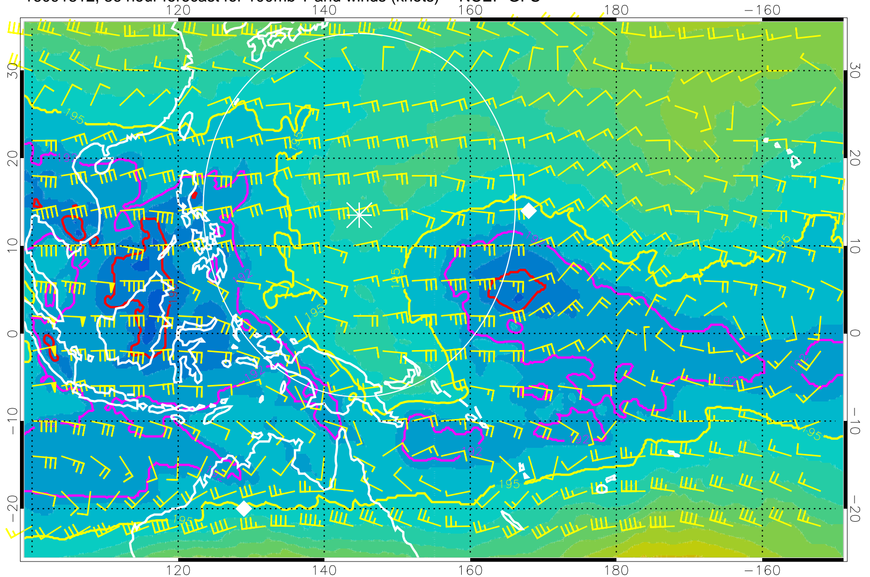
16091812, 36 hour forecast for 100mb T and winds (knots) -- NCEP GFS
