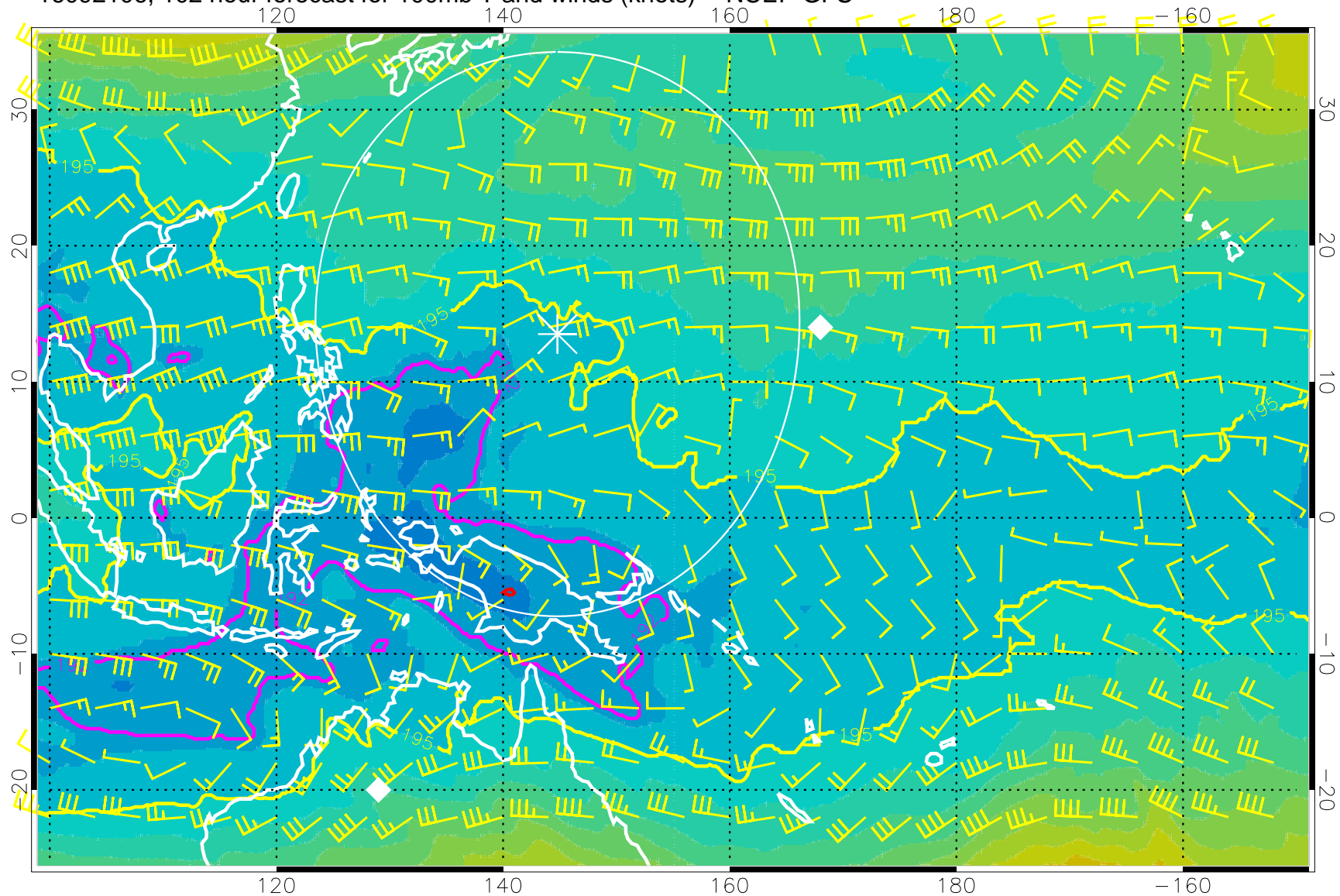
16092106, 102 hour forecast for 100mb T and winds (knots) -- NCEP GFS
