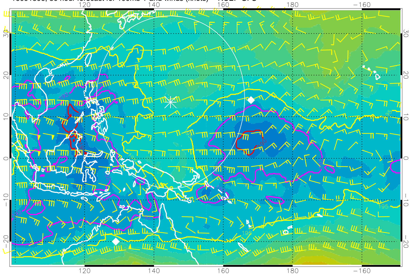
16091806, 30 hour forecast for 100mb T and winds (knots) -- NCEP GFS
